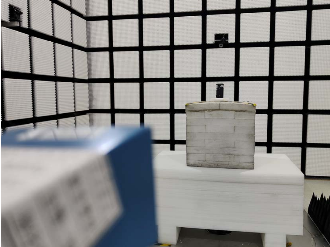
Radiated Emission 26.5GHz~40GHz View
