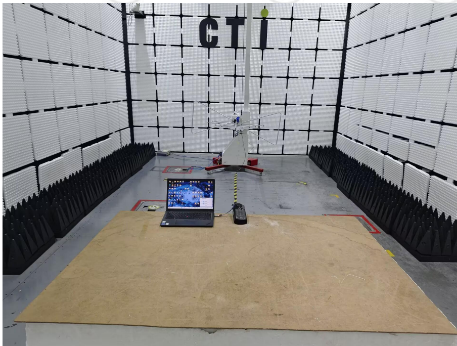
Radiated spurious emission Test Setup-1(30MHz to 1GHz)
