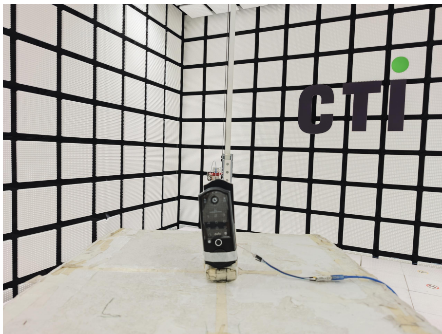
Radiated spurious emission Test Setup-3(18GHz to 41GHz)
