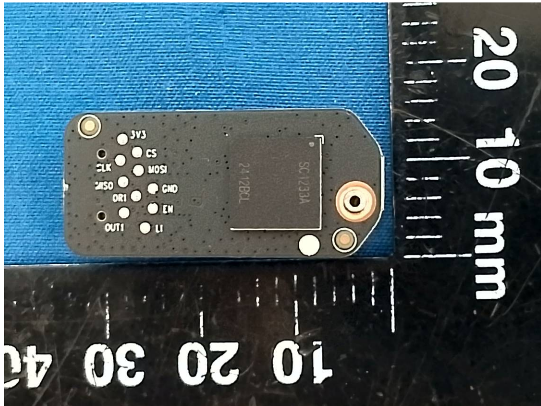
Radar Chip&Antenna
