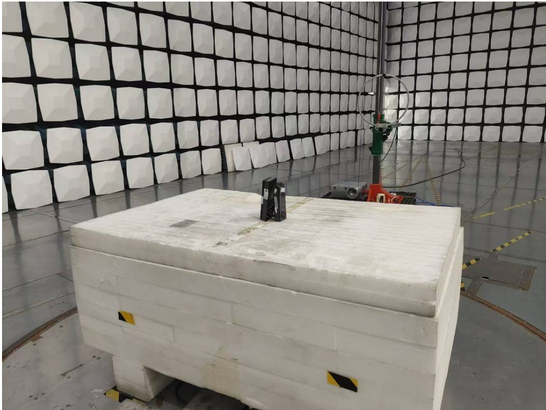
Radiated Emission 9k-30MHz Perpendicular View-T85V0
