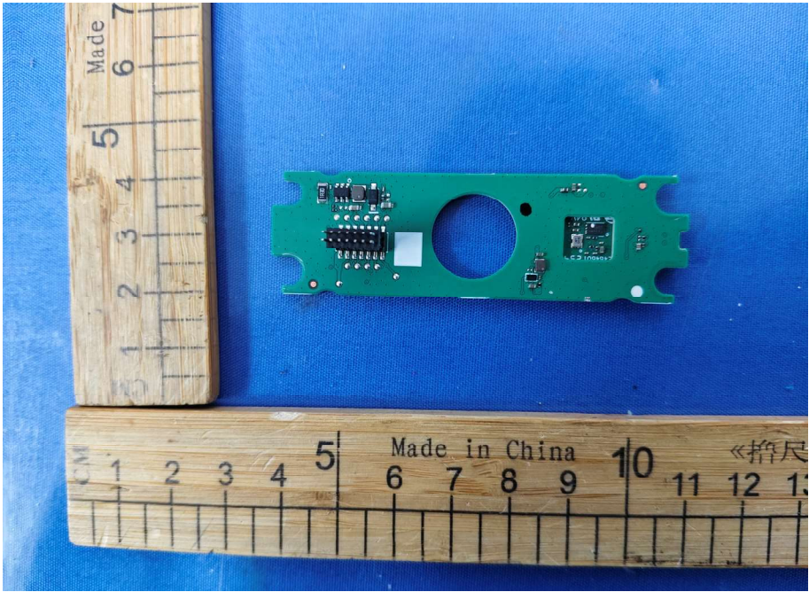
BT/WIFI Antenna Location Diagram
