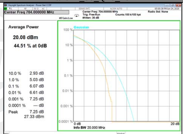
Band12_50_QPSK_Middle
