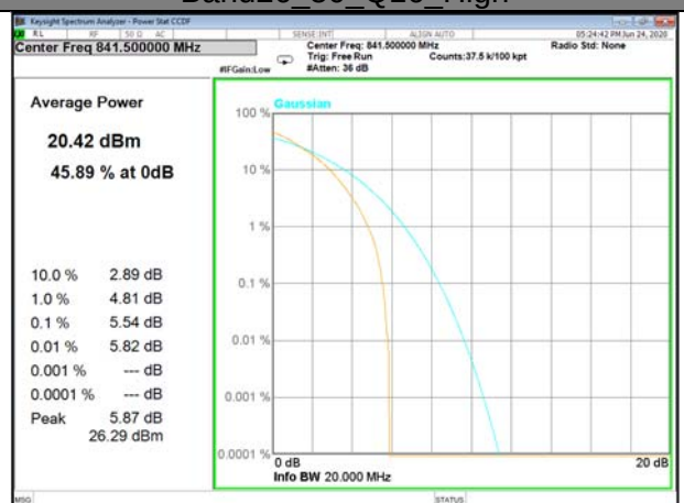
Band26_50_Q16_High
