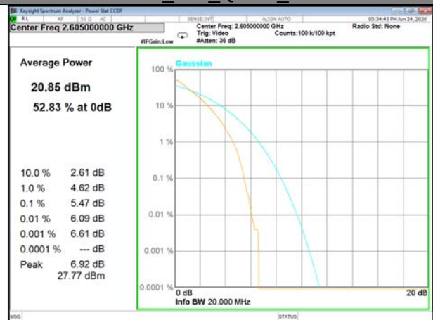
Band41_100_QPSK_Middle
