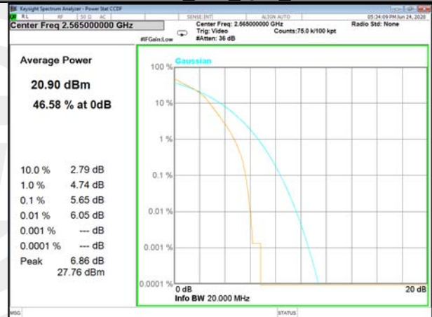
Band41_100_QPSK_Middle
