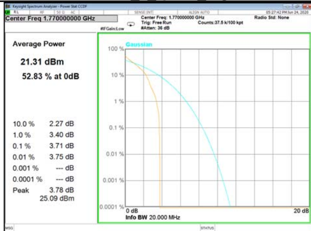
Band66_1_Q16_High
