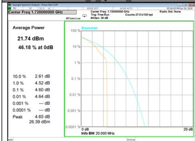
Band66_1_Q16_Low
