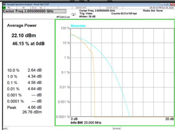
Band41_1_QPSK_Middle
