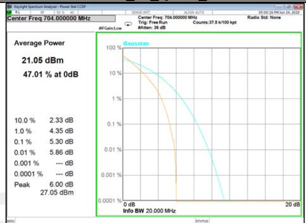
Band12_50_Q16_Low
