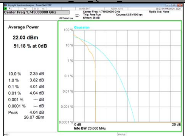
Band66_100_QPSK_Middle
