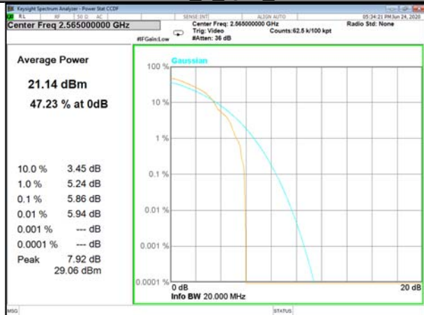
Band41_1_QPSK_Middle
