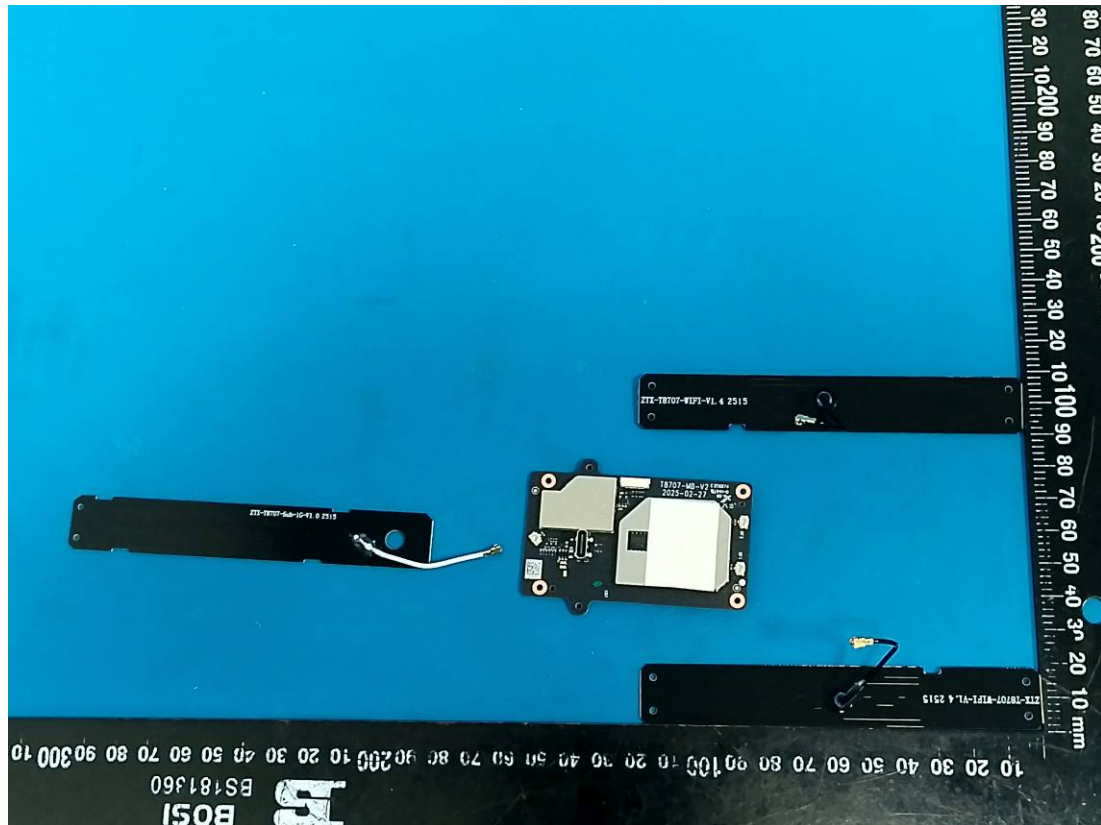
2.4G/5G SRD Antenna
