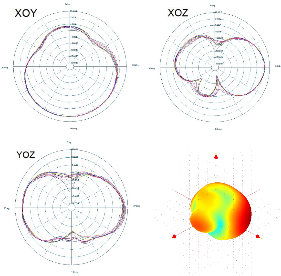
WIFI1:2.4G direction diagram
