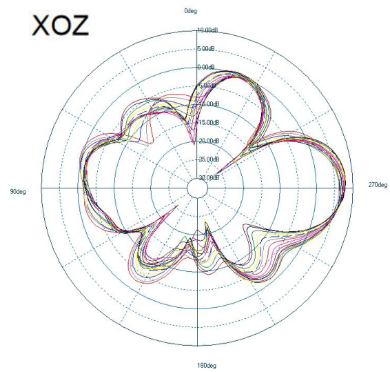
WIFI11:5G direction diagram
