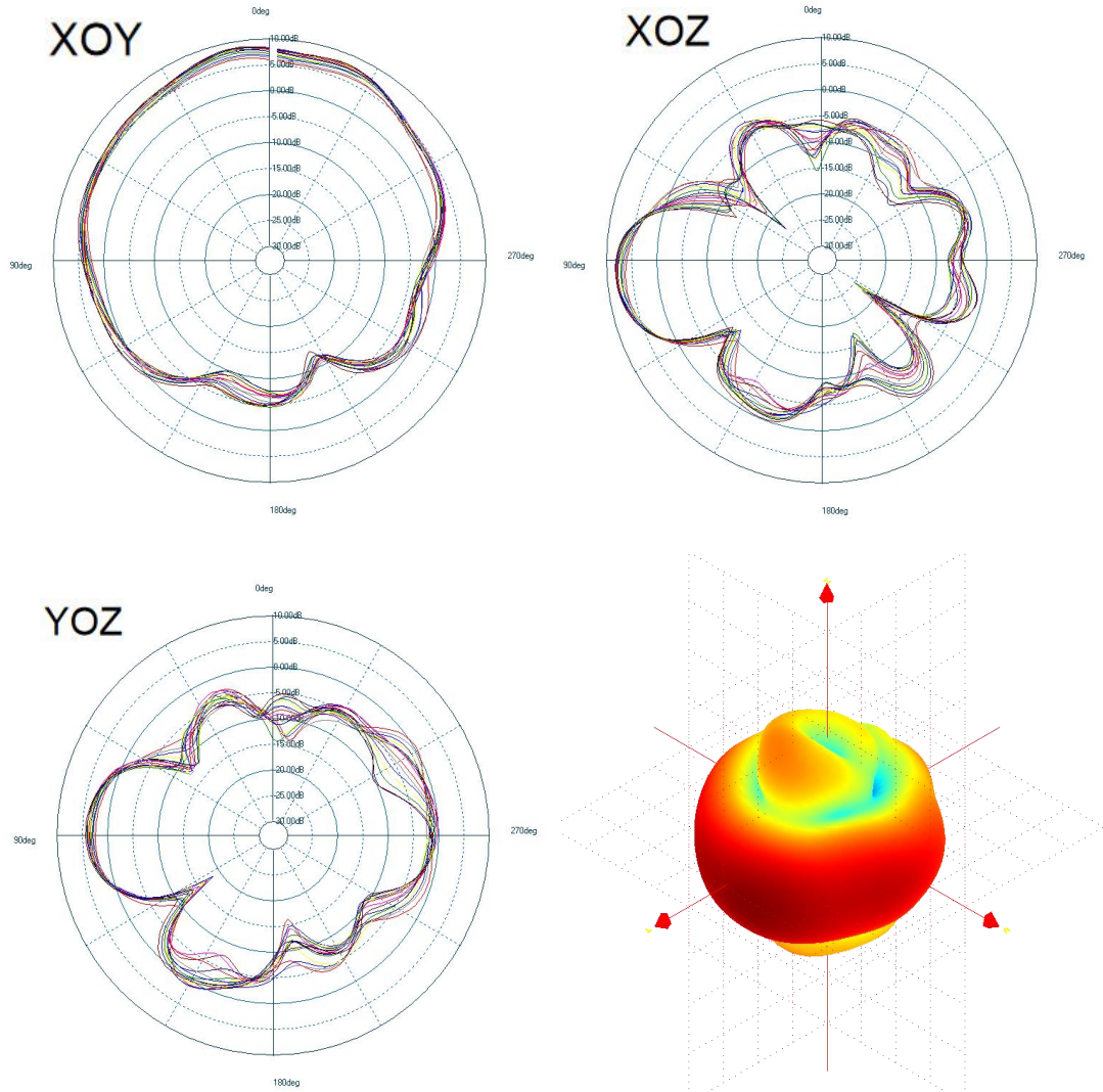
WIFI2: 5G direction diagram
