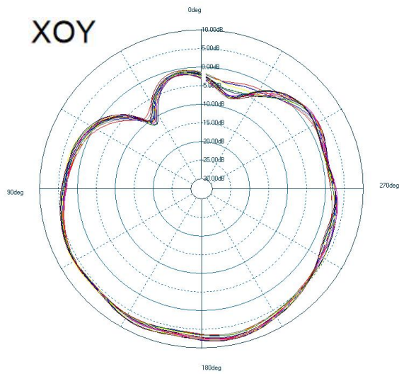
WIFI11:5G direction diagram
