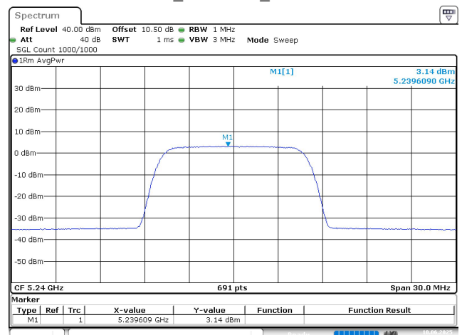
10M_5240MHz_Chain 1
