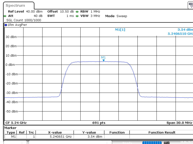
10M_5240MHz_Chain 0
