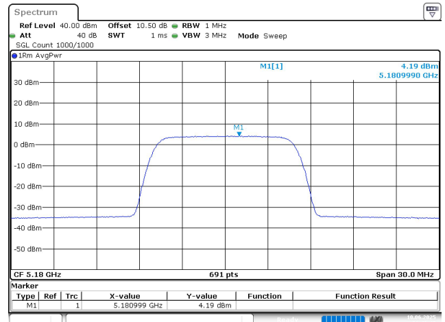
10M_5180MHz_Chain 1
