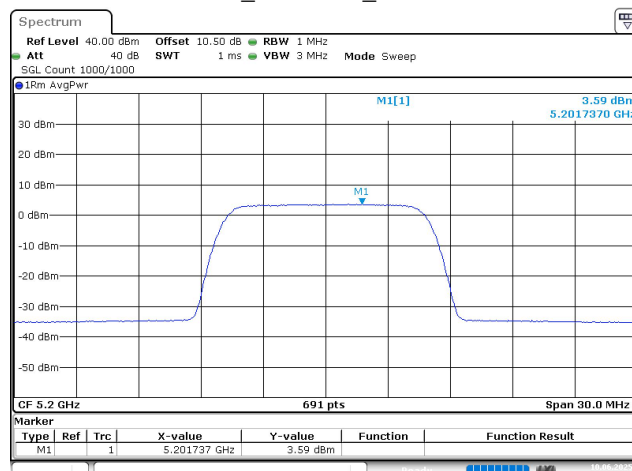
10M_5200MHz_Chain 1
