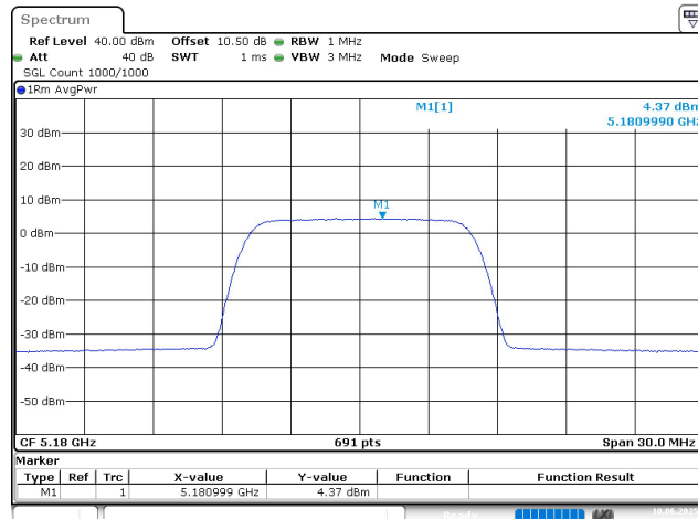
10M_5180MHz_Chain 0
