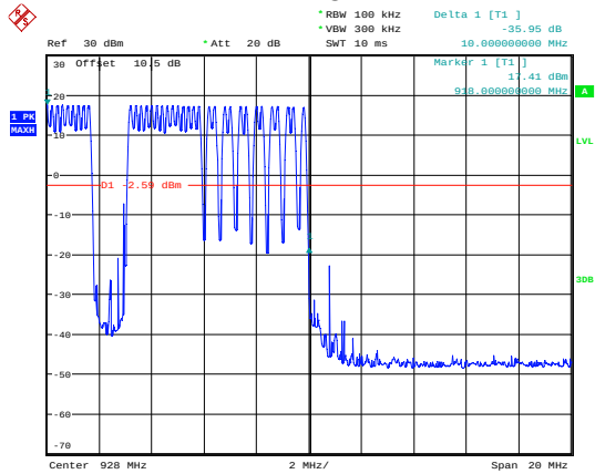
Hopping_Highest Channel
