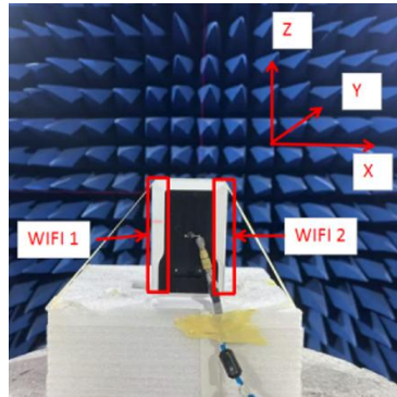
WIFI1:2.4G direction diagram
