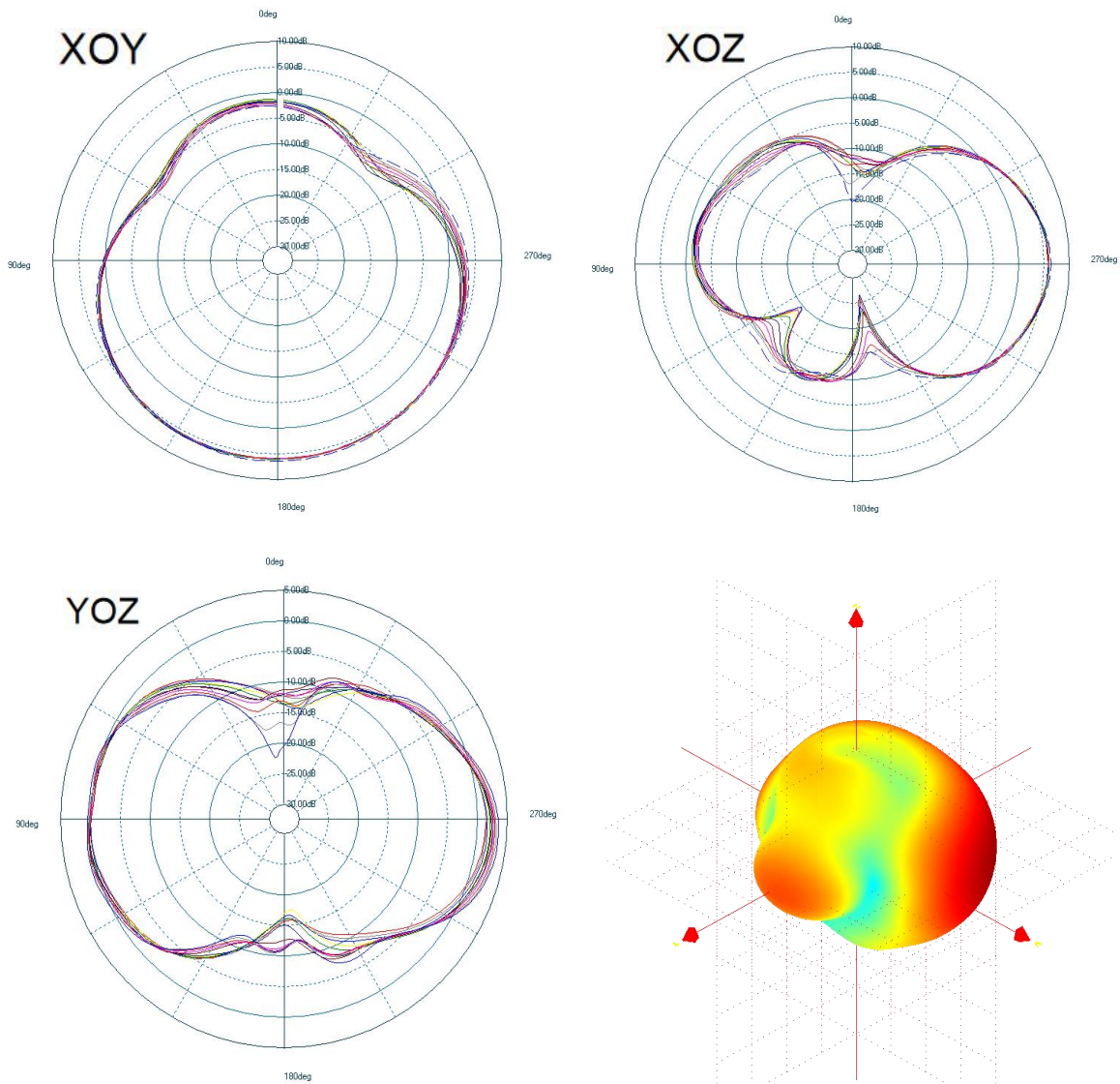
WIFI1:2.4G direction diagram
