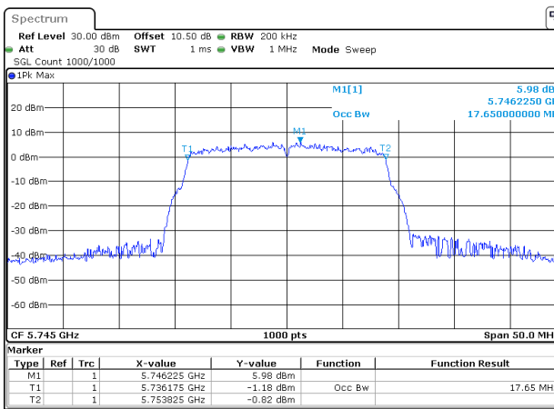
802.11n20_5745MHz_Chain 0
