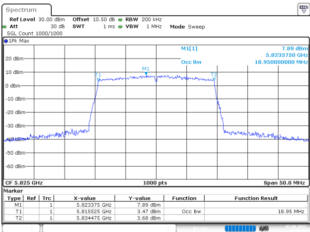
802.11ax20_5825MHz_Chain 0
