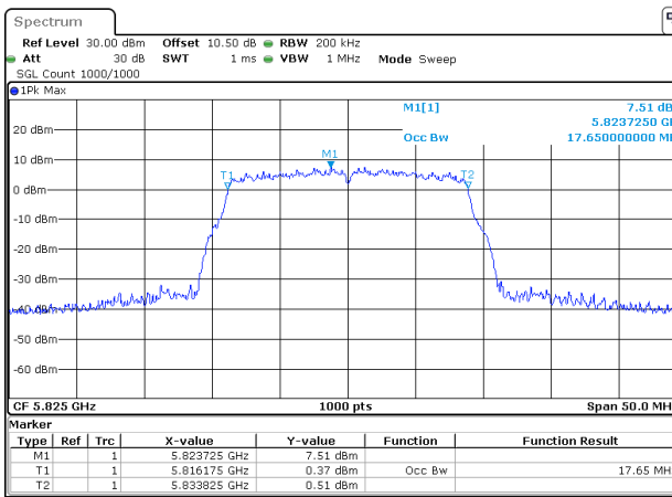
802.11n20_5825MHz_Chain 0
