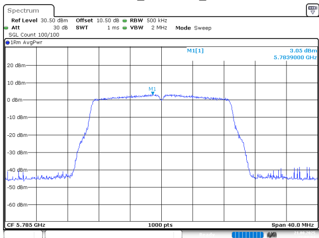
802.11ax20_5785MHz_Chain 0
