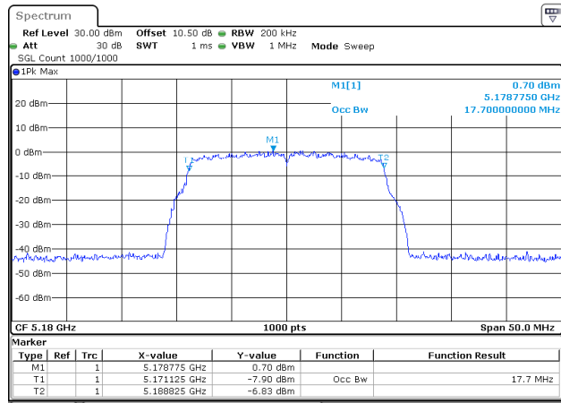
802.11n20_5180MHz_Chain 0
