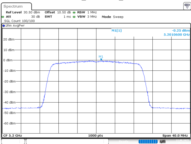
802.11ax20_5200MHz_Chain 0
