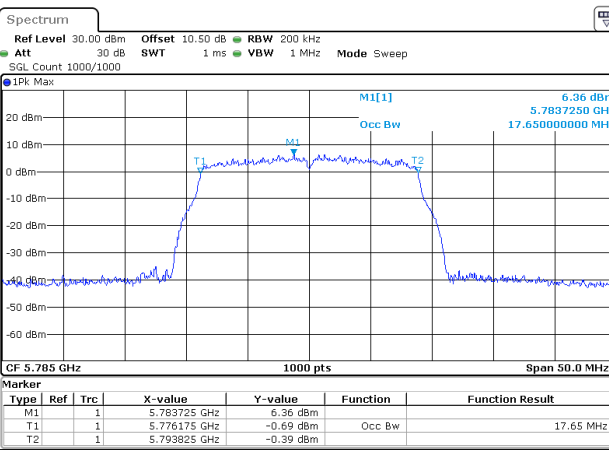
802.11n20_5785MHz_Chain 0
