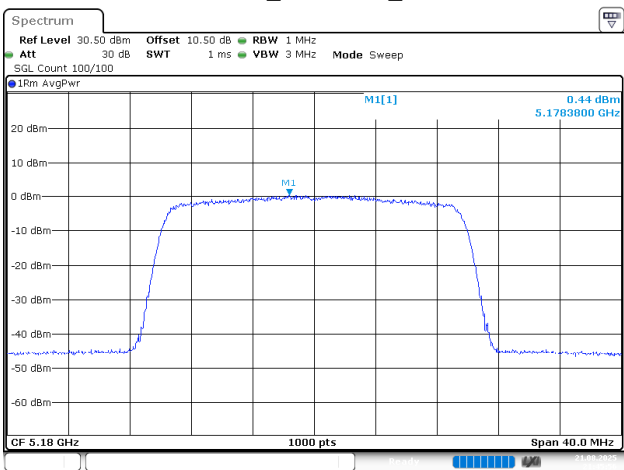
802.11ax20_5180MHz_Chain 1
