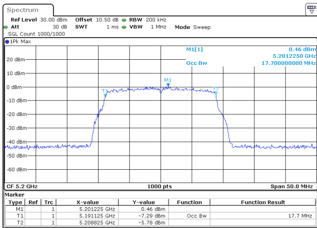
802.11n20_5200MHz_Chain 0
