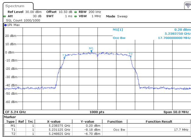
802.11n20_5240MHz_Chain 0
