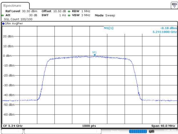
802.11ax20_5240MHz_Chain 1
