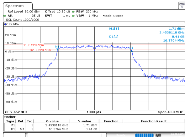
802.11g_2462MHz_Chain 0
