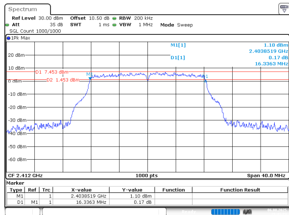
802.11g_2412MHz_Chain 0
