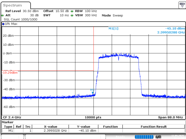
802.11ax20_2412MHz_Chain 0
