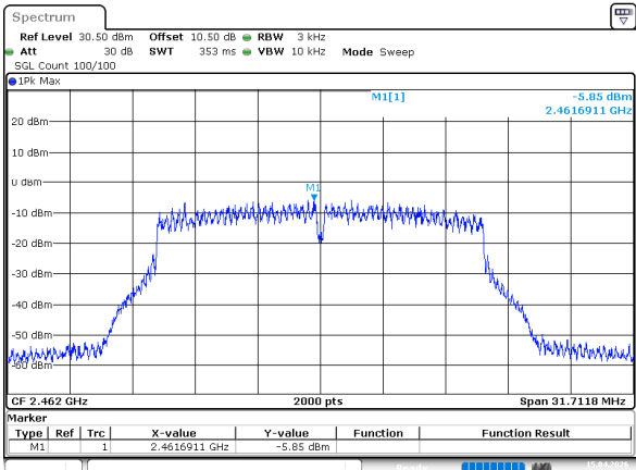
802.11g_2462MHz_Chain 0
