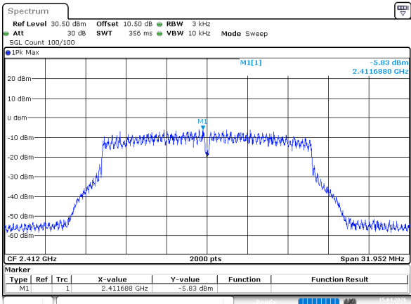
802.11g_2412MHz_Chain 0
