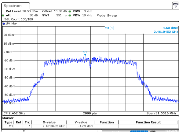
802.11g_2462MHz_Chain 1
