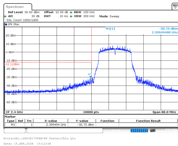
802.11g_2412MHz_Chain 0
