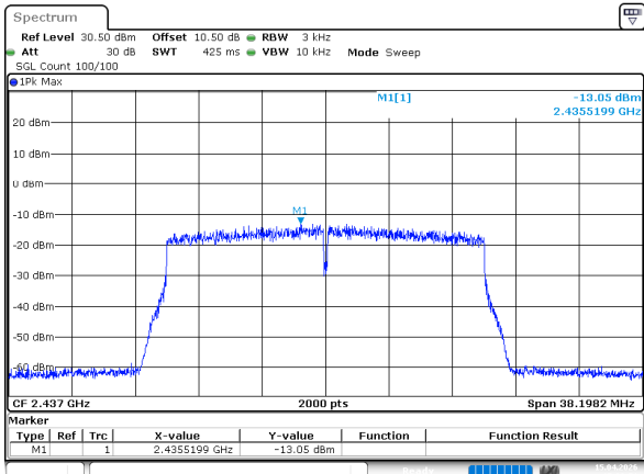
802.11ax20_2437MHz_RU_Full_Chain 0
