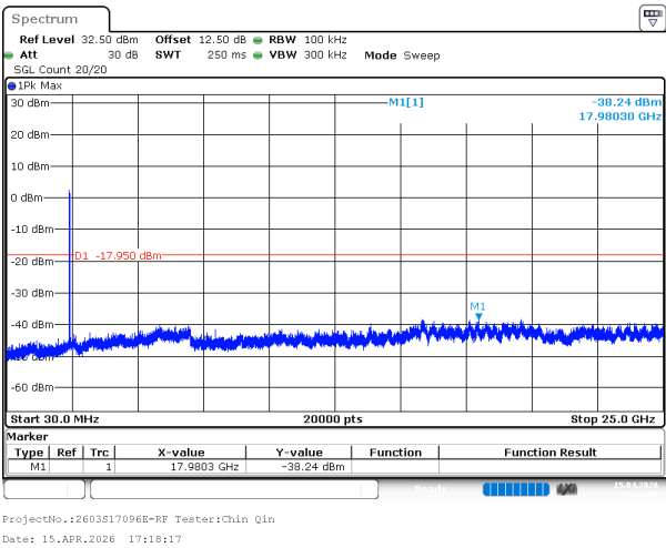
802.11ax20_2412MHz_RU_Full_Chain 1
