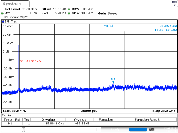
802.11g_2437MHz_Chain 1
