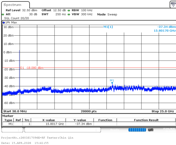
802.11ax20_2462MHz_RU_Full_Chain 0
