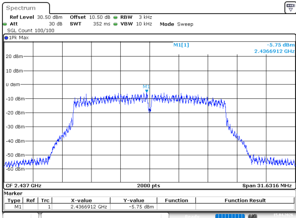
802.11g_2437MHz_Chain 0
