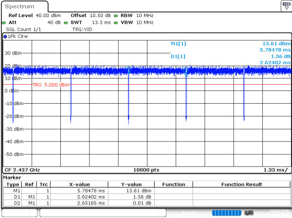
802.11ax20_2437MHz_RU_Full_Chain 0
