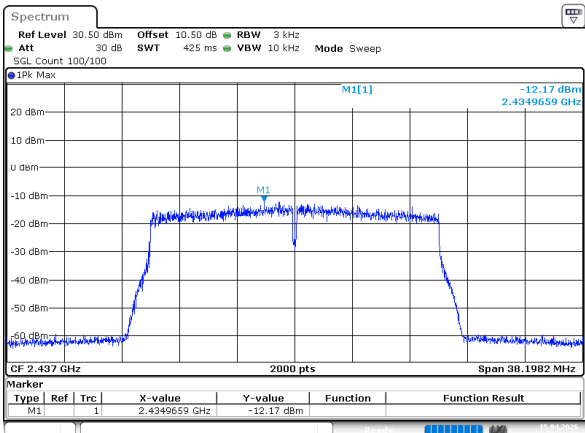
802.11ax20_2437MHz_RU_Full_Chain 1
