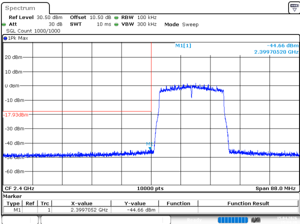
802.11ax20_2412MHz_RU_Full_Chain 0
