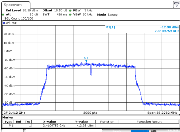
802.11ax20_2412MHz_RU_Full_Chain 1
