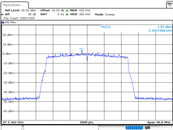
802.11ax20_2462MHz_RU_Full_Chain 0
