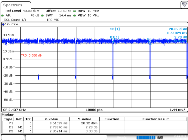
802.11g_2437MHz_Chain 0
