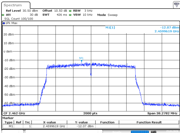
802.11ax20_2462MHz_RU_Full_Chain 1
