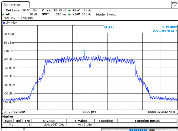
802.11g_2412MHz_Chain 1
