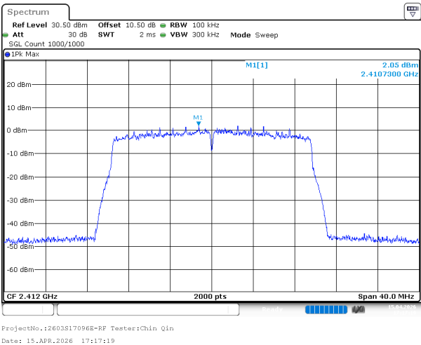
802.11ax20_2412MHz_RU_Full_Chain 1
