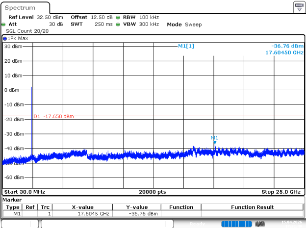
802.11ax20_2437MHz_RU_Full_Chain 1
