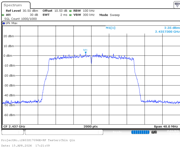
802.11ax20_2437MHz_RU_Full_Chain 1
