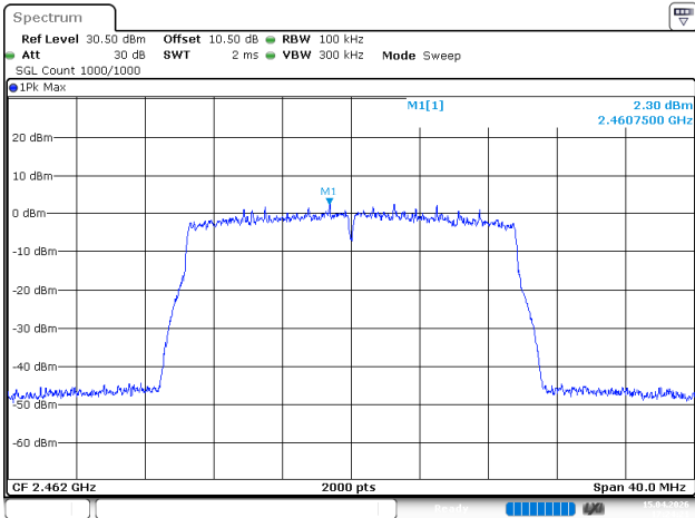
802.11ax20_2462MHz_RU_Full_Chain 1
