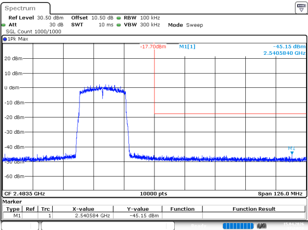
802.11ax20_2462MHz_RU_Full_Chain 1
