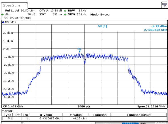
802.11g_2437MHz_Chain 1
