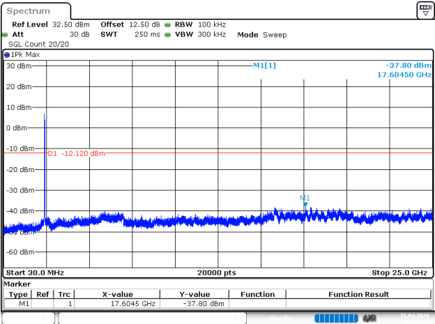
802.11g_2412MHz_Chain 0
