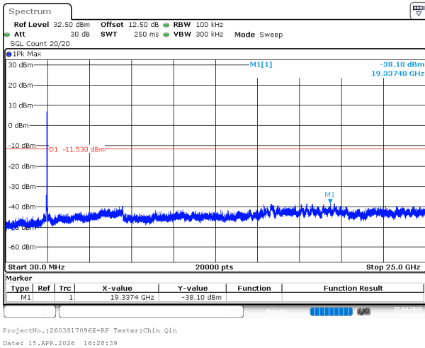
802.11g_2462MHz_Chain 1
