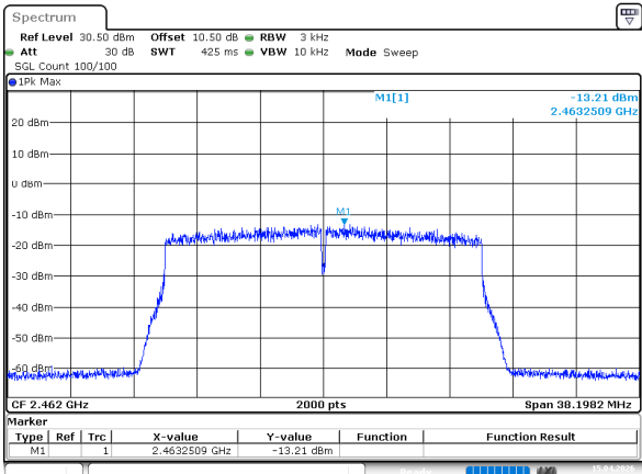
802.11ax20_2462MHz_RU_Full_Chain 0
