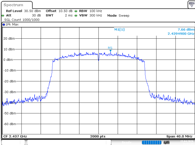
802.11g_2437MHz_Chain 0
