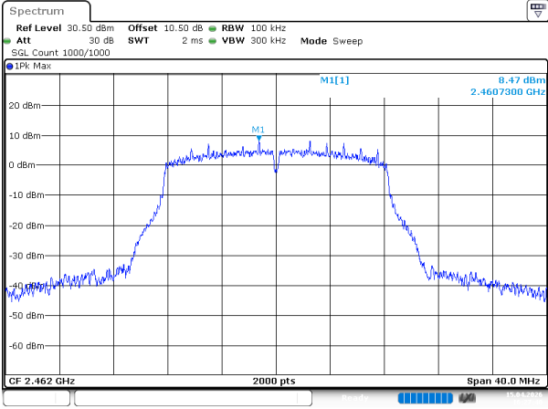
802.11g_2462MHz_Chain 1
