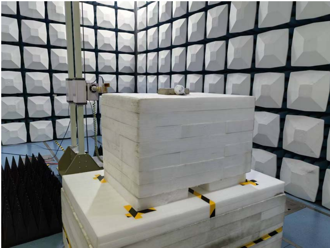
Radiated Emission 40-60GHz View
