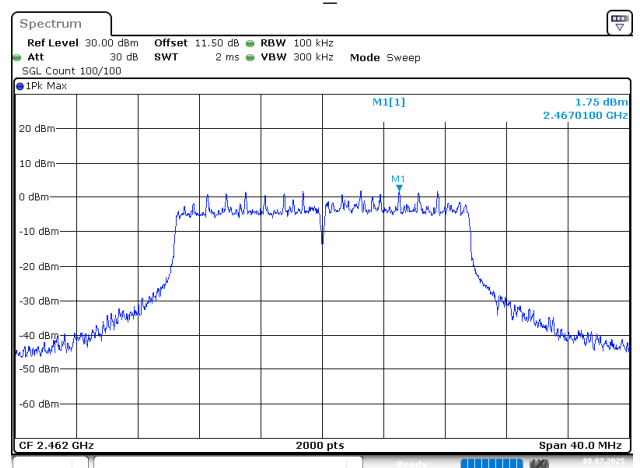
802.11ax20 2462MHz
