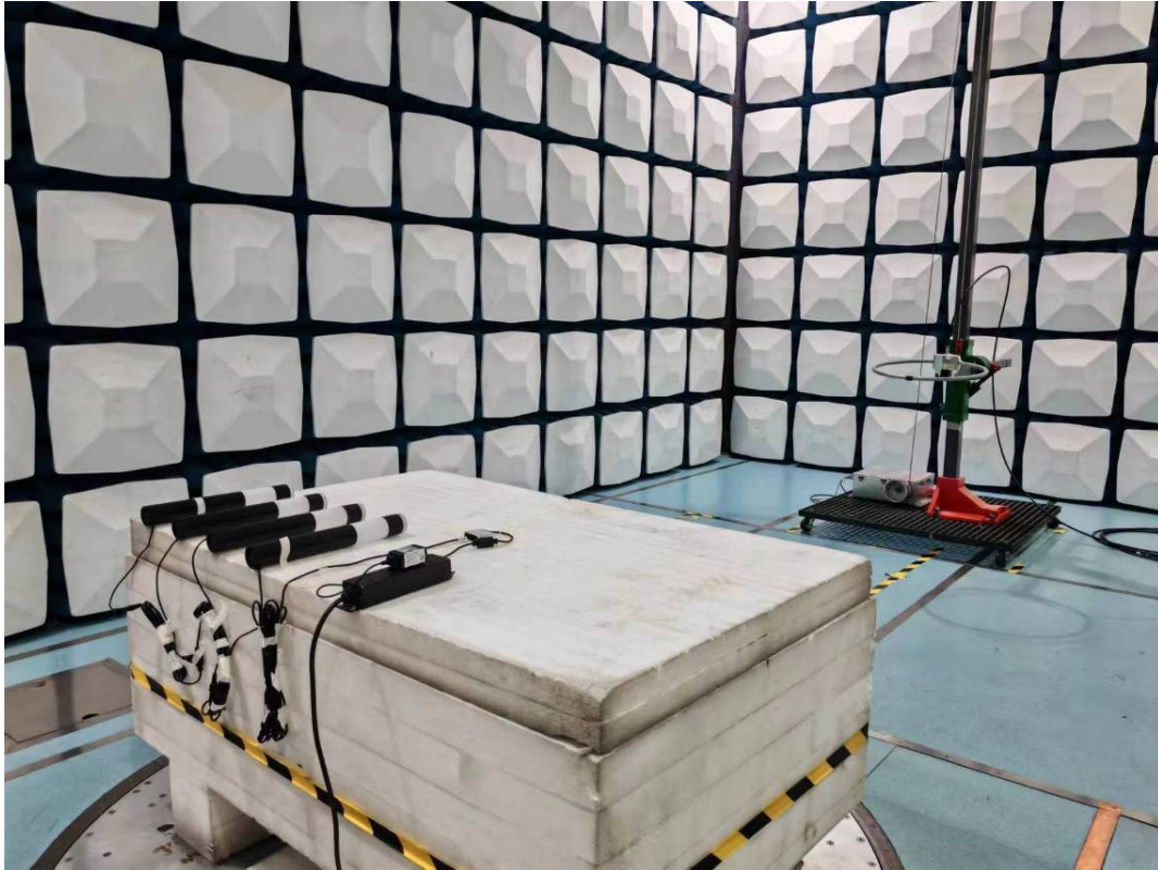
Radiated Emission Below 1G front View
