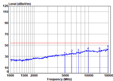
antenna 0 BLE_1M_TX_CH_39_Horizontal-Avg
