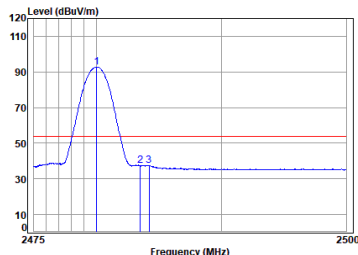
antenna 1 BLE_1M_TX_CH_39_Vertical-Avg
