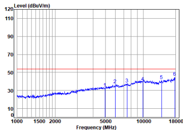
antenna 0 BLE_1M_TX_CH_39_Vertical-Avg
