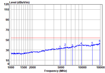
antenna 0 BLE_1M_TX_CH_19_Horizontal-Avg
