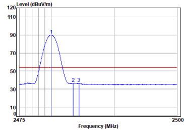
antenna 0 BLE_1M_TX_CH_39_Horizontal-Avg
