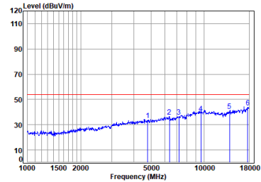
antenna 1 BLE_1M_TX_CH_00_Horizontal-Avg
