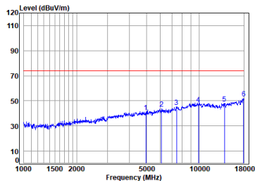
antenna 0 BLE_1M_TX_CH_39_Vertical-Peak
