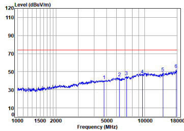
antenna 1 BLE_1M_TX_CH_00_Vertical-Peak
