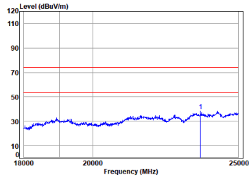
antenna 1 BLE_1M_TX_CH_19_Horizontal-Peak
