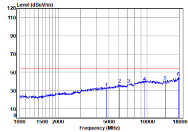
antenna 1 BLE_1M_TX_CH_00_Vertical-Avg
