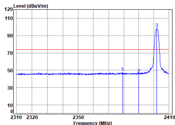
antenna 1 BLE_1M_TX_CH_00_Horizontal-Peak
