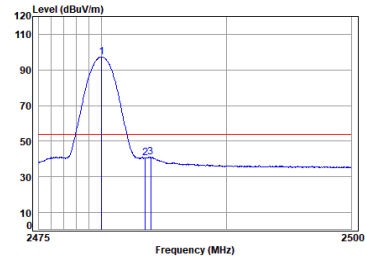
antenna 0 BLE_1M_TX_CH_39_Vertical-Avg
