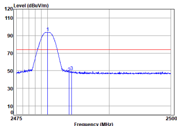
antenna 1 BLE_1M_TX_CH_39_Vertical-Peak
