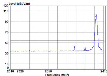
antenna 1 BLE_1M_TX_CH_00_Horizontal-Avg
