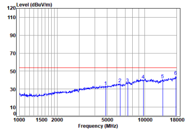
antenna 0 BLE_1M_TX_CH_19_Vertical-Avg
