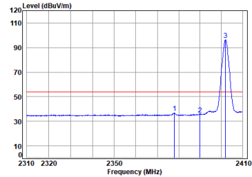
antenna 1 BLE_2M_TX_CH_00_Horizontal-Avg
