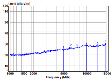
antenna 0 BLE_1M_TX_CH_39_Horizontal-Peak
