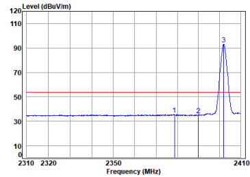
antenna 1 BLE_2M_TX_CH_00_Vertical-Avg
