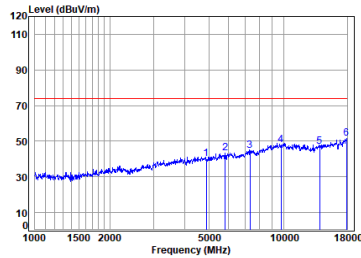
antenna 0 BLE_1M_TX_CH_19_Vertical-Peak
