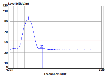
antenna 1 BLE_1M_TX_CH_39_Horizontal-Avg
