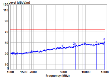
antenna 1 11n_HT(20M)_TX_CH_06_Horizontal-Peak
