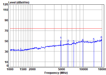
antenna 1 11b_TX_CH_11_Horizontal-Peak
