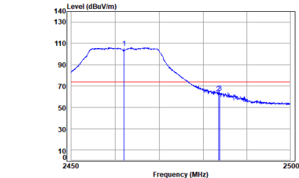
antenna 0 11g_TX_CH_11_Vertical-Peak
