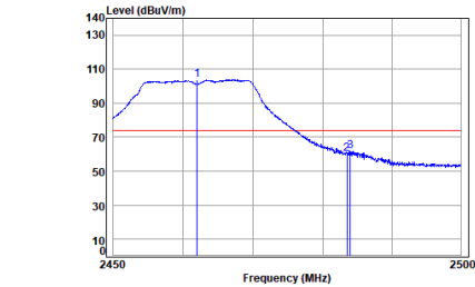
antenna 1 11g_TX_CH_11_Vertical-Peak
