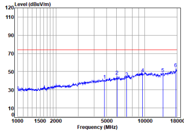
antenna 0 11n_HT(20M)_TX_CH_01_Horizontal-Peak
