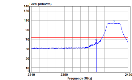
antenna 1 11n_HT(20M)_TX_CH_01_Vertical-Peak
