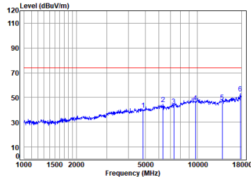
antenna 0 11n_HT(20M)_TX_CH_06_Horizontal-Peak
