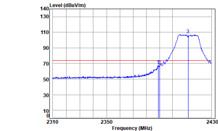
antenna 1 11g_TX_CH_01_Horizontal-Peak
