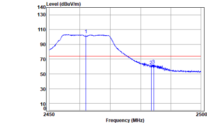
antenna 1 11g_TX_CH_11_Horizontal-Peak
