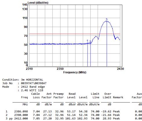
antenna 0 11b_TX_CH_01_Horizontal-Peak
