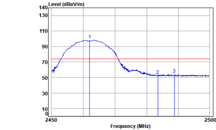
antenna 0 11b_TX_CH_11_Horizontal-Peak
