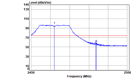
antenna 0 11g_TX_CH_11_Horizontal-Peak
