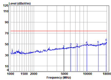
antenna 0 11b_TX_CH_11_Vertical-Peak
