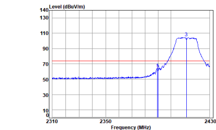
antenna 1 11g_TX_CH_01_Vertical-Peak
