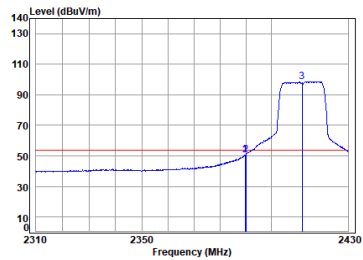
antenna 0 11g_TX_CH_01_Vertical-Avg
