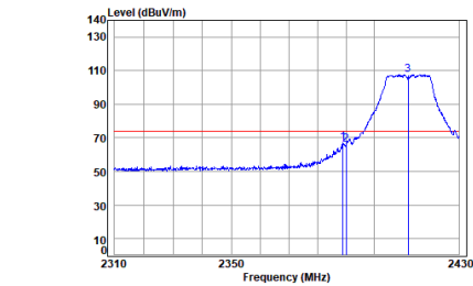
antenna 0 11g_TX_CH_01_Vertical-Peak
