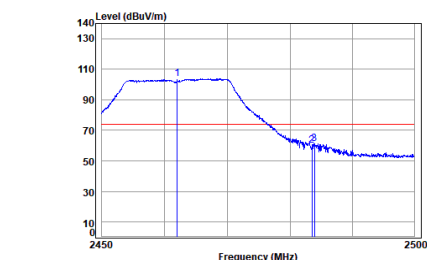
antenna 1 11n_HT(20M)_TX_CH_11_Vertical-Peak
