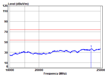
antenna 1 11b_TX_CH_06_Horizontal-Peak
