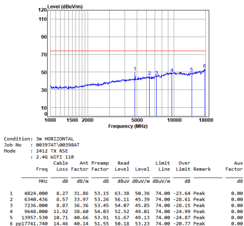
antenna 0 11b_TX_CH_01_Horizontal-Peak
