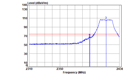
antenna 1 11n_HT(20M)_TX_CH_01_Horizontal-Peak
