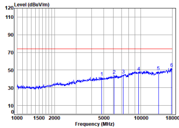
antenna 0 11n_HT(20M)_TX_CH_01_Vertical-Peak
