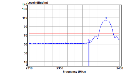
antenna 1 11b_TX_CH_01_Vertical-Peak
