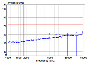
antenna 0 11b_TX_CH_06_Horizontal-Peak
