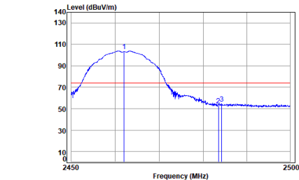
antenna 1 11b_TX_CH_11_Horizontal-Peak
