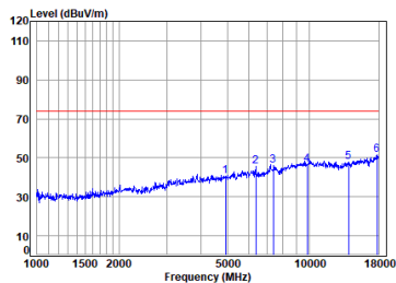
antenna 1 11n_HT(20M)_TX_CH_11_Horizontal-Peak
