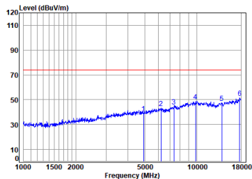
antenna 1 11n_HT(20M)_TX_CH_11_Vertical-Peak
