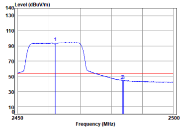
antenna 1 11g_TX_CH_11_Vertical-Avg
