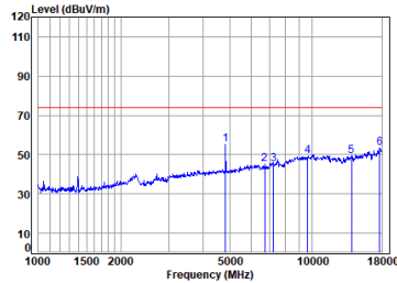
antenna 1 11b_TX_CH_01_Horizontal-Peak
