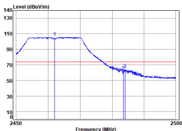
antenna 0 11n_HT(20M)_TX_CH_11_Vertical-Peak
