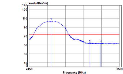
antenna 1 11b_TX_CH_11_Vertical-Peak
