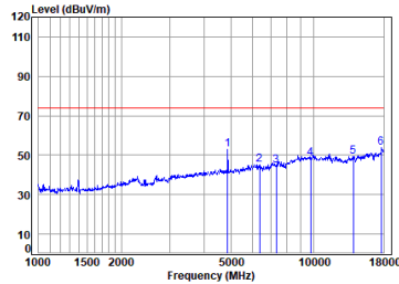
antenna 1 11b_TX_CH_06_Horizontal-Peak
