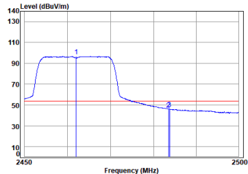
antenna 0 11g_TX_CH_11_Vertical-Avg
