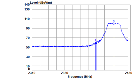
antenna 0 11g_TX_CH_01_Horizontal-Peak
