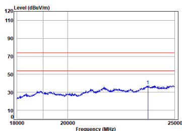
antenna 0 11b_TX_CH_06_Vertical-Peak
