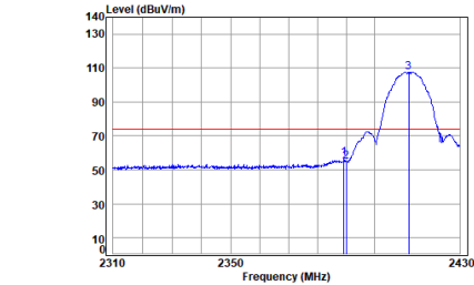
antenna 1 11b_TX_CH_01_Horizontal-Peak
