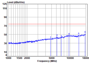
antenna 1 11n_HT(20M)_TX_CH_01_Vertical-Peak
