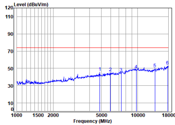
antenna 1 11b_TX_CH_06_Vertical-Peak
