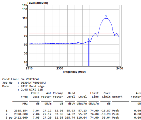
antenna 0 11b_TX_CH_01_Vertical-Peak
