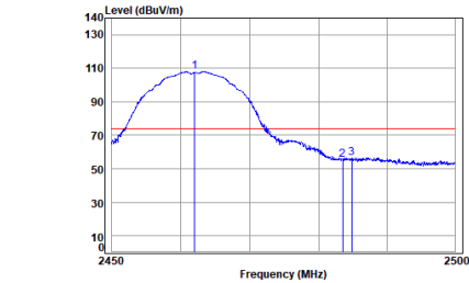
antenna 0 11b_TX_CH_11_Vertical-Peak
