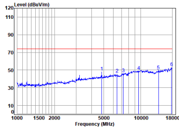
antenna 1 11b_TX_CH_01_Vertical-Peak
