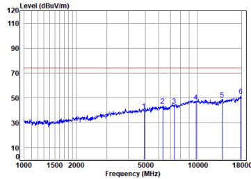
antenna 0 11n_HT(20M)_TX_CH_11_Horizontal-Peak
