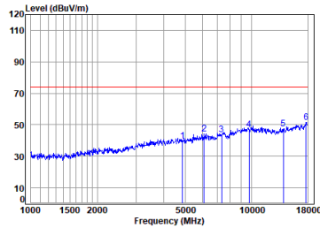
antenna 1 11n_HT(20M)_TX_CH_06_Vertical-Peak
