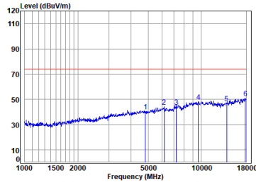
antenna 1 11n_HT(20M)_TX_CH_01_Horizontal-Peak
