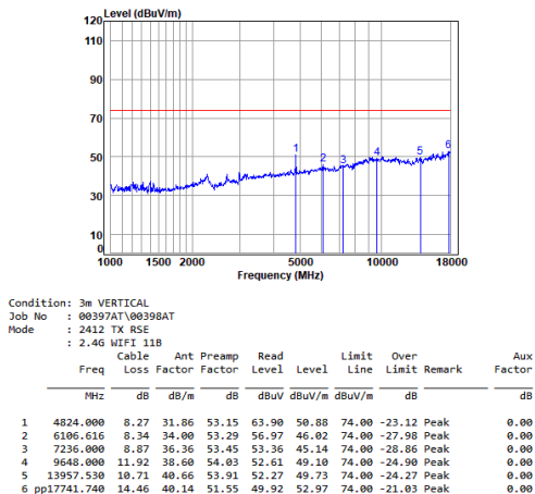
antenna 0 11b_TX_CH_01_Vertical-Peak
