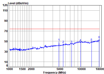
antenna 0 11b_TX_CH_06_Vertical-Peak
