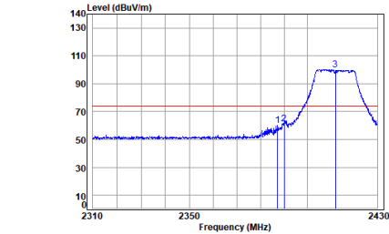
antenna 0 11n_HT(20M)_TX_CH_01_Horizontal-Peak
