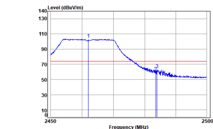
antenna 1 11n_HT(20M)_TX_CH_11_Horizontal-Peak
