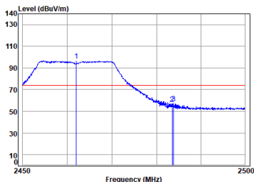
antenna 0 11n_HT(20M)_TX_CH_11_Horizontal-Peak
