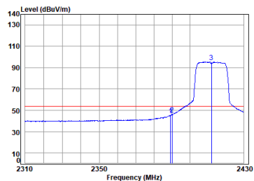
antenna 1 11g_TX_CH_01_Vertical-Avg
