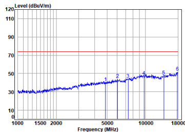
antenna 0 11n_HT(20M)_TX_CH_06_Vertical-Peak
