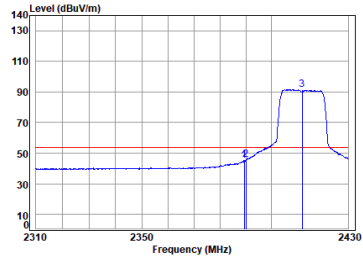
antenna 0 11g_TX_CH_01_Horizontal-Avg
