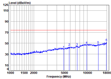
antenna 0 11n_HT(20M)_TX_CH_11_Vertical-Peak
