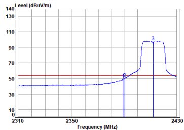
antenna 1 11g_TX_CH_01_Horizontal-Avg
