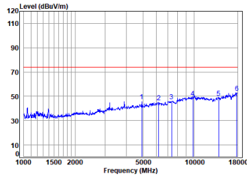
antenna 1 11b_TX_CH_11_Vertical-Peak
