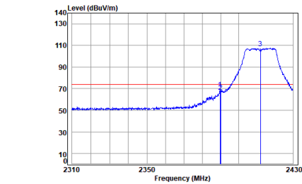
antenna 0 11n_HT(20M)_TX_CH_01_Vertical-Peak
