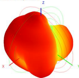
2450.0MHz H+V, Eff: 39.7%
