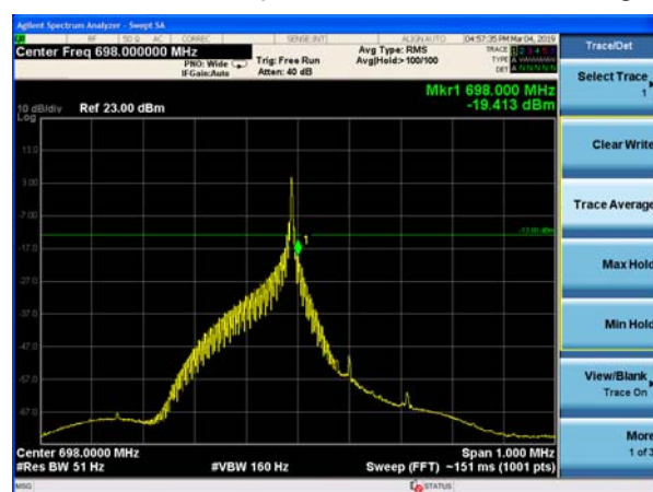
NB-IOT Band 71 QPSK 15kHz 1@0 CH-High
