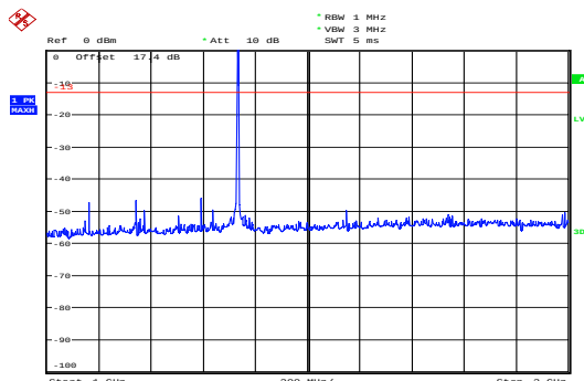
NB-IOT Band 4 QPSK 15KHz CH-Middle 1GHz~3GHz
