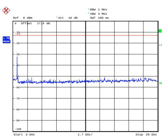
NB-IOT Band 4 QPSK 15KHz CH-Middle 3GHz~20GHz
