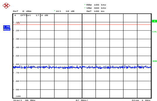
NB-IOT Band 4 QPSK 15KHz CH-Low 30MHz~1GHz
