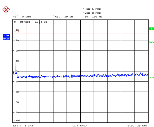
NB-IOT Band 4 QPSK 15KHz CH-Low 3GHz~20GHz
