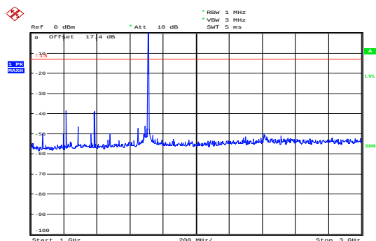
NB-IOT Band 4 QPSK 15KHz CH-Low 1GHz~3GHz
