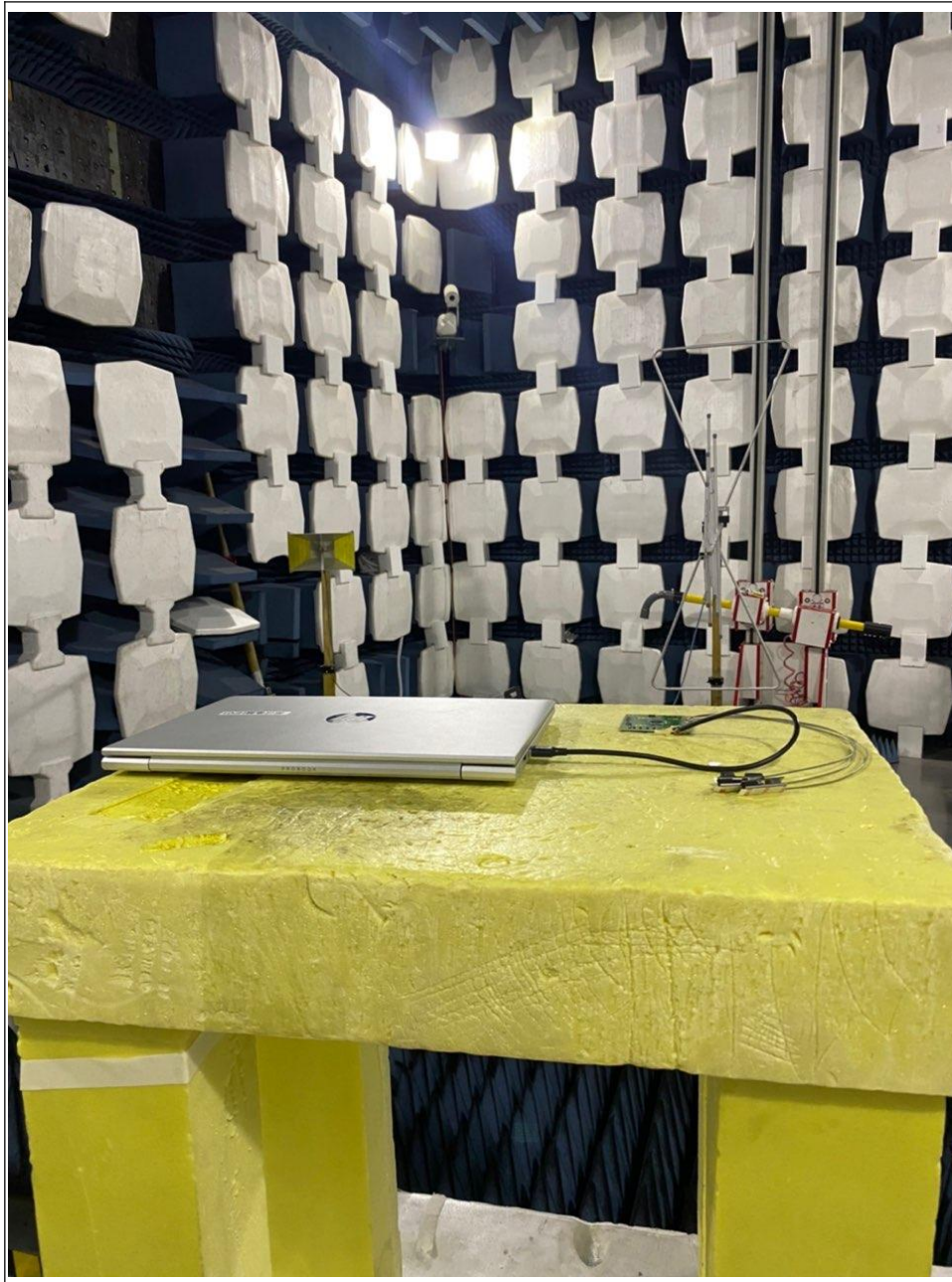
RADIATED SPURIOUS EMISSION TEST (ABOVE 1G)-1
