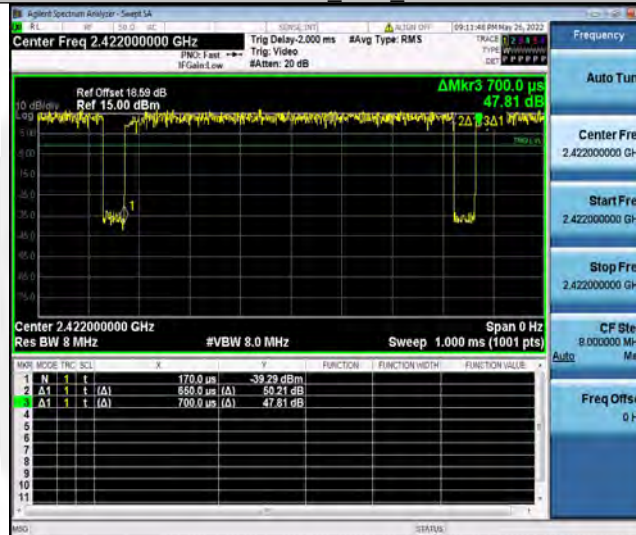
11N40SISO Ant2 2422
