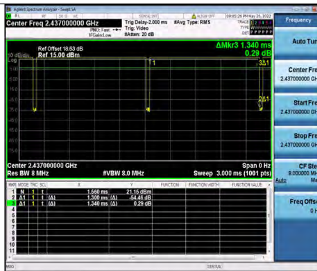
11N20SISO Ant2 2437
