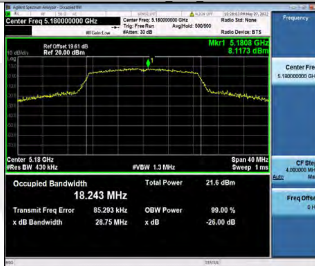
11AC20SISO_Ant2_5180
