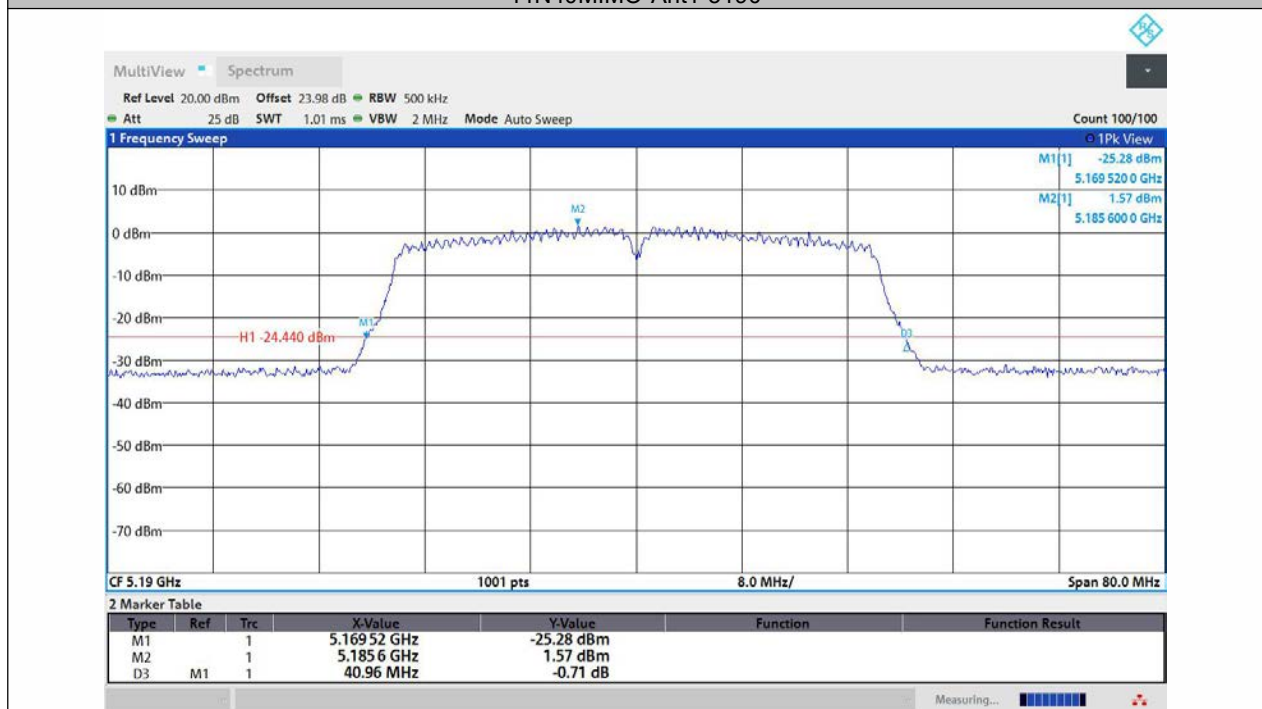
11N40MIMO-Ant2-5190
