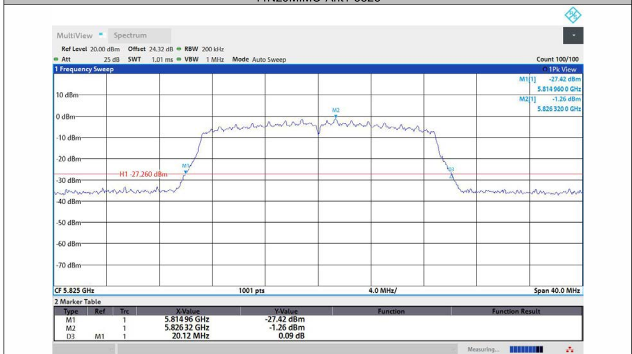
11N20MIMO-Ant2-5825
