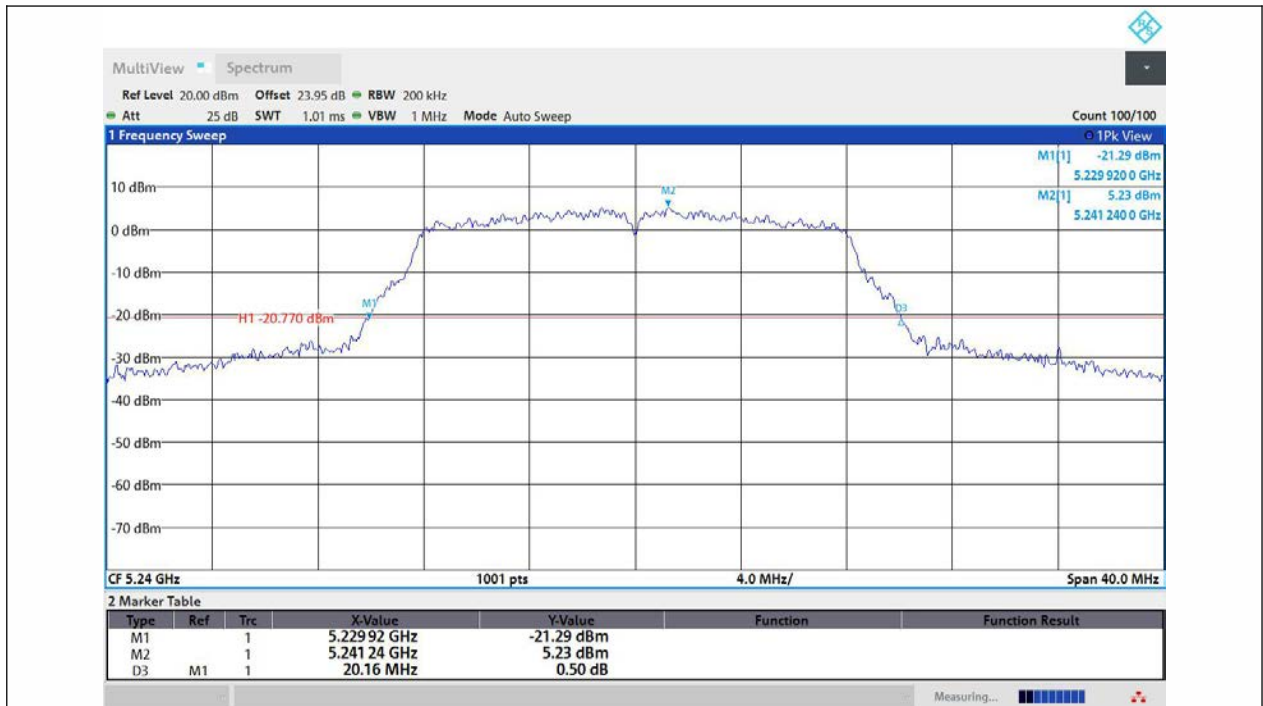
11A-Ant1-5240
