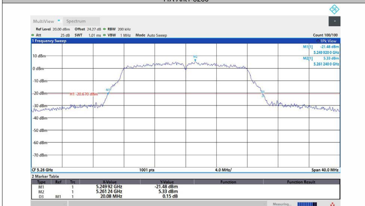
11A-Ant2-5260
