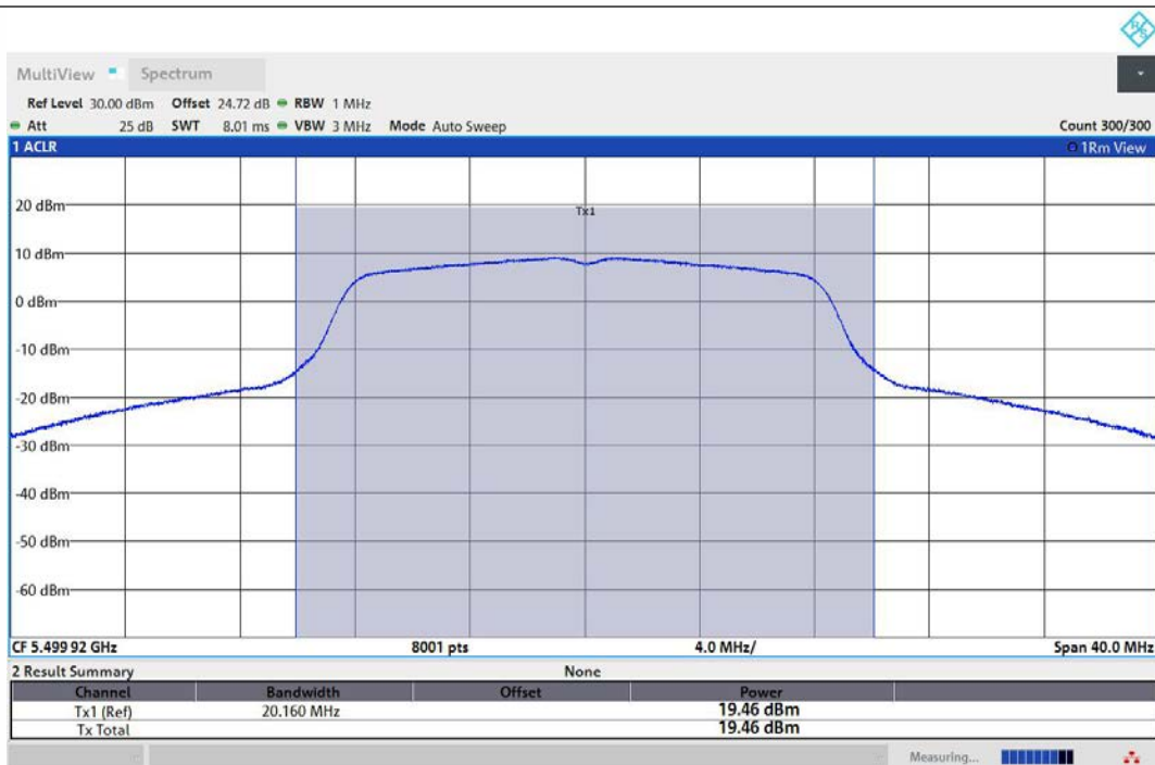
11A-Ant1-5500-PASS
