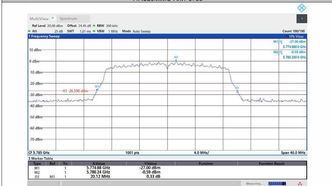
11AC20MIMO-Ant2-5785
