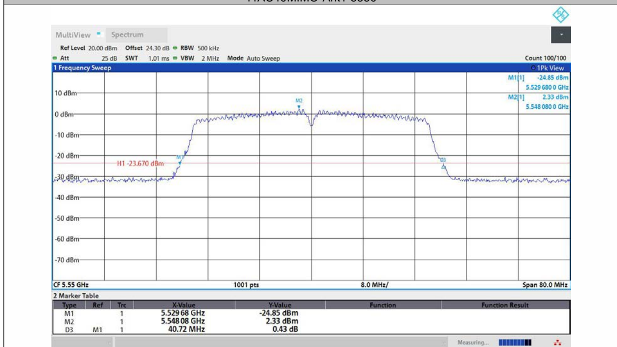
11AC40MIMO-Ant2-5550
