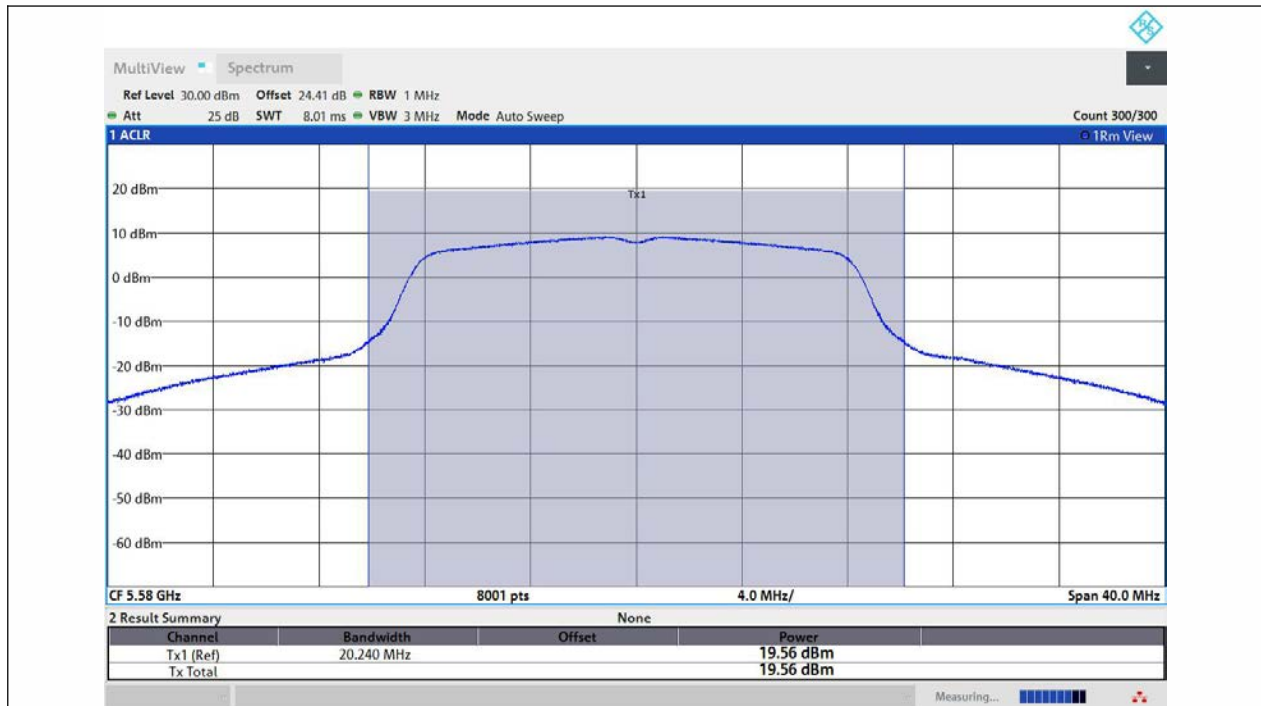
11A-Ant1-5580-PASS
