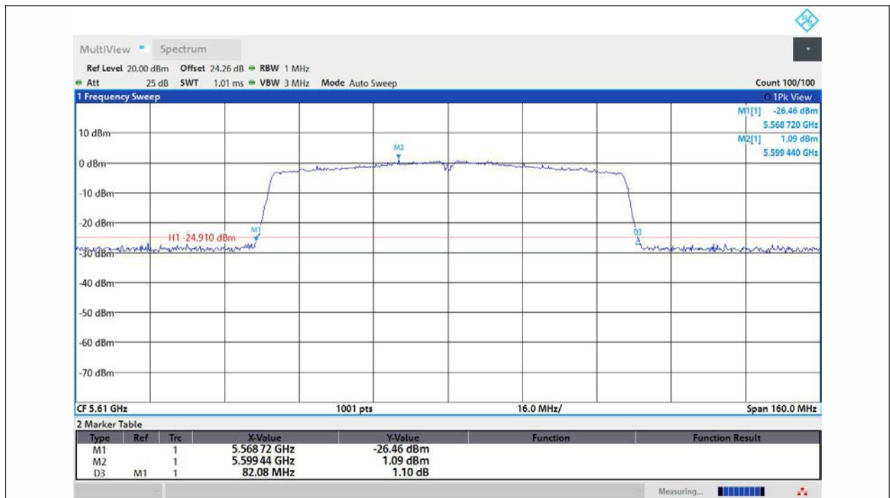
11AC80MIMO-Ant1-5610
