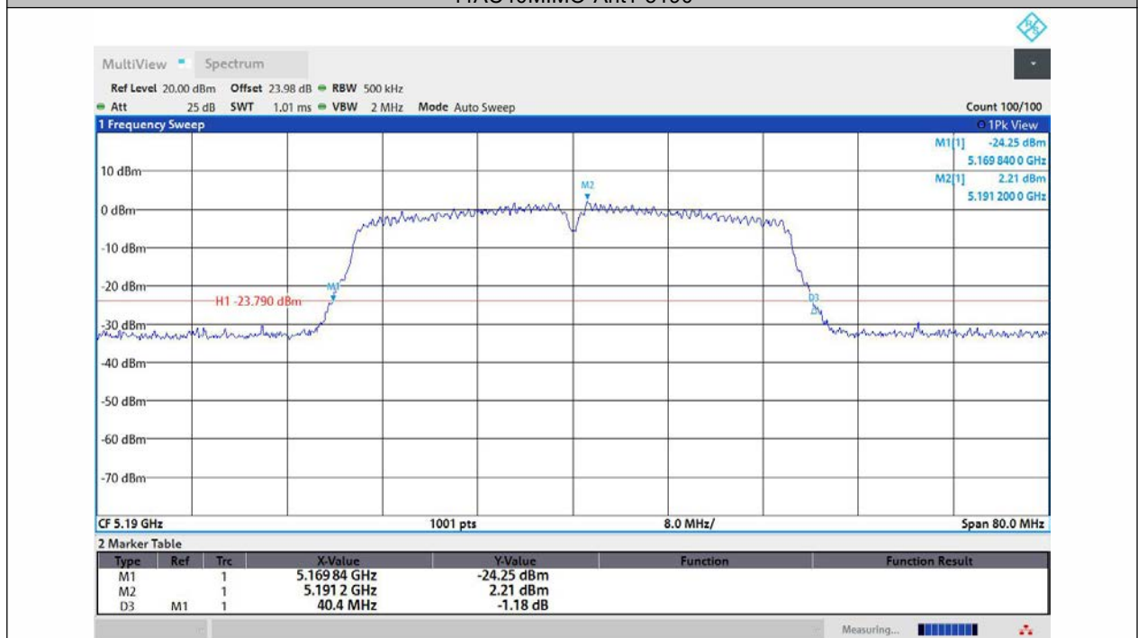
11AC40MIMO-Ant2-5190
