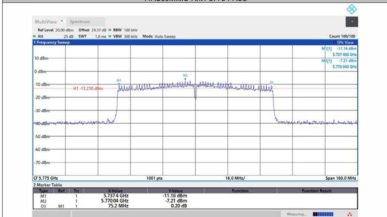
11AC80MIMO-Ant2-5775-PASS
