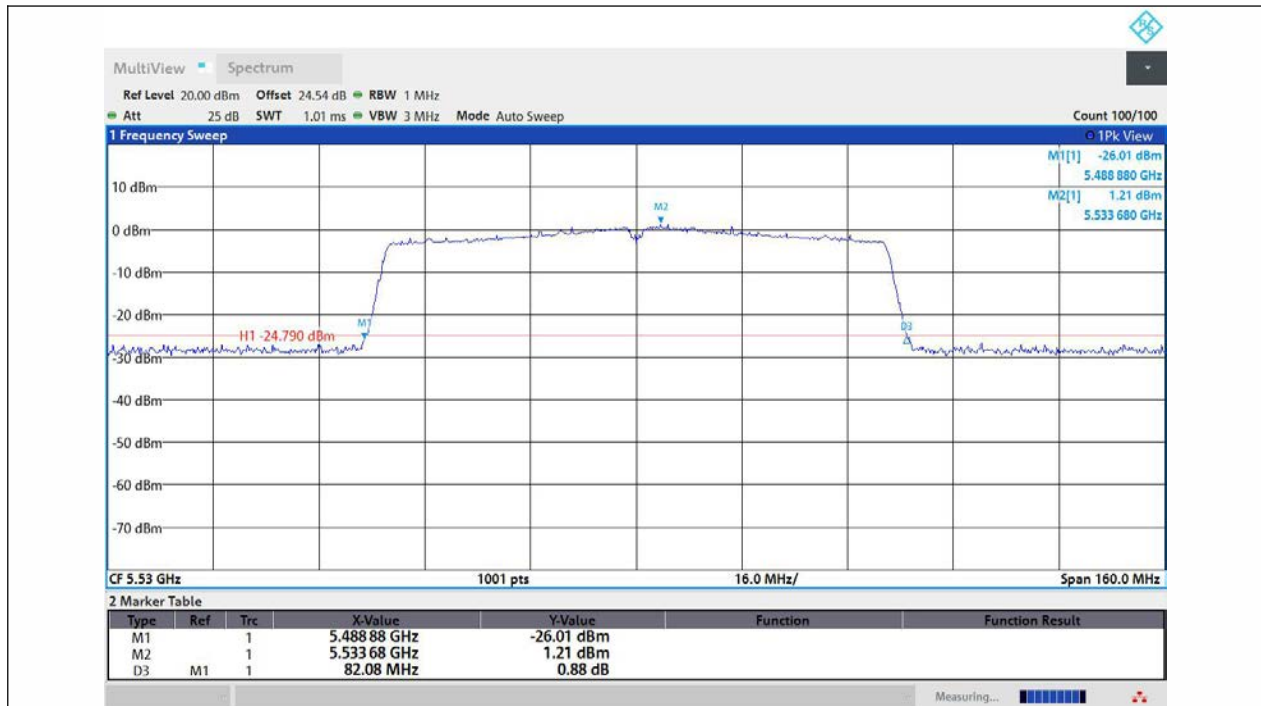
11AC80MIMO-Ant1-5530
