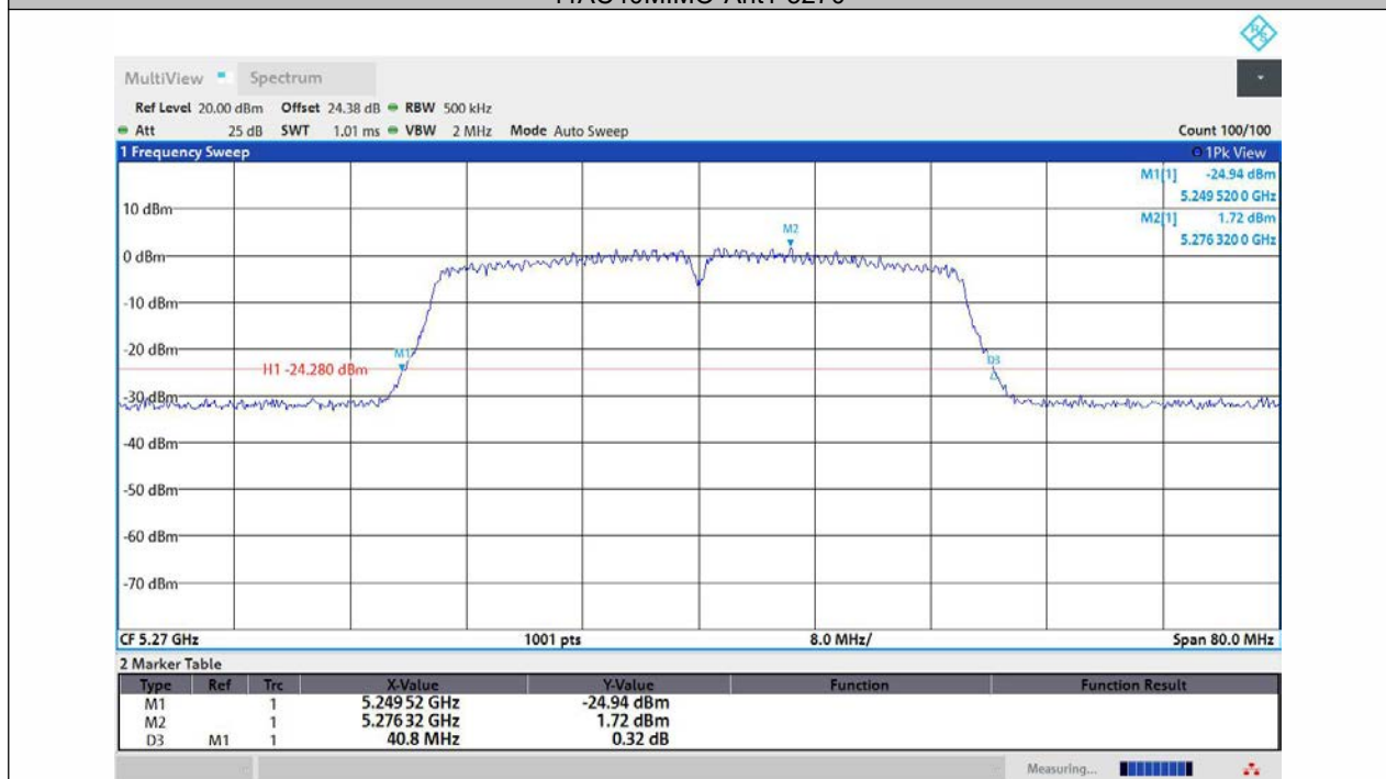
11AC40MIMO-Ant2-5270
