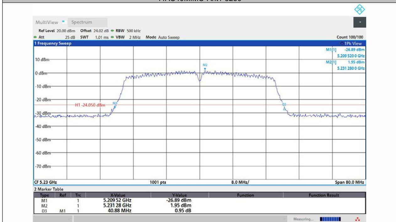
11AC40MIMO-Ant2-5230
