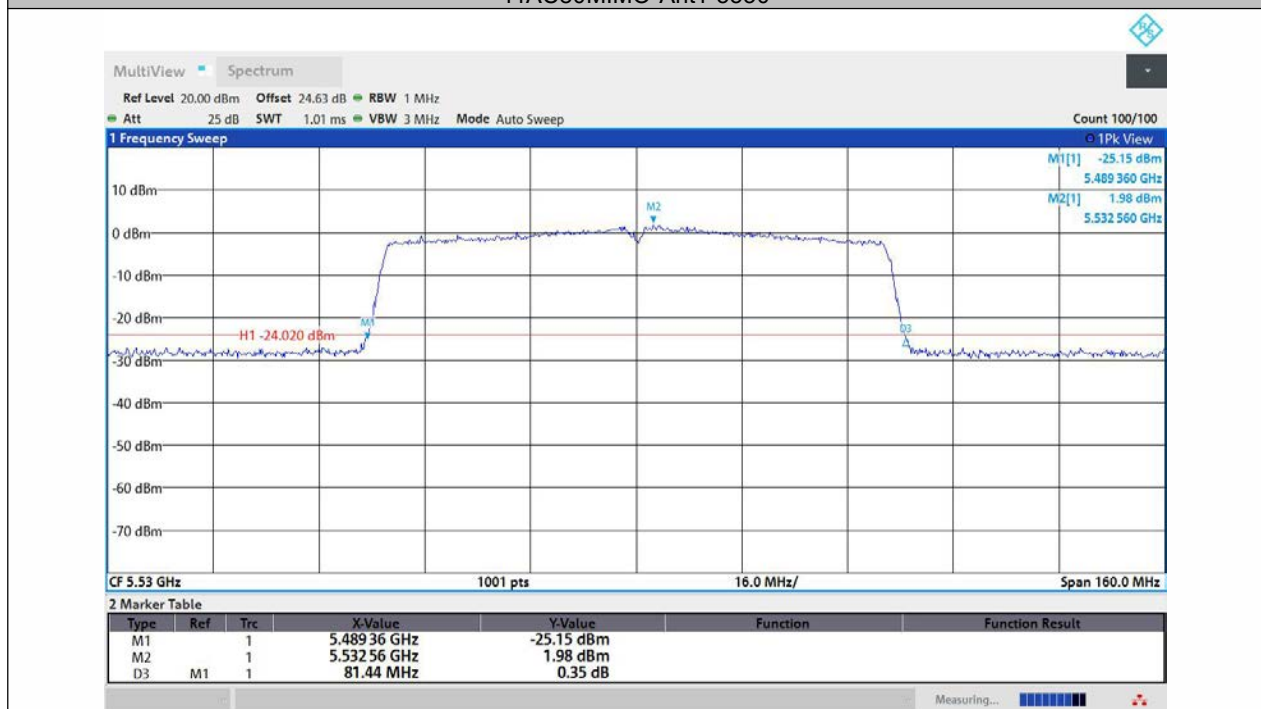
11AC80MIMO-Ant2-5530
