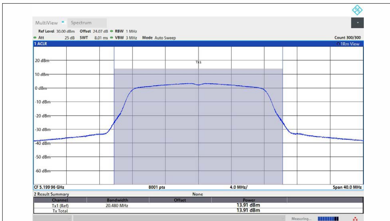
11A-Ant1-5200-PASS
