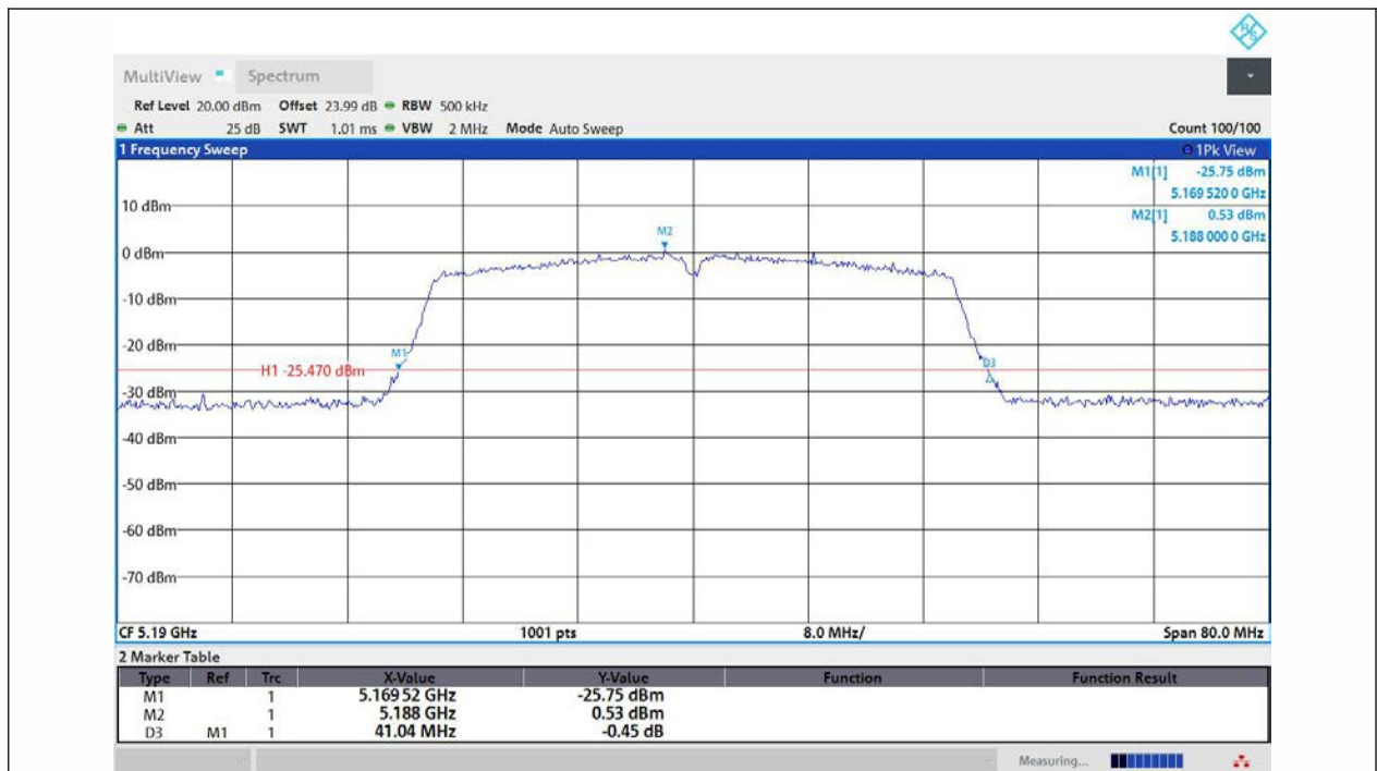
11AC40MIMO-Ant1-5190
