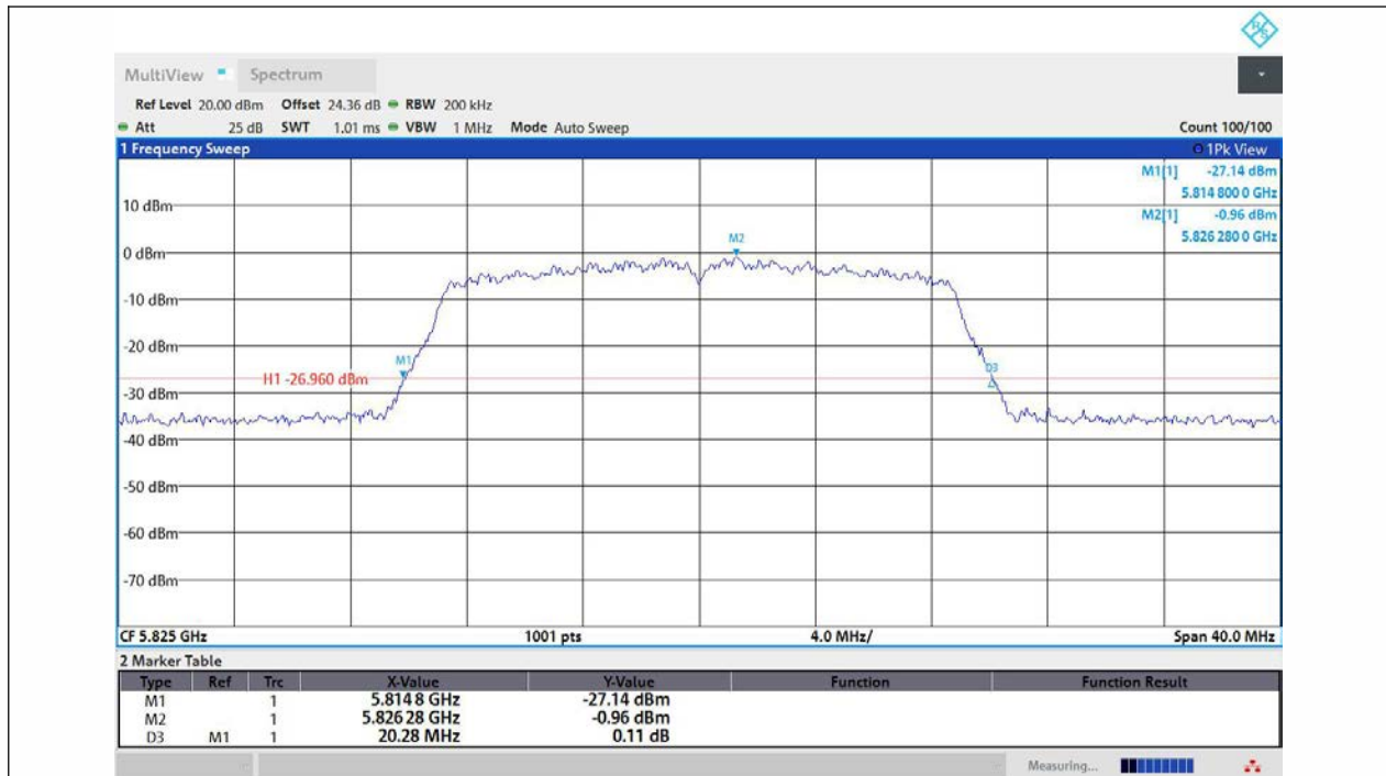
11AC20MIMO-Ant1-5825
