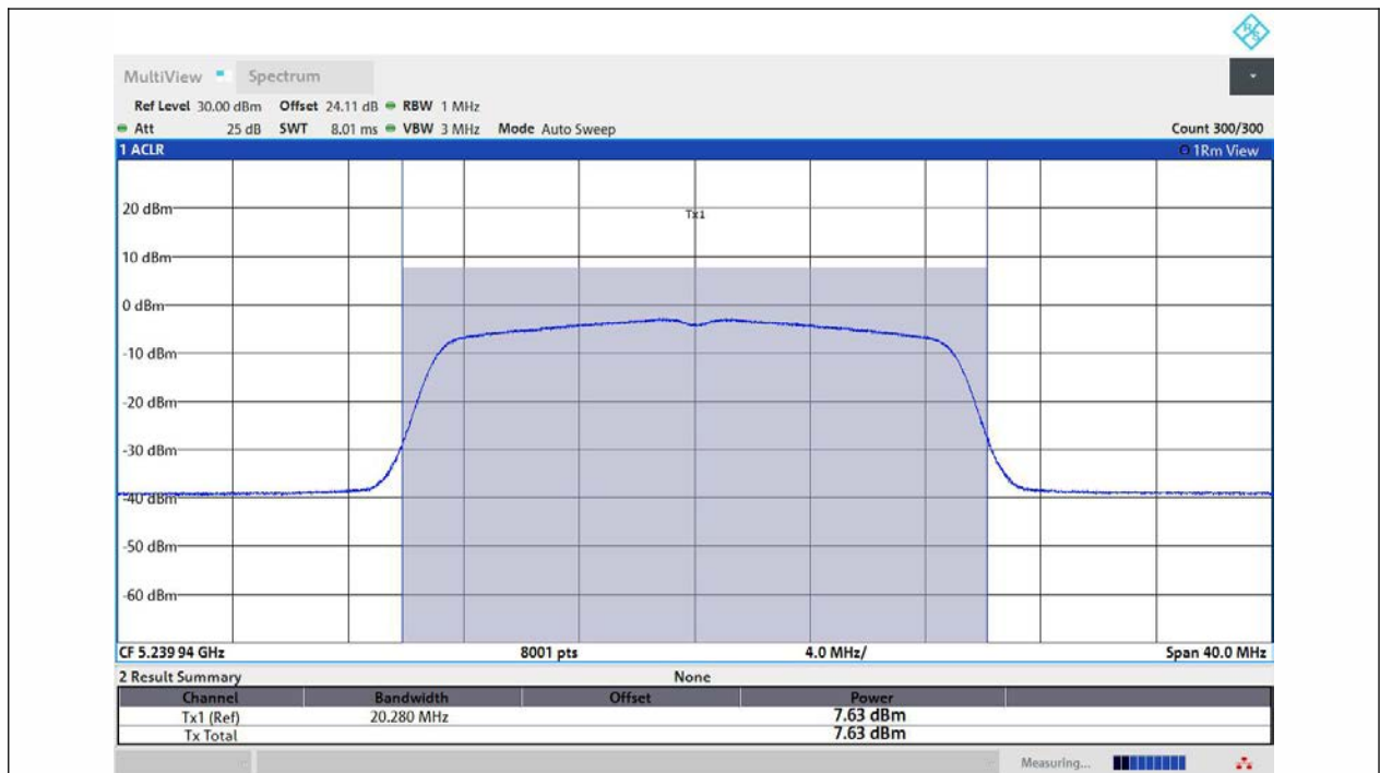
11N20MIMO-Ant1-5240-PASS
