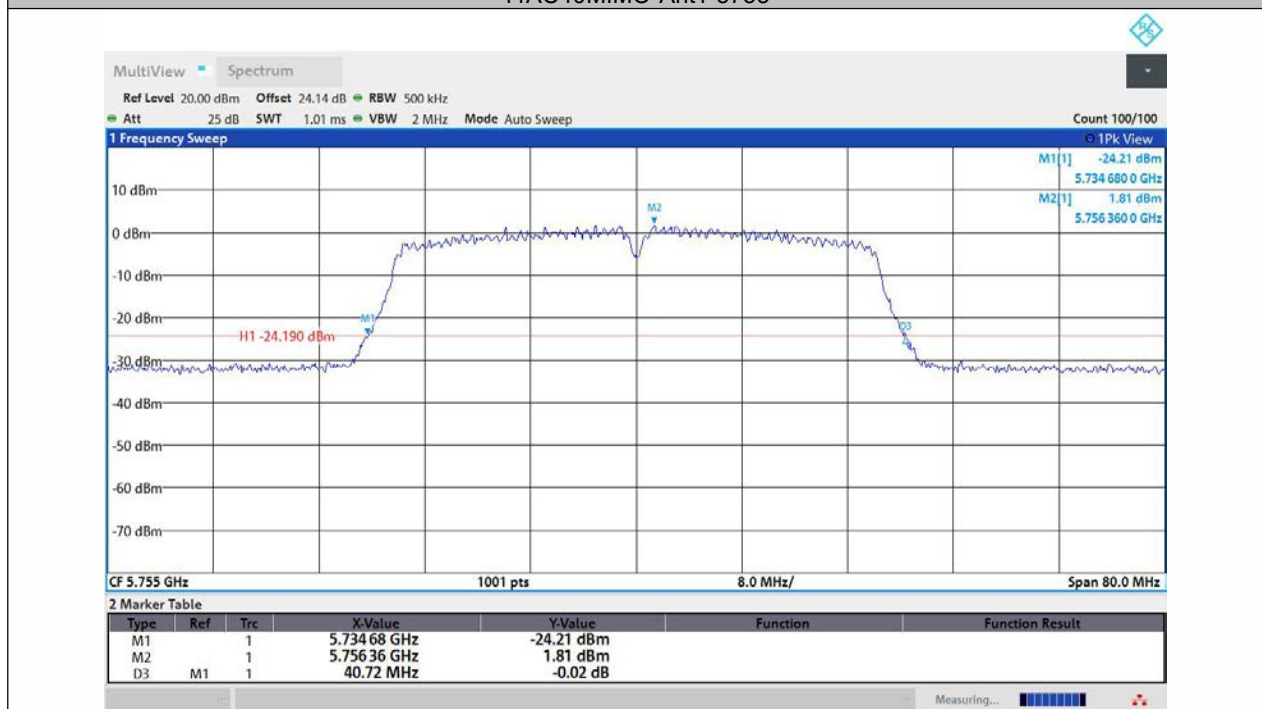
11AC40MIMO-Ant2-5755
