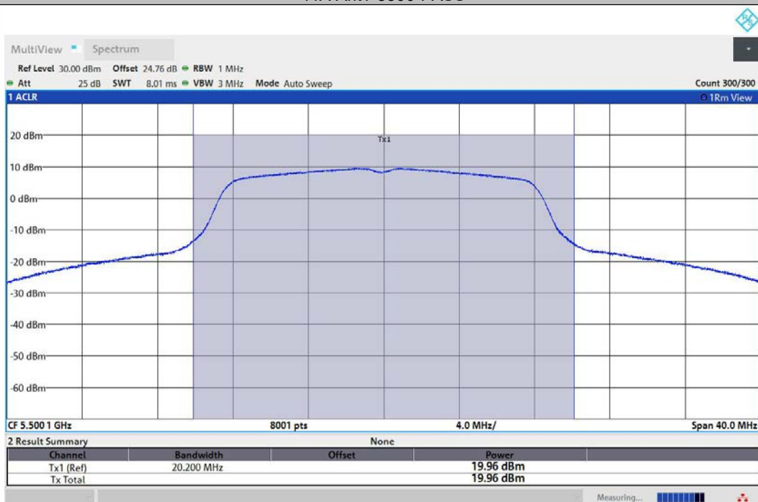
11A-Ant2-5500-PASS
