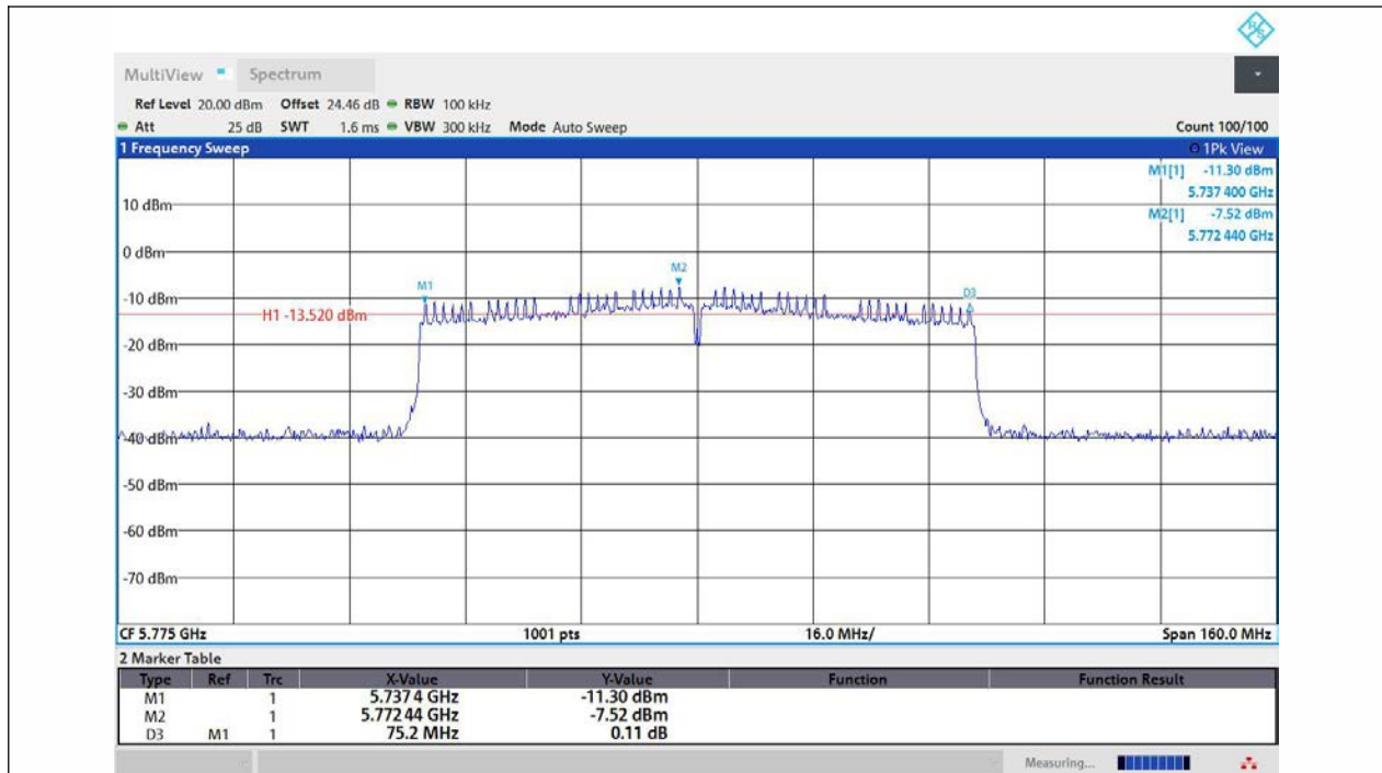
11AC80MIMO-Ant1-5775-PASS
