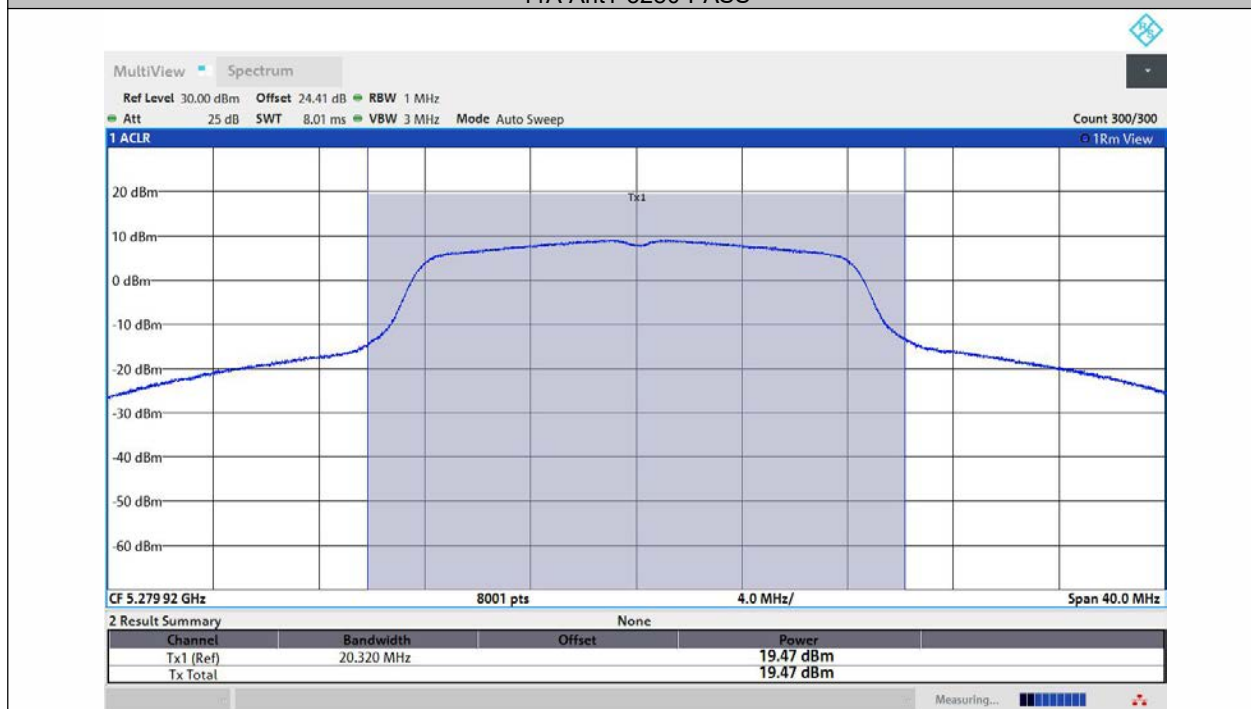
11A-Ant2-5280-PASS
