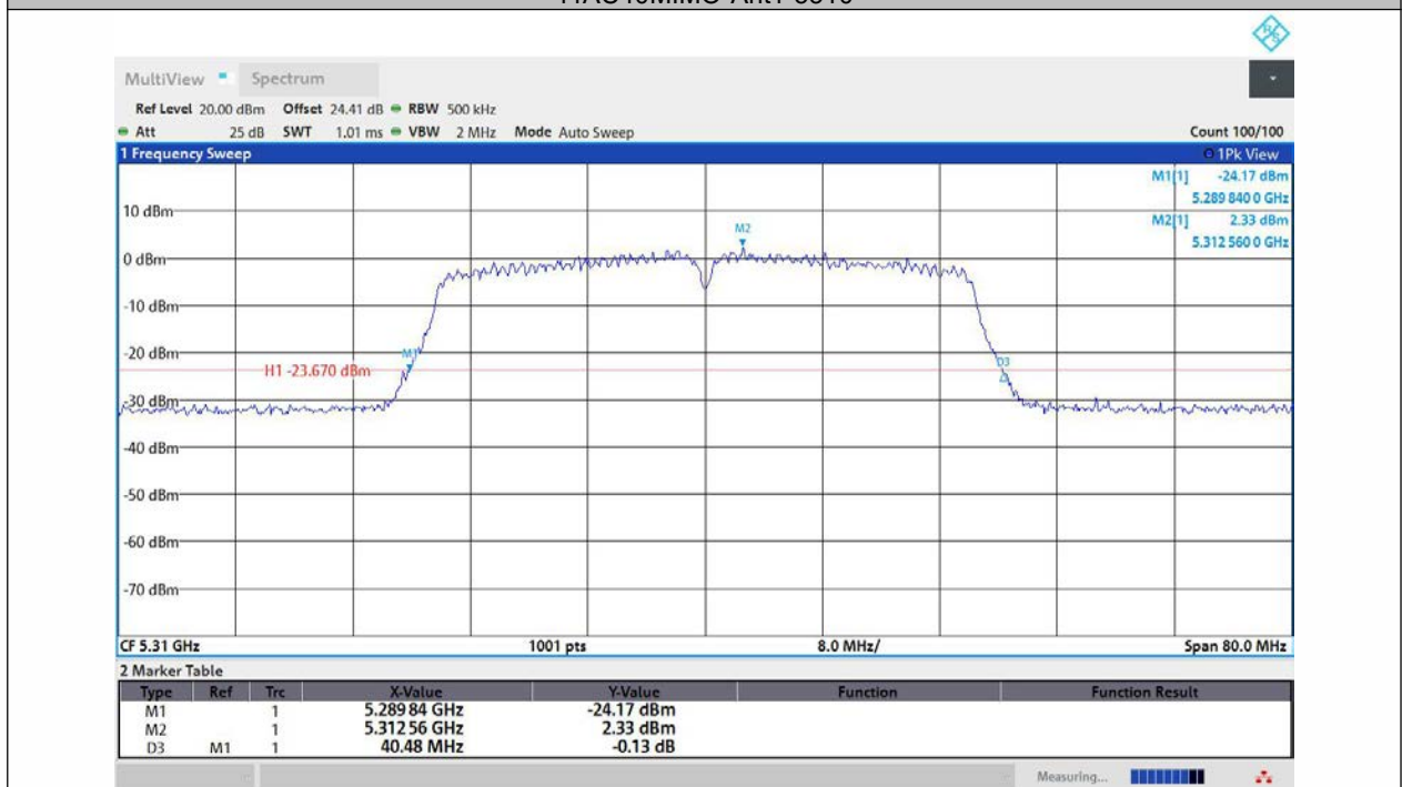
11AC40MIMO-Ant2-5310
