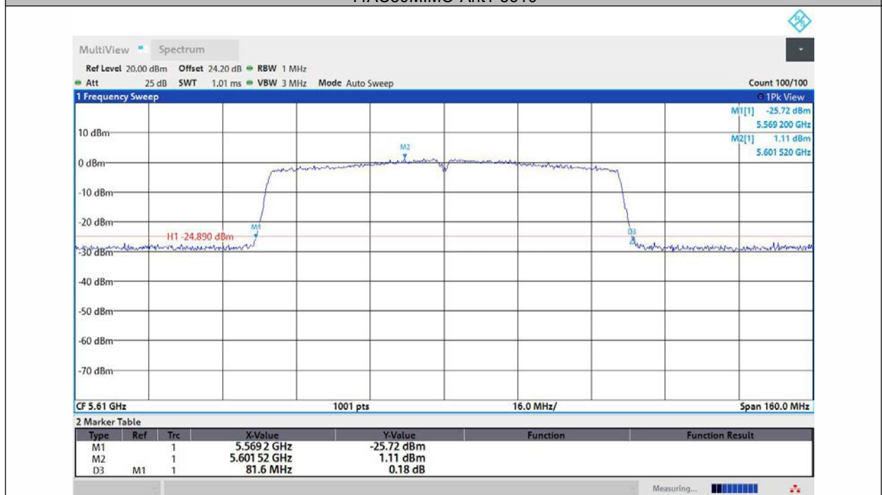
11AC80MIMO-Ant2-5610
