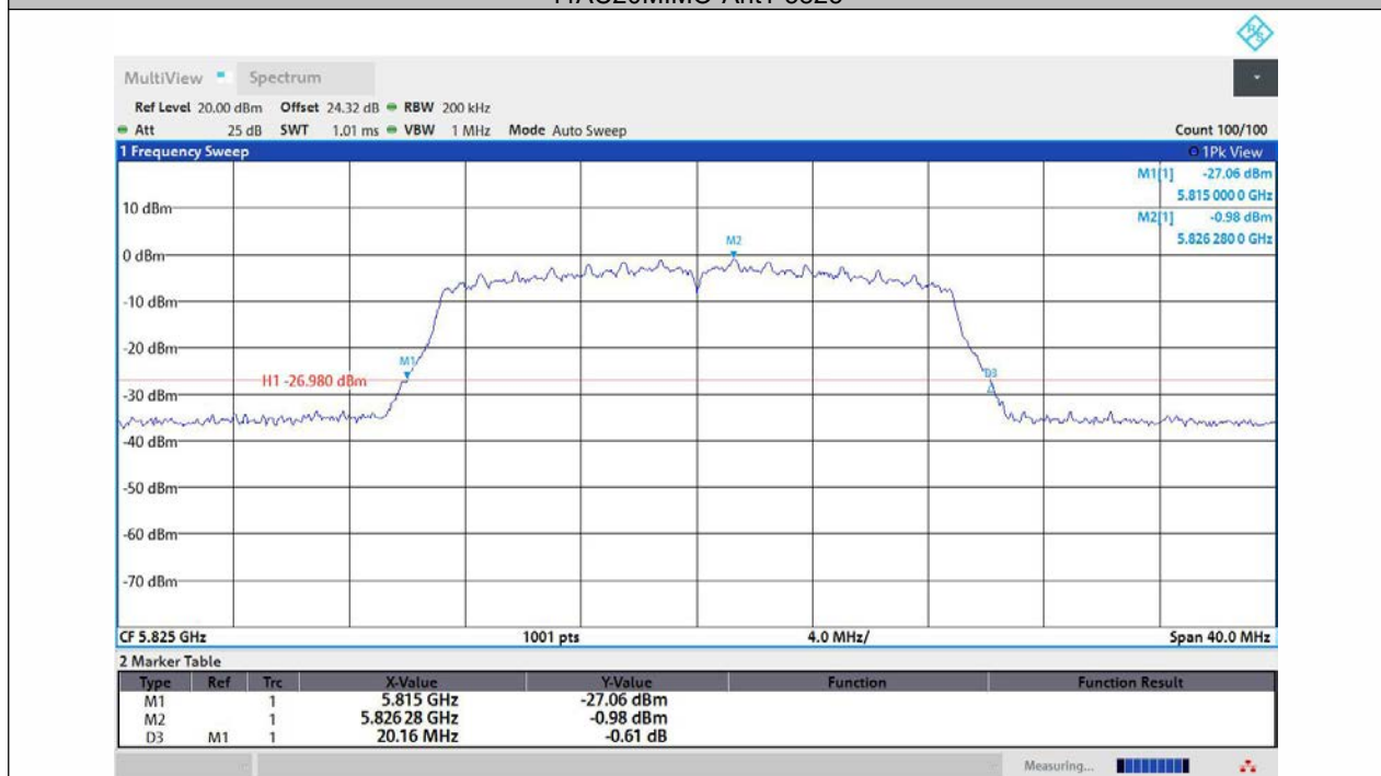
11AC20MIMO-Ant2-5825
