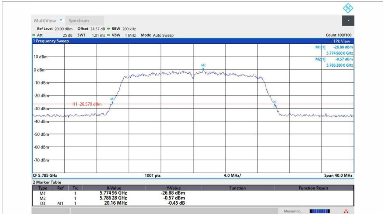
11AC20MIMO-Ant1-5785
