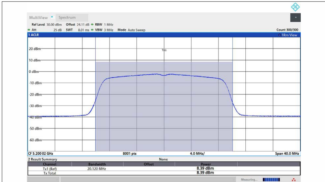
11N20MIMO-Ant2-5200-PASS
