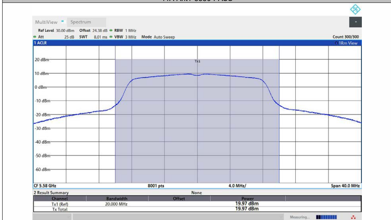
11A-Ant2-5580-PASS
