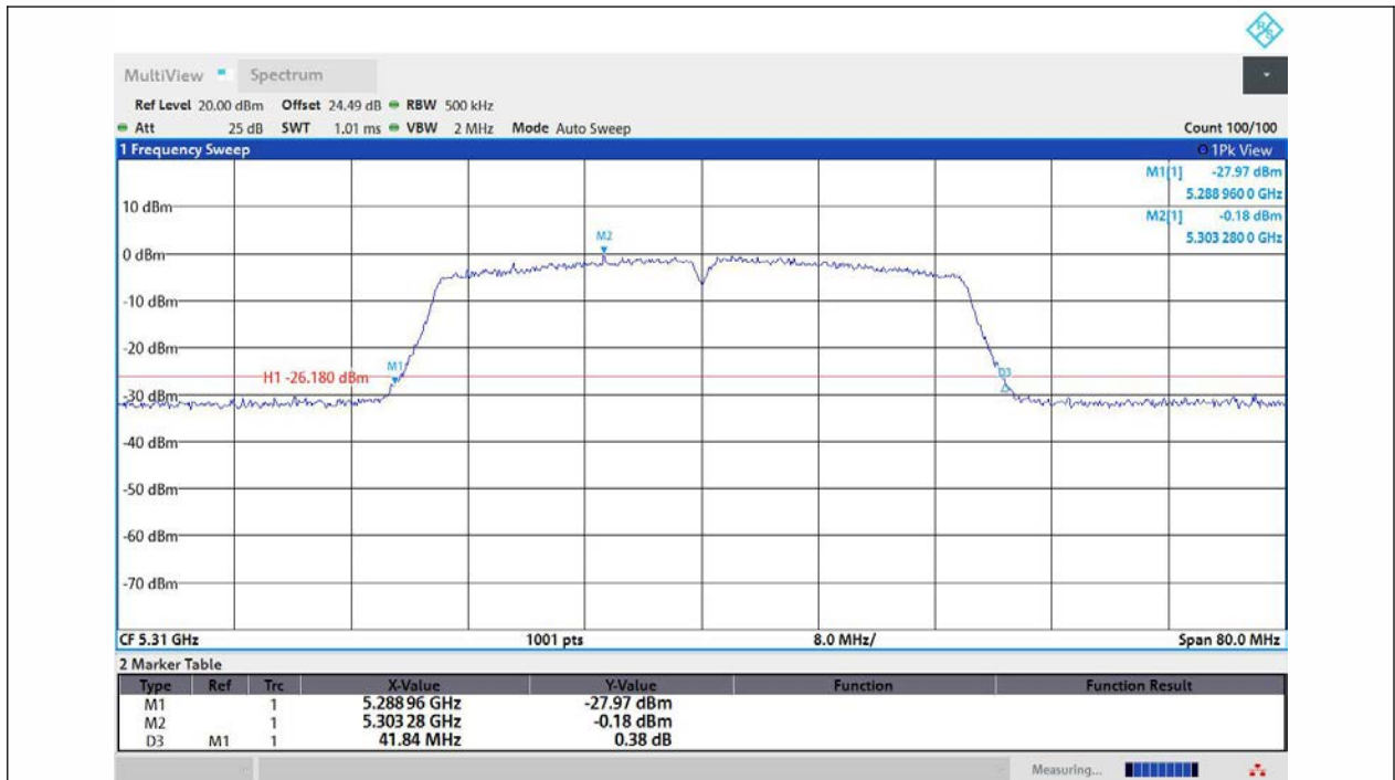
11AC40MIMO-Ant1-5310
