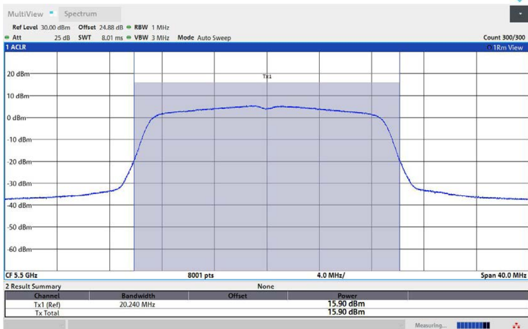
11AC20MIMO-Ant1-5500-PASS
