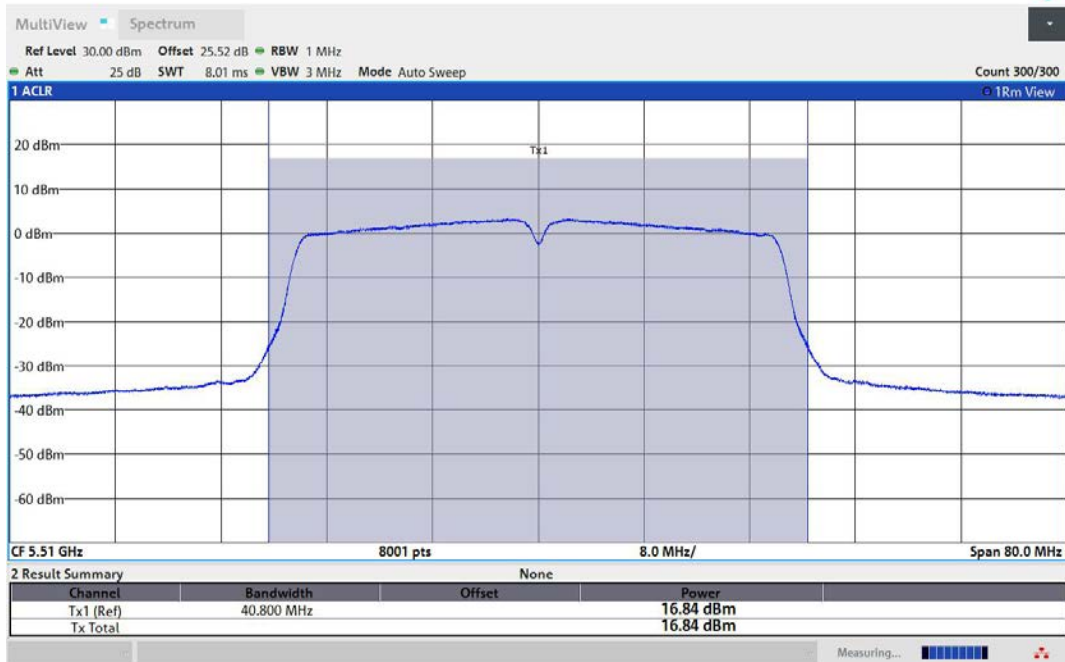
11AC40MIMO-Ant2-5510-PASS
