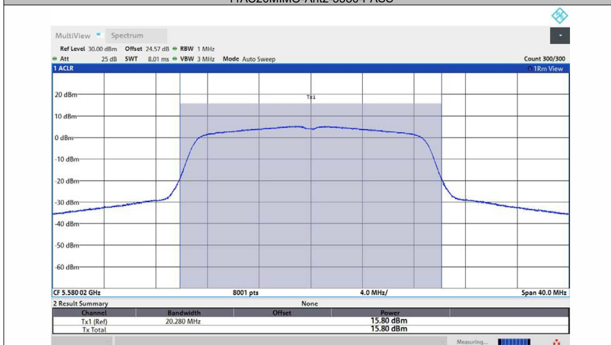
11AC20MIMO-Ant1-5580-PASS
