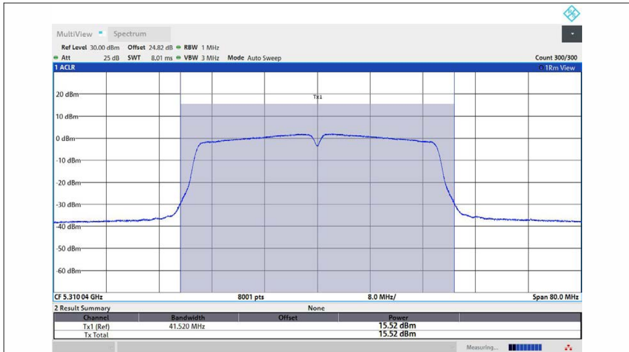
11N40MIMO-Ant1-5310-PASS
