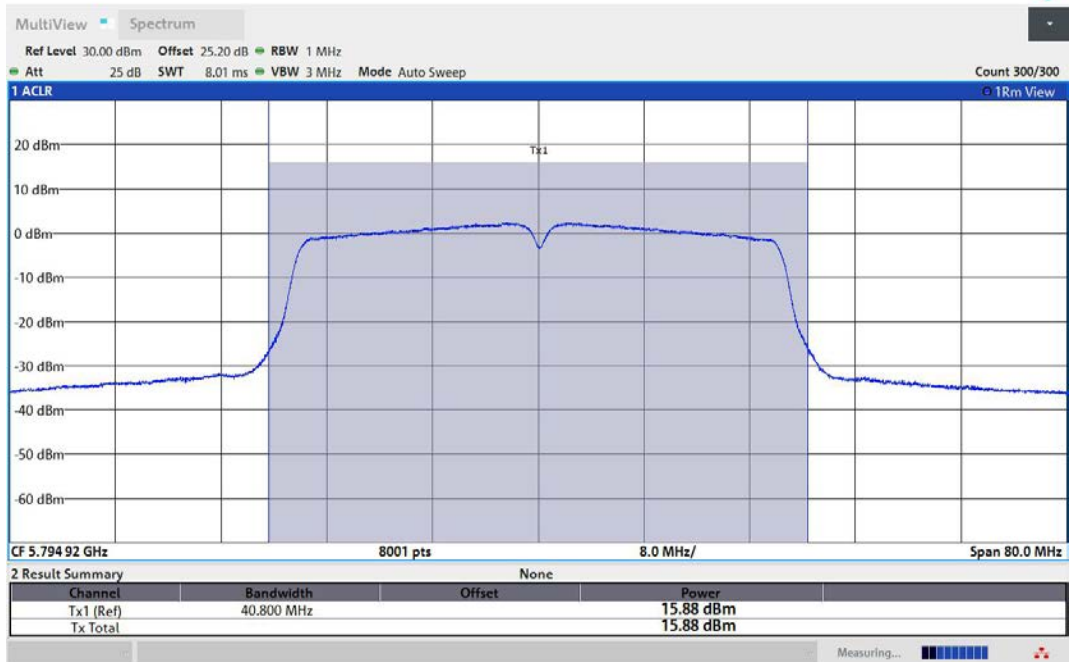
11AC40MIMO-Ant2-5795-PASS
