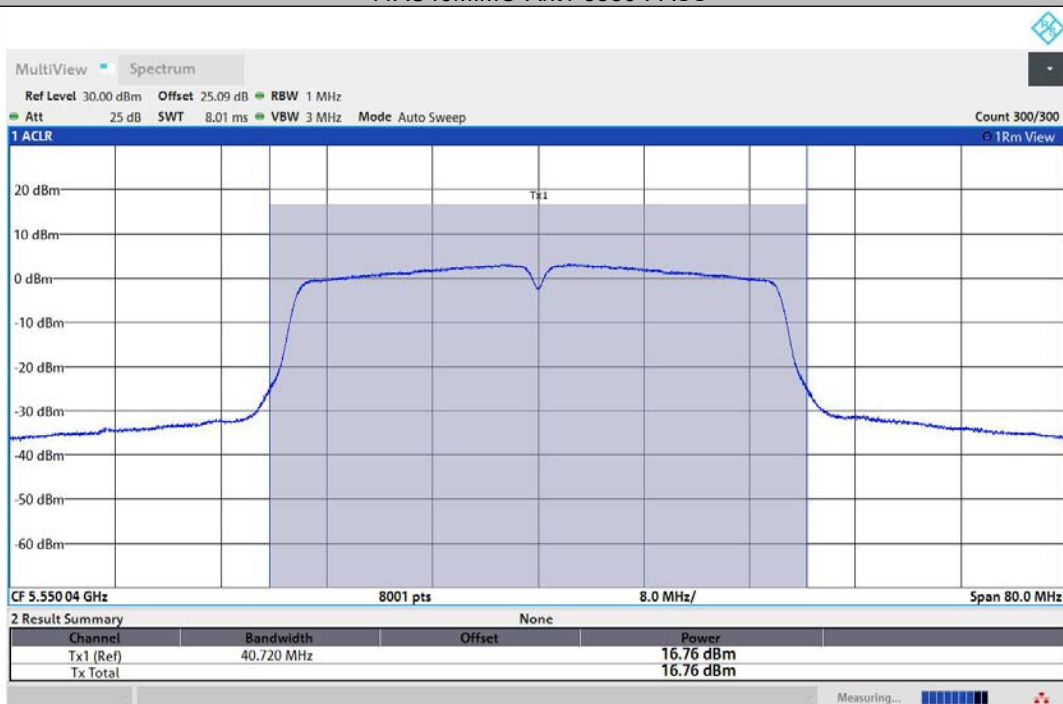
11AC40MIMO-Ant2-5550-PASS
