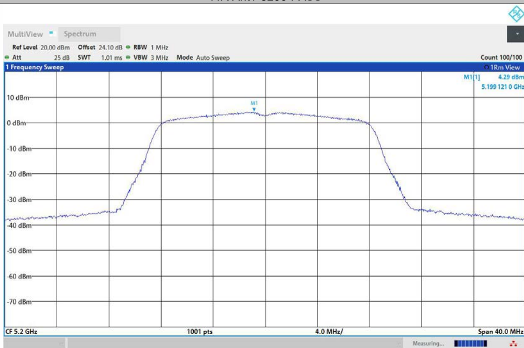
11A-Ant2-5200-PASS
