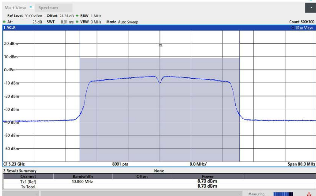
11N40MIMO-Ant2-5230-PASS
