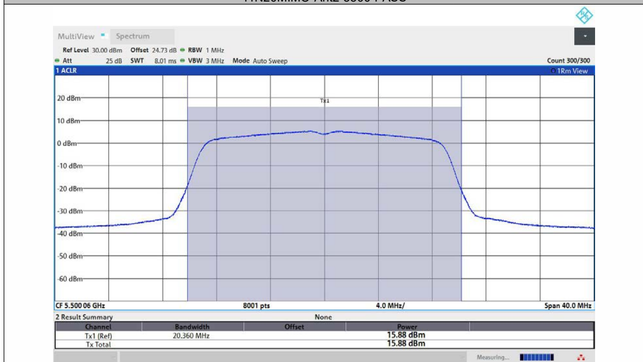
11N20MIMO-Ant1-5500-PASS
