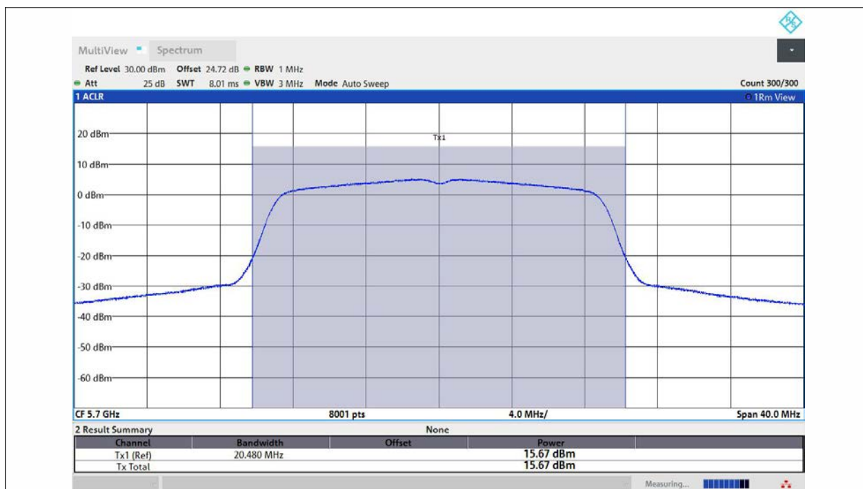
11AC20MIMO-Ant1-5700-PASS
