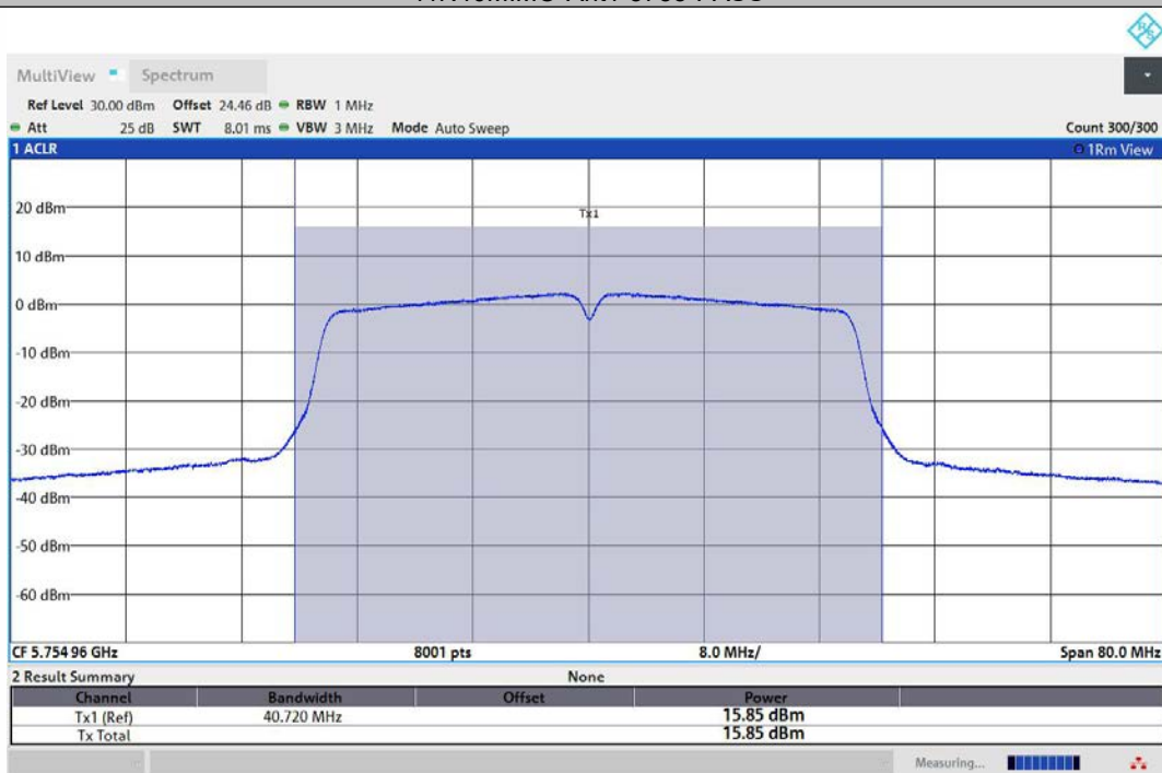
11N40MIMO-Ant2-5755-PASS
