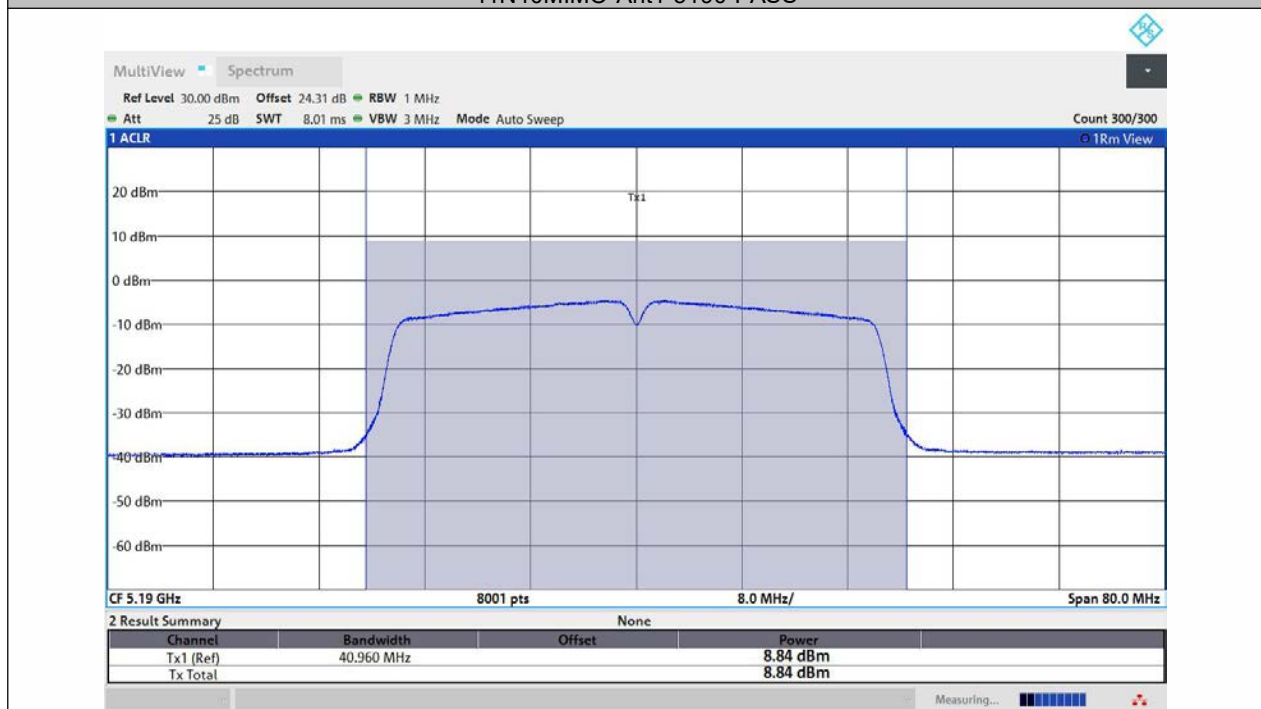
11N40MIMO-Ant2-5190-PASS
