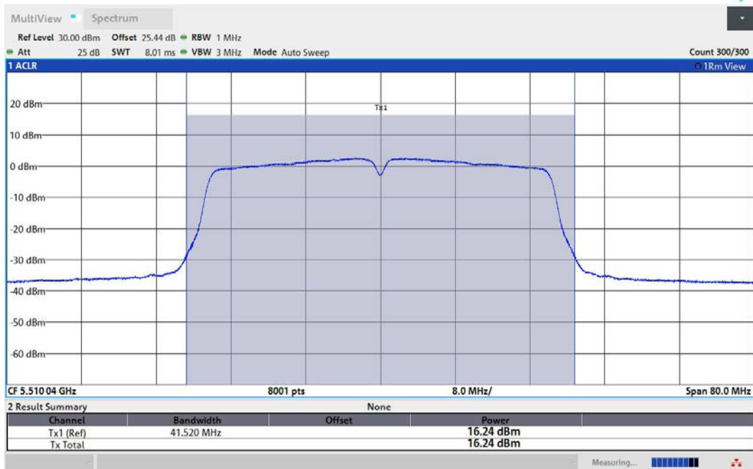
11AC40MIMO-Ant1-5510-PASS
