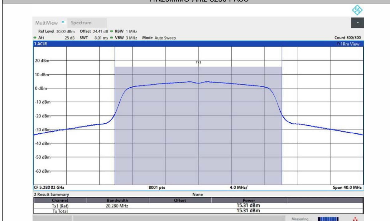
11N20MIMO-Ant1-5280-PASS
