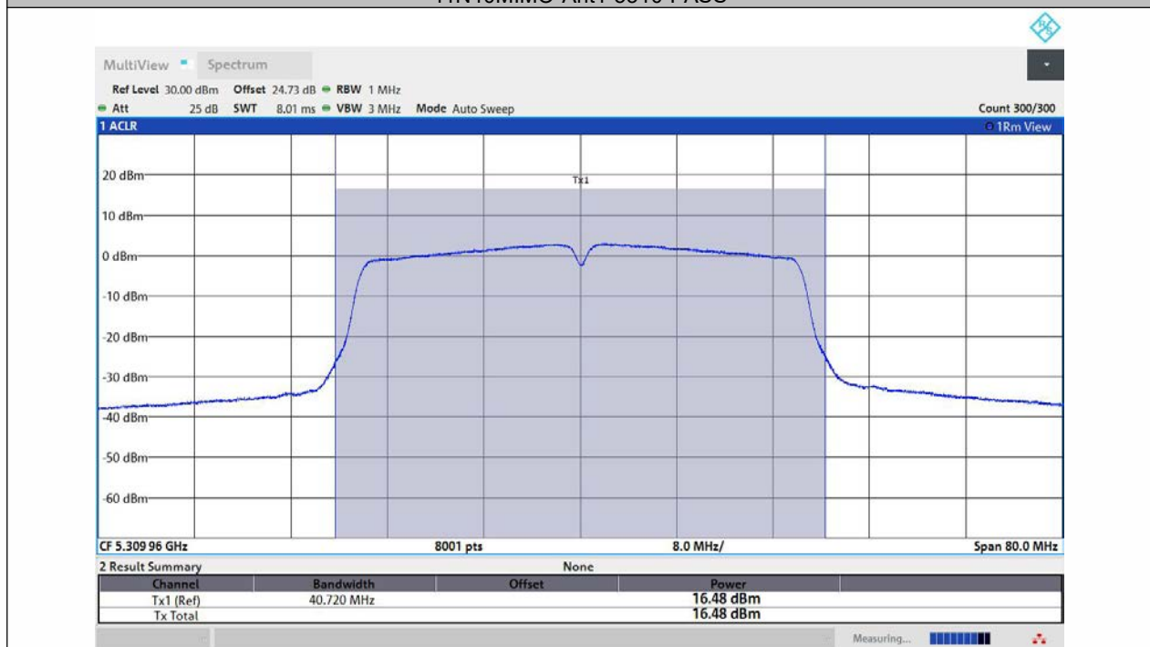
11N40MIMO-Ant2-5310-PASS
