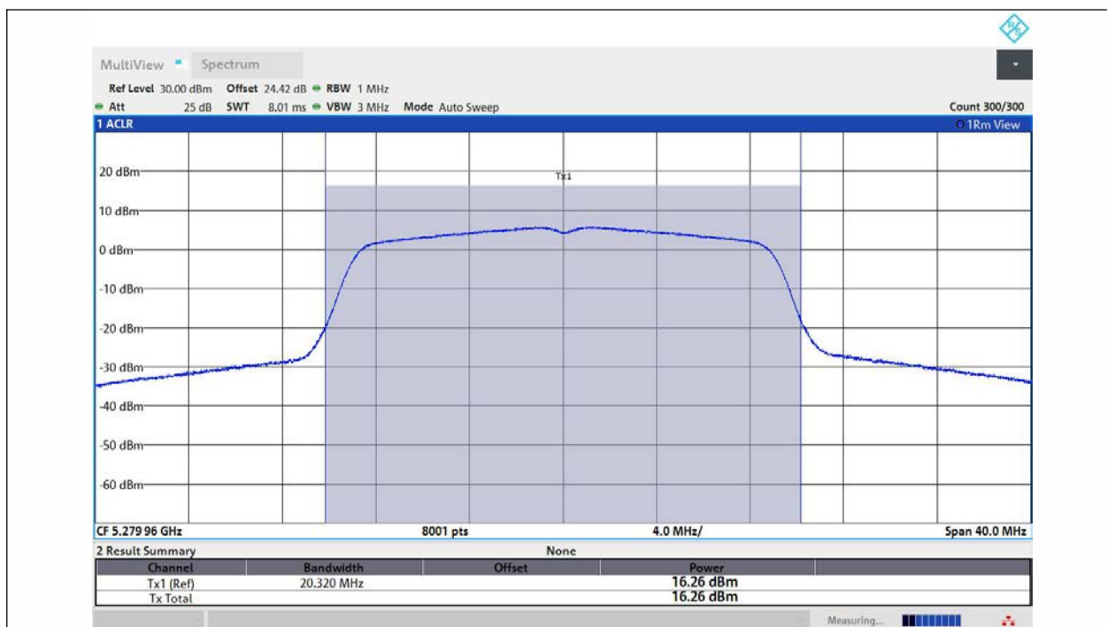
11N20MIMO-Ant2-5280-PASS
