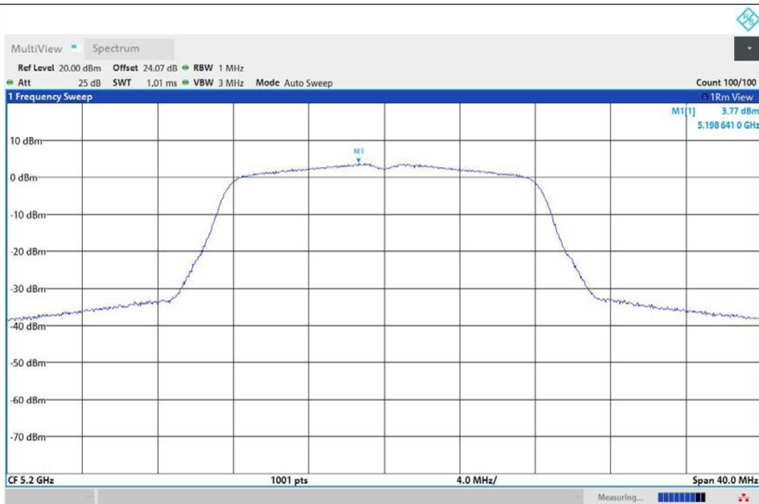
11A-Ant1-5200-PASS
