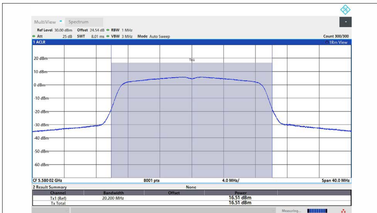
11AC20MIMO-Ant2-5580-PASS
