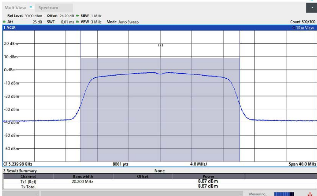
11N20MIMO-Ant2-5240-PASS
