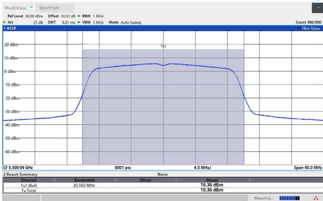
11AC20MIMO-Ant2-5500-PASS
