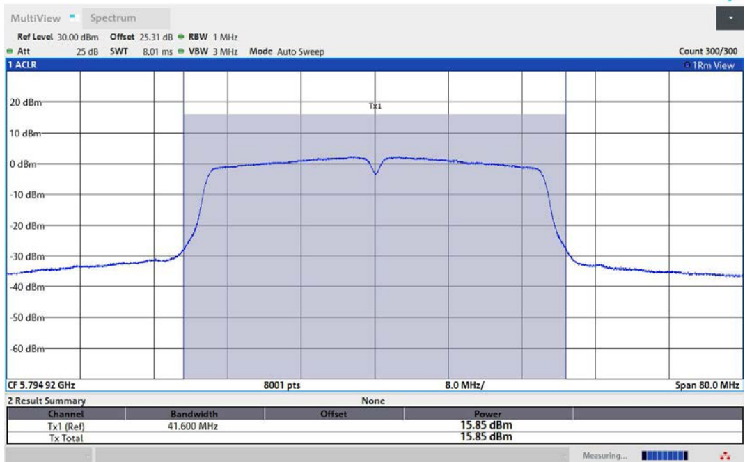
11AC40MIMO-Ant1-5795-PASS
