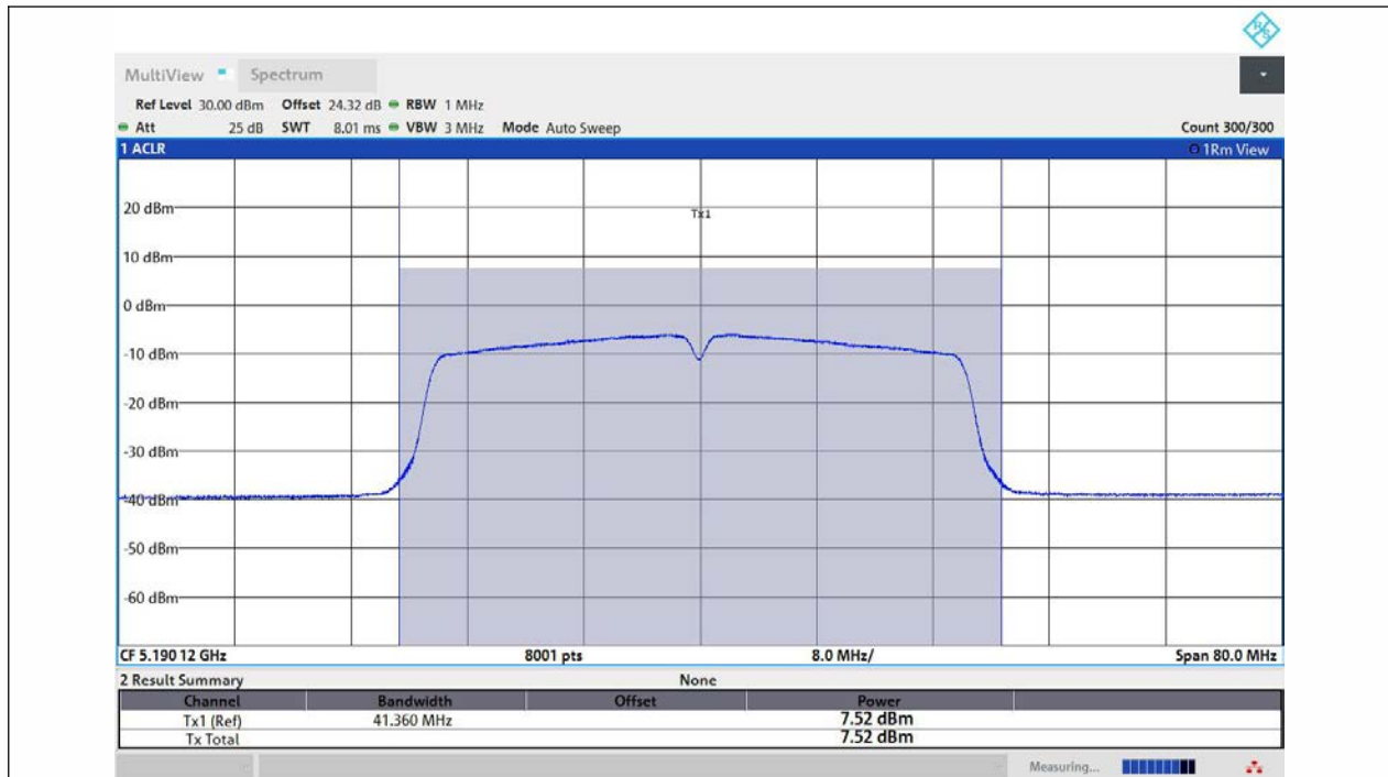
11N40MIMO-Ant1-5190-PASS
