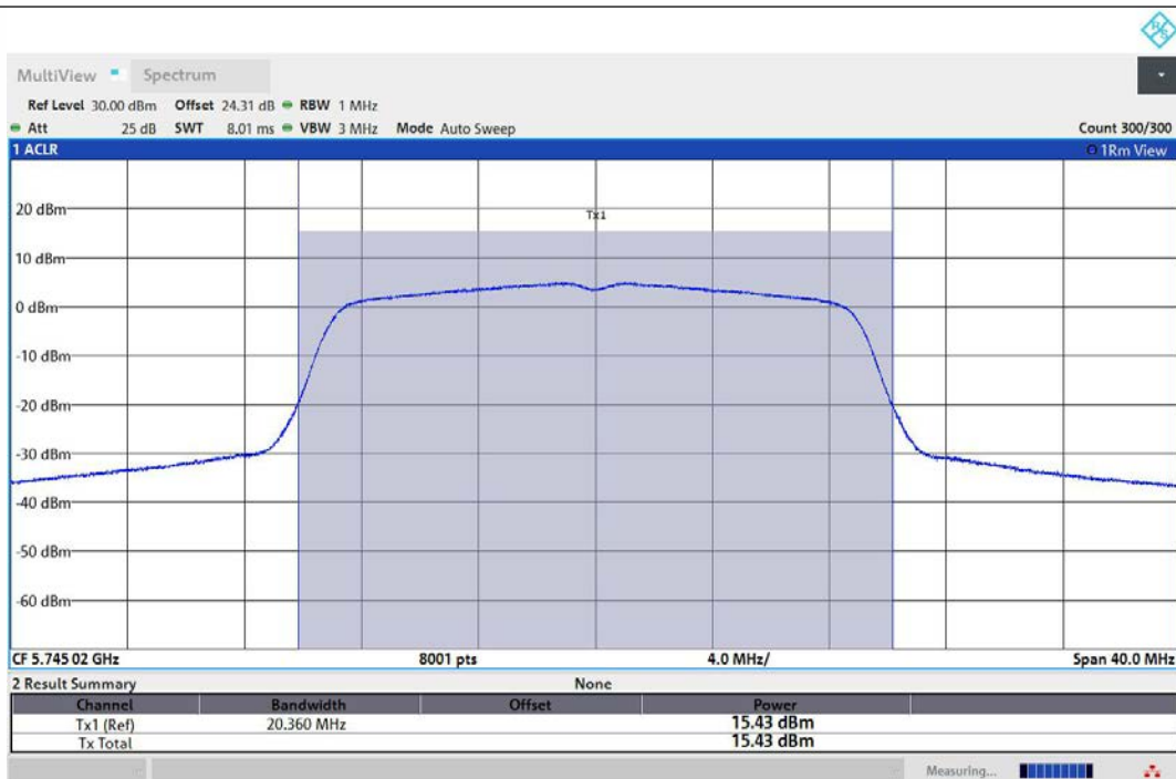
11N20MIMO-Ant1-5745-PASS
