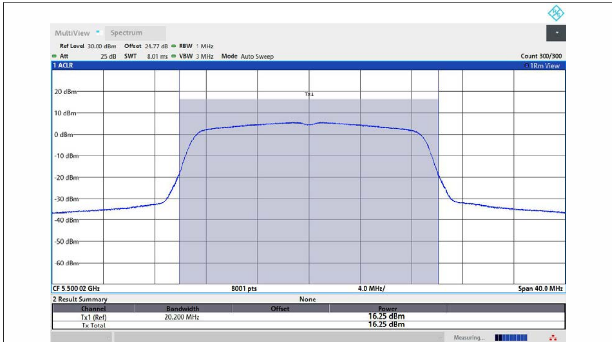
11N20MIMO-Ant2-5500-PASS
