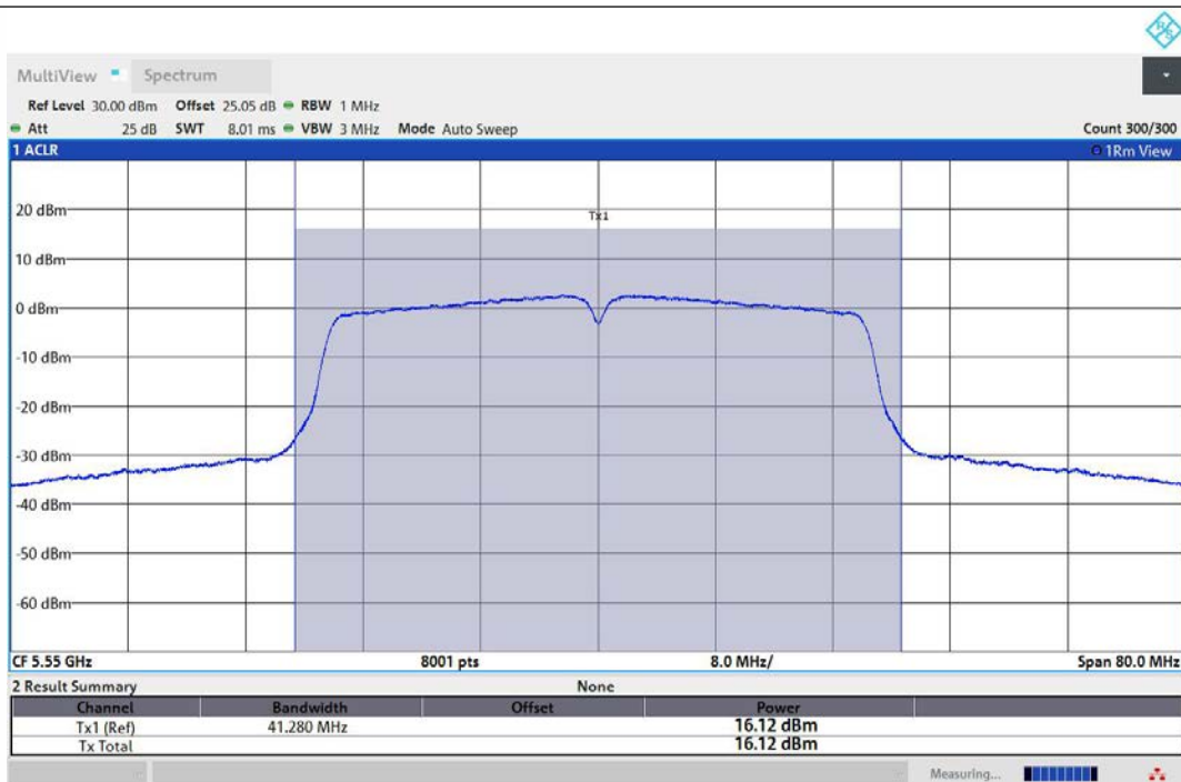
11AC40MIMO-Ant1-5550-PASS
