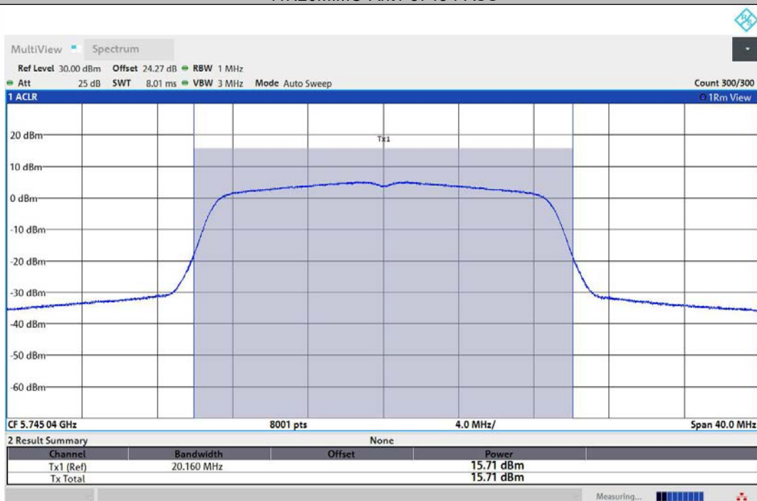
11N20MIMO-Ant2-5745-PASS
