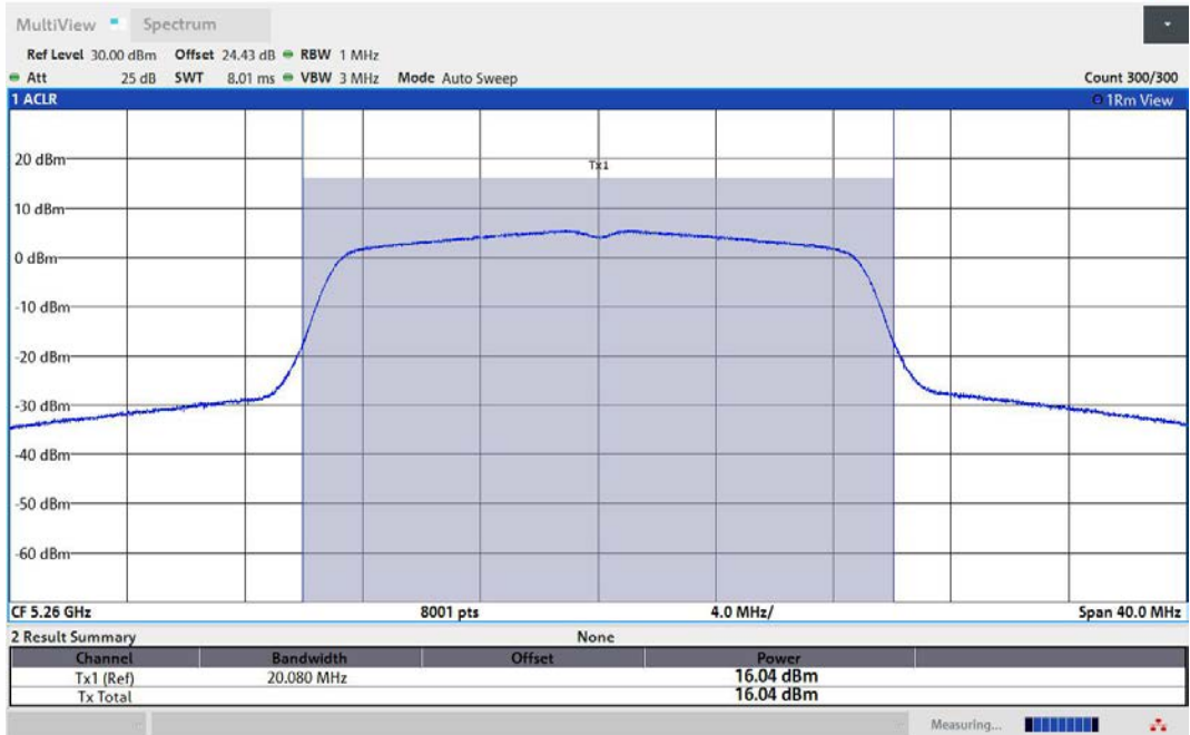
11N20MIMO-Ant2-5260-PASS
