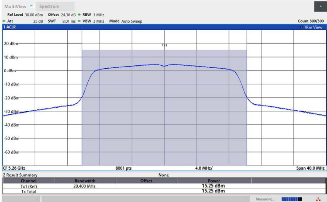
11N20MIMO-Ant1-5260-PASS
