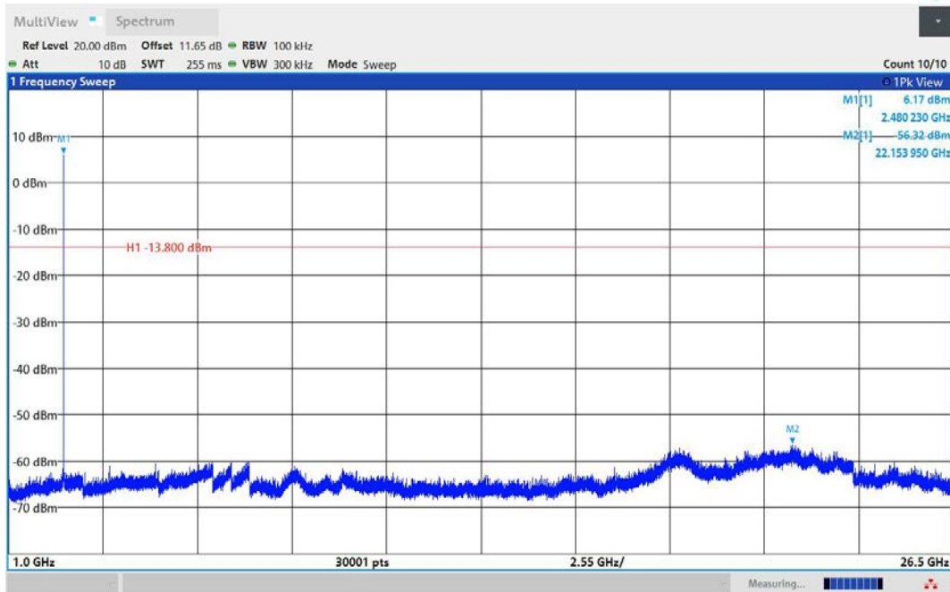
DH5-Ant1-2480-1000~26500-PASS
