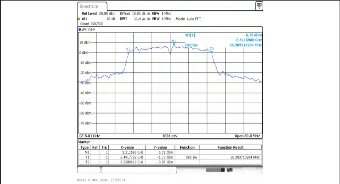
11N40MIMO-Ant2-5510
