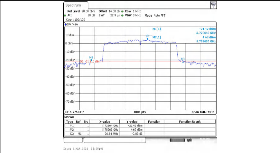
11AC80MIMO-Ant2-5775
