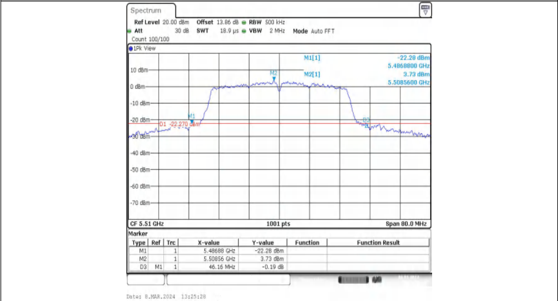
11N40MIMO-Ant2-5510
