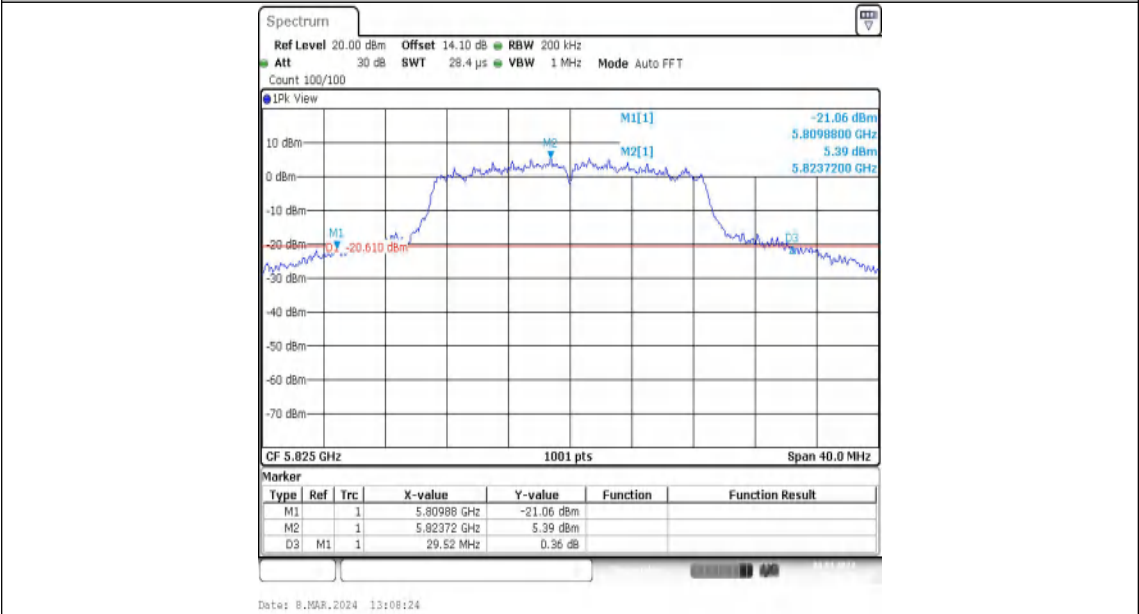
11N20MIMO-Ant2-5825
