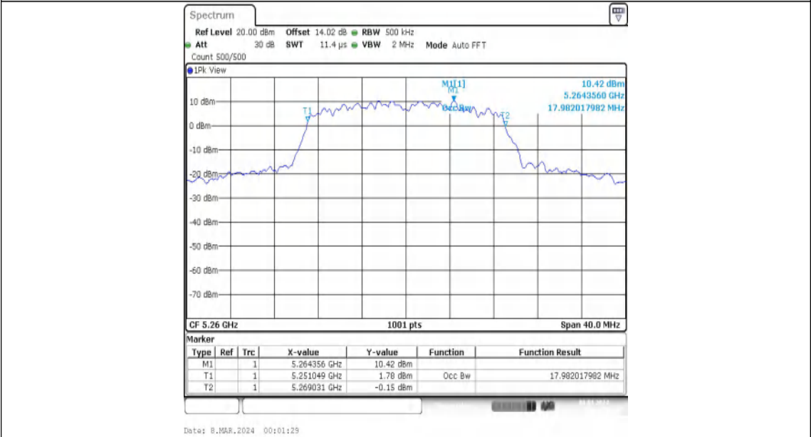
11N20MIMO-Ant2-5260
