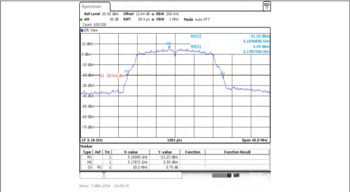
11A-Ant1-5180
