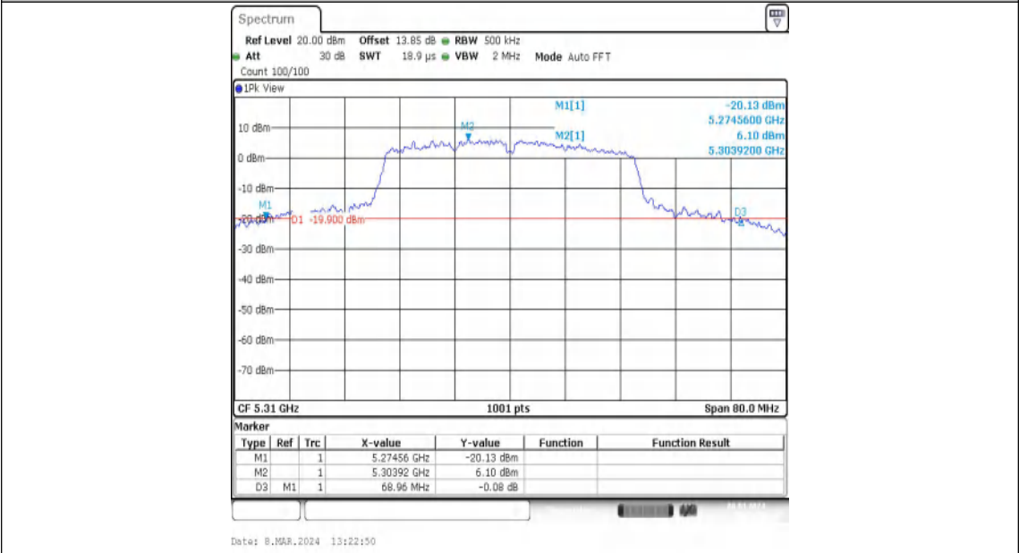
11N40MIMO-Ant2-5310
