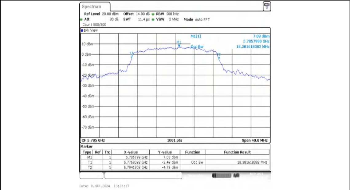
11N20MIMO-Ant2-5785
