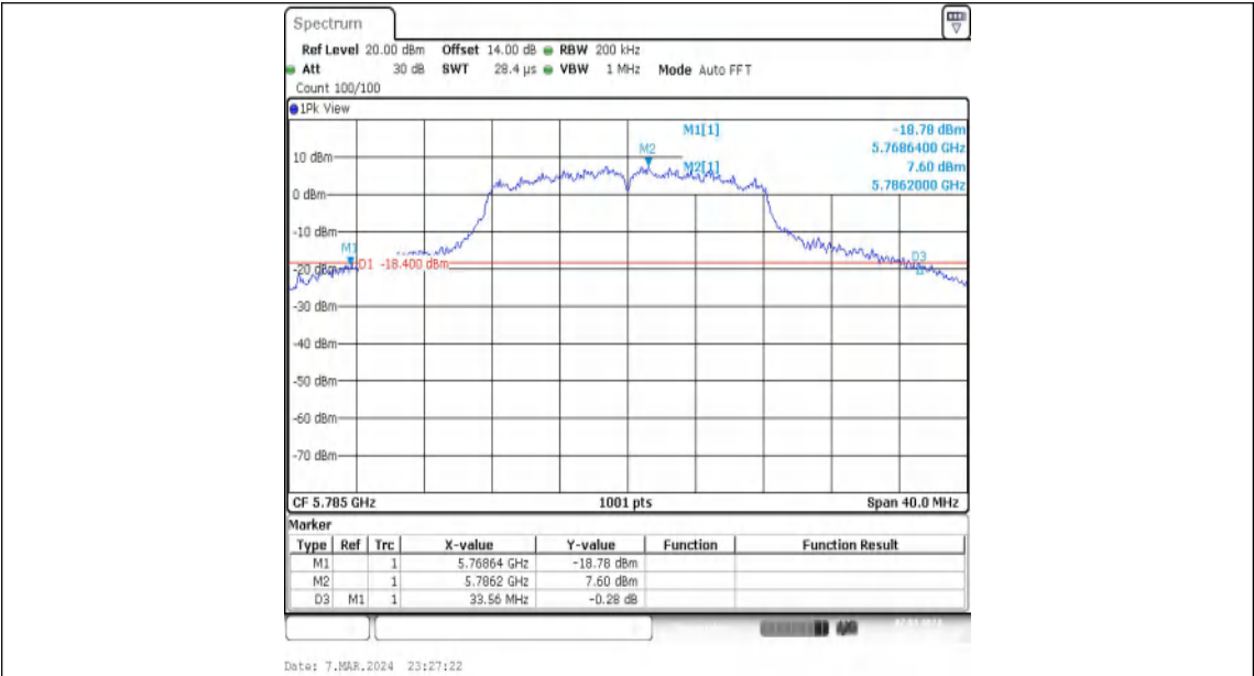
11A-Ant2-5785
