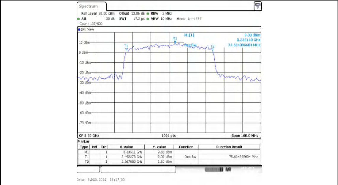
11AC80MIMO-Ant2-5530
