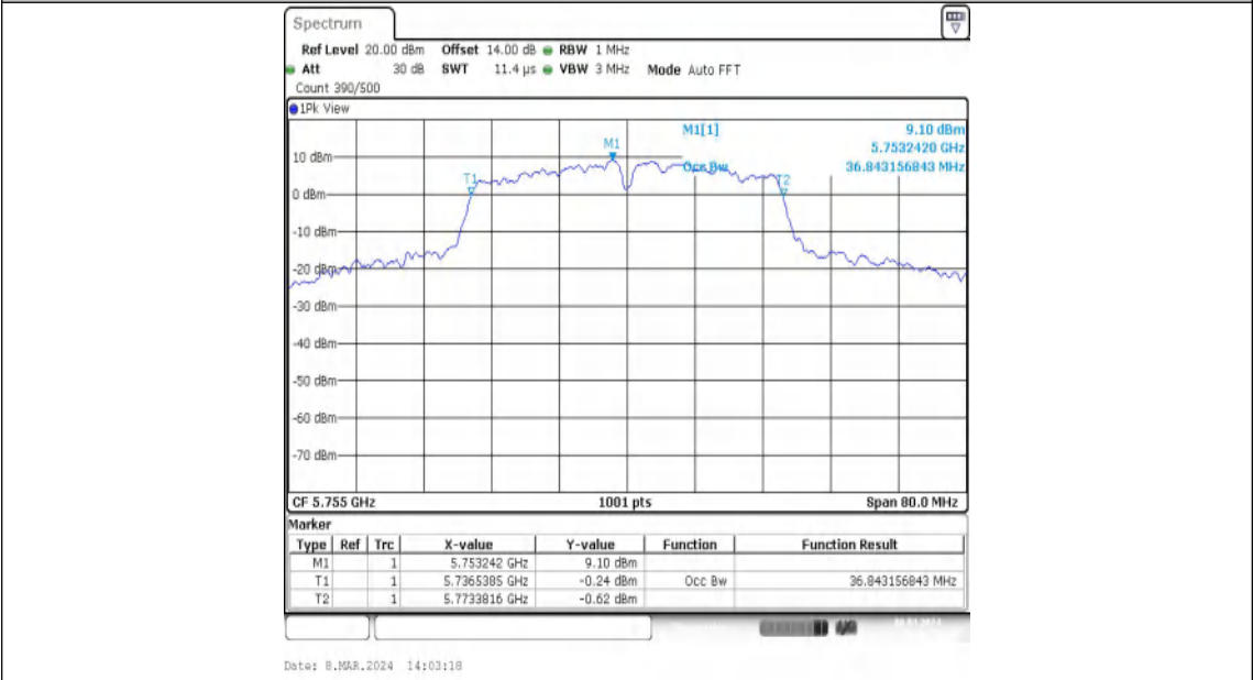
11N40MIMO-Ant2-5755
