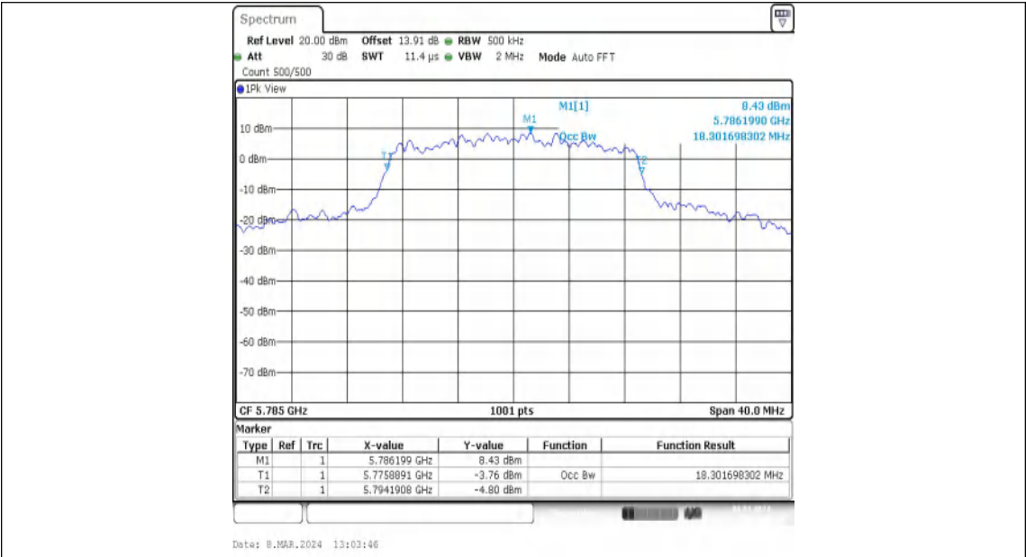
11N20MIMO-Ant1-5785
