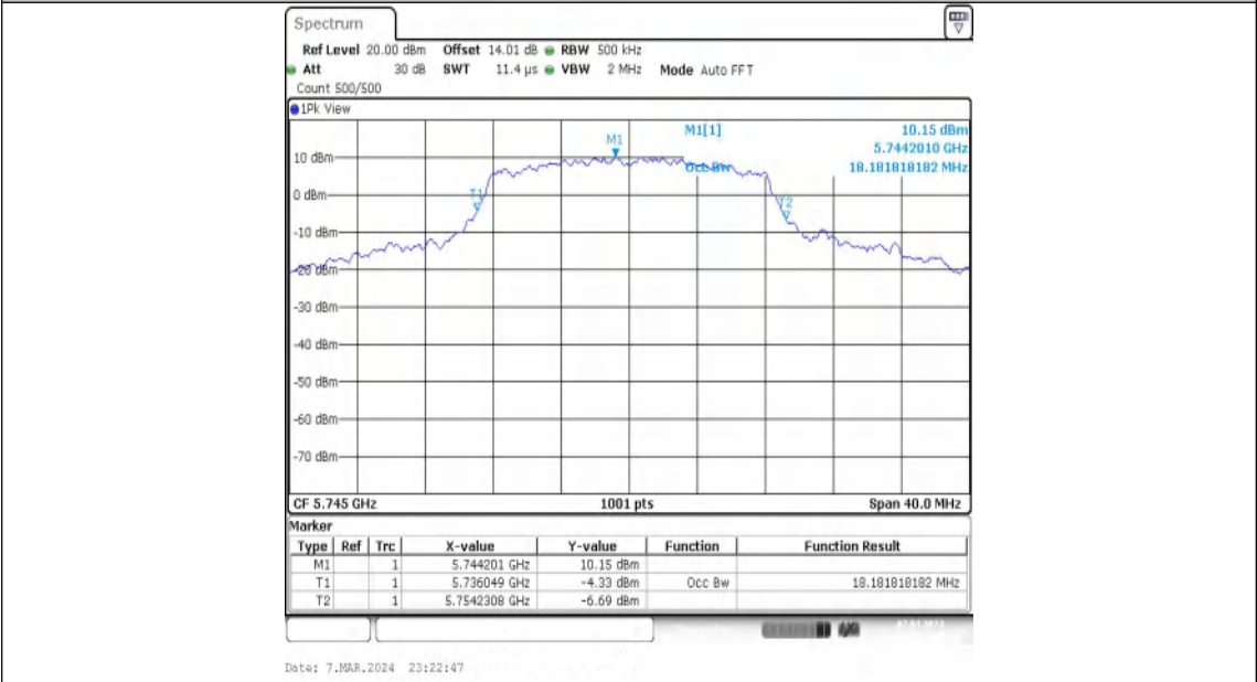
11A-Ant2-5745
