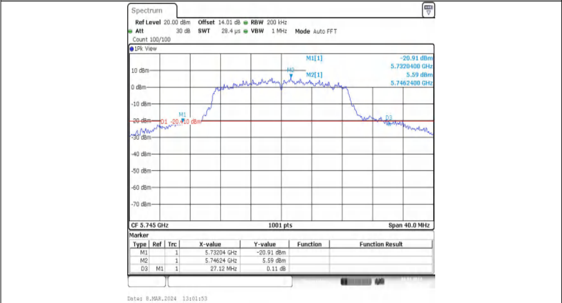
11N20MIMO-Ant2-5745
