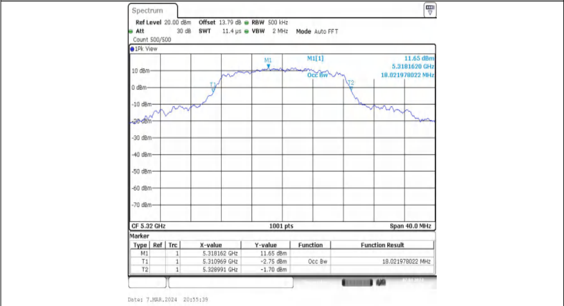
11A-Ant1-5320
