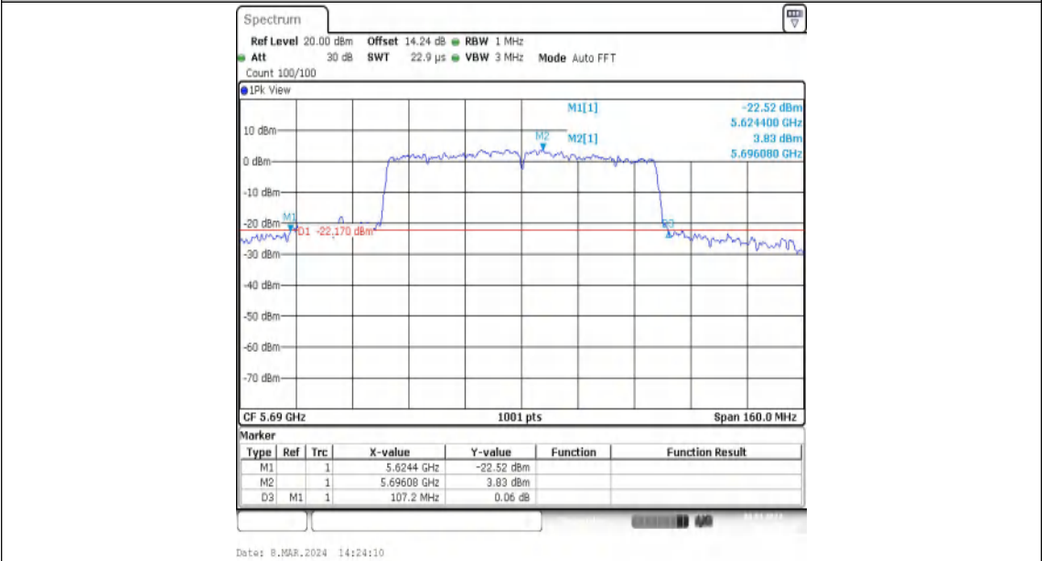
11AC80MIMO-Ant2-5690
