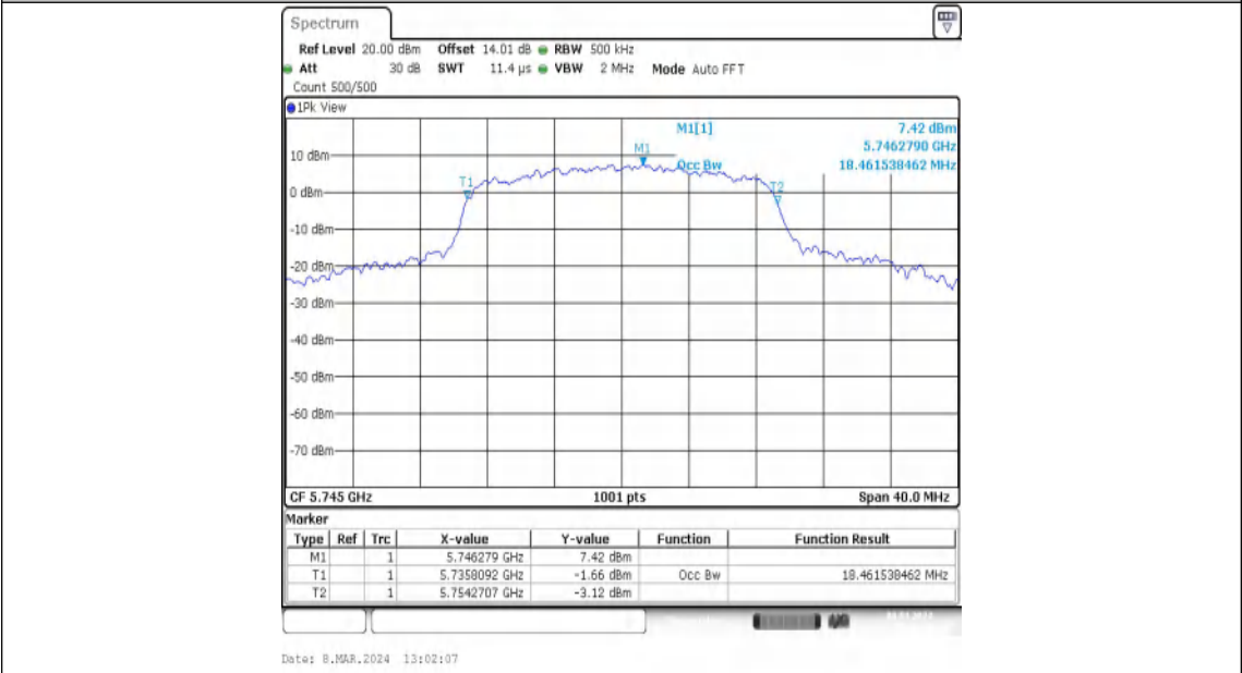
11N20MIMO-Ant2-5745
