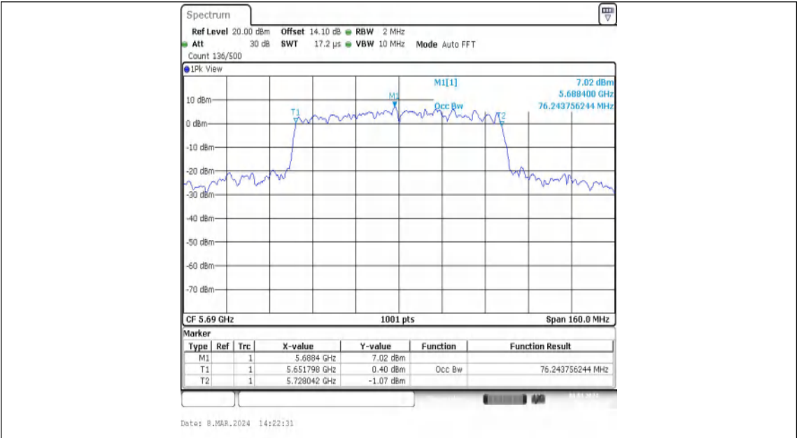
11AC80MIMO-Ant1-5690
