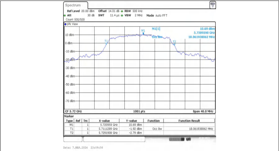
11A-Ant2-5720
