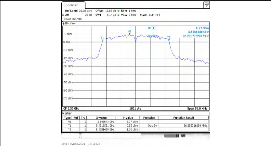
11N40MIMO-Ant2-5550
