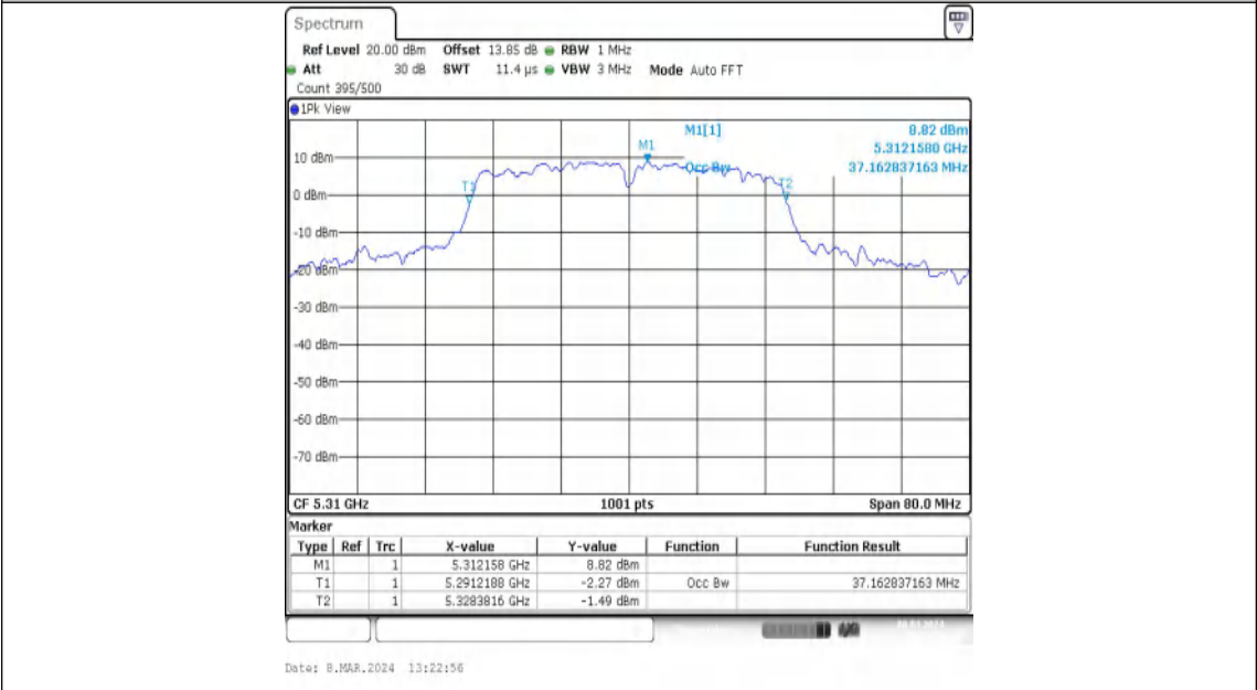
11N40MIMO-Ant2-5310
