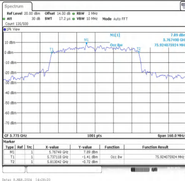
11AC80MIMO-Ant2-5775
