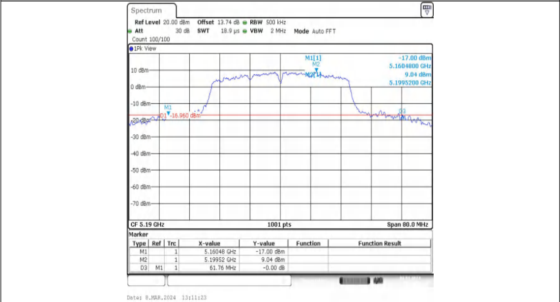
11N40MIMO-Ant2-5190
