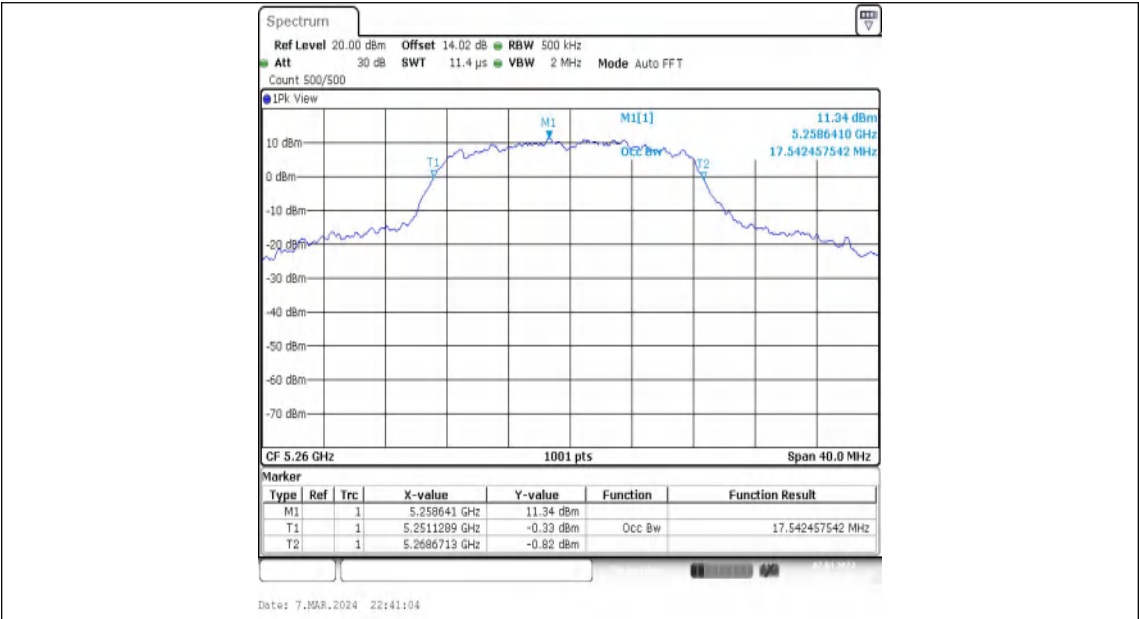
11A-Ant2-5260
