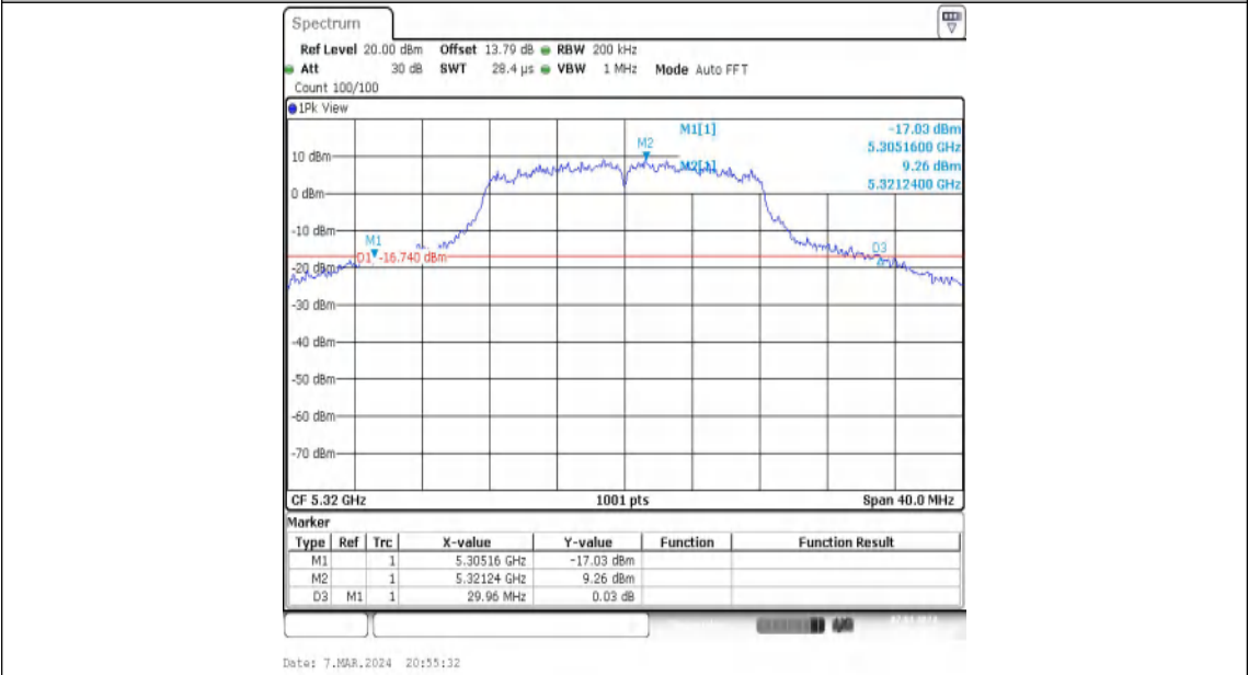
11A-Ant1-5320
