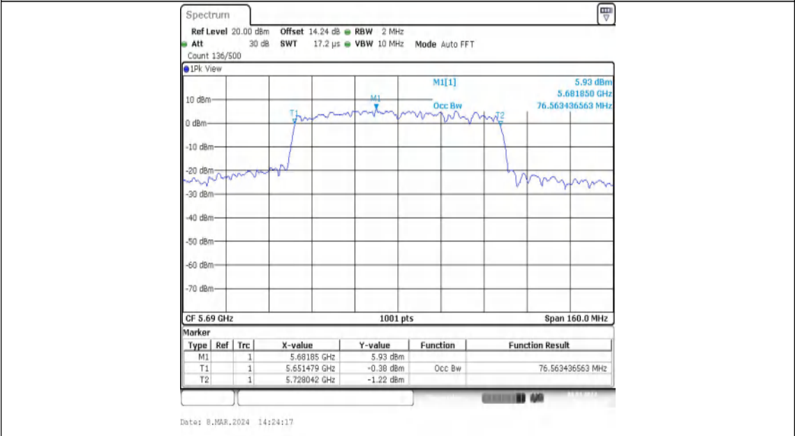
11AC80MIMO-Ant2-5690
