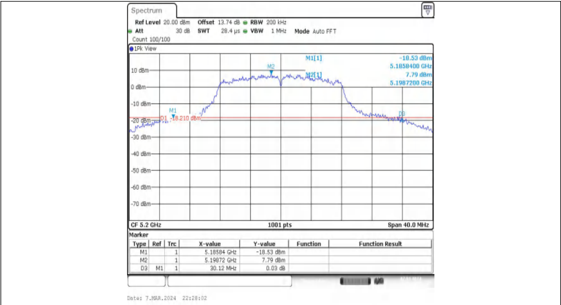
11A-Ant2-5200
