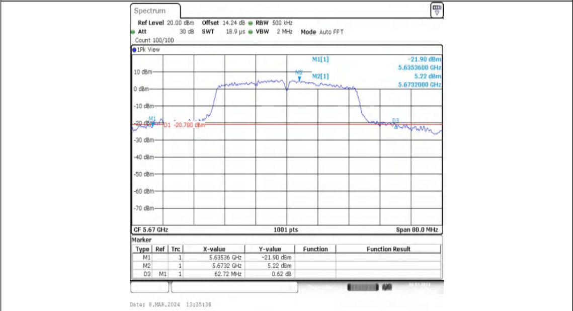
11N40MIMO-Ant2-5670
