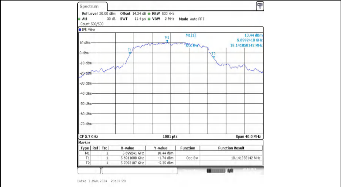
11A-Ant2-5700
