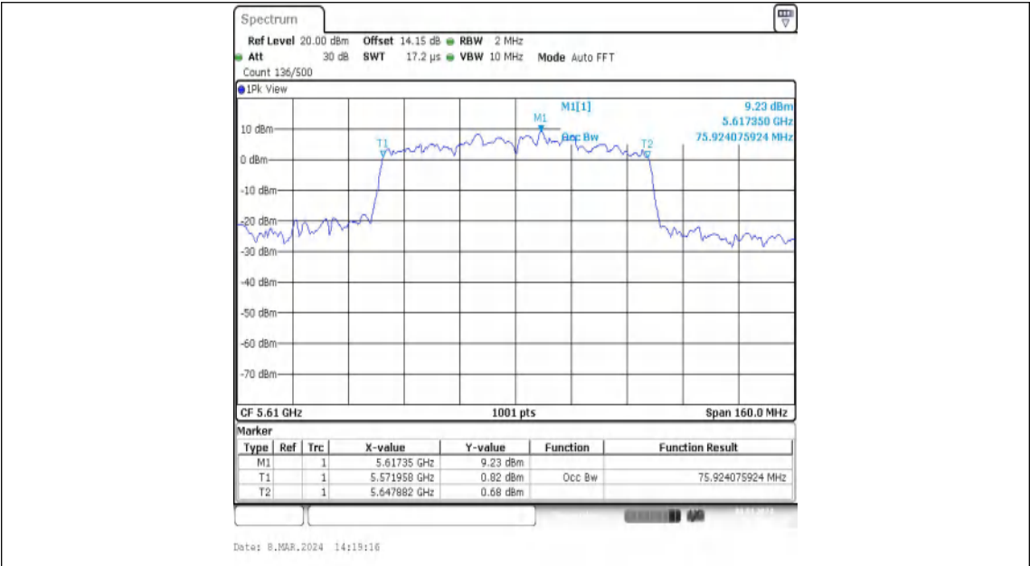
11AC80MIMO-Ant1-5610
