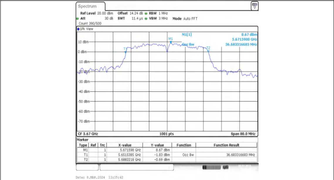
11N40MIMO-Ant2-5670
