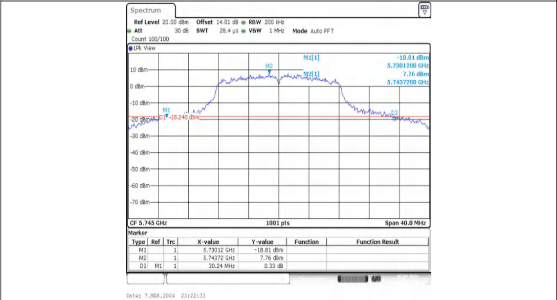
11A-Ant2-5745
