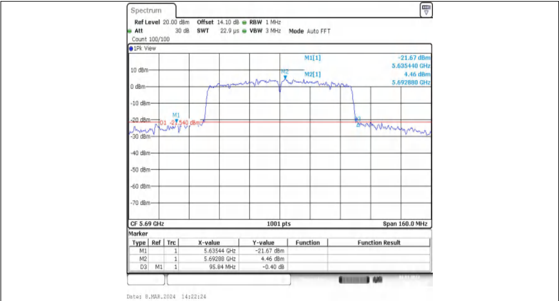
11AC80MIMO-Ant1-5690
