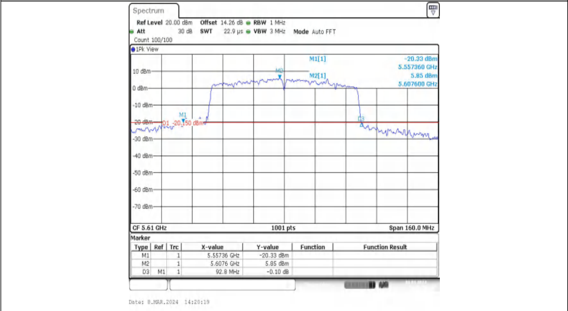
11AC80MIMO-Ant2-5610
