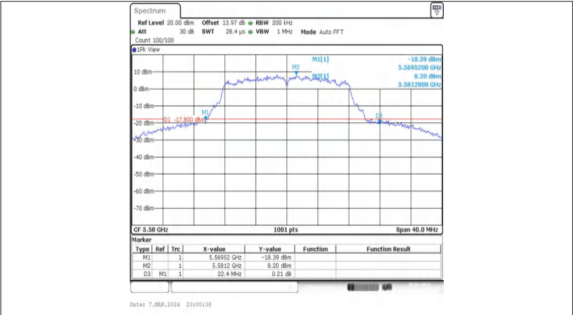
11A-Ant2-5580
