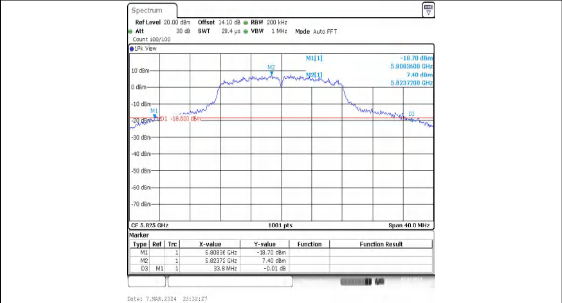
11A-Ant2-5825
