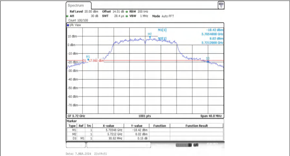
11A-Ant2-5720
