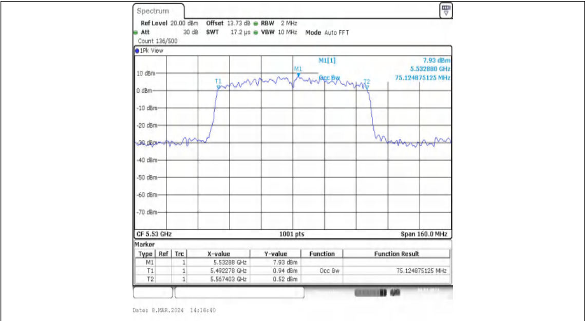
11AC80MIMO-Ant1-5530
