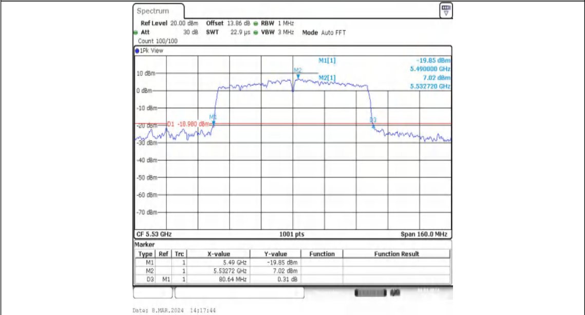
11AC80MIMO-Ant2-5530
