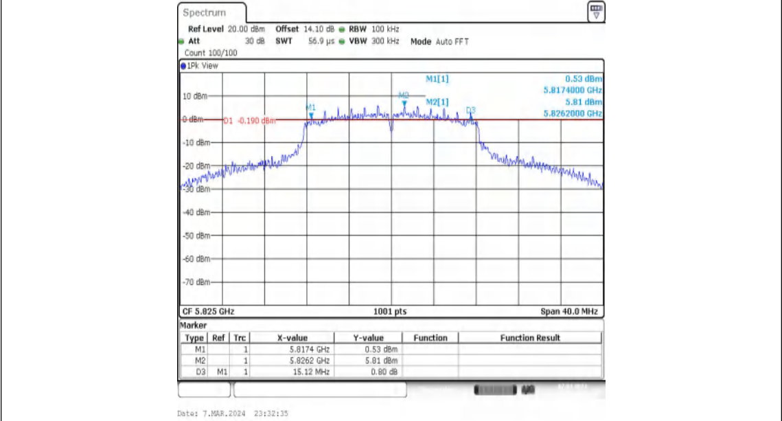
11A-Ant2-5825-PASS
