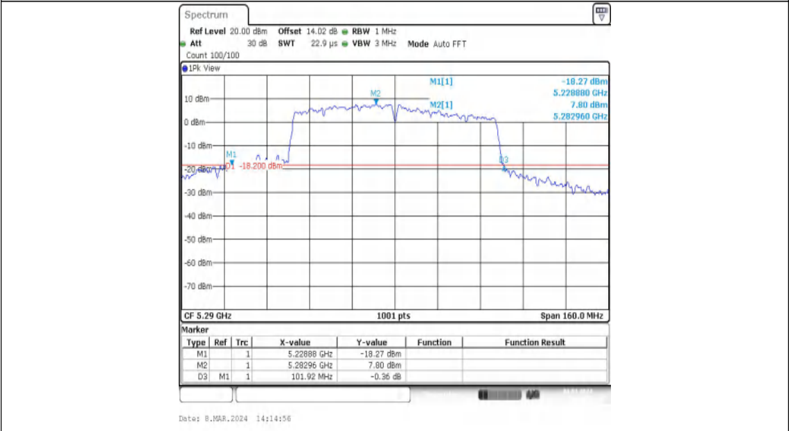
11AC80MIMO-Ant2-5290
