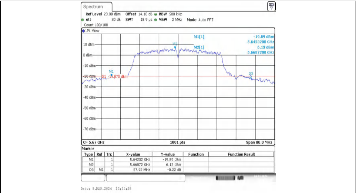
11N40MIMO-Ant1-5670
