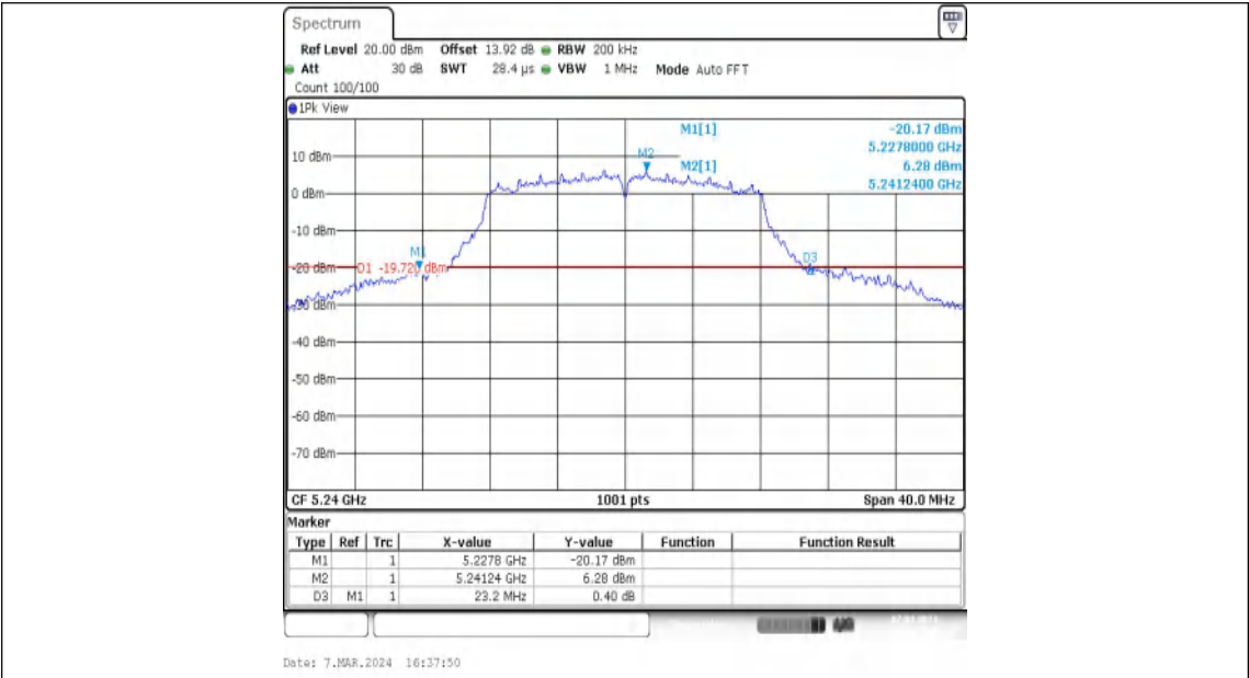
11A-Ant1-5240
