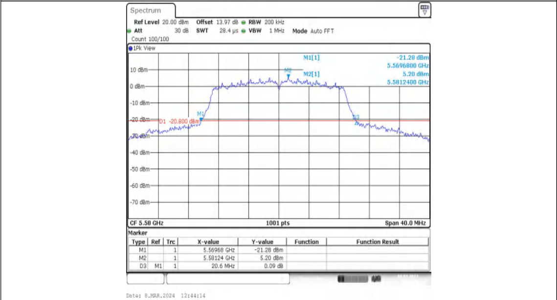
11N20MIMO-Ant2-5580
