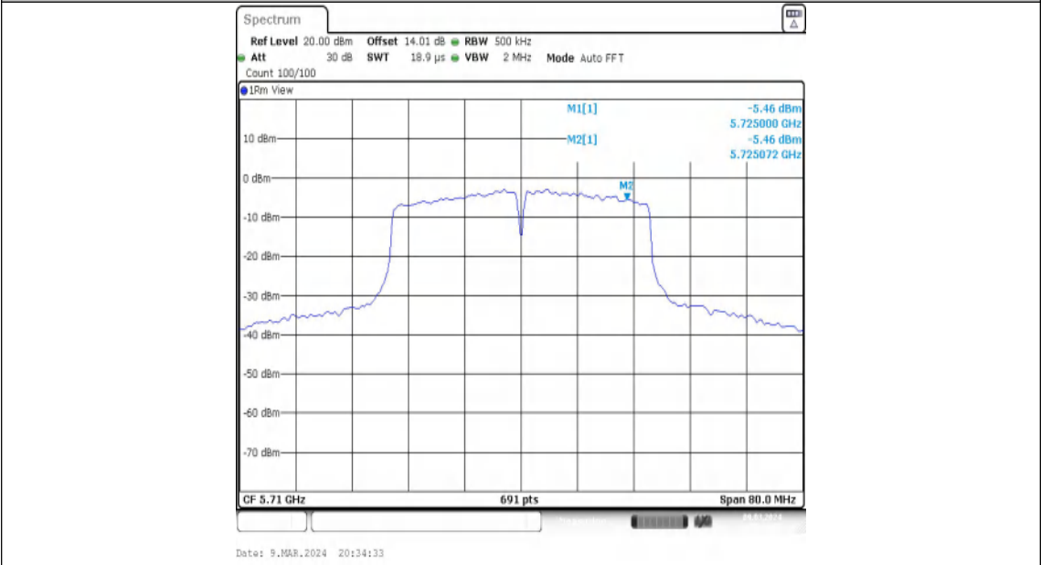
11N40MIMO-Ant2-5710_UNII-3-PASS
