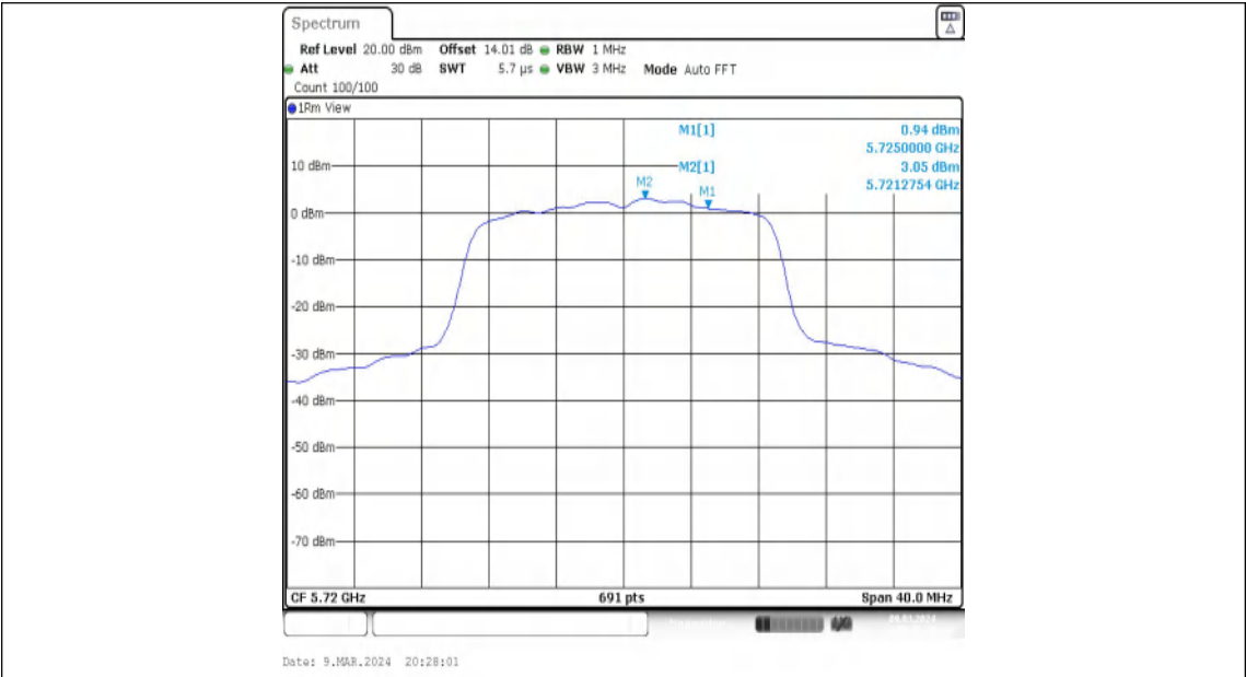
11N20MIMO-Ant2-5720_UNII-2C-PASS
