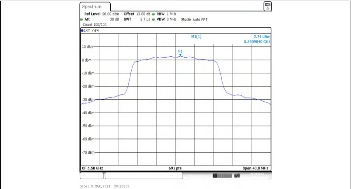
11N20MIMO-Ant1-5580-PASS
