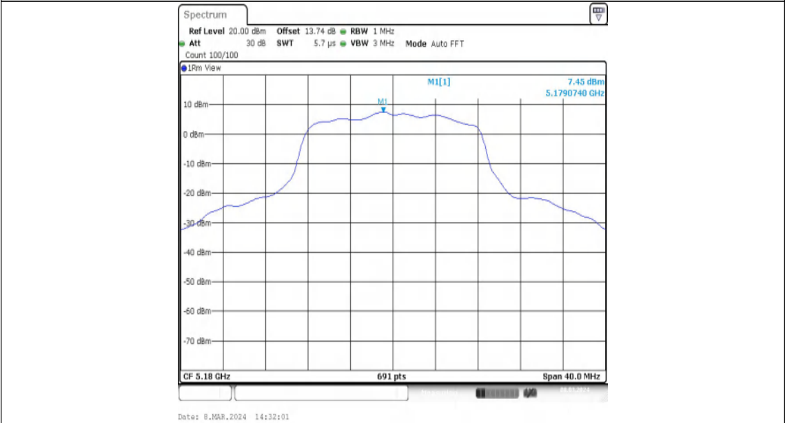
11A-Ant2-5180-PASS
