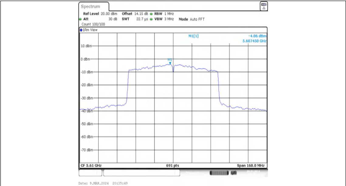
11AC80MIMO-Ant1-5610-PASS
