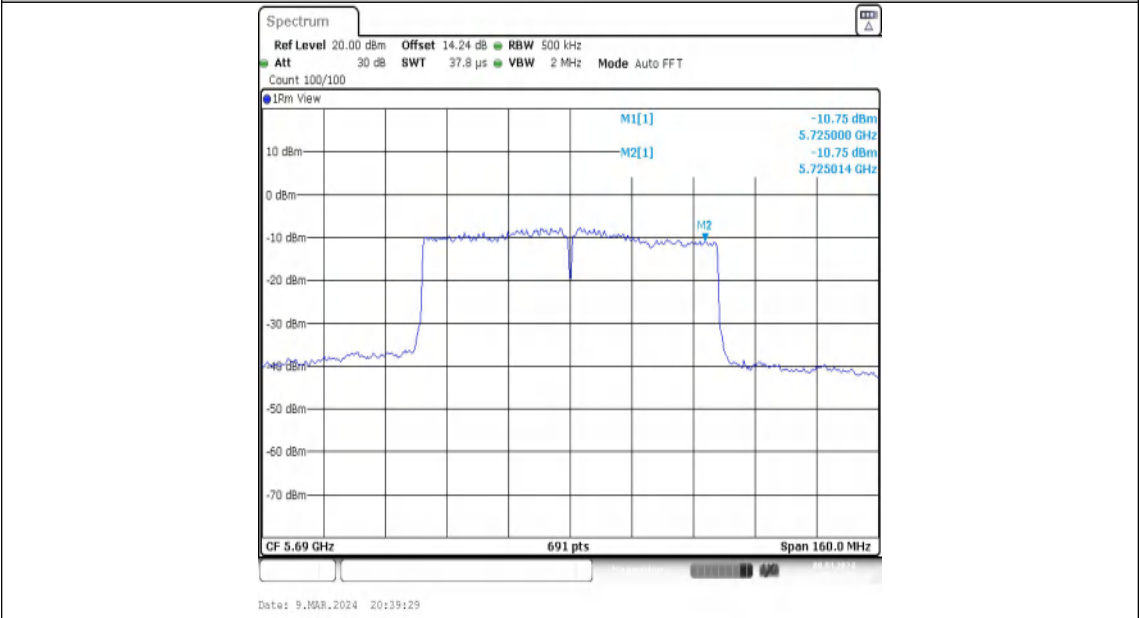
11AC80MIMO-Ant2-5690_UNII-3-PASS
