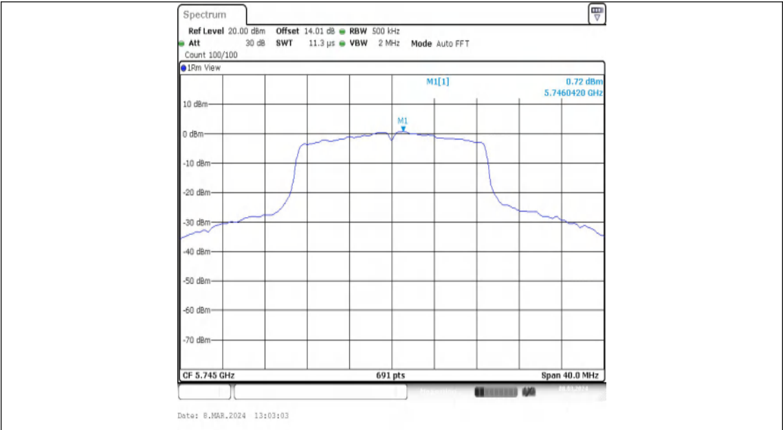
11N20MIMO-Ant2-5745-PASS
