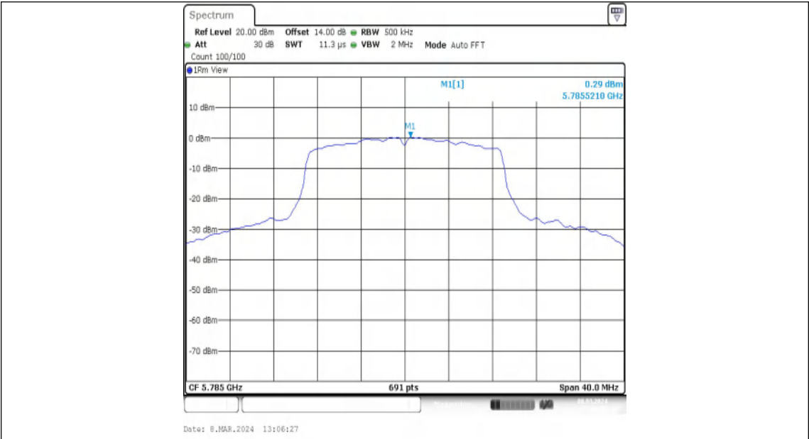
11N20MIMO-Ant2-5785-PASS
