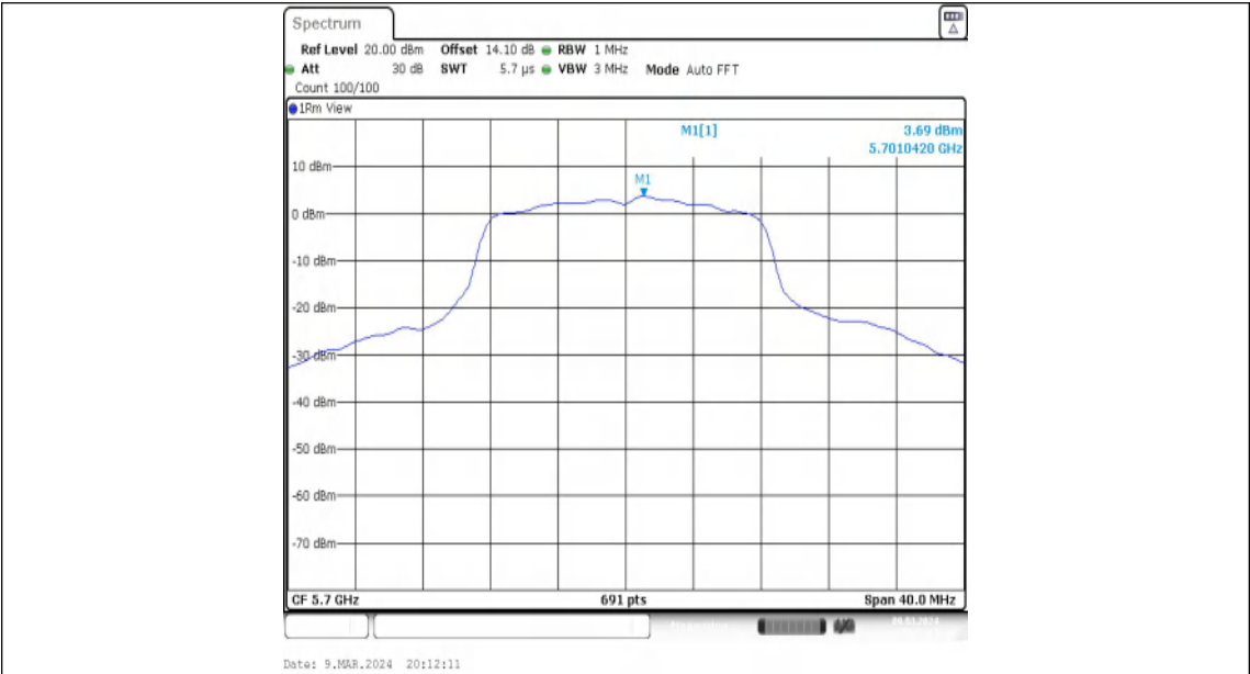
11A-Ant1-5700-PASS
