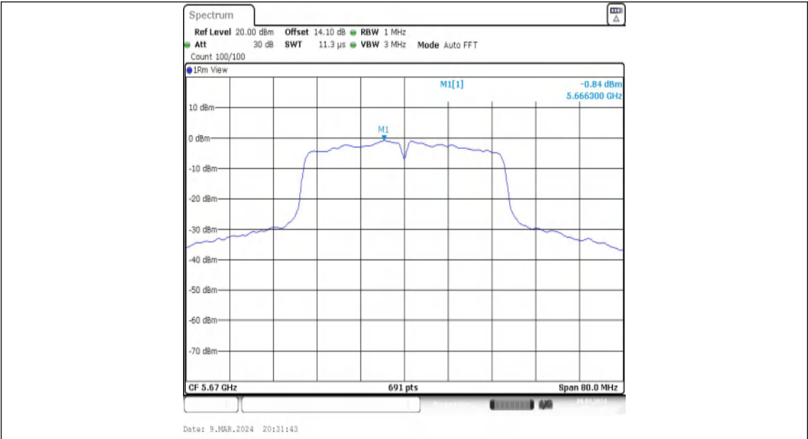
11N40MIMO-Ant1-5670-PASS
