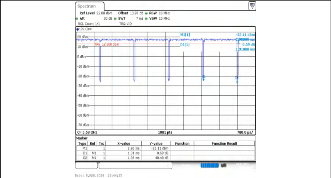
NTNV-11N20MIMO-Ant2-5580
