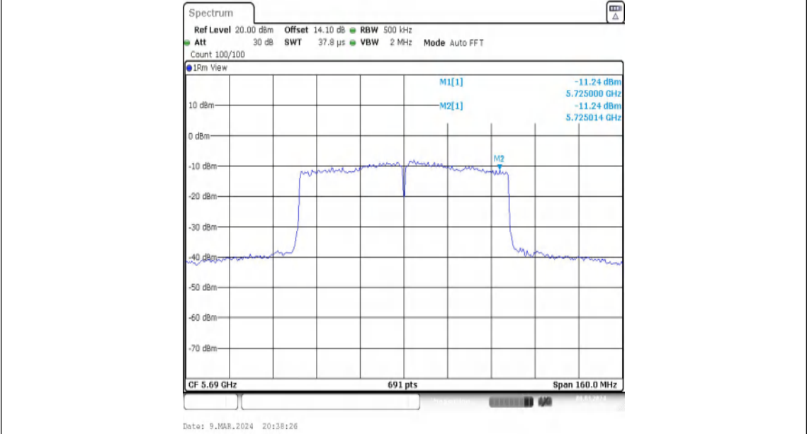
11AC80MIMO-Ant1-5690_UNII-3-PASS
