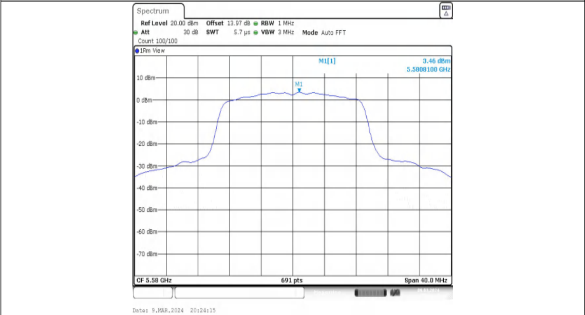
11N20MIMO-Ant2-5580-PASS
