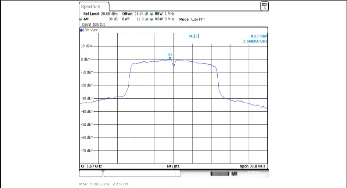
11N40MIMO-Ant2-5670-PASS
