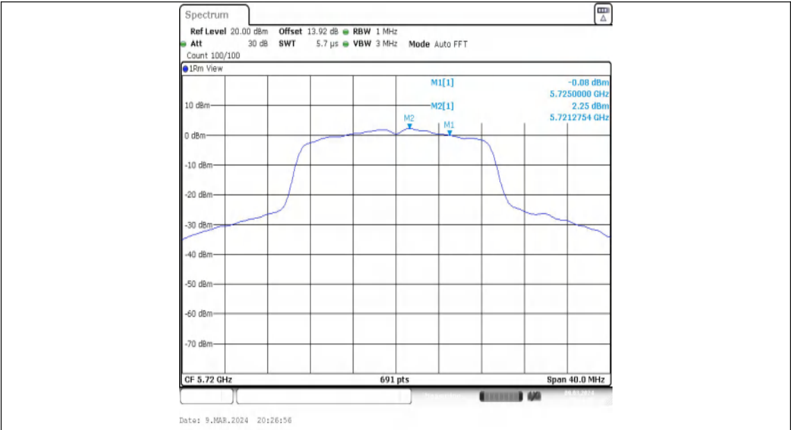
11N20MIMO-Ant1-5720_UNII-2C-PASS
