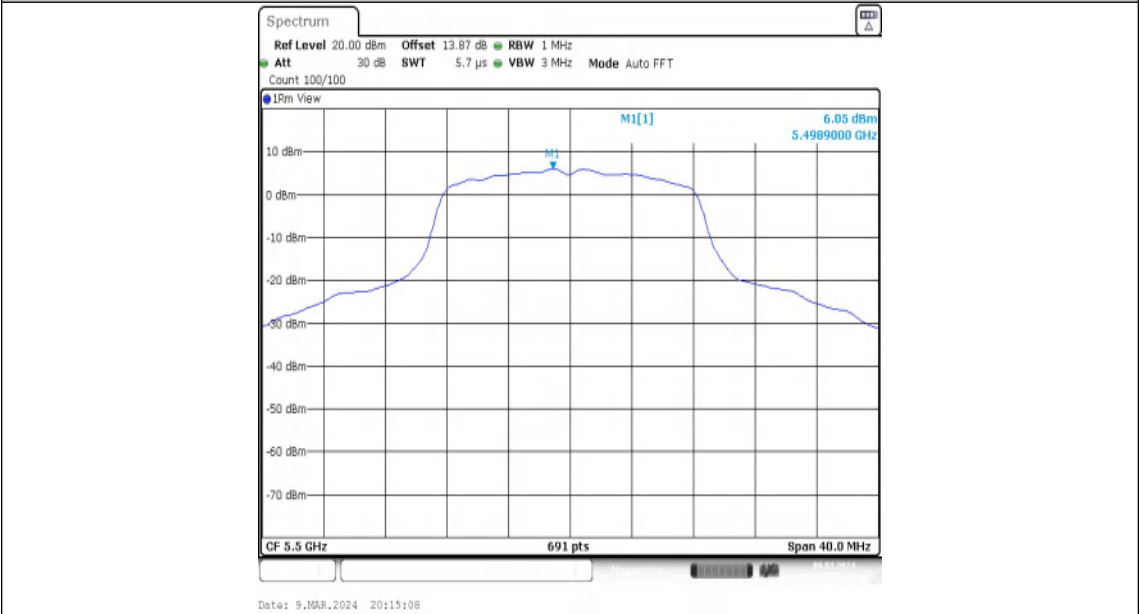
11A-Ant2-5500-PASS
