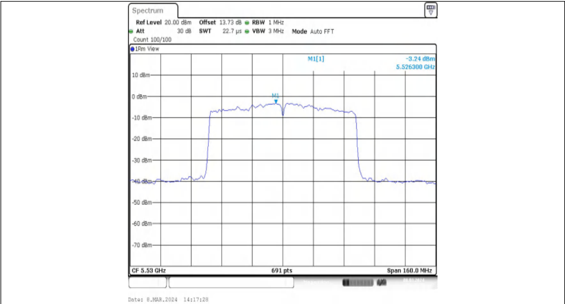
11AC80MIMO-Ant1-5530-PASS
