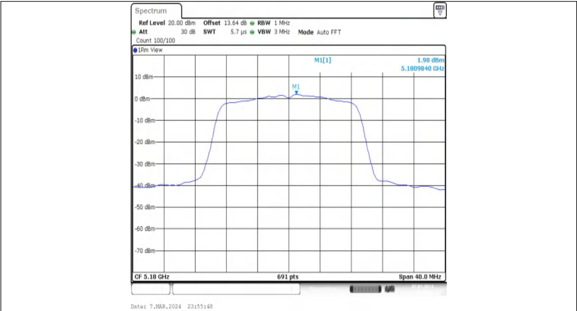
11N20MIMO-Ant1-5180-PASS
