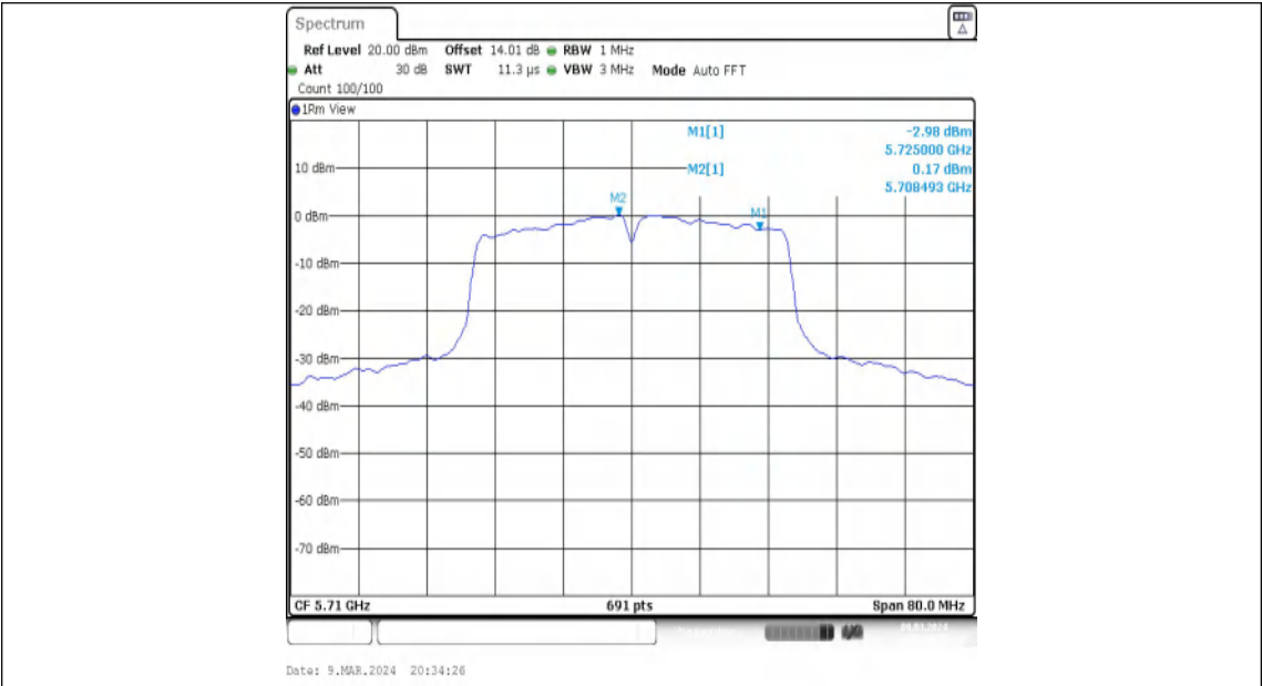
11N40MIMO-Ant2-5710_UNII-2C-PASS
