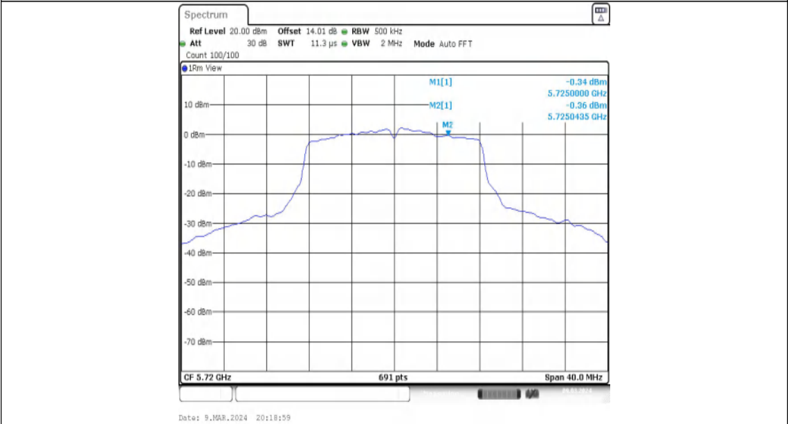
11A-Ant2-5720_UNII-3-PASS
