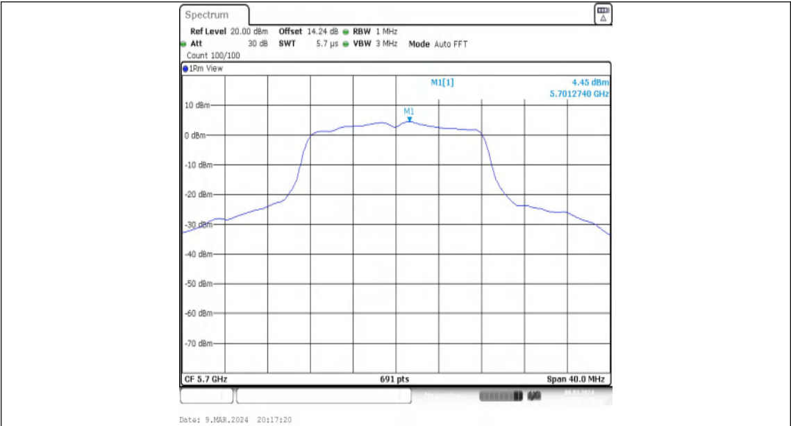
11A-Ant2-5700-PASS
