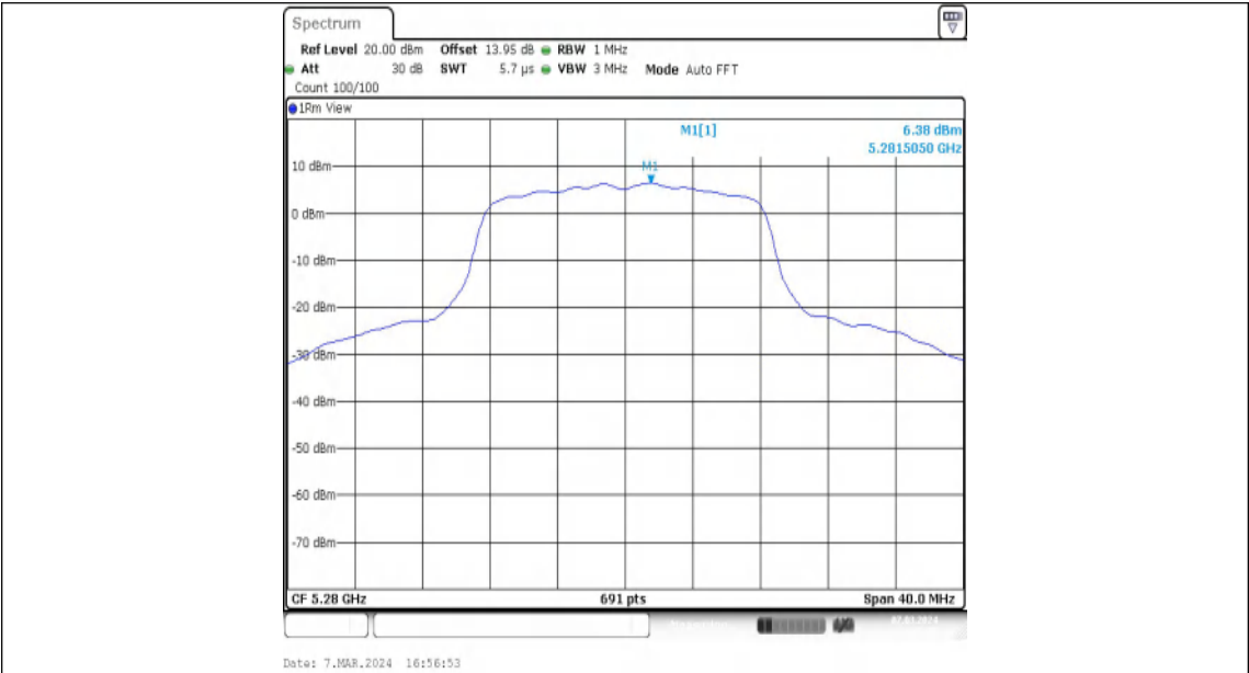
11A-Ant1-5280-PASS
