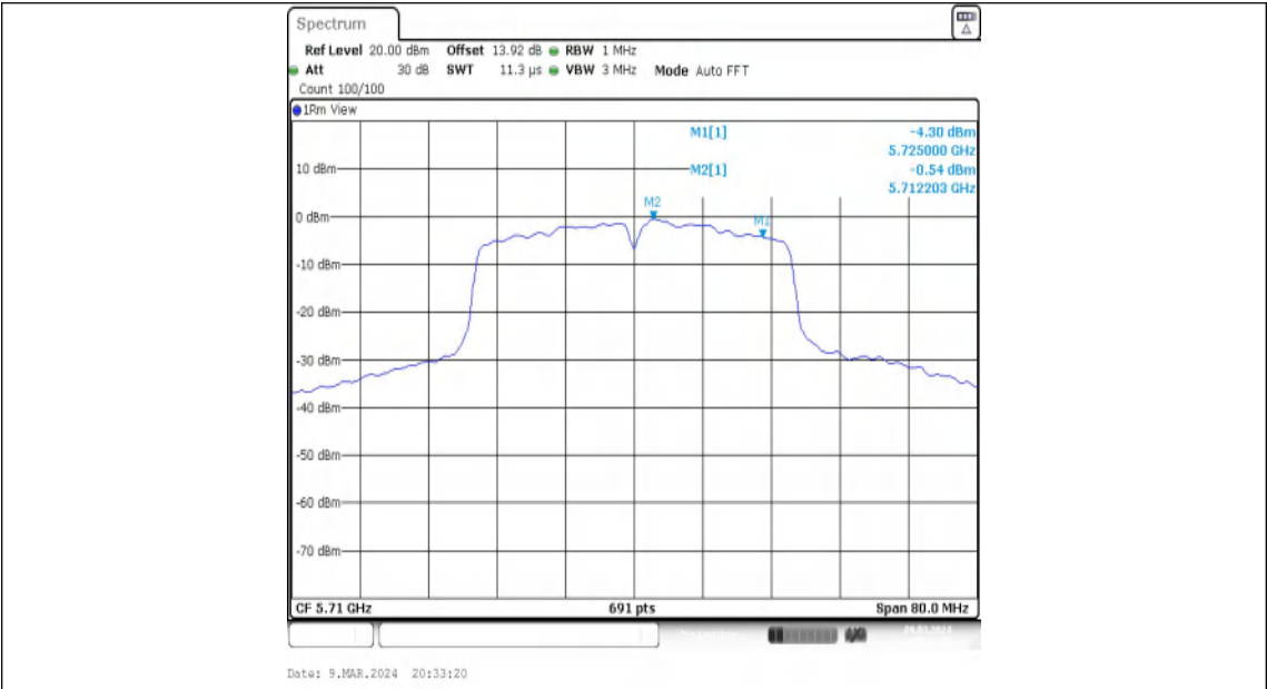
11N40MIMO-Ant1-5710_UNII-2C-PASS
