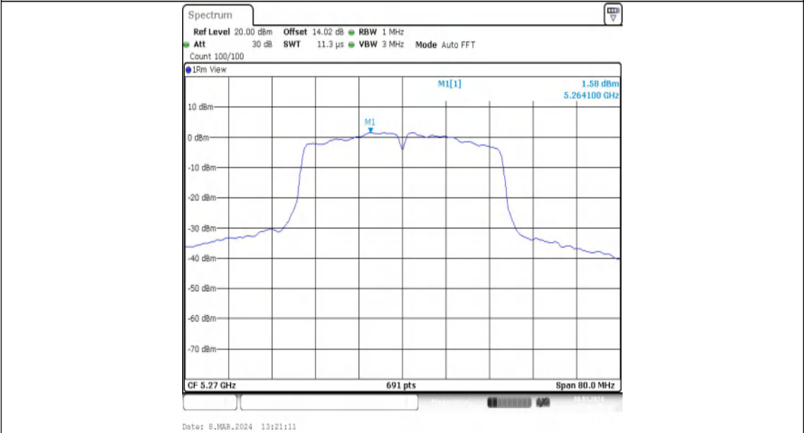
11N40MIMO-Ant2-5270-PASS
