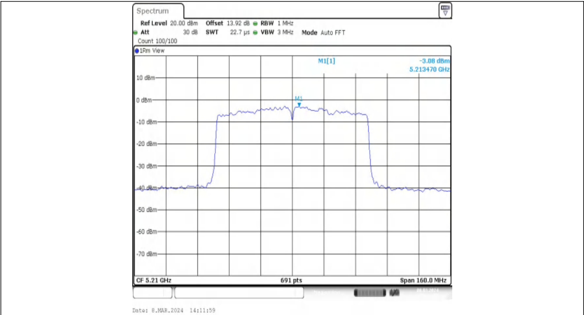
11AC80MIMO-Ant1-5210-PASS
