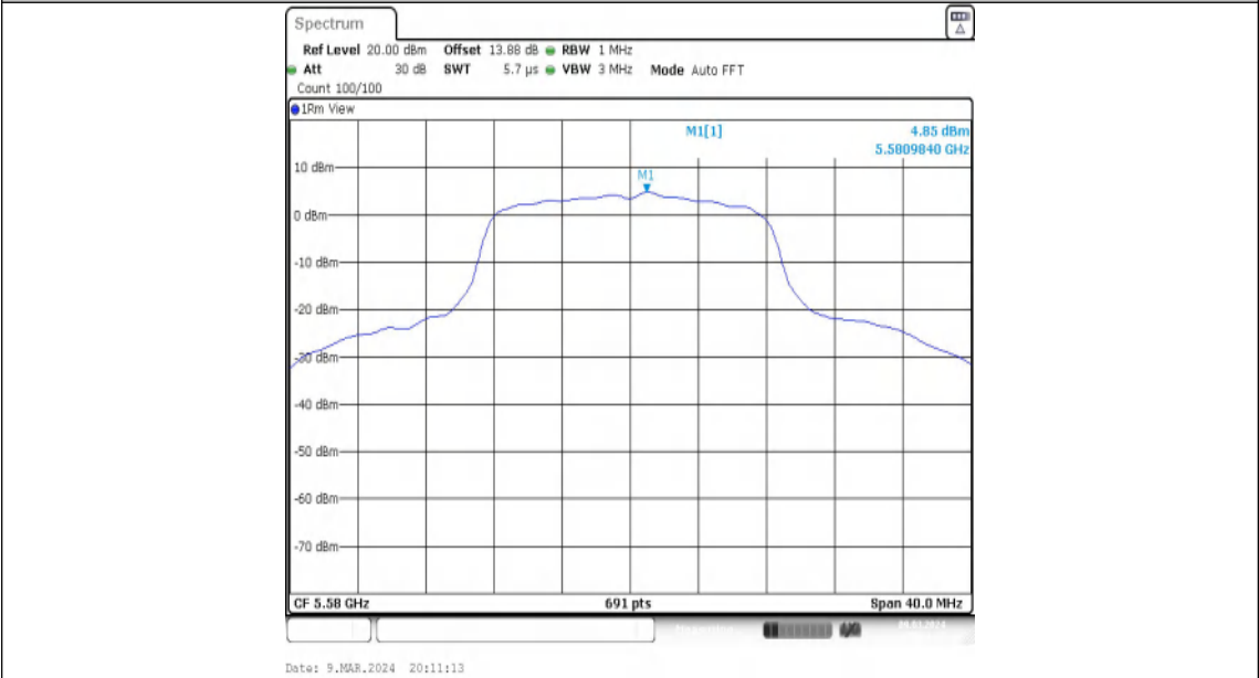
11A-Ant1-5580-PASS
