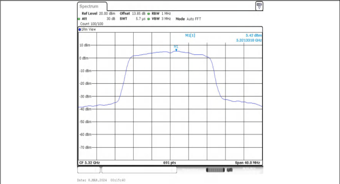
11N20MIMO-Ant2-5320-PASS
