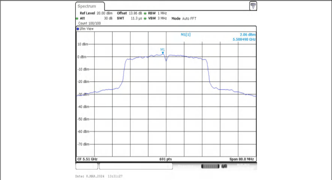
11N40MIMO-Ant2-5510-PASS
