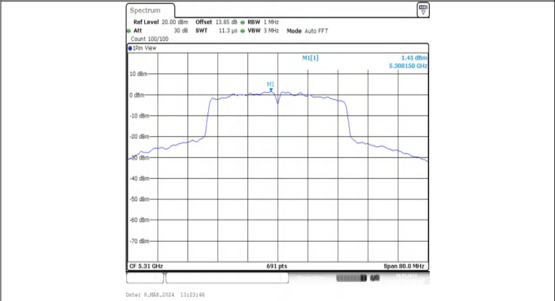
11N40MIMO-Ant2-5310-PASS
