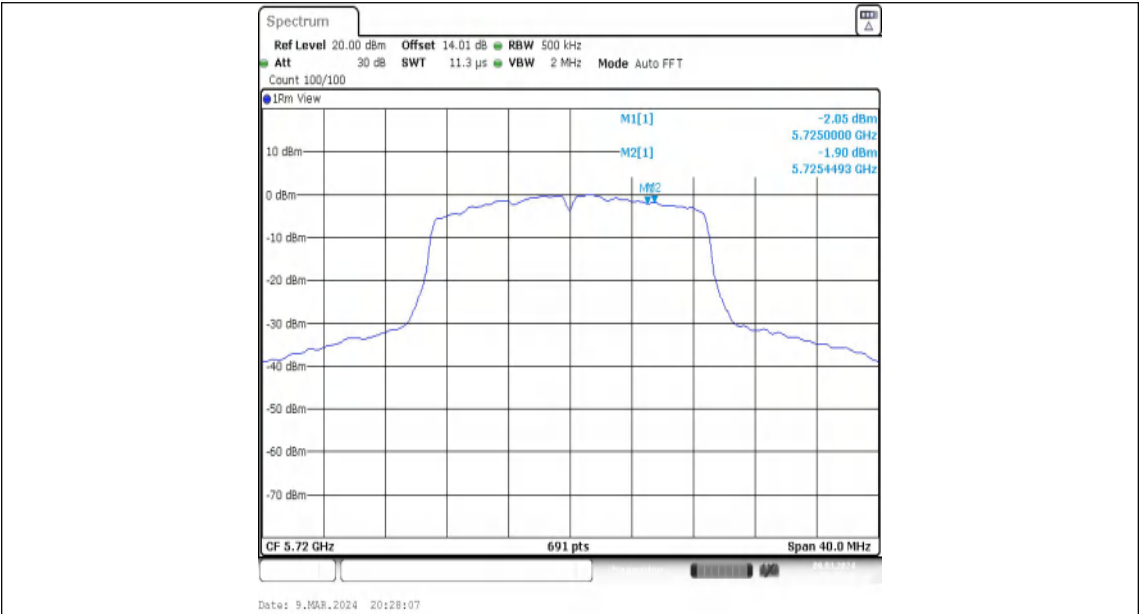
11N20MIMO-Ant2-5720_UNII-3-PASS
