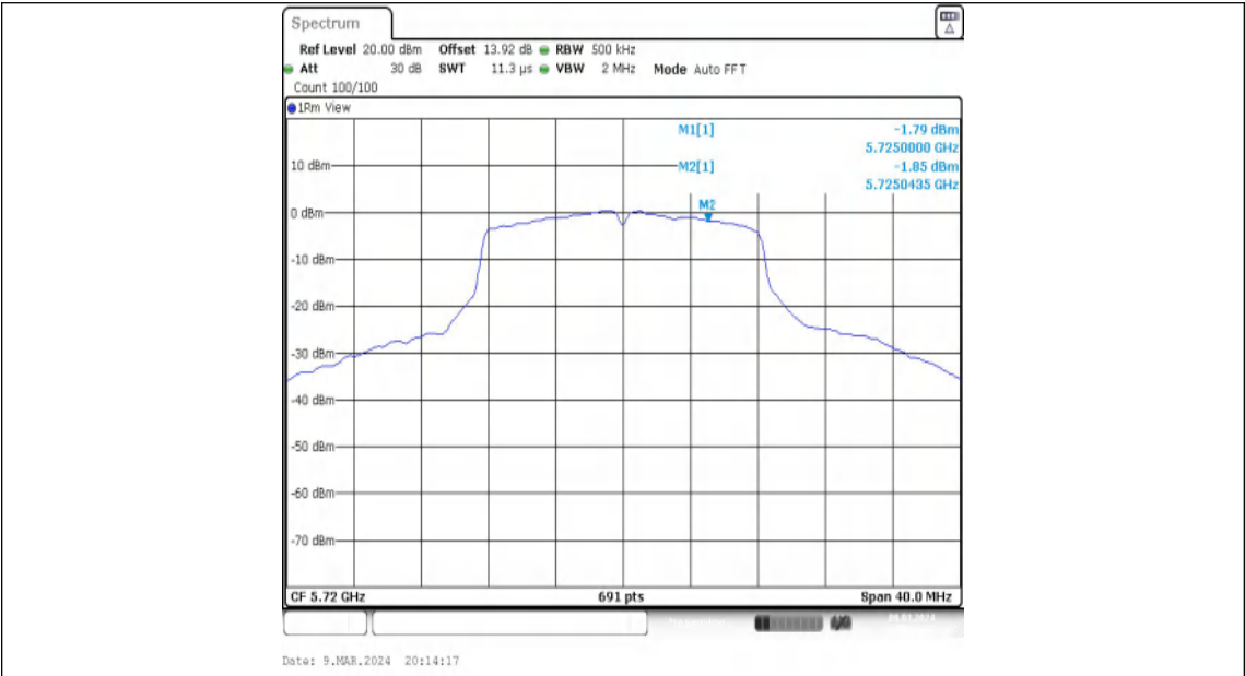
11A-Ant1-5720_UNII-3-PASS
