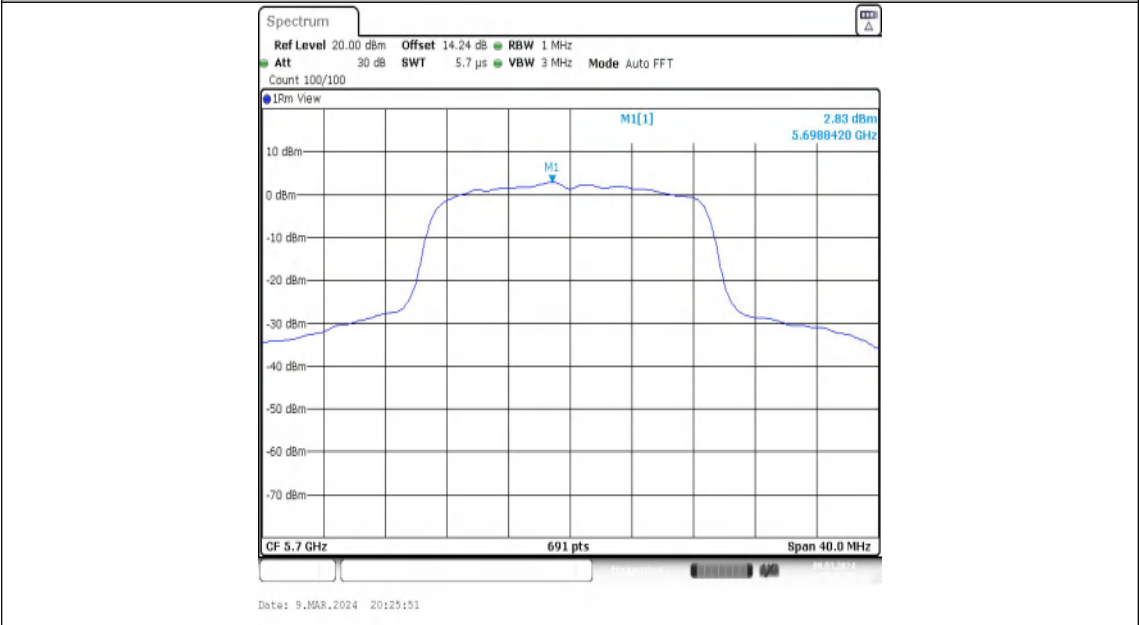
11N20MIMO-Ant2-5700-PASS
