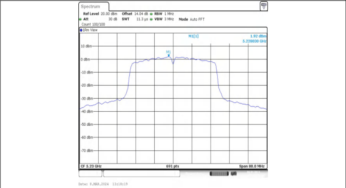
11N40MIMO-Ant2-5230-PASS
