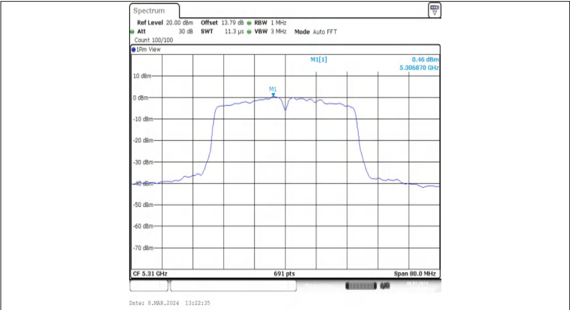
11N40MIMO-Ant1-5310-PASS
