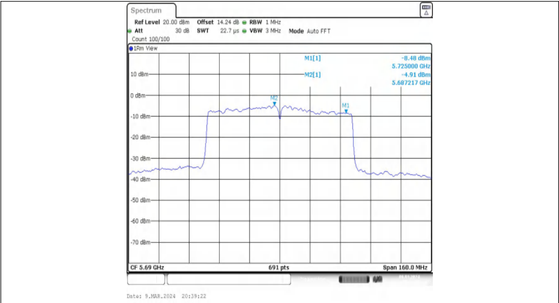
11AC80MIMO-Ant2-5690_UNII-2C-PASS
