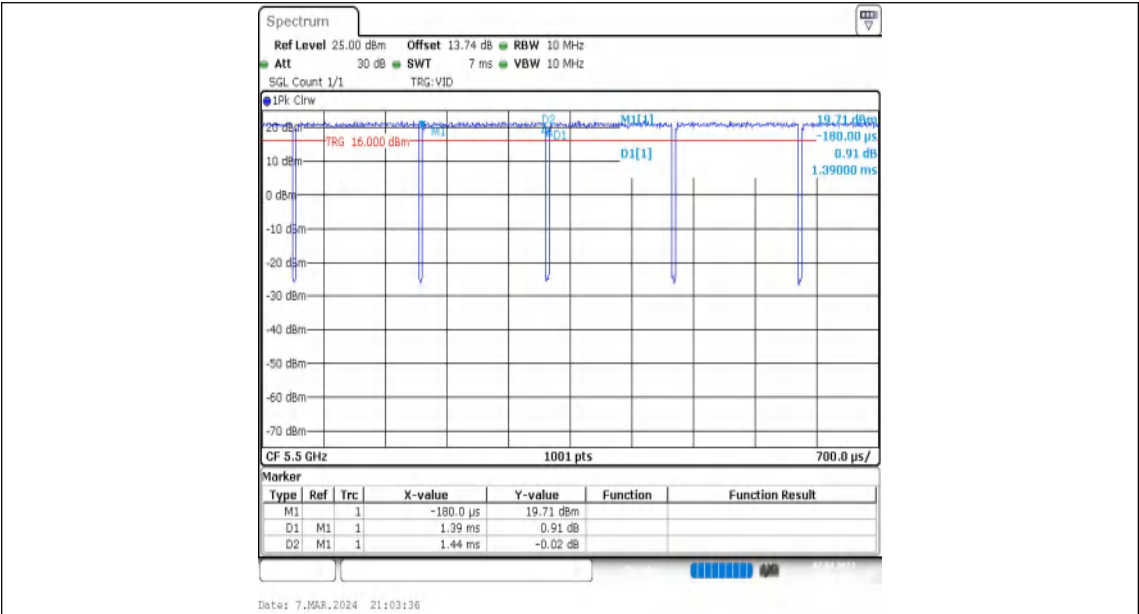
NTNV-11A-Ant1-5500
