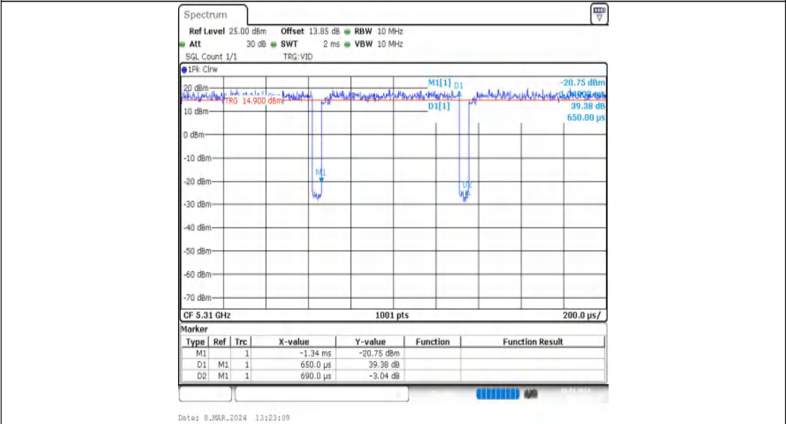
NTVN-11N40MIMO-Ant2-5310
