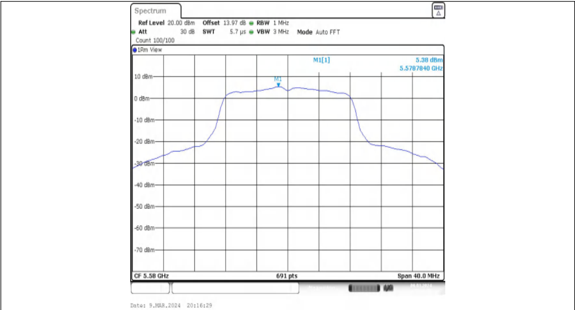
11A-Ant2-5580-PASS
