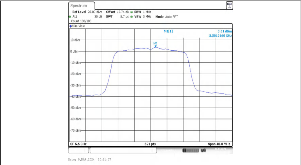
11N20MIMO-Ant1-5500-PASS
