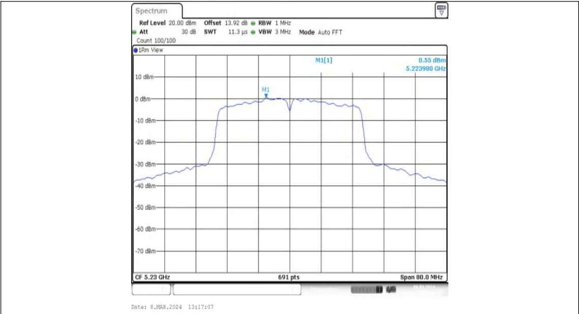
11N40MIMO-Ant1-5230-PASS
