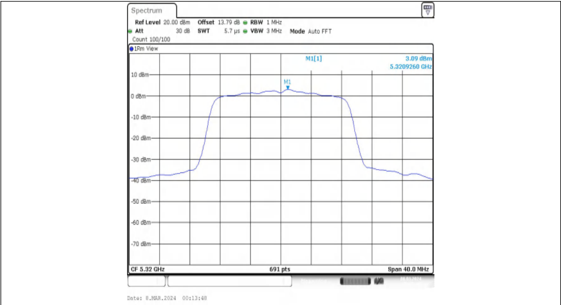
11N20MIMO-Ant1-5320-PASS
