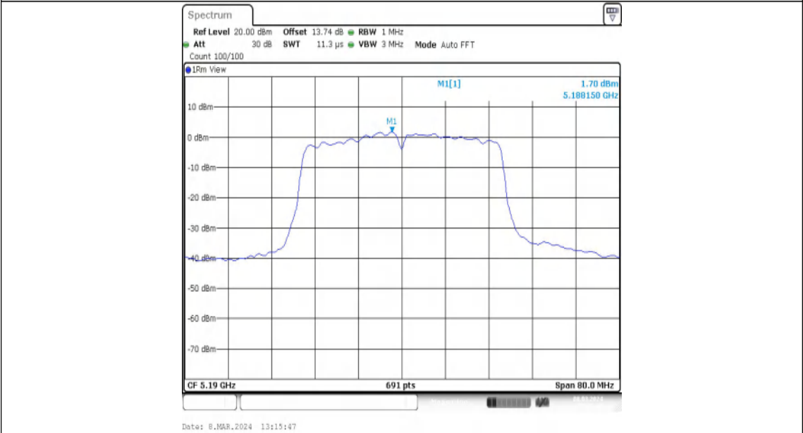
11N40MIMO-Ant2-5190-PASS
