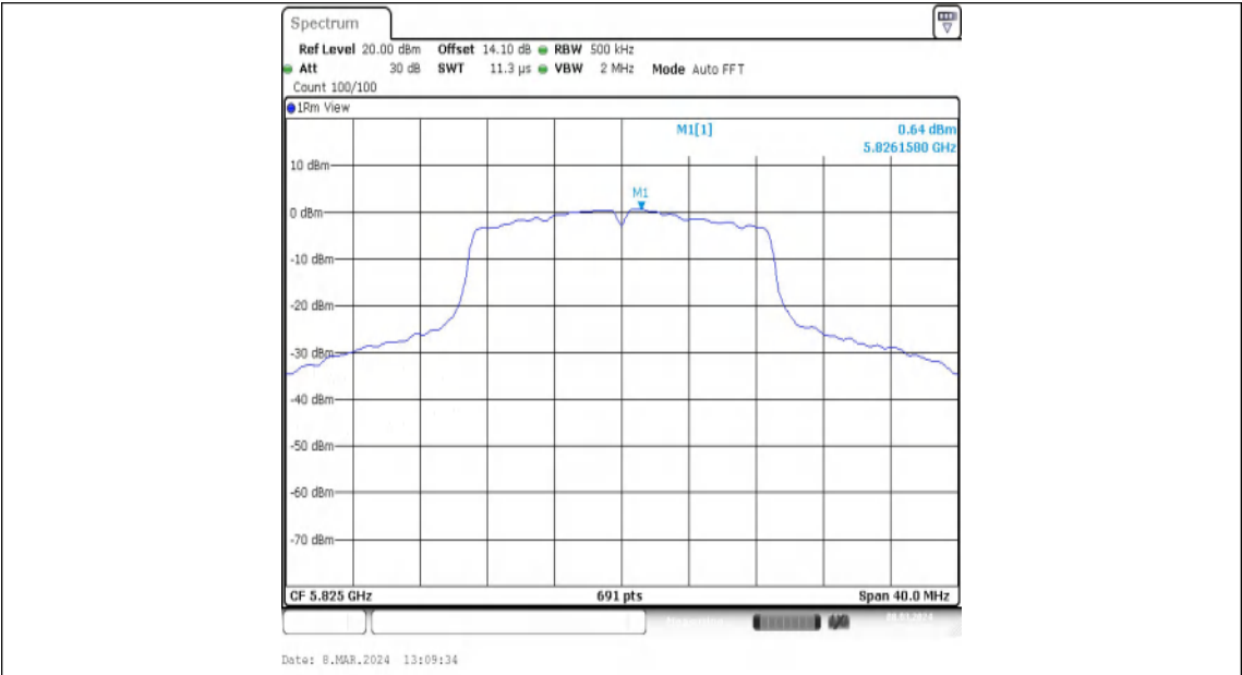
11N20MIMO-Ant2-5825-PASS
