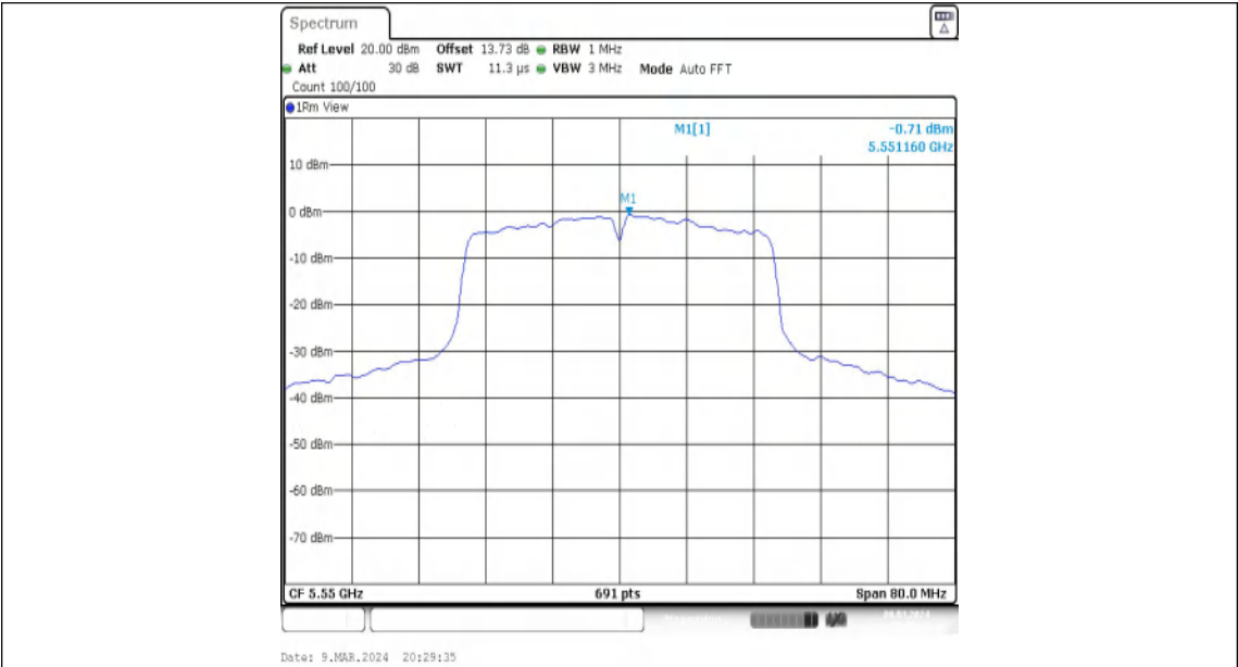
11N40MIMO-Ant1-5550-PASS
