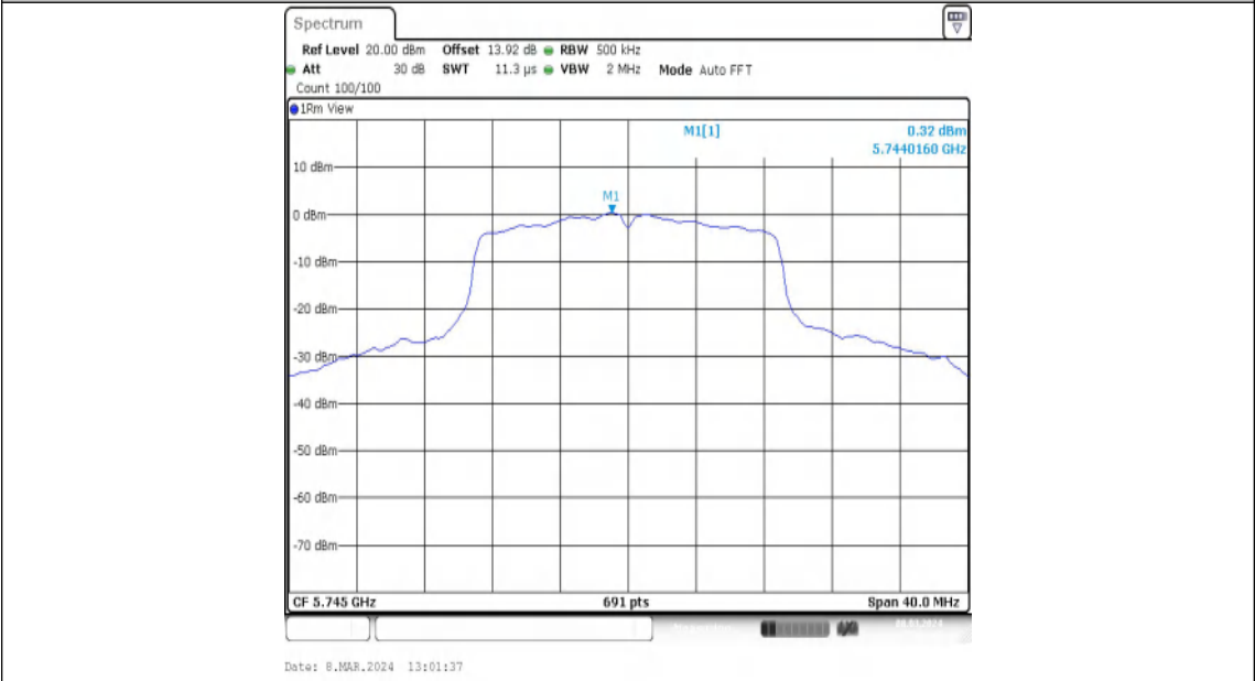
11N20MIMO-Ant1-5745-PASS
