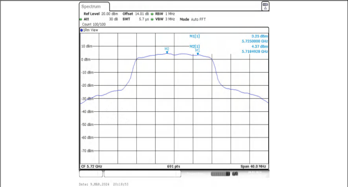
11A-Ant2-5720_UNII-2C-PASS
