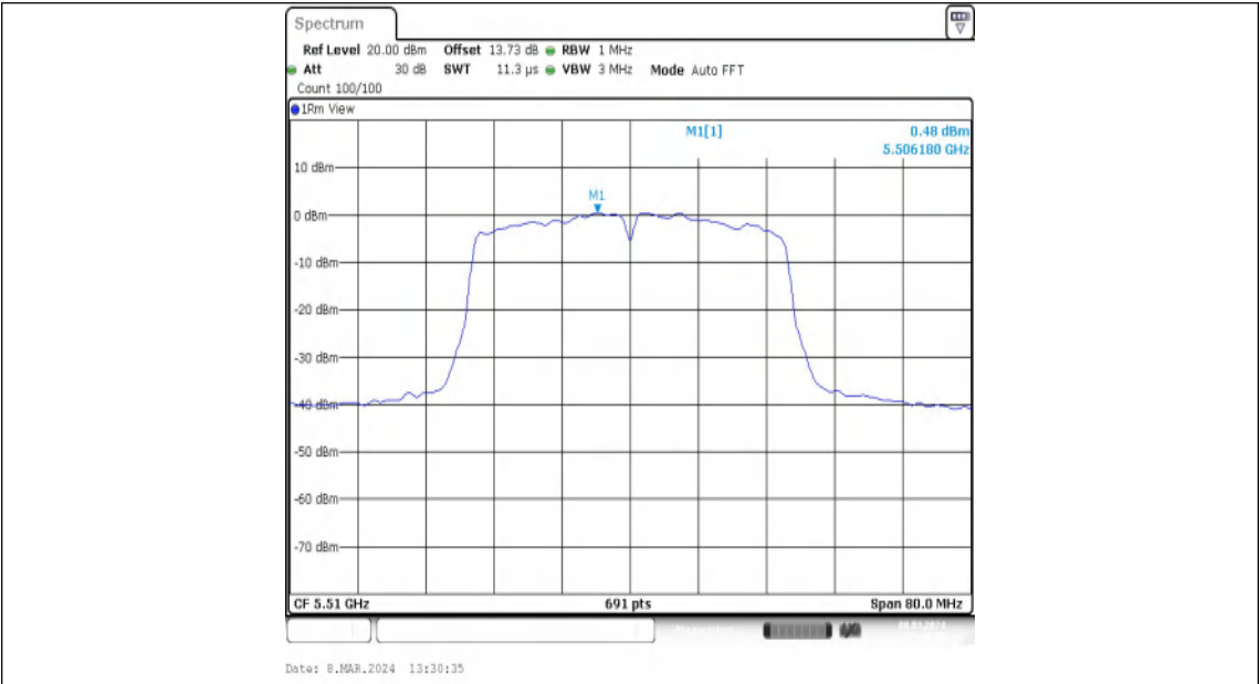
11N40MIMO-Ant1-5510-PASS
