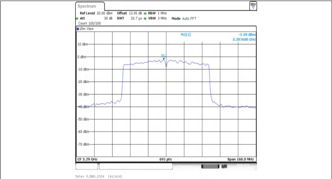
11AC80MIMO-Ant1-5290-PASS
