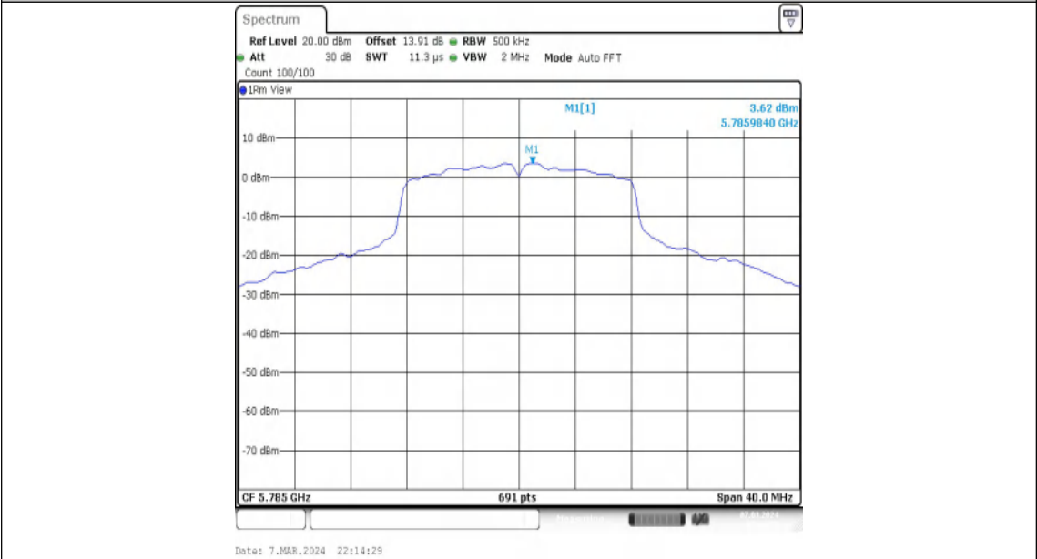
11A-Ant1-5785-PASS
