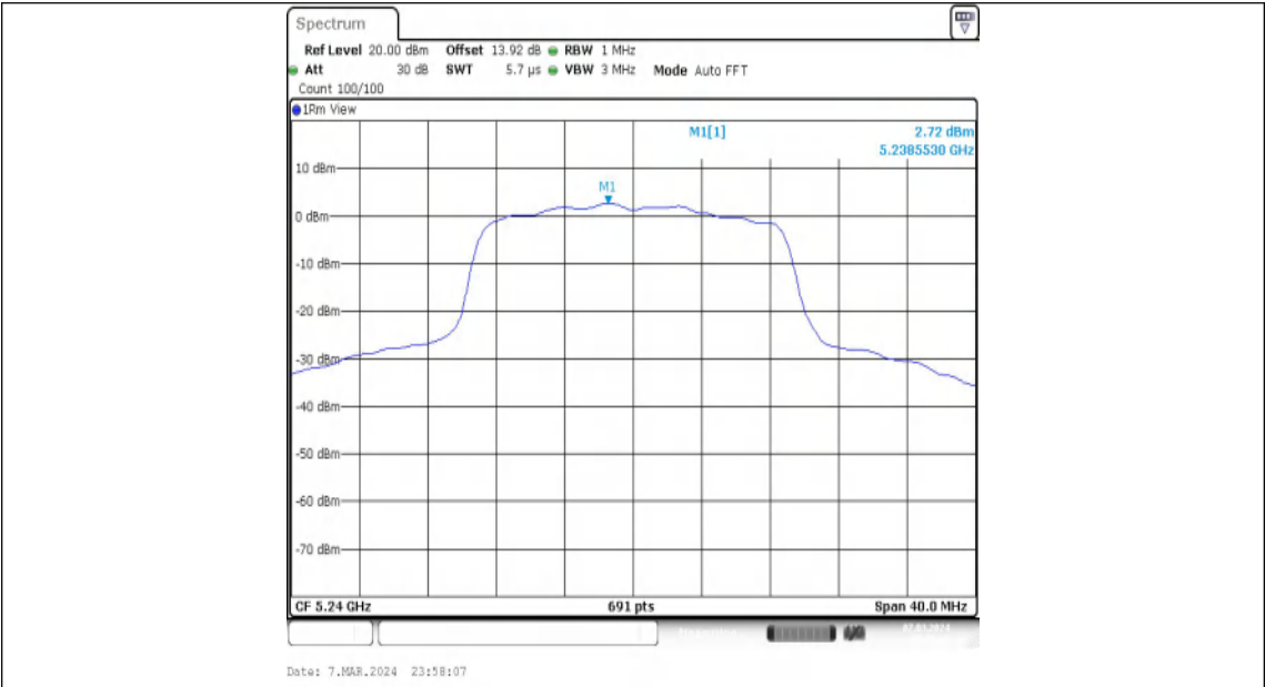
11N20MIMO-Ant1-5240-PASS
