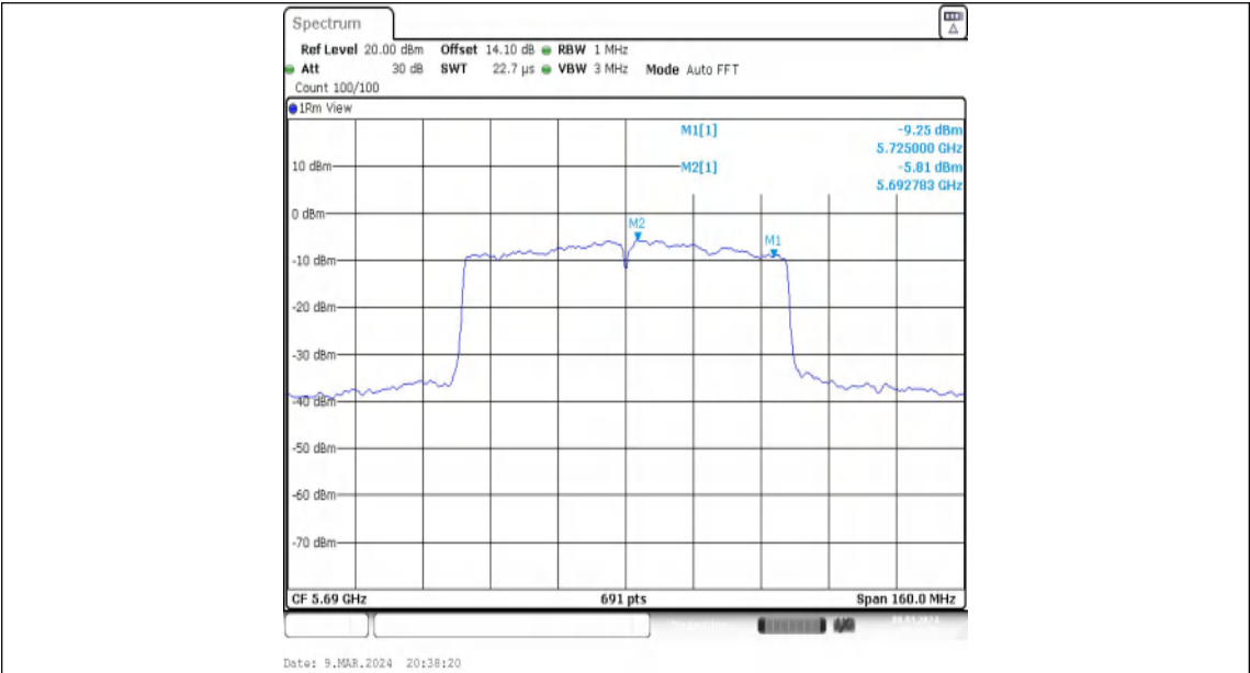
11AC80MIMO-Ant1-5690_UNII-2C-PASS
