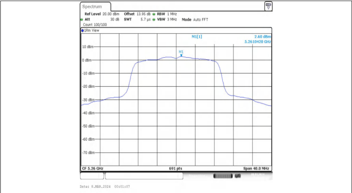
11N20MIMO-Ant1-5260-PASS
