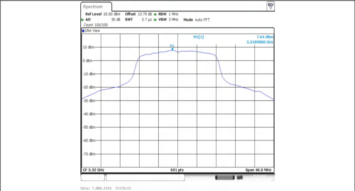
11A-Ant1-5320-PASS
