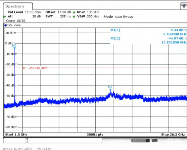
BLE_2M_Ant1_2440_1000~26500
