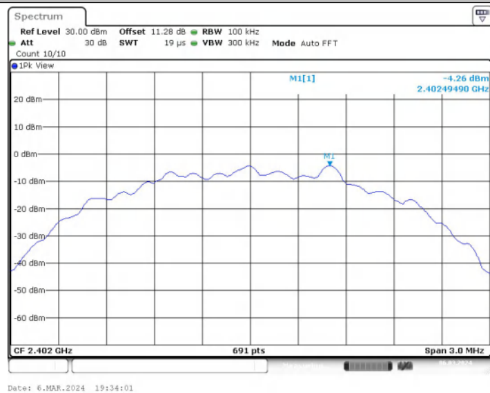
BLE_2M_Ant1_2402_0~Reference
