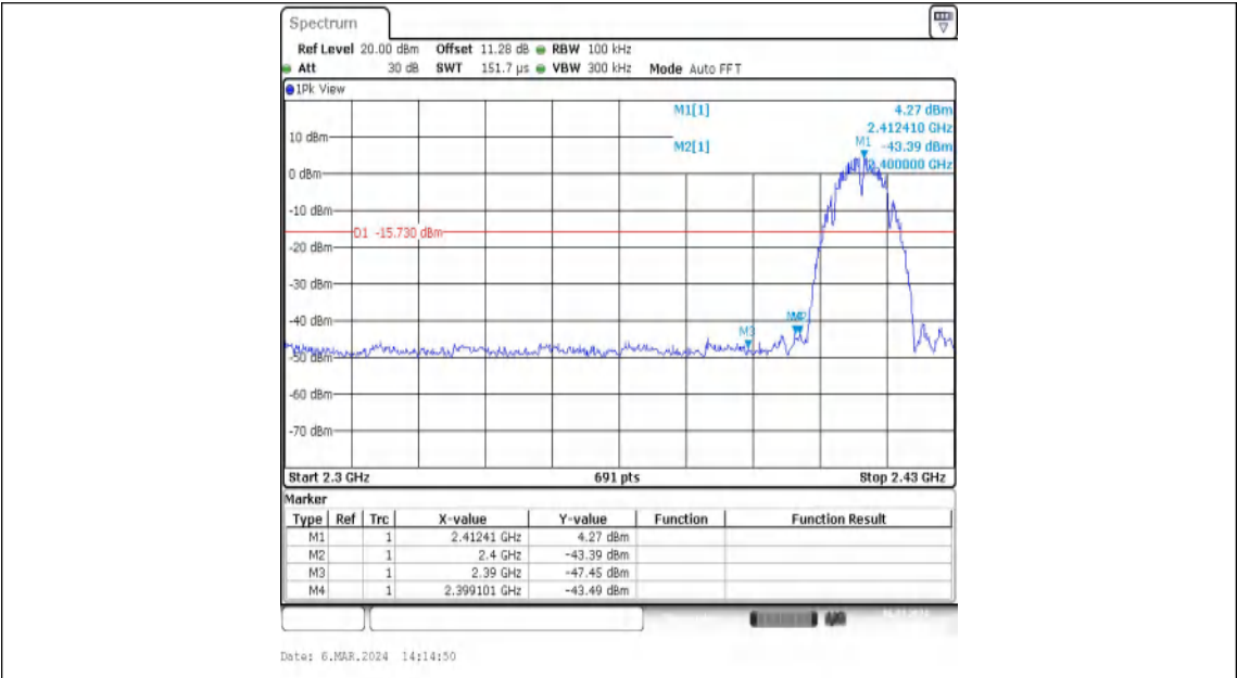
11B-Ant1-2412-PASS
