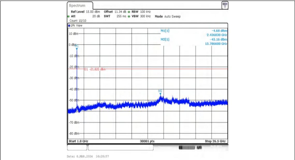
11G-Ant2-2437-1000~26500-PASS
