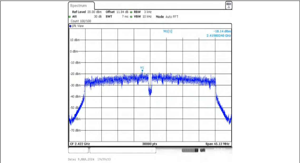
11N40MIMO-Ant2-2422-PASS
