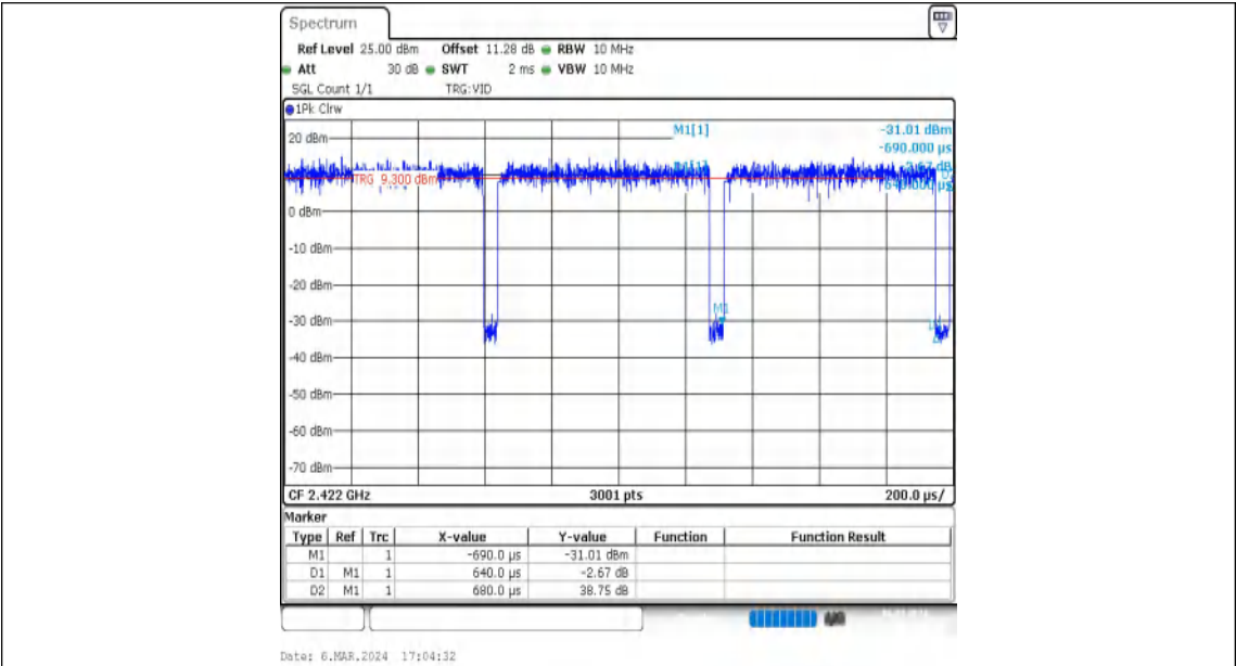
NTNV-11N40MIMO-Ant1-2422
