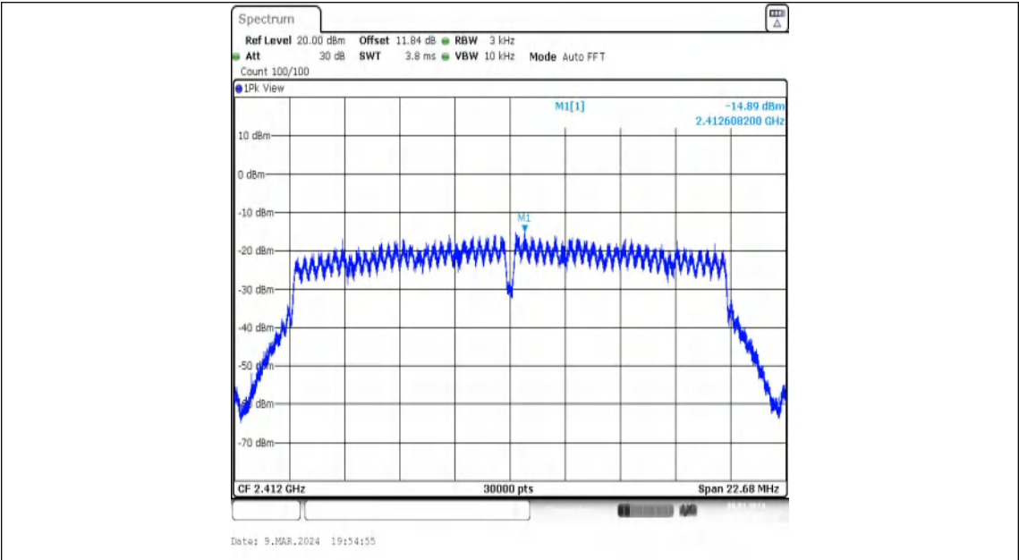
11N20MIMO-Ant2-2412-PASS
