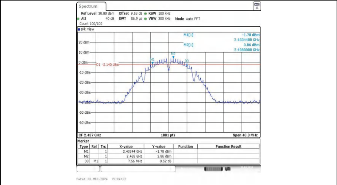
11B-Ant2-2437-PASS
