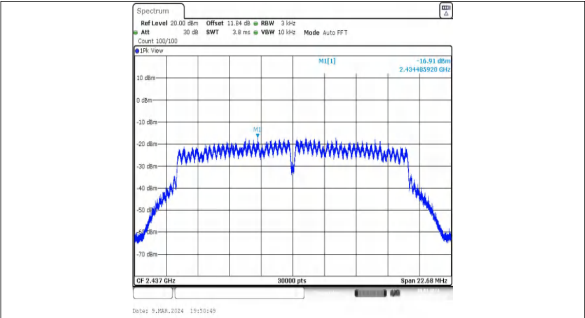
11G-Ant2-2437-PASS
