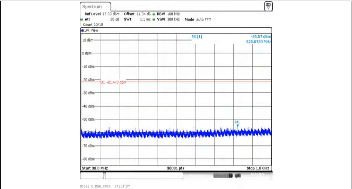
11N40MIMO-Ant2-2437-30~1000-PASS
