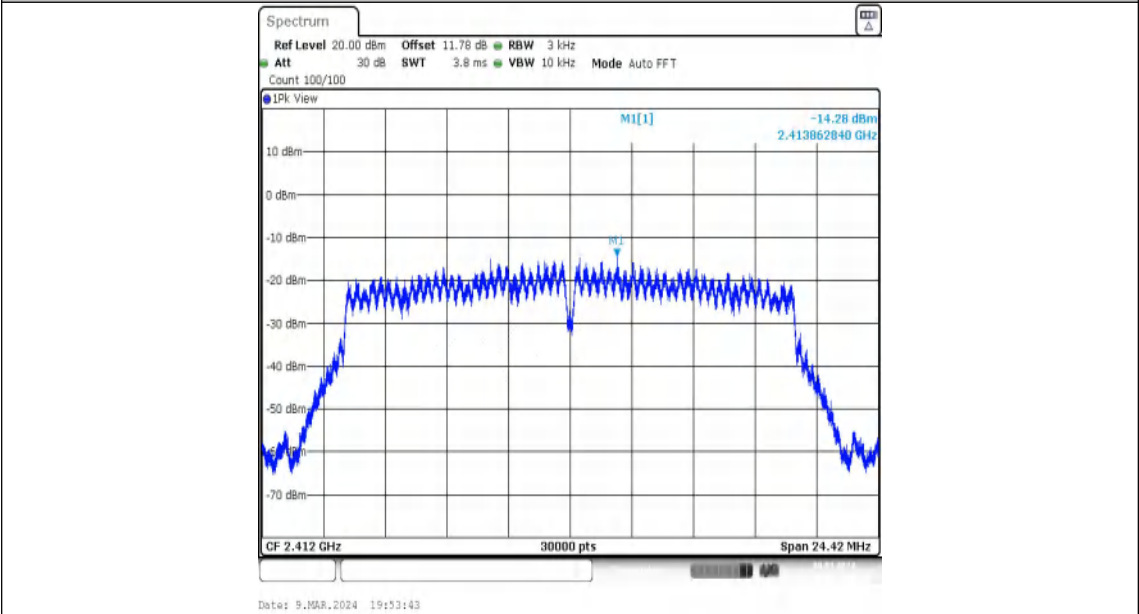
11N20MIMO-Ant1-2412-PASS
