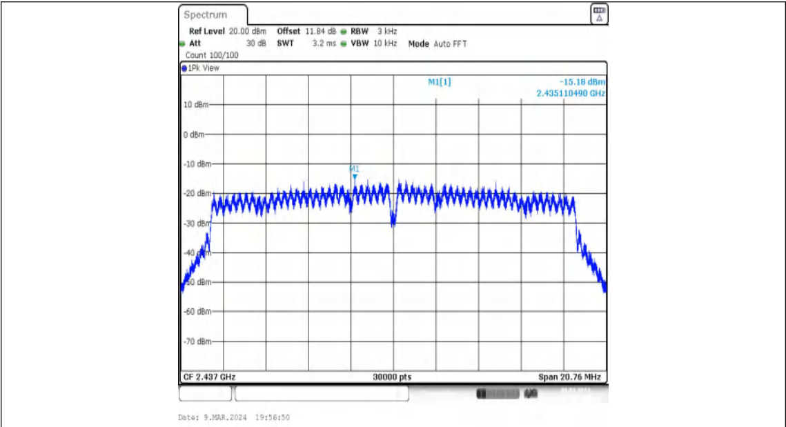
11N20MIMO-Ant2-2437-PASS
