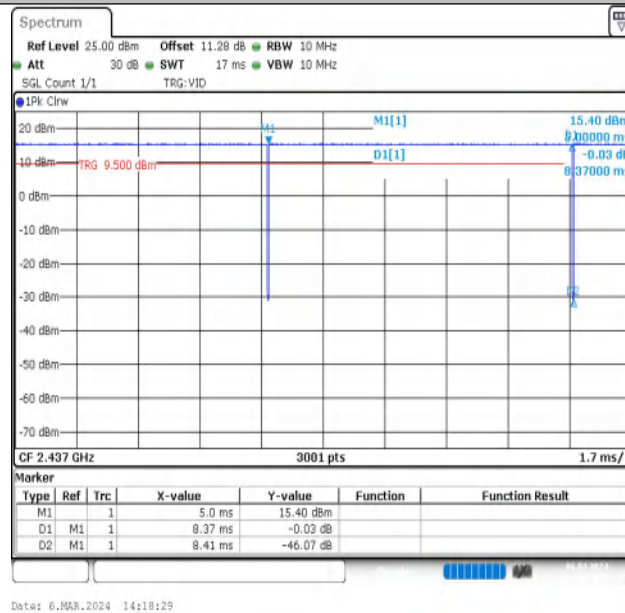
NTNV-11B-Ant1-2437
