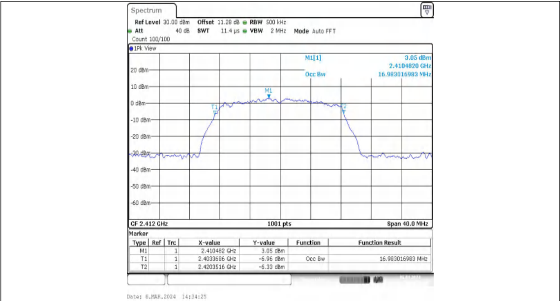
11G-Ant1-2412
