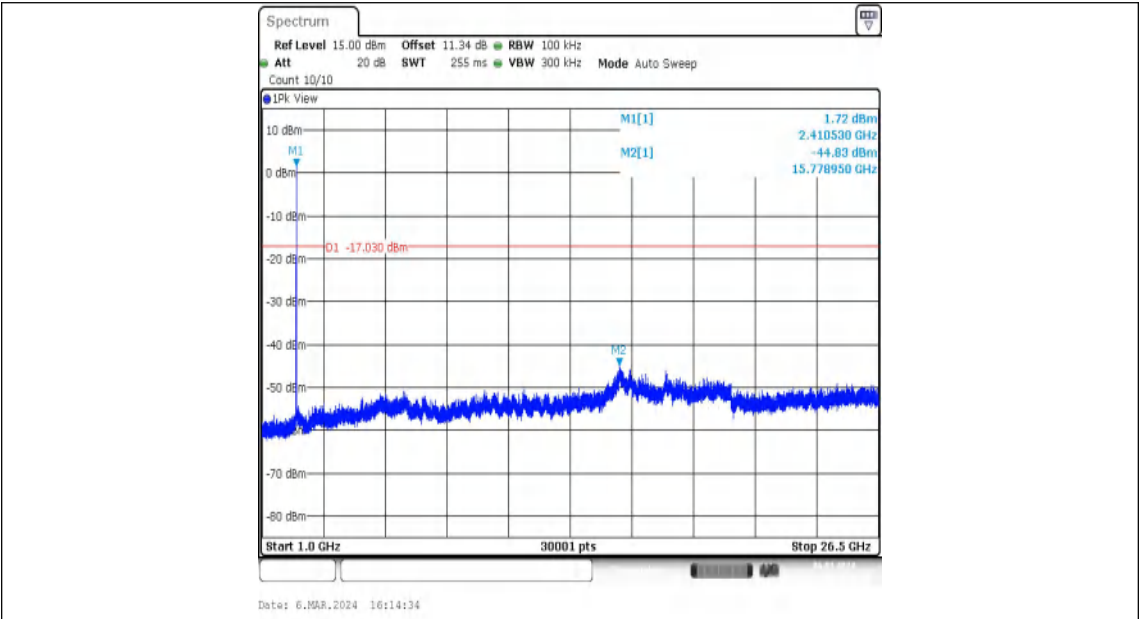
11B-Ant2-2412-1000~26500-PASS
