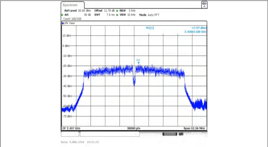
11N40MIMO-Ant1-2437-PASS
