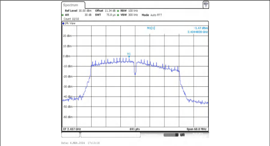
11N40MIMO-Ant2-2437-0~Reference-PASS
