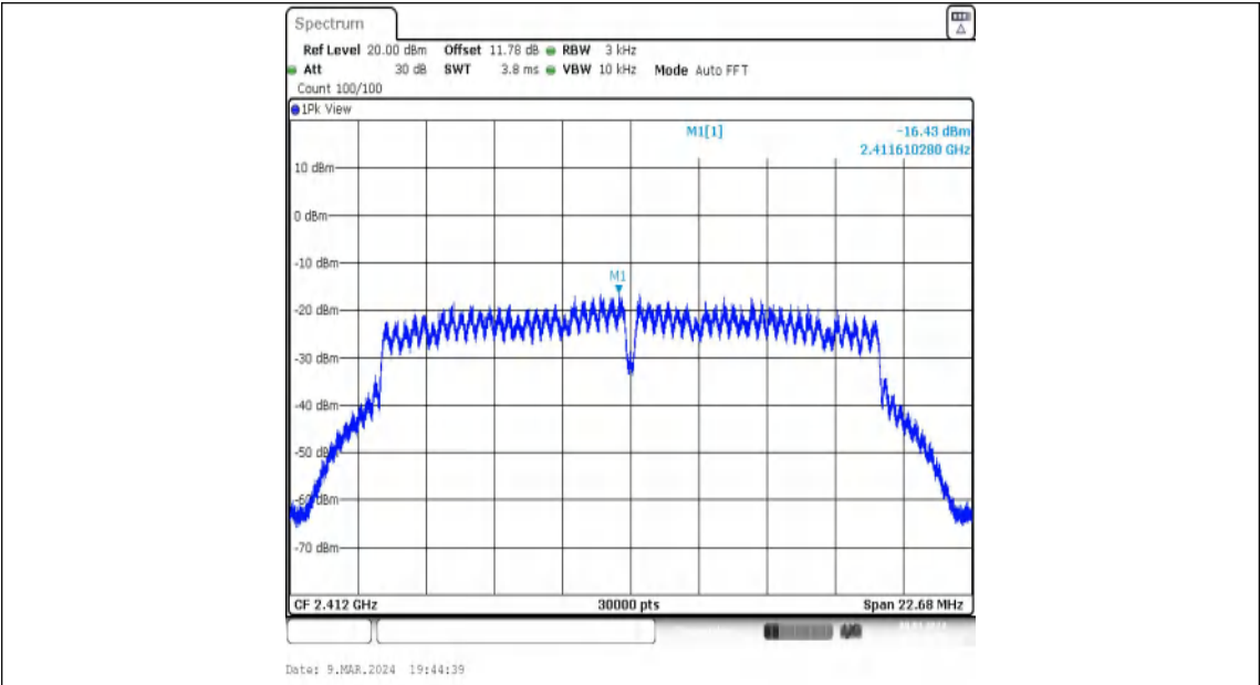
11G-Ant1-2412-PASS
