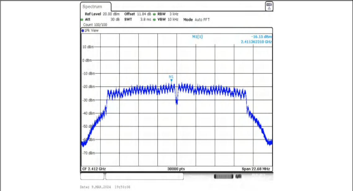
11G-Ant2-2412-PASS
