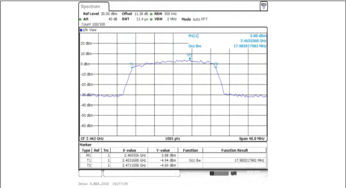
11N20MIMO-Ant2-2462
