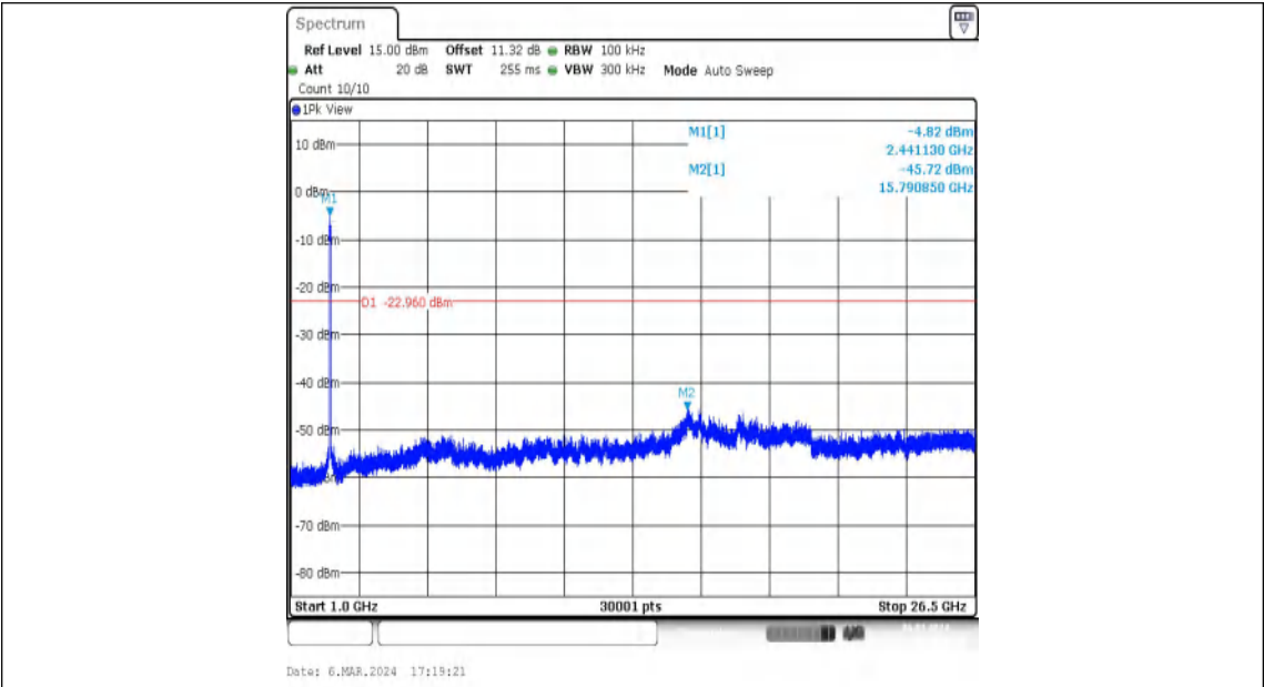
11N40MIMO-Ant1-2452-1000~26500-PASS
