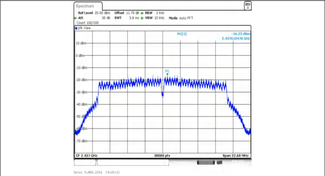
11G-Ant1-2437-PASS
