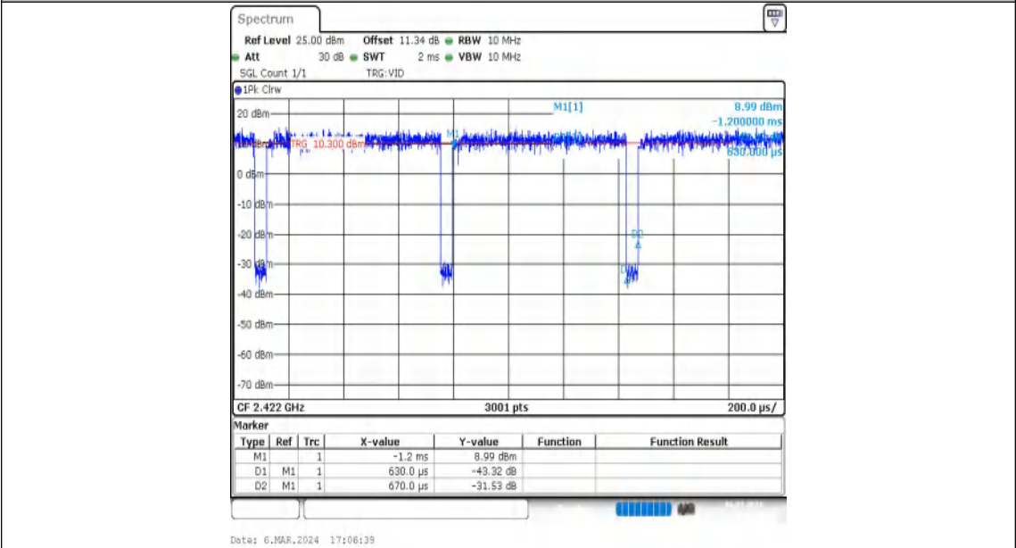
NTNV-11N40MIMO-Ant2-2422
