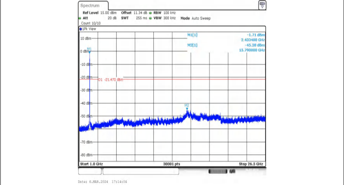
11N40MIMO-Ant2-2437-1000~26500-PASS
