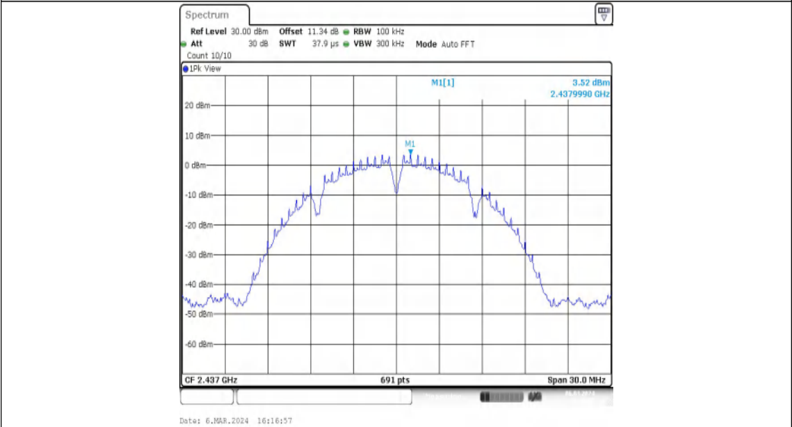
11B-Ant2-2437-0~Reference-PASS
