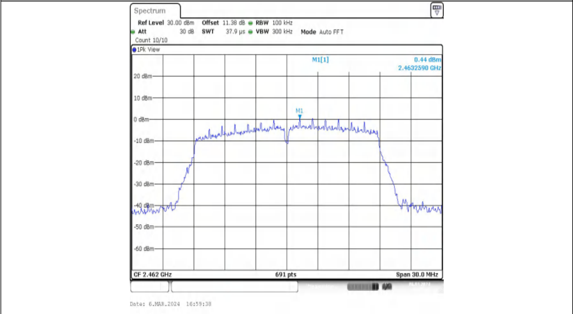
11N20MIMO-Ant2-2462-0~Reference-PASS
