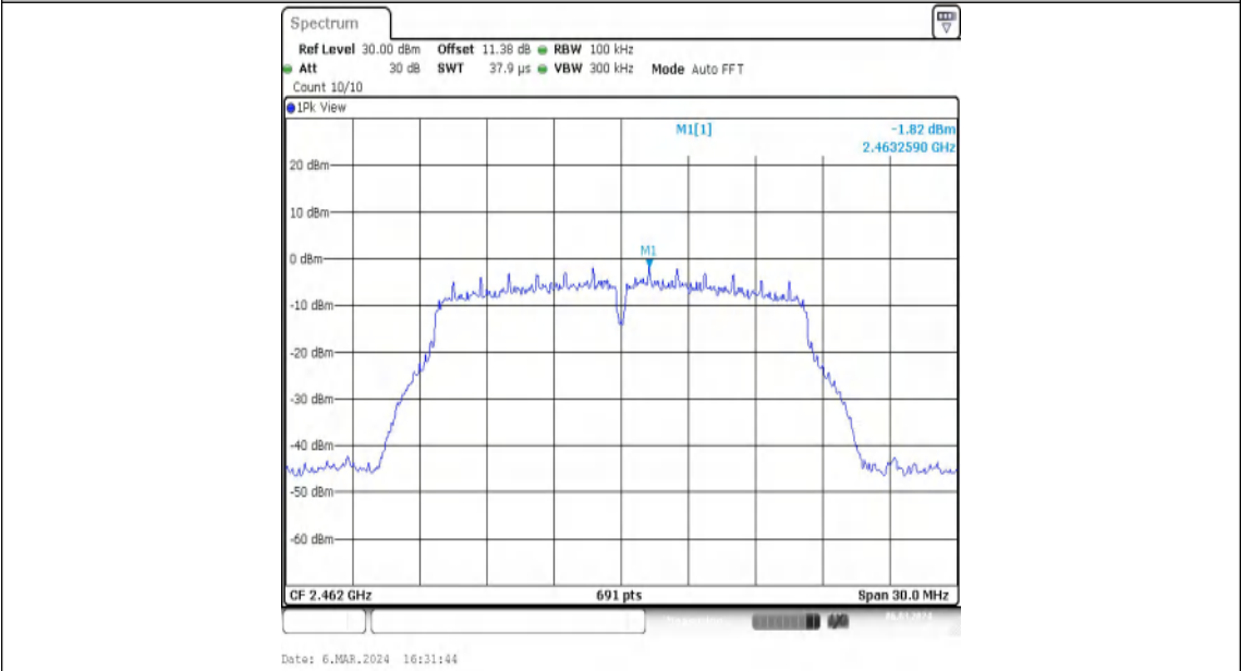
11G-Ant2-2462-0~Reference-PASS
