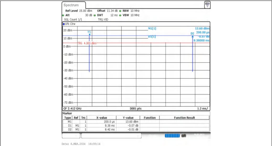
NTNV-11B-Ant2-2412
