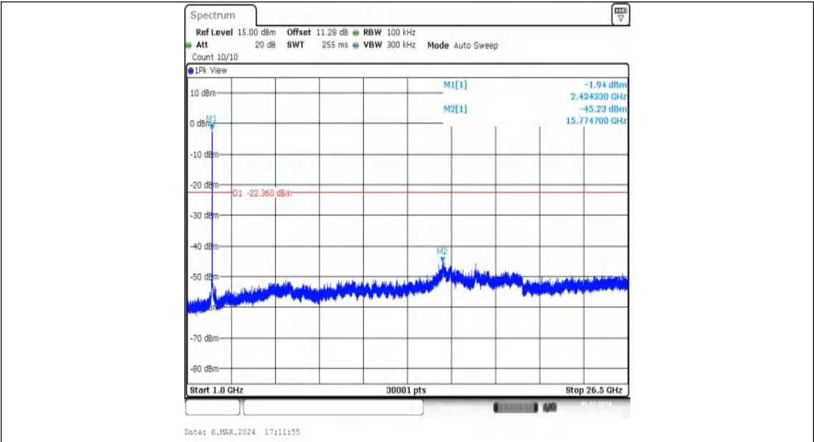
11N40MIMO-Ant1-2437-1000~26500-PASS
