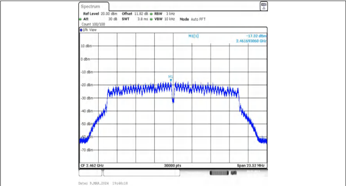
11G-Ant1-2462-PASS
