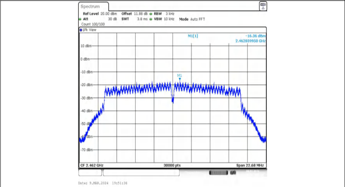
11G-Ant2-2462-PASS
