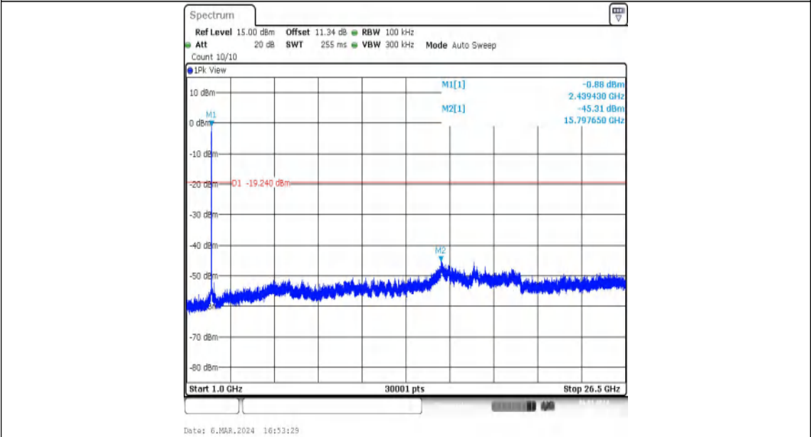
11N20MIMO-Ant2-2437-1000~26500-PASS
