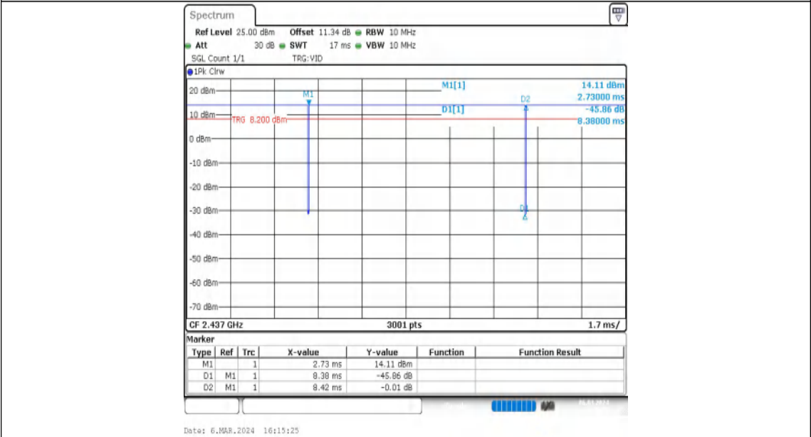
NTNV-11B-Ant2-2437
