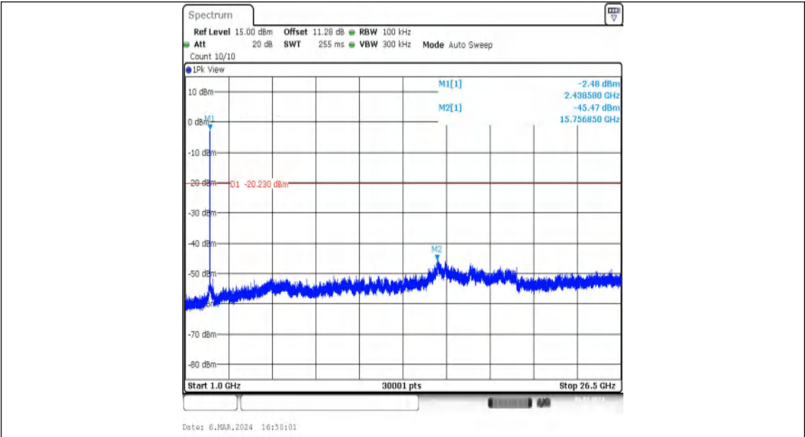
11N20MIMO-Ant1-2437-1000~26500-PASS
