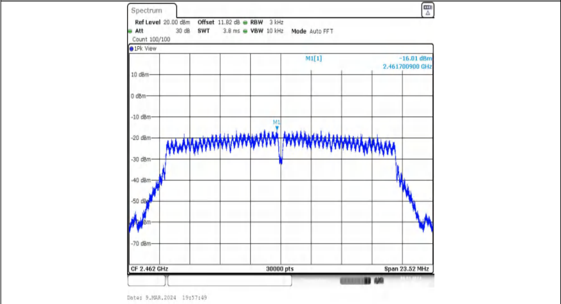
11N20MIMO-Ant1-2462-PASS
