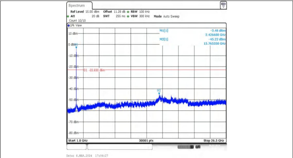
11N40MIMO-Ant1-2422-1000~26500-PASS
