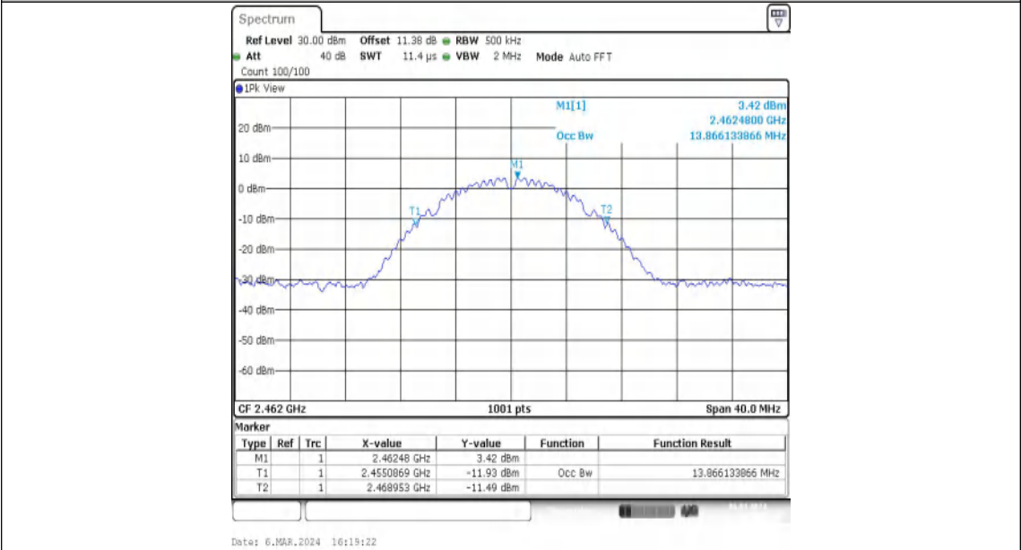
11B-Ant2-2462
