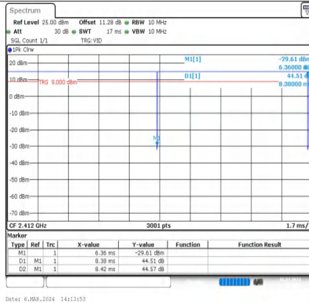
NTNV-11B-Ant1-2412
