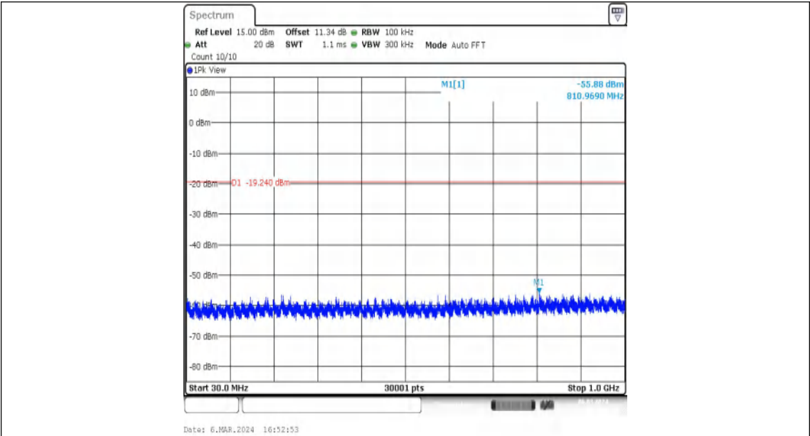
11N20MIMO-Ant2-2437-30~1000-PASS
