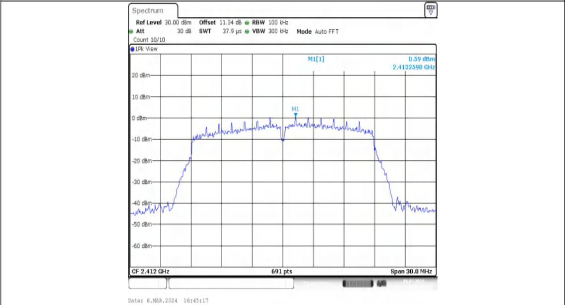
11N20MIMO-Ant2-2412-0~Reference-PASS
