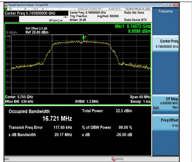
11a-CDD-Ant2-5745
