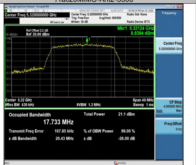
11ac20MIMO-Ant2-5320
