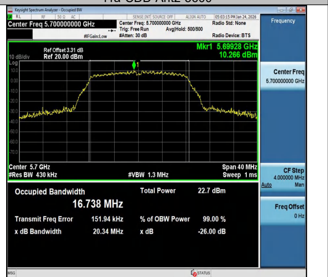
11a-CDD-Ant2-5700
