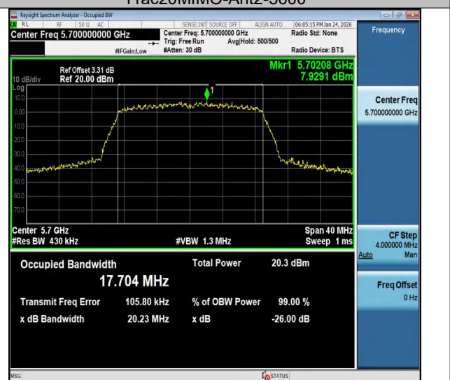
11ac20MIMO-Ant2-5700
