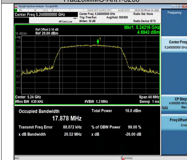
11ac20MIMO-Ant1-5240
