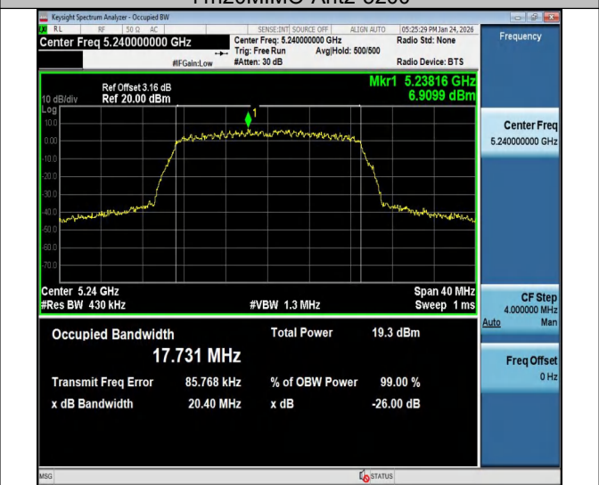
11n20MIMO-Ant2-5240
