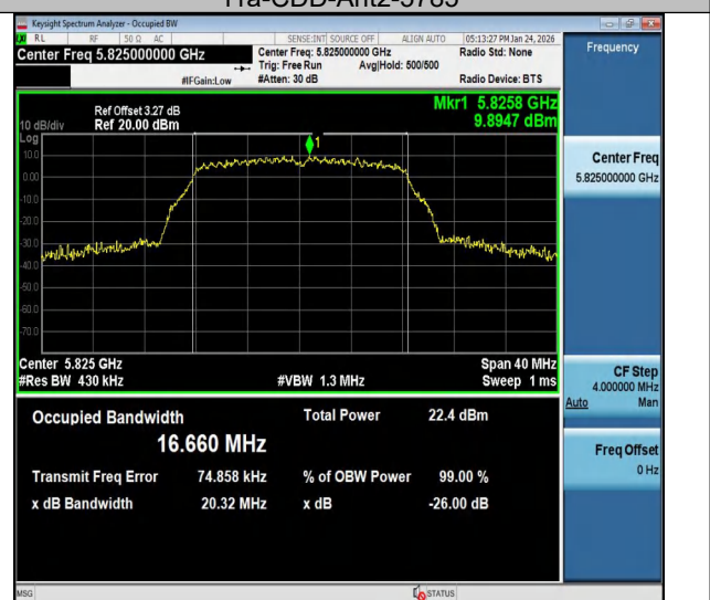
11a-CDD-Ant2-5825
