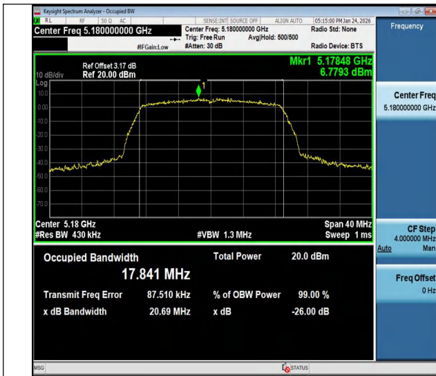
11n20MIMO-Ant1-5180
