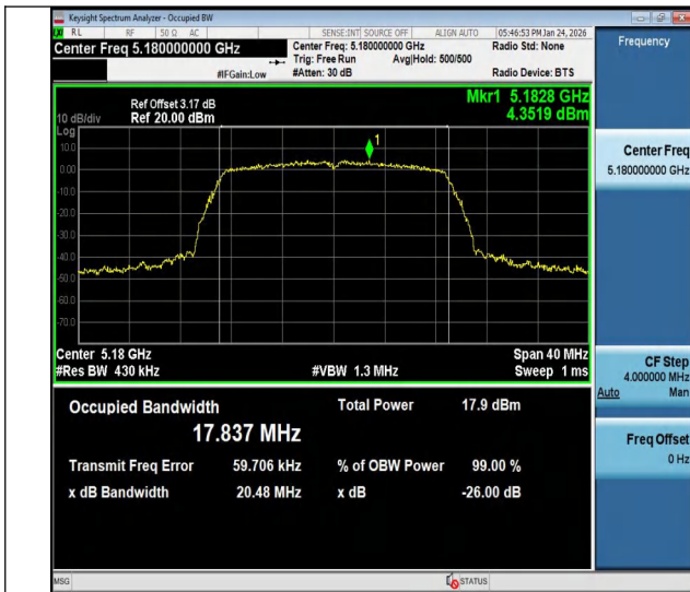
11ac20MIMO-Ant1-5180
