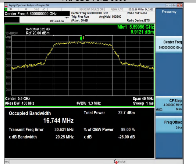
11a-CDD-Ant2-5600
