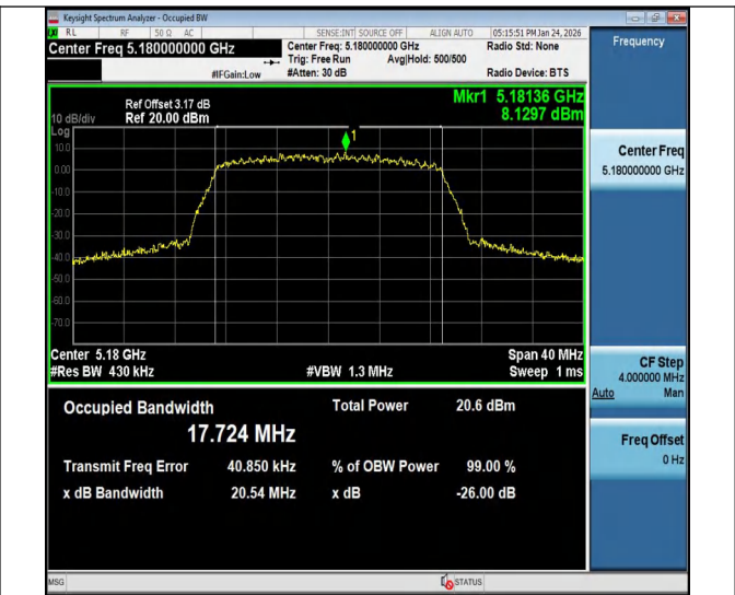
11n20MIMO-Ant2-5180
