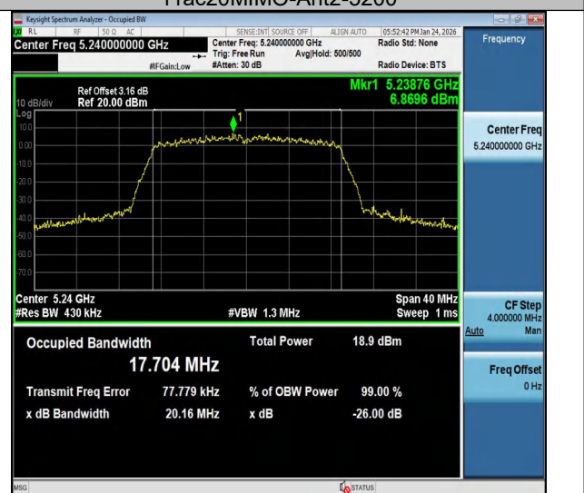
11ac20MIMO-Ant2-5240
