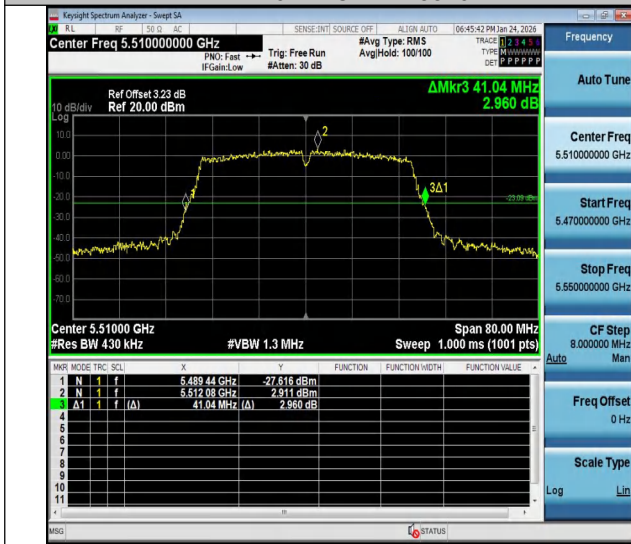
11ac40MIMO-Ant1-5510
