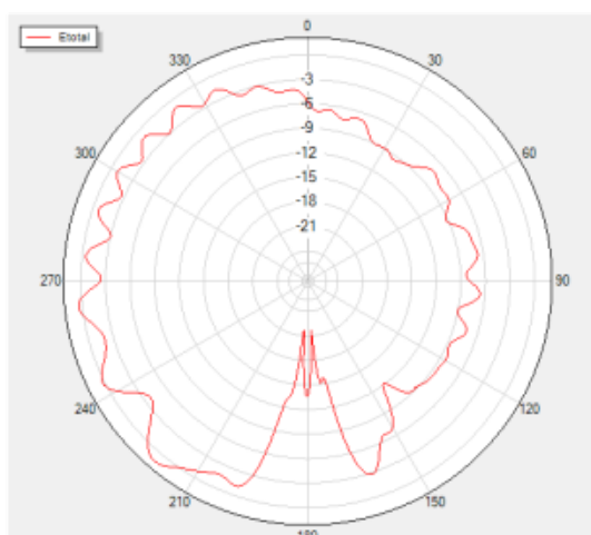
Phi=0 Freq=5850MHz
