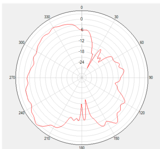
Phi=90 Freq=5650MHz
