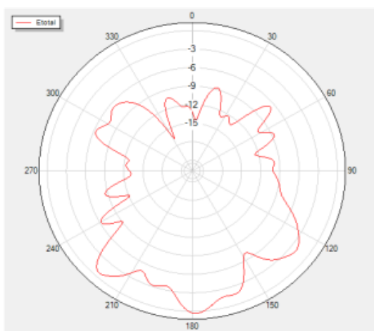
Theta=90 Freq=5350MHz
