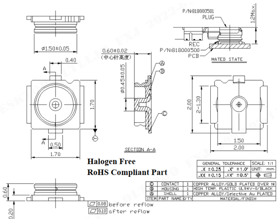
Figure 2: The dimensions of the connector
