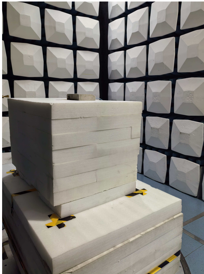
Radiated Emission 90-140GHz View
