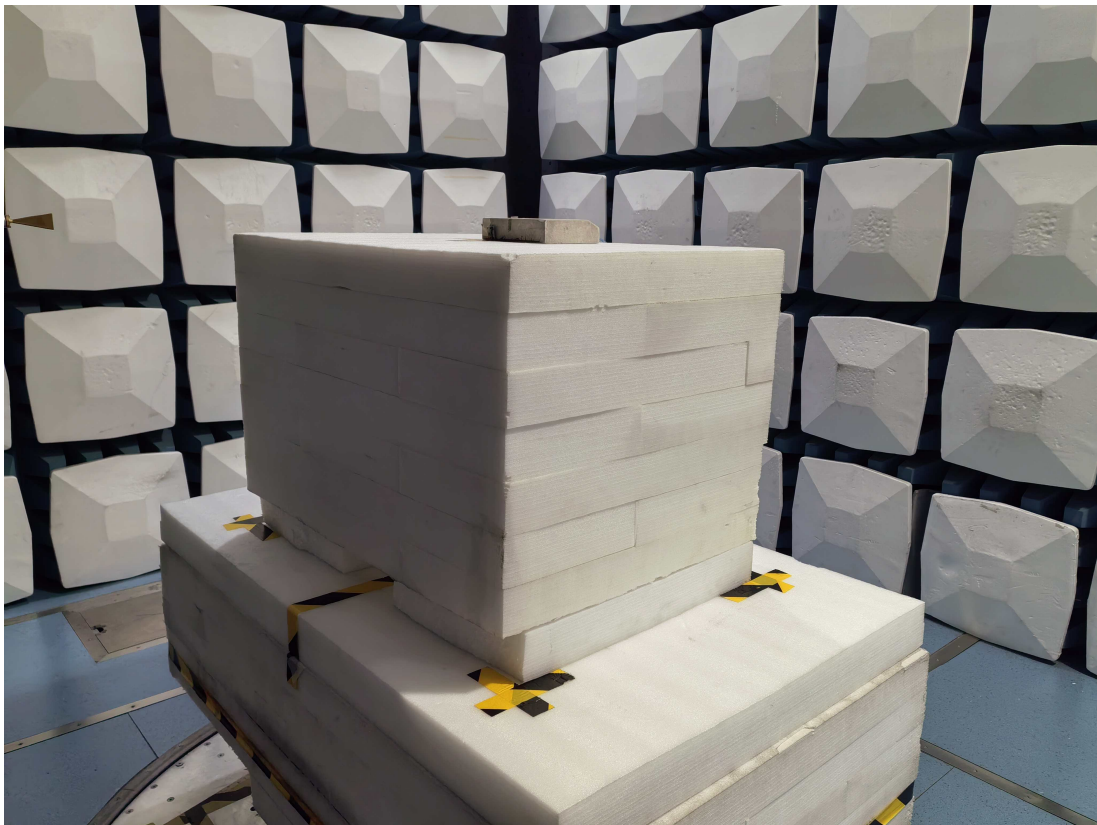
Radiated Emission 90-140GHz View
