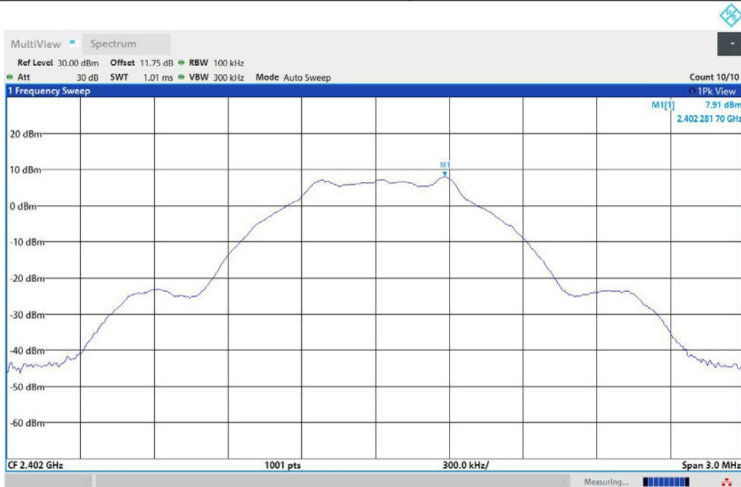
BLE_1M-Ant1-2402-0~Reference-PASS
