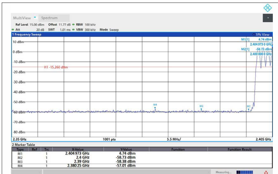
DH5-Ant1-Hop_2402-PASS
