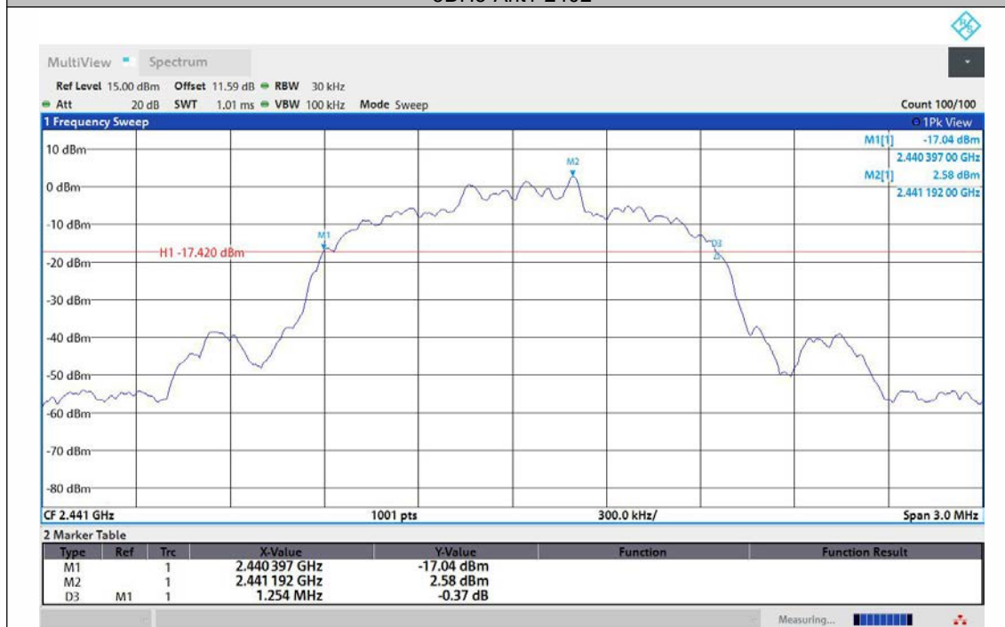
3DH5-Ant1-2441
