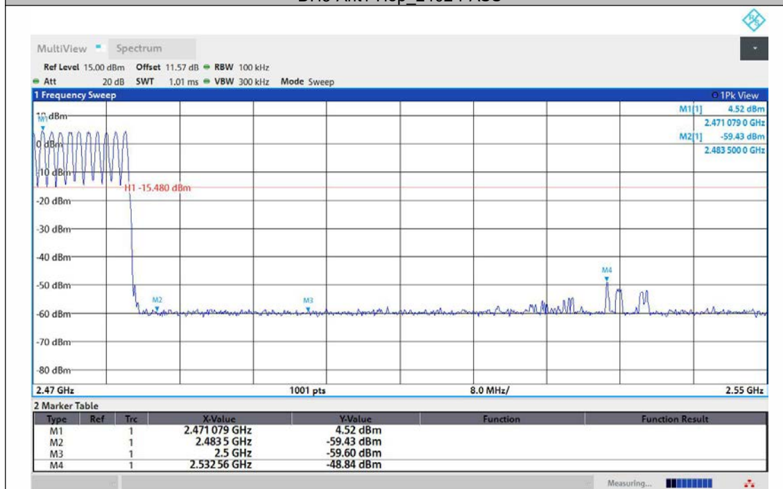
DH5-Ant1-Hop_2480-PASS
