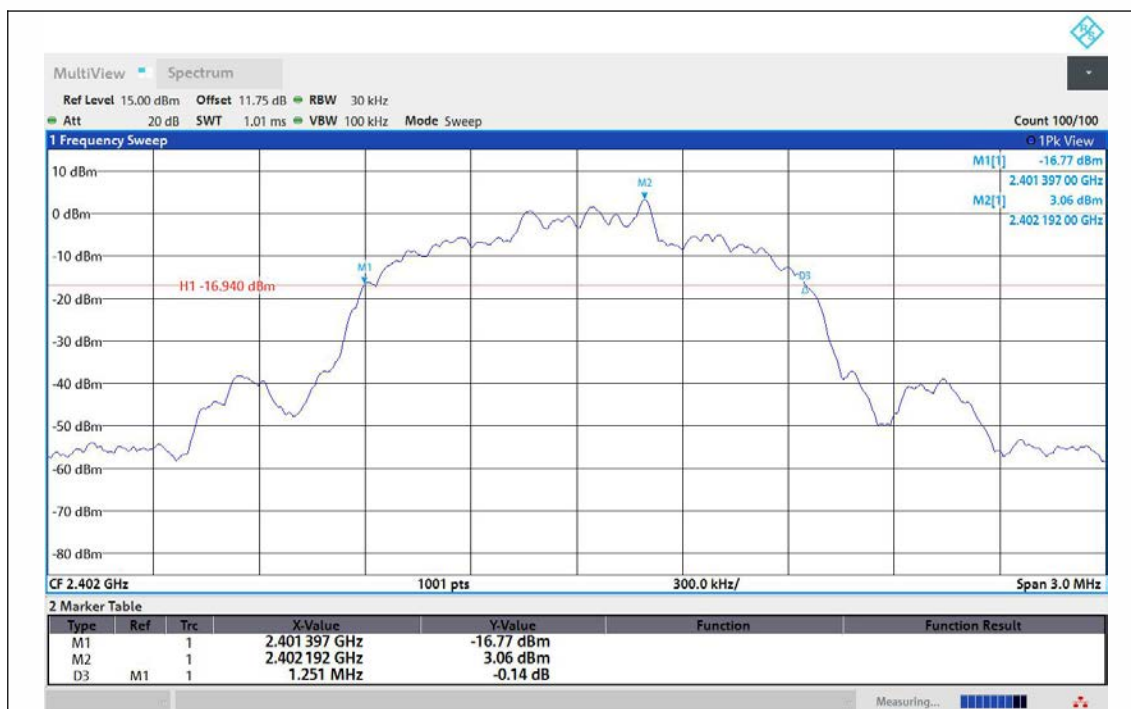
3DH5-Ant1-2402
