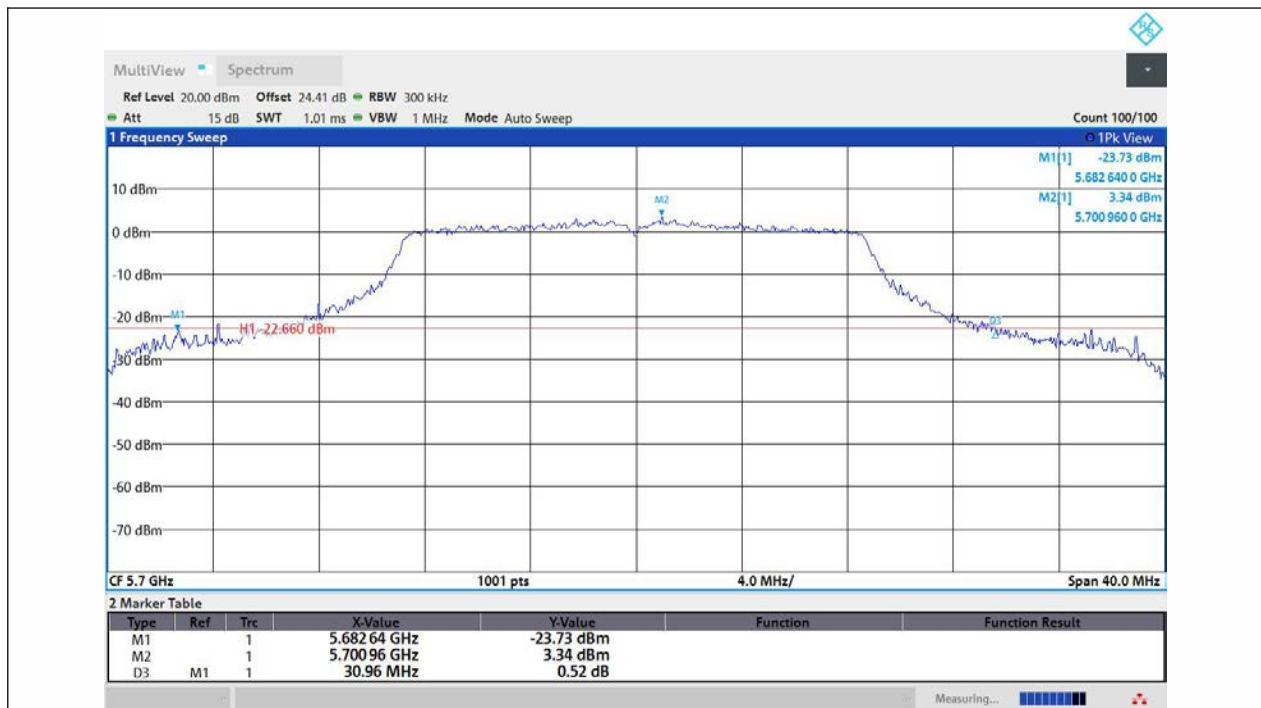
11AC20MIMO-Ant1-5700
