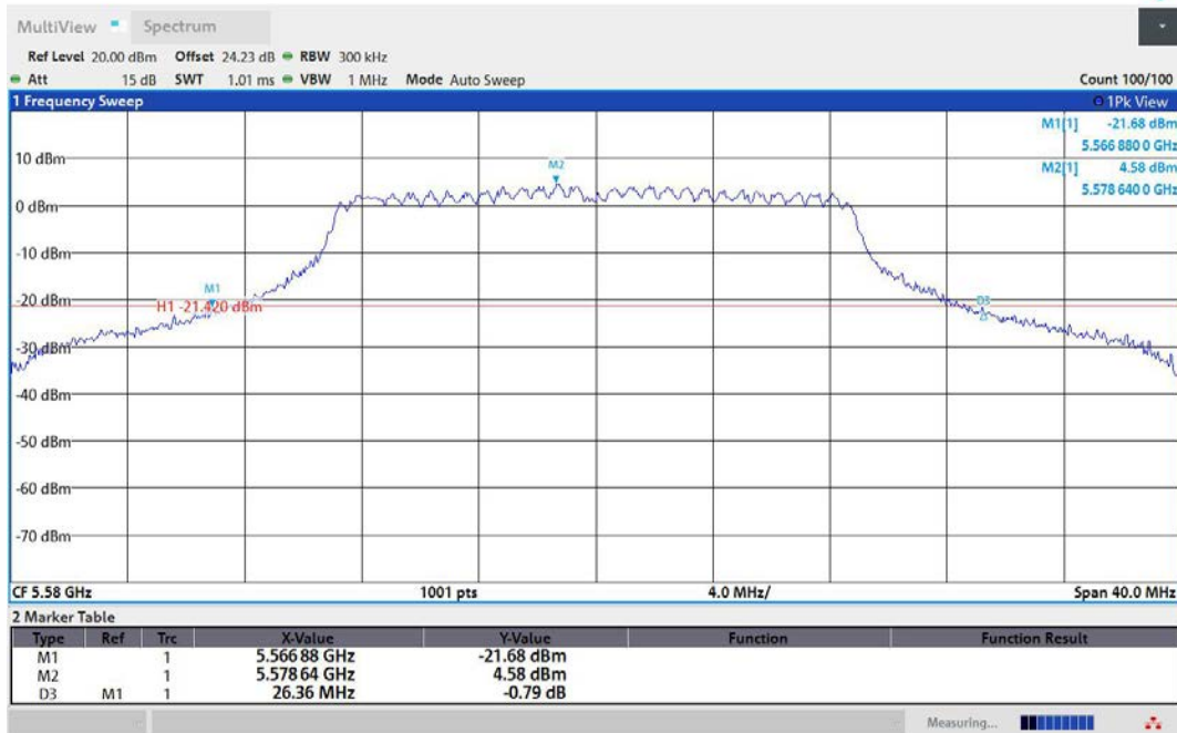
11N20MIMO-Ant2-5580
