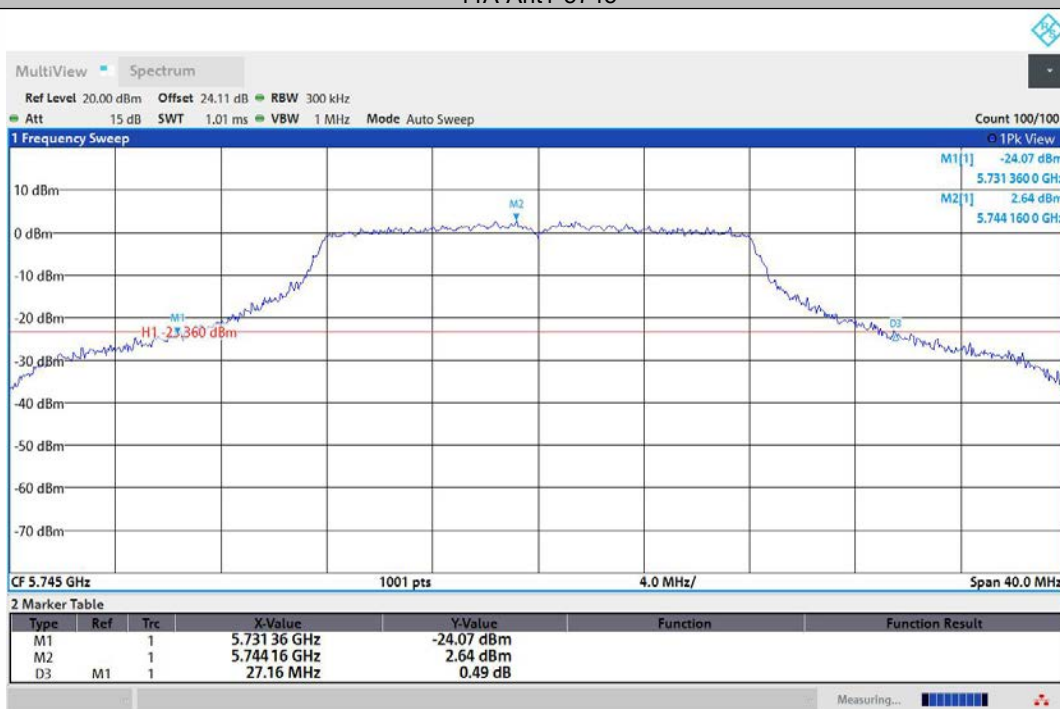
11A-Ant2-5745
