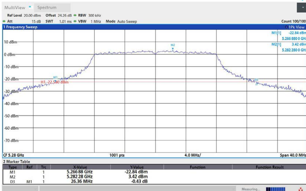
11A-Ant2-5280
