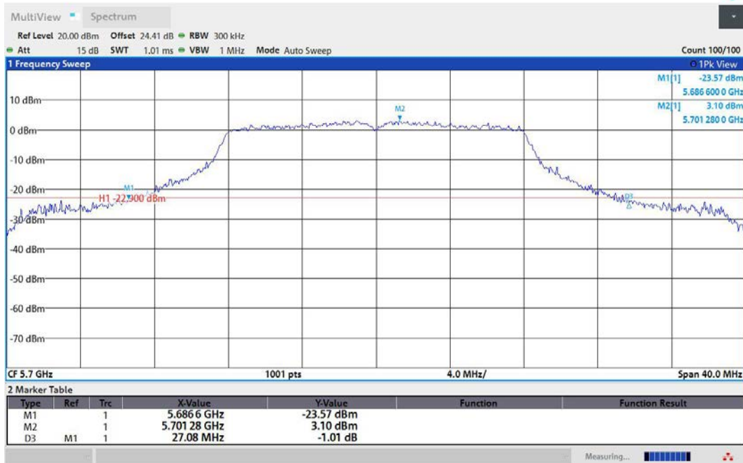
11A-Ant2-5700
