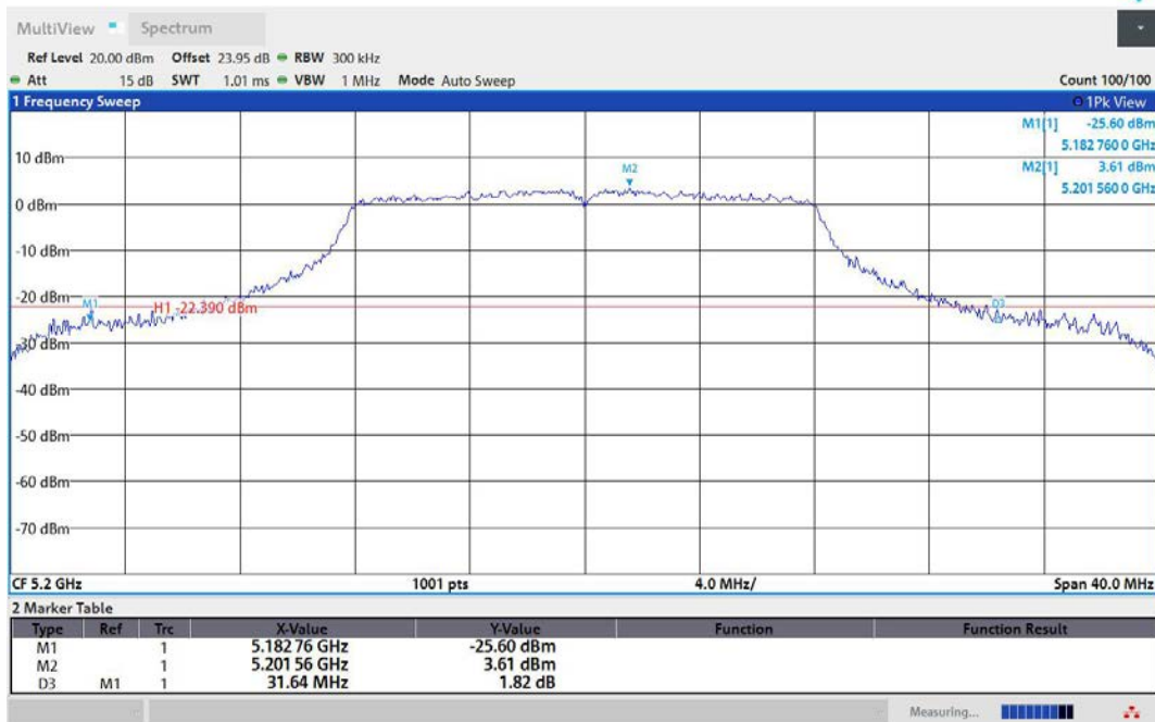
11A-Ant2-5200
