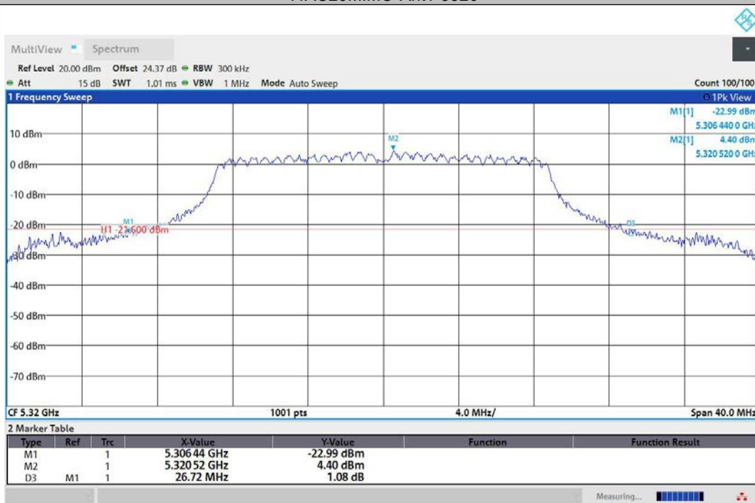
11AC20MIMO-Ant2-5320
