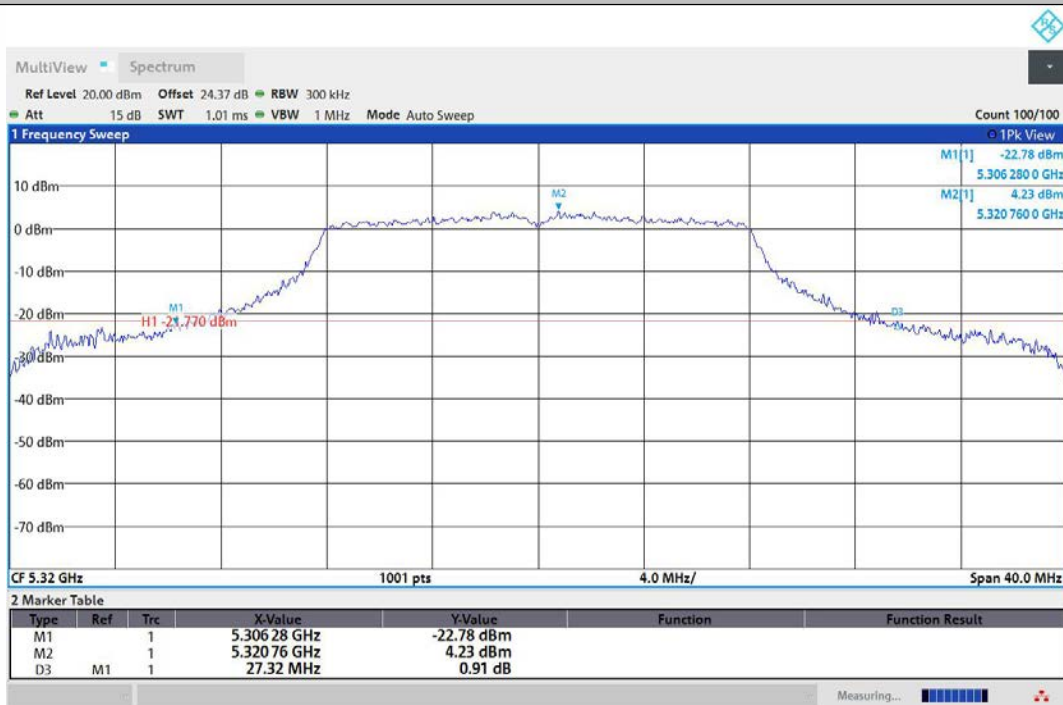
11A-Ant2-5320
