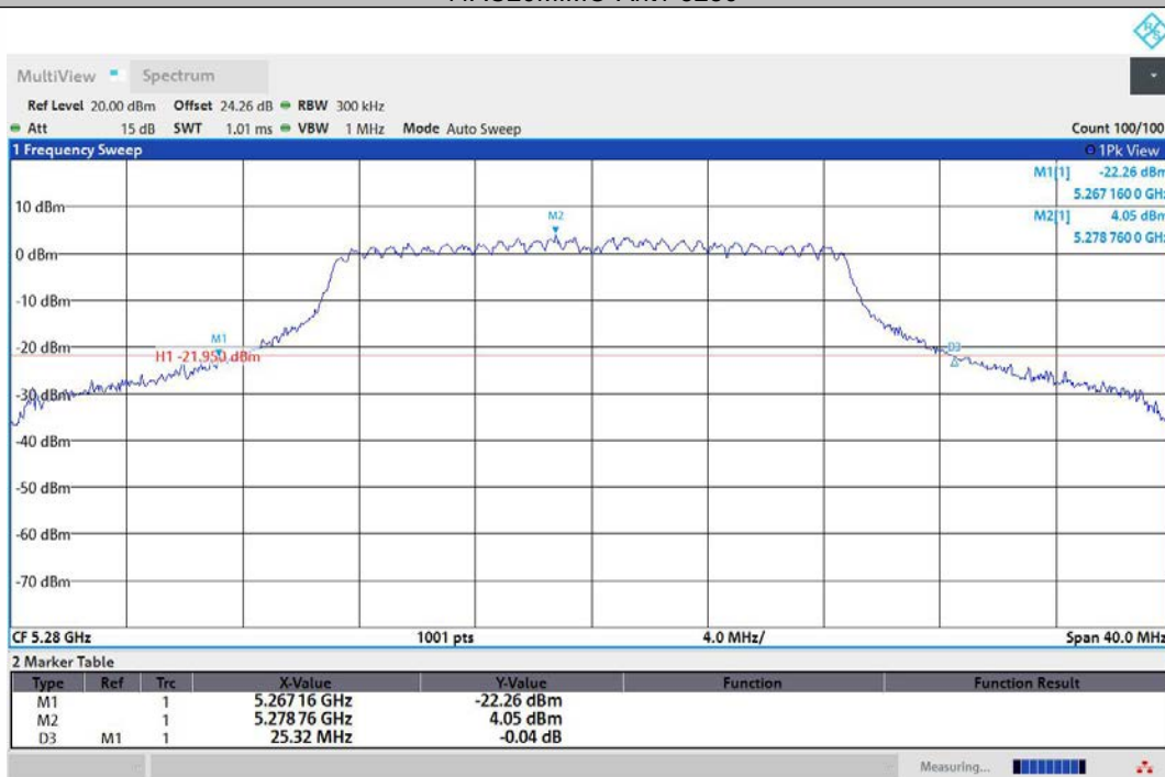
11AC20MIMO-Ant2-5280
