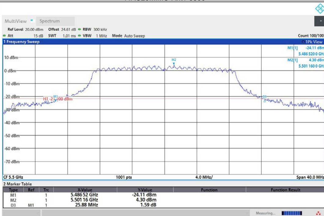
11AC20MIMO-Ant2-5500
