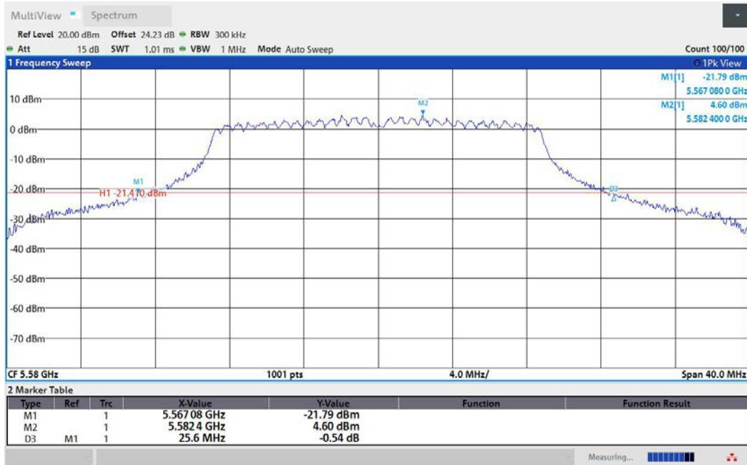
11AC20MIMO-Ant2-5580
