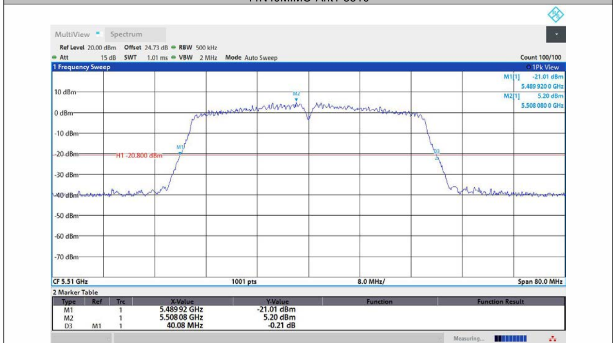
11N40MIMO-Ant2-5510
