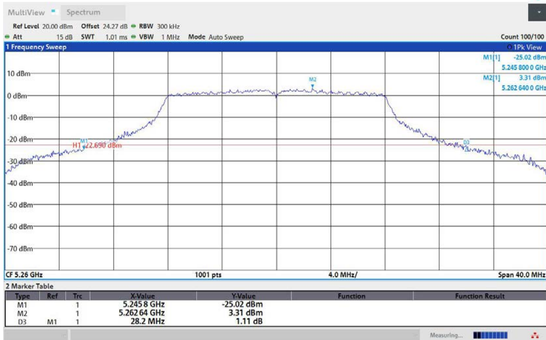
11A-Ant2-5260
