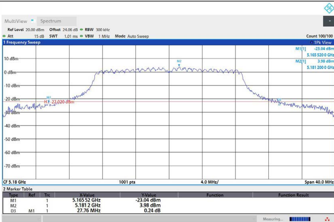
11AC20MIMO-Ant2-5180
