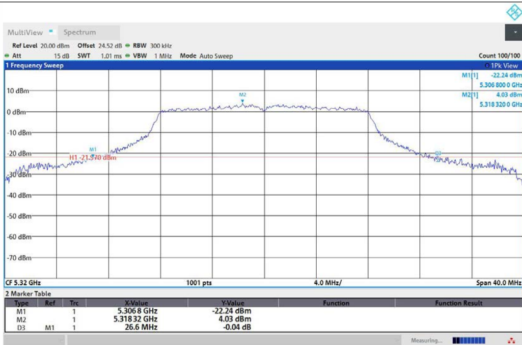
11A-Ant1-5320
