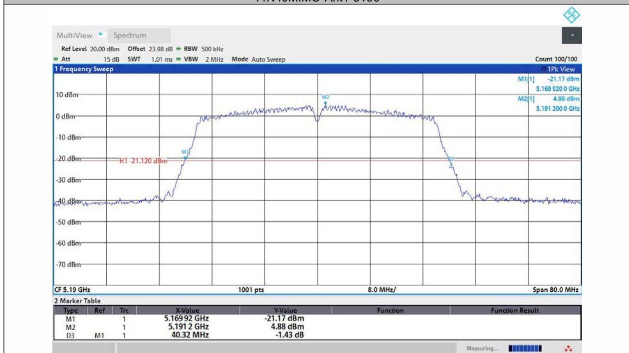
11N40MIMO-Ant2-5190
