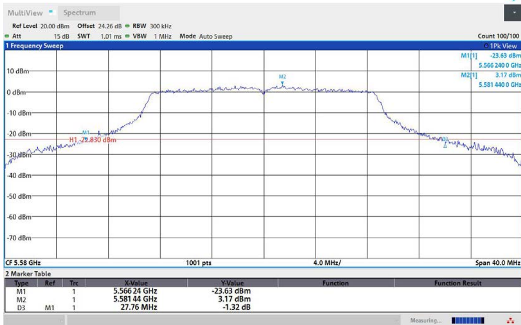
11AC20MIMO-Ant1-5580
