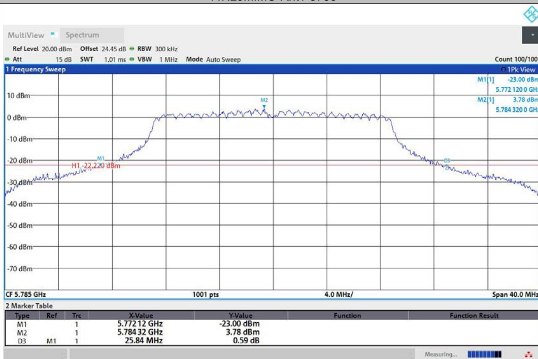
11N20MIMO-Ant2-5785
