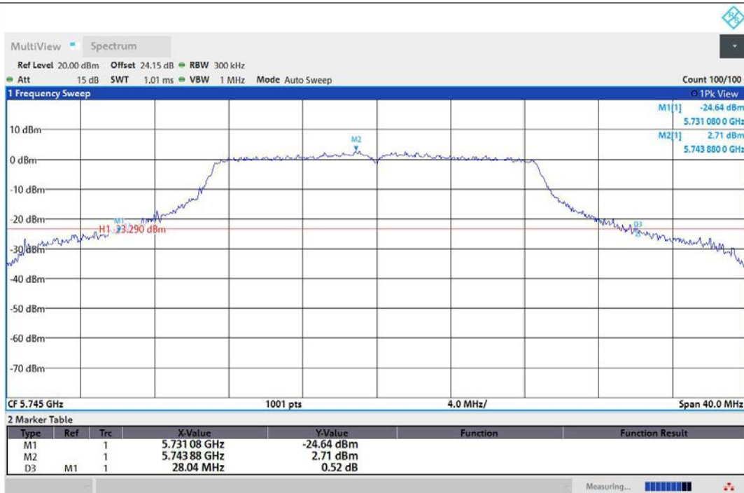
11AC20MIMO-Ant1-5745
