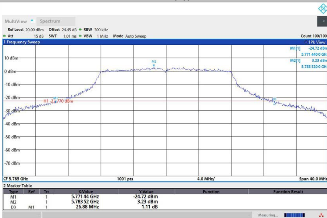
11A-Ant2-5785
