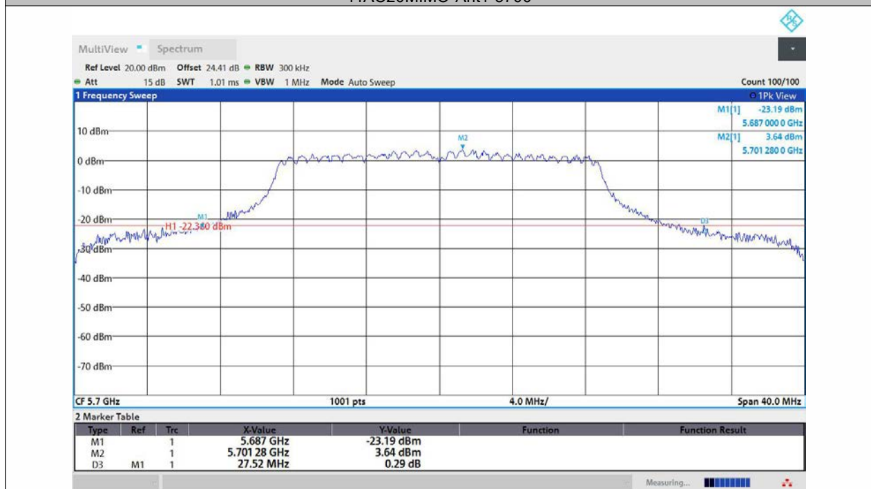
11AC20MIMO-Ant2-5700
