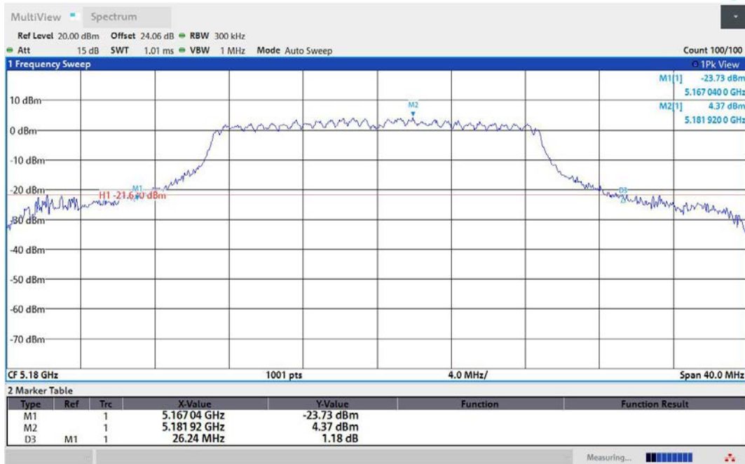
11N20MIMO-Ant2-5180
