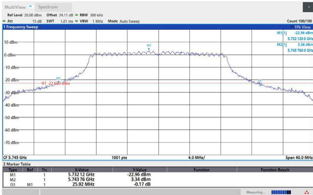
11N20MIMO-Ant2-5745
