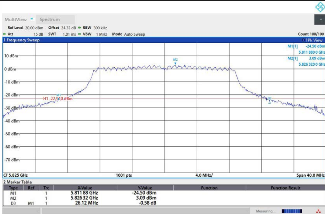
11N20MIMO-Ant2-5825
