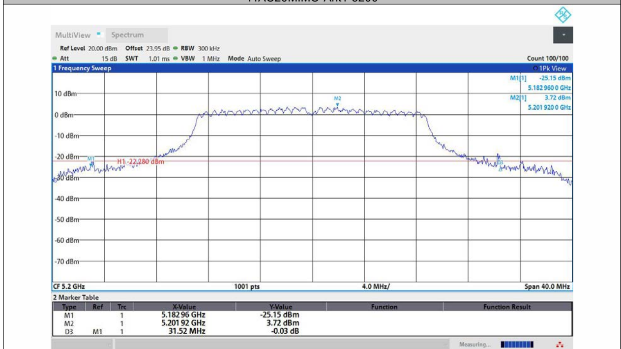
11AC20MIMO-Ant2-5200
