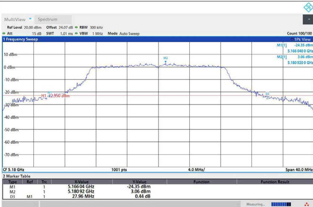
11AC20MIMO-Ant1-5180
