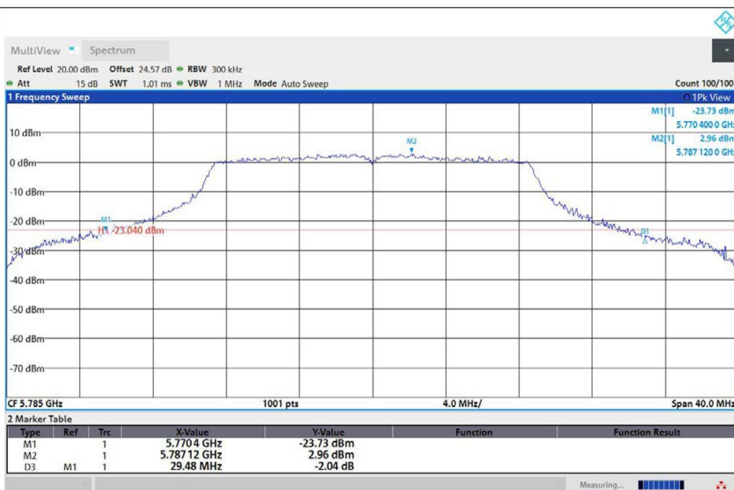
11N20MIMO-Ant1-5785
