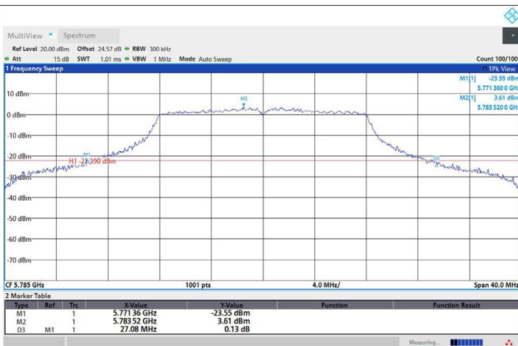
11A-Ant1-5785
