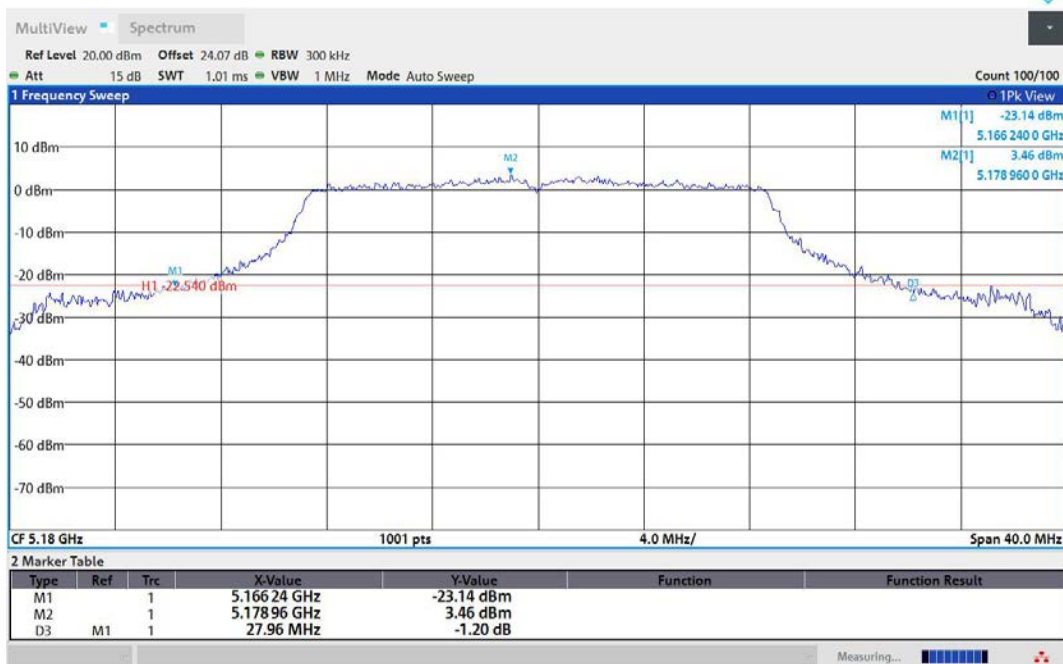
11N20MIMO-Ant1-5180
