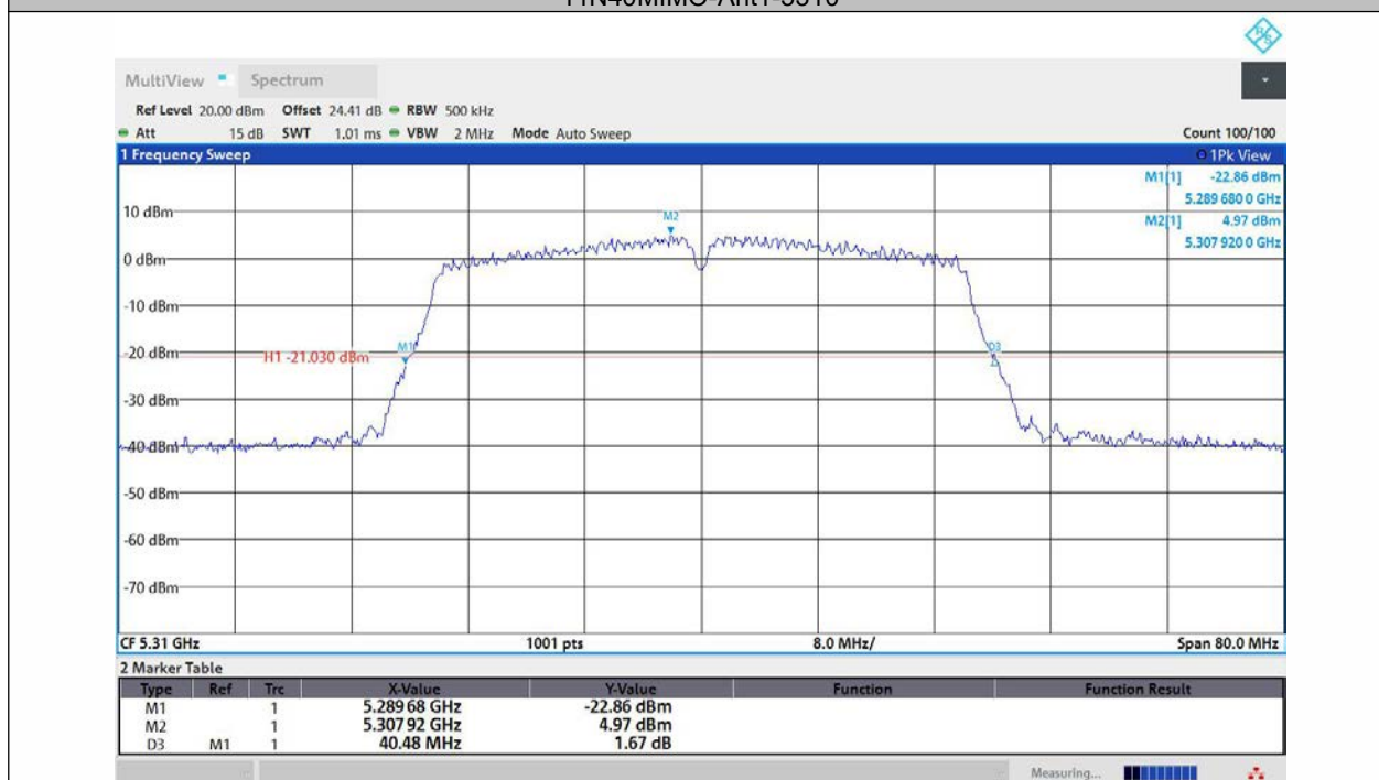
11N40MIMO-Ant2-5310
