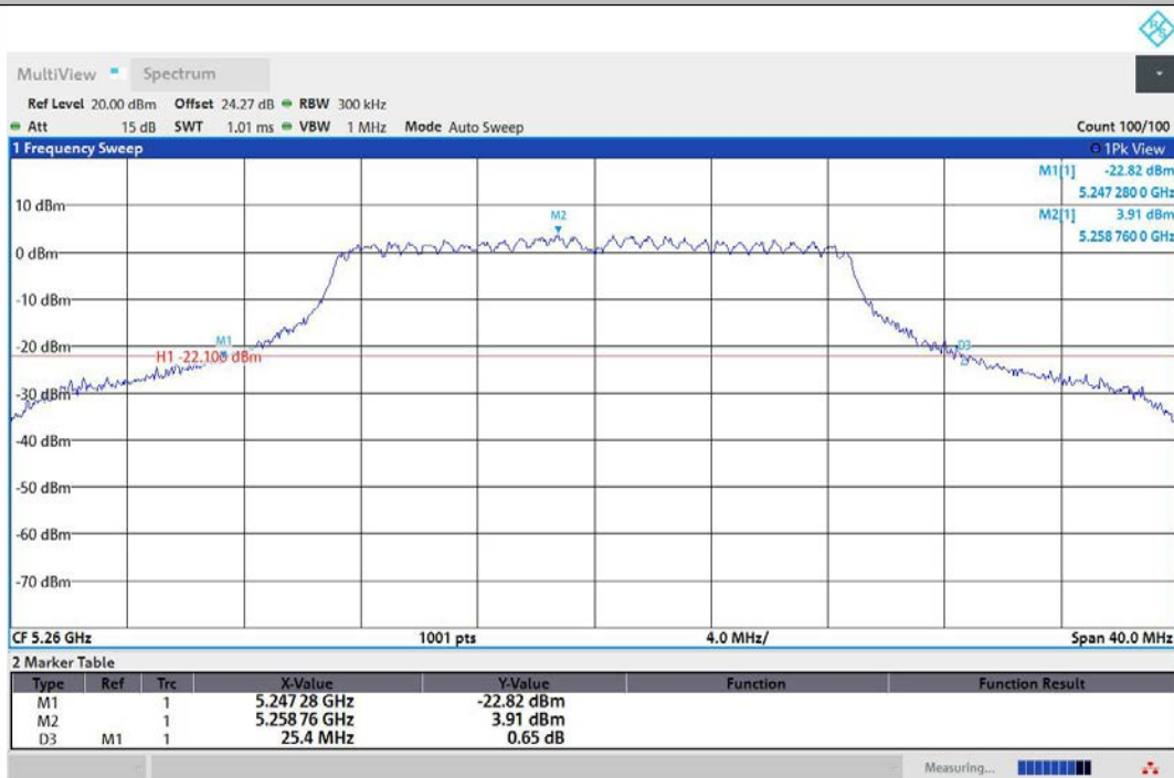
11N20MIMO-Ant2-5260
