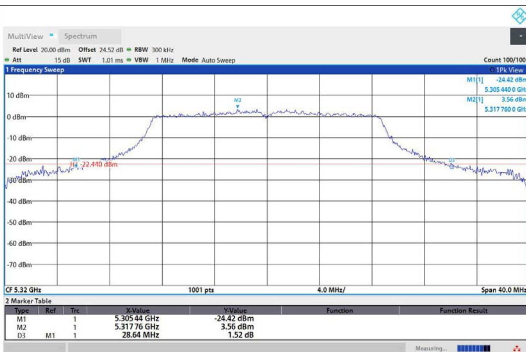
11AC20MIMO-Ant1-5320
