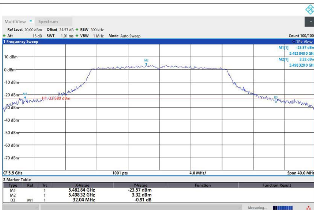
11AC20MIMO-Ant1-5500
