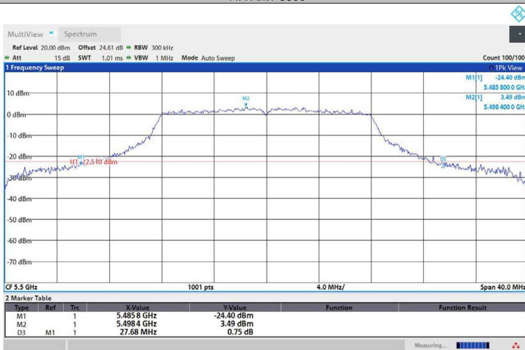
11A-Ant2-5500
