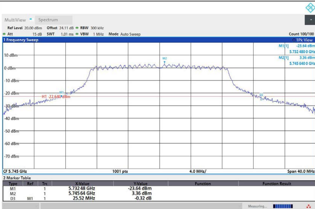
11AC20MIMO-Ant2-5745
