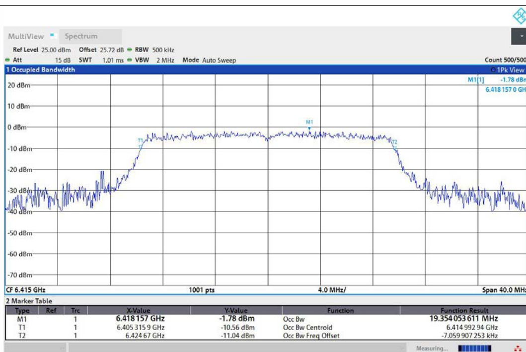
11AX20MIMO-Ant1-6415-PASS
