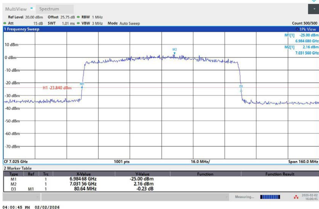
11AX80MIMO-Ant2-7025
