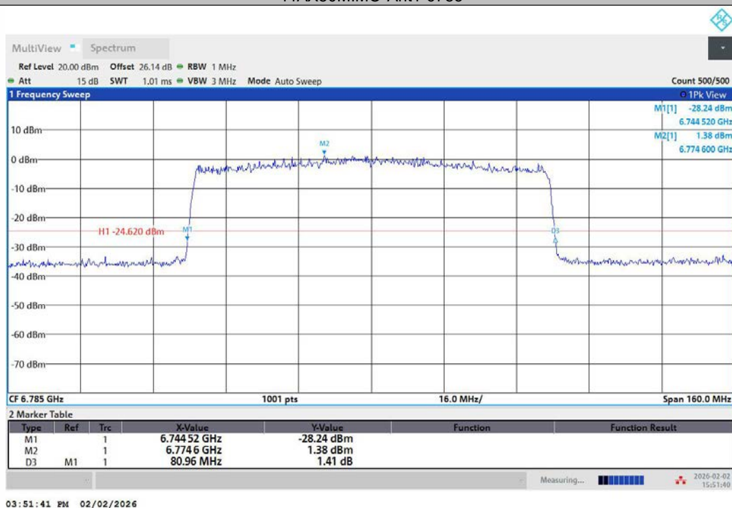
11AX80MIMO-Ant2-6785
