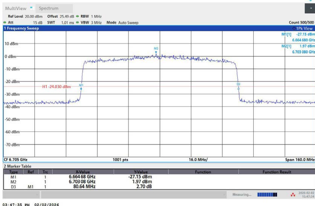
11AX80MIMO-Ant1-6705
