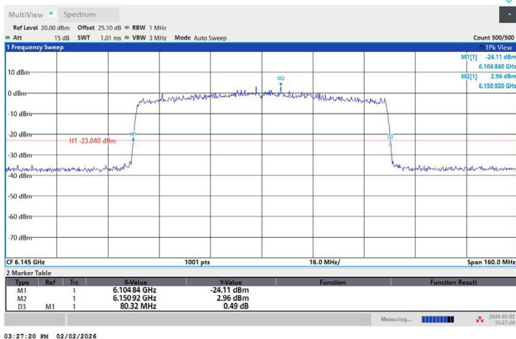
11AX80MIMO-Ant2-6145
