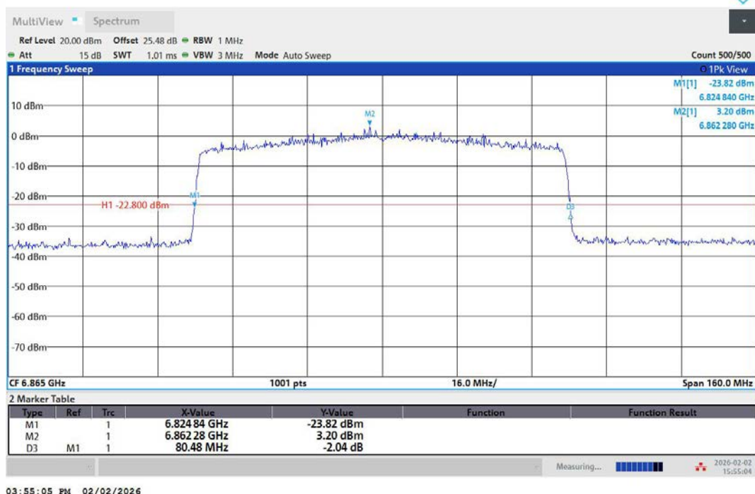
11AX80MIMO-Ant2-6865
