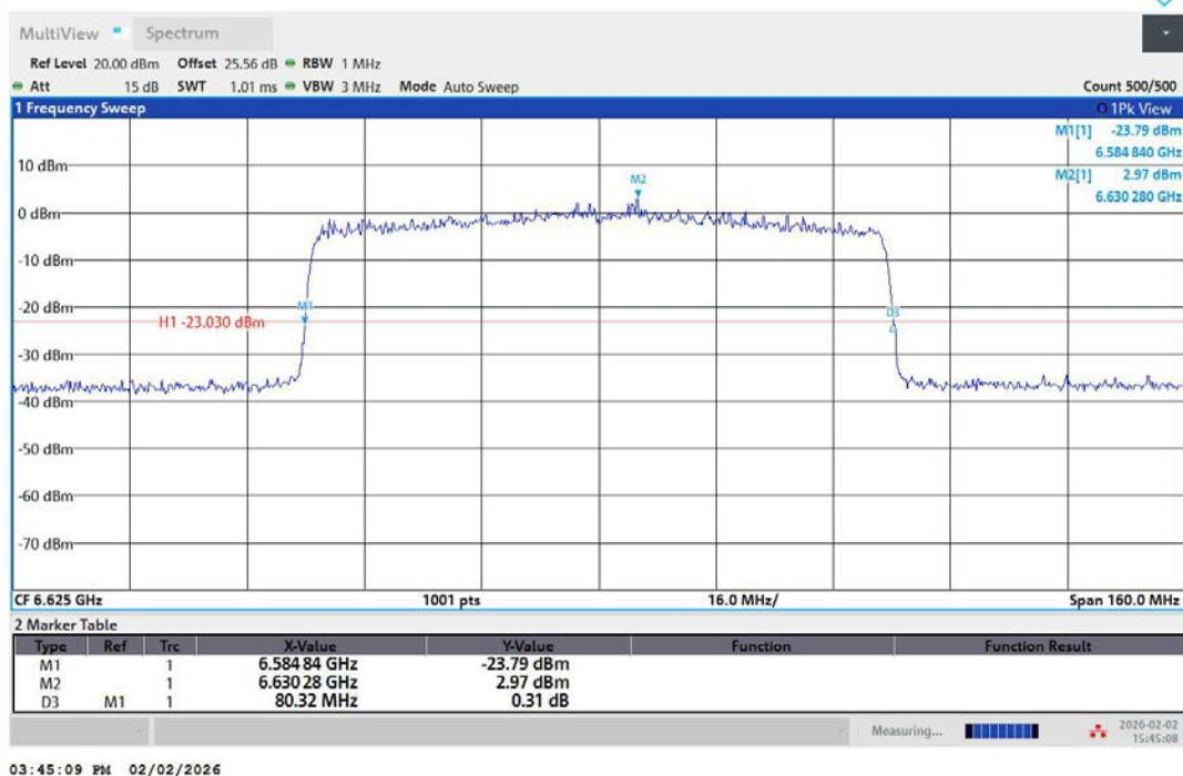
11AX80MIMO-Ant2-6625
