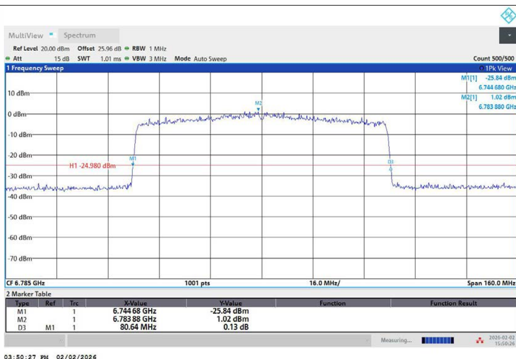
11AX80MIMO-Ant1-6785
