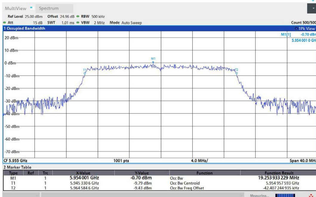
11AX20MIMO-Ant2-5955-PASS
