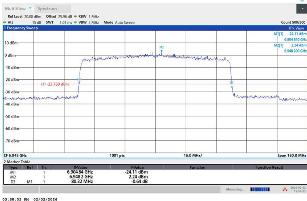
11AX80MIMO-Ant2-6945
