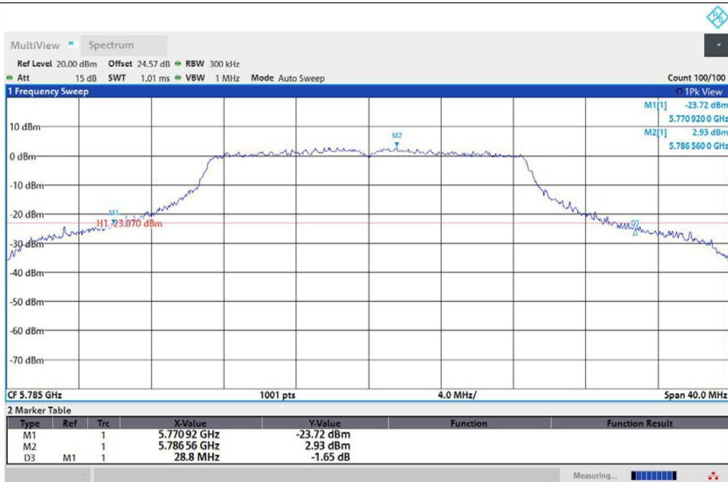
11AC20MIMO-Ant1-5785
