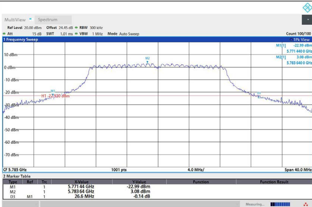
11AC20MIMO-Ant2-5785
