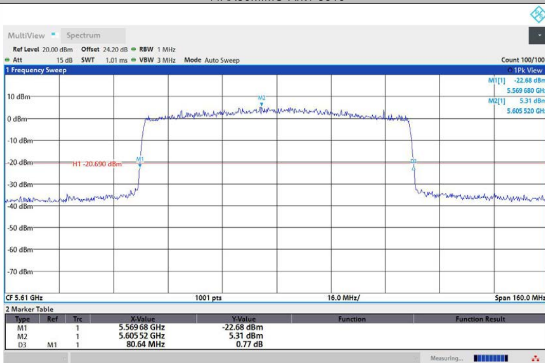
11AX80MIMO-Ant2-5610
