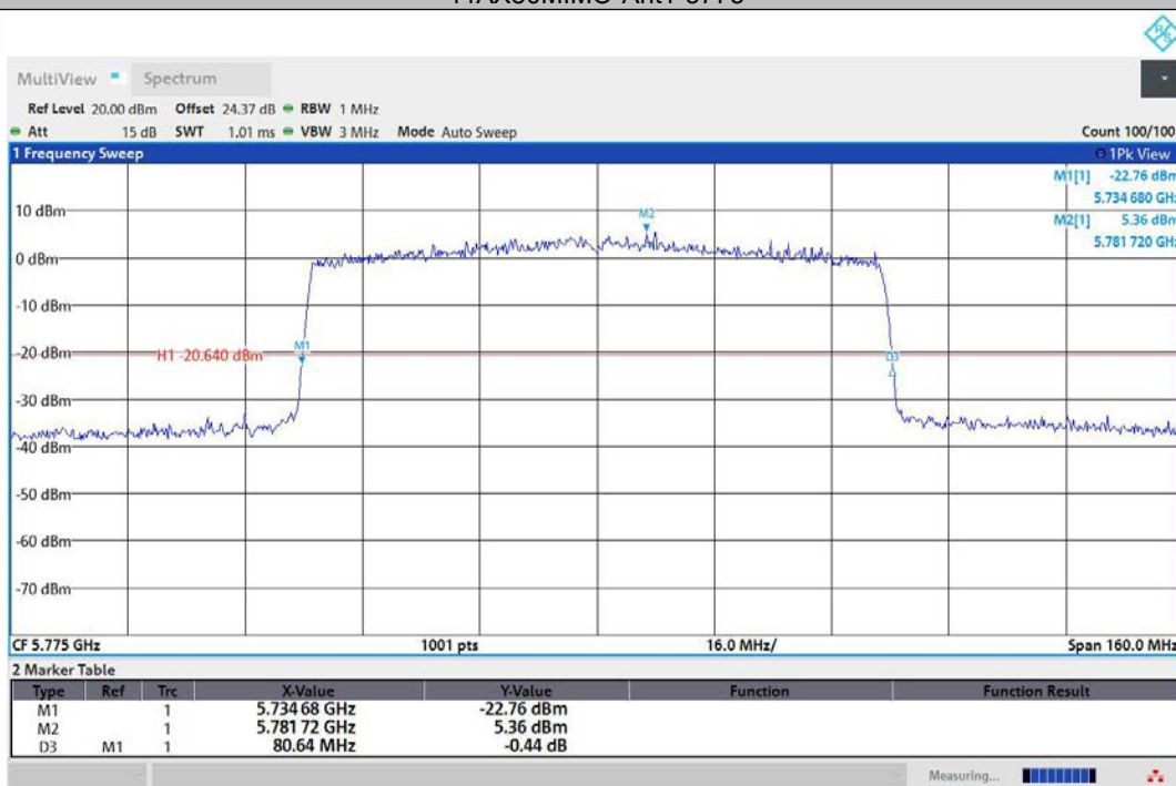
11AX80MIMO-Ant2-5775
