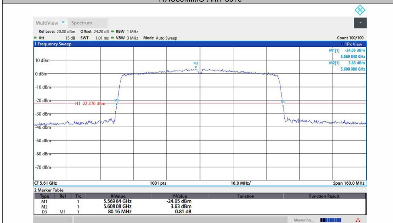
11AC80MIMO-Ant2-5610
