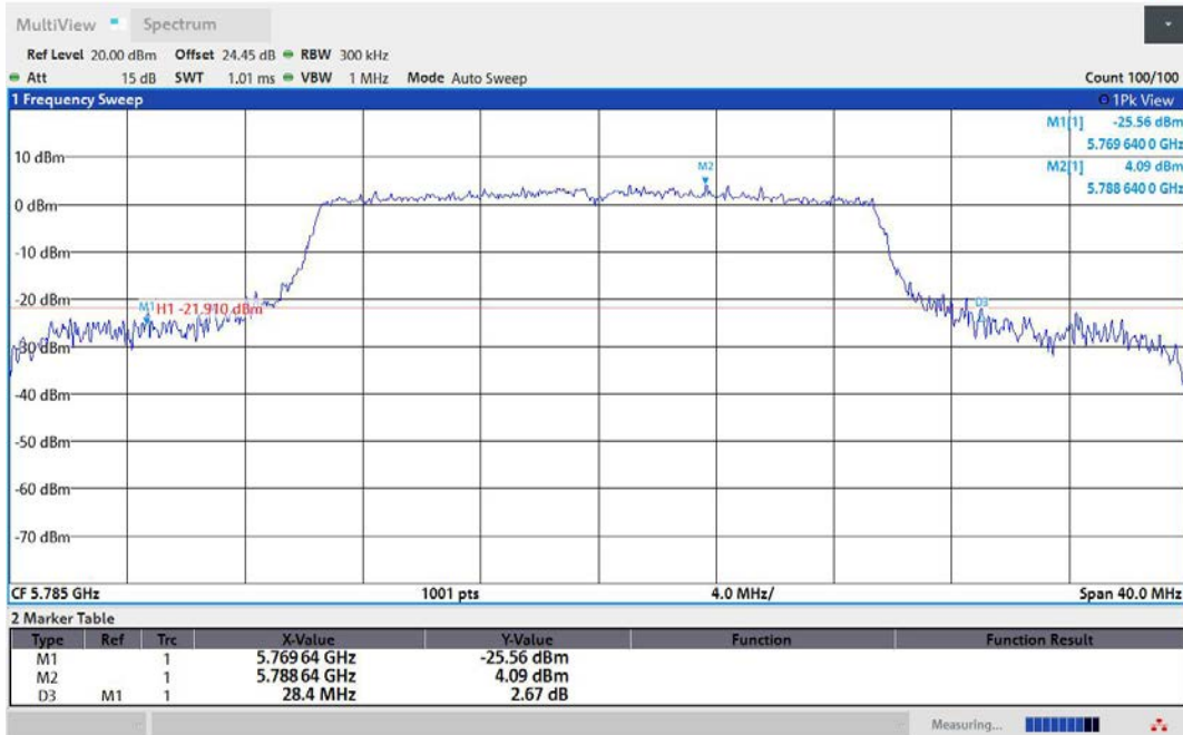
11AX20MIMO-Ant2-5785
