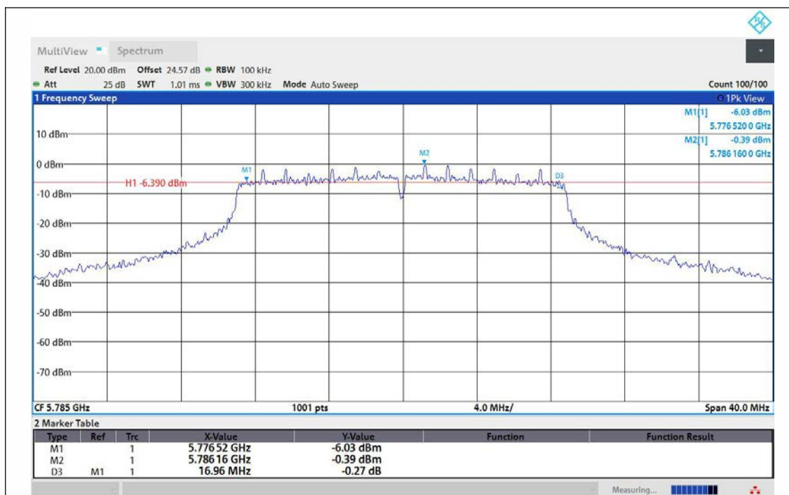
11N20MIMO-Ant1-5785-PASS
