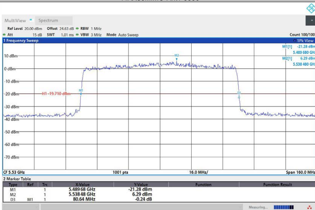
11AX80MIMO-Ant2-5530
