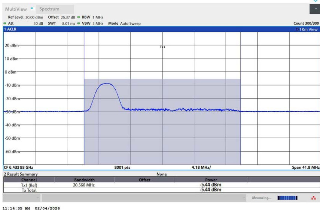
11AX20MIMO-Ant2-6435-26Tone-RU0-PASS
