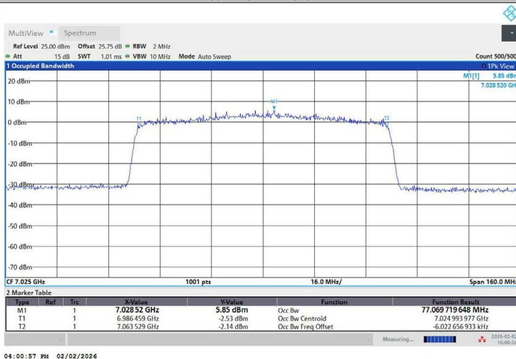
11AX80MIMO-Ant2-7025-PASS
