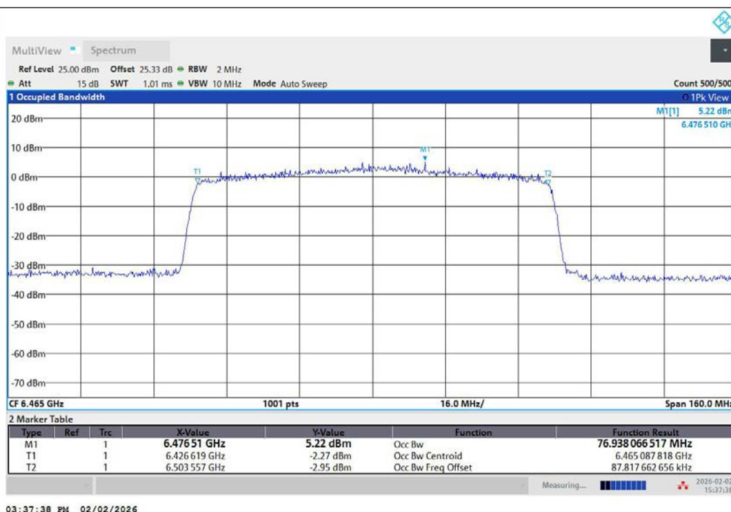
11AX80MIMO-Ant1-6465-PASS
