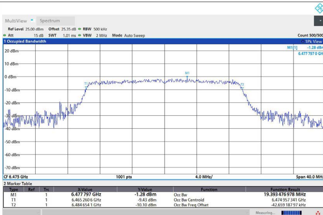
11AX20MIMO-Ant1-6475-PASS
