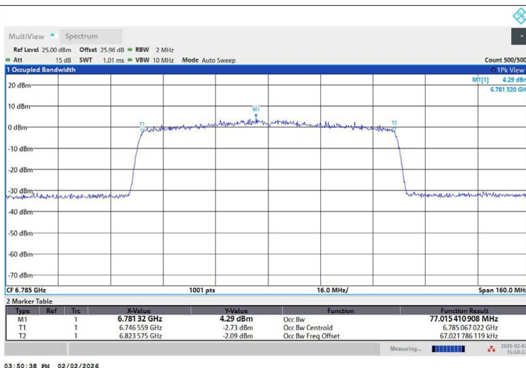
11AX80MIMO-Ant1-6785-PASS
