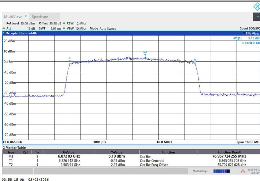
11AX80MIMO-Ant2-6865-PASS
