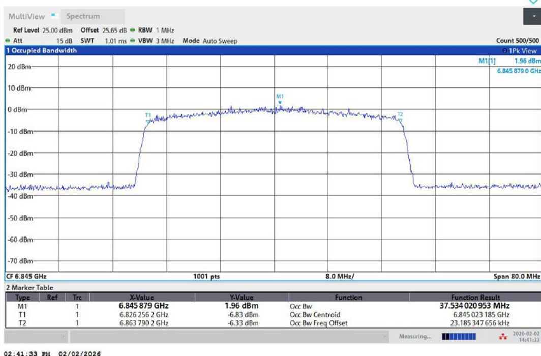
11AX40MIMO-Ant2-6845-PASS
