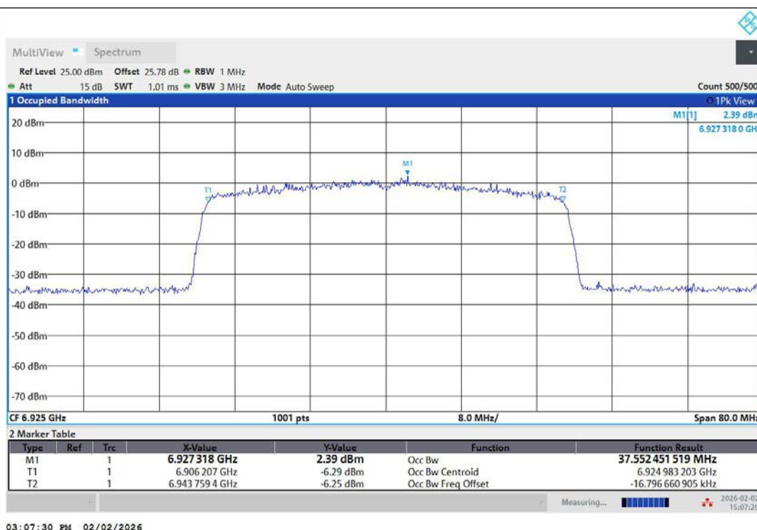
11AX40MIMO-Ant1-6925-PASS
