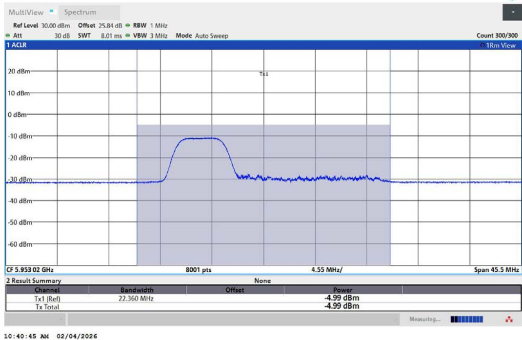
11AX20MIMO-Ant2-5955-52Tone-RU37-PASS
