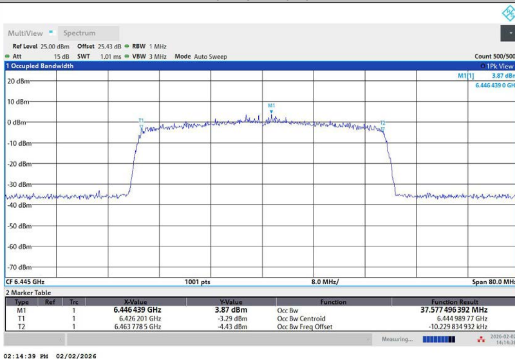
11AX40MIMO-Ant2-6445-PASS
