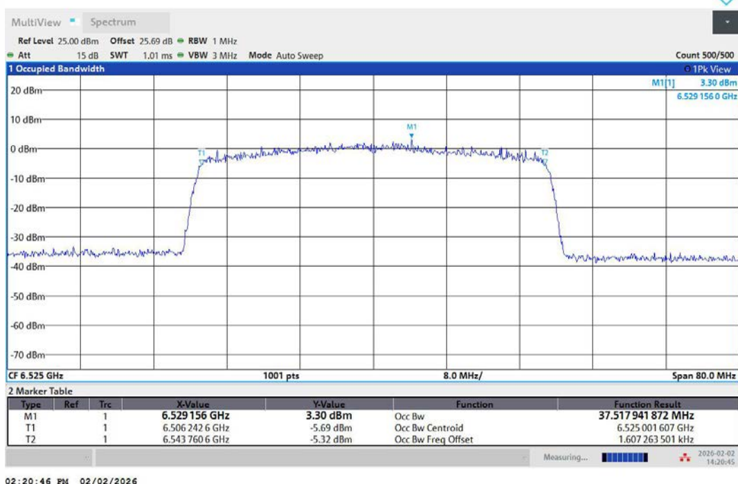
11AX40MIMO-Ant2-6525-PASS
