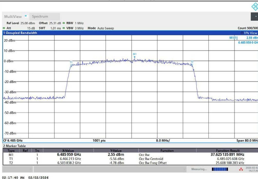
11AX40MIMO-Ant2-6485-PASS
