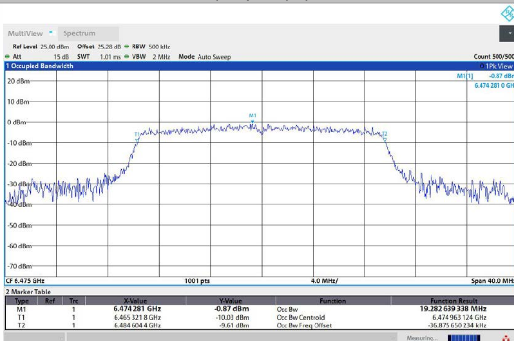
11AX20MIMO-Ant2-6475-PASS
