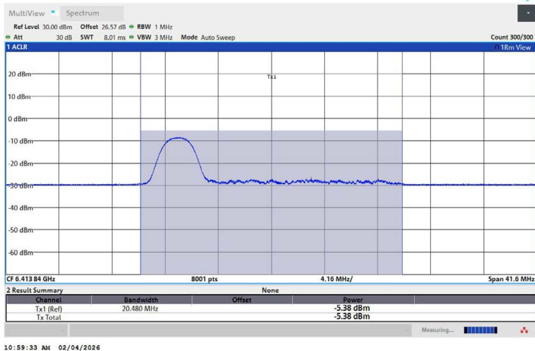
11AX20MIMO-Ant1-6415-26Tone-RU0-PASS
