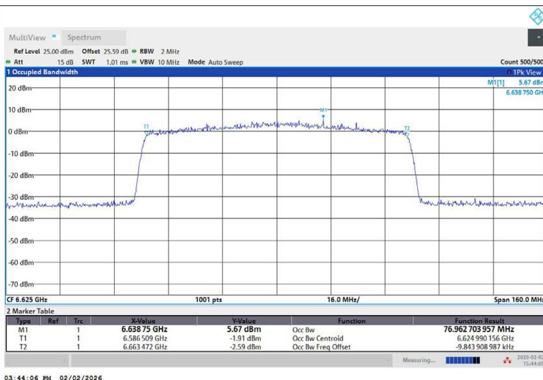
11AX80MIMO-Ant1-6625-PASS
