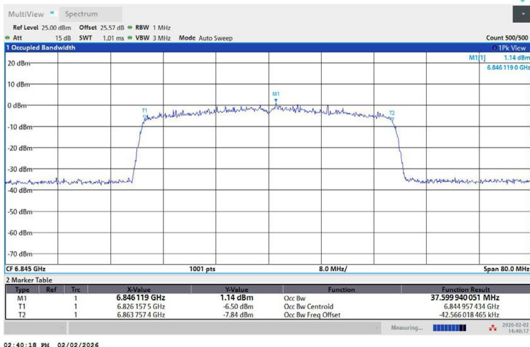
11AX40MIMO-Ant1-6845-PASS
