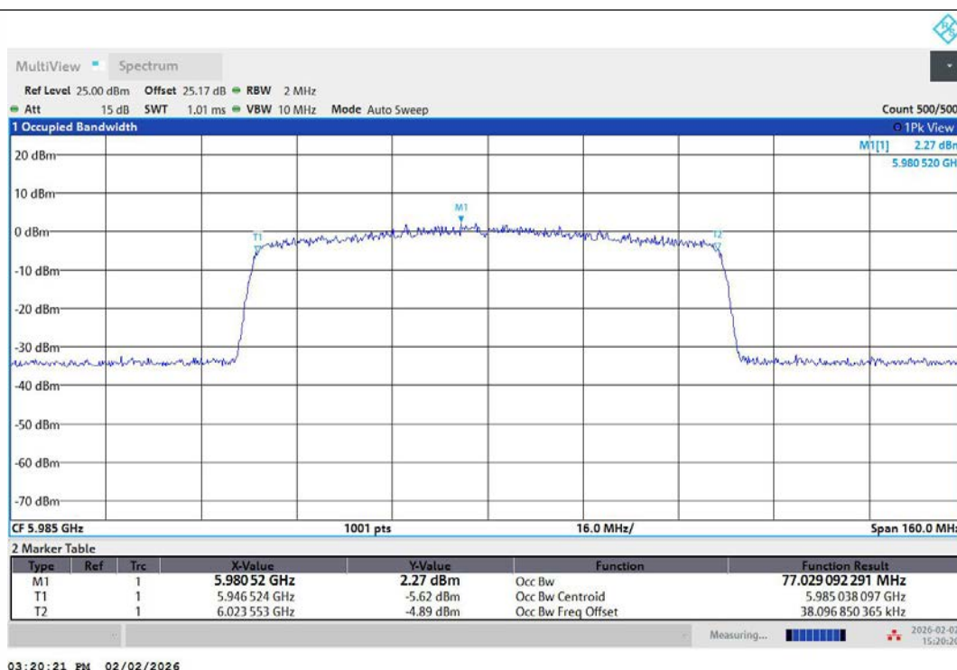
11AX80MIMO-Ant1-5985-PASS
