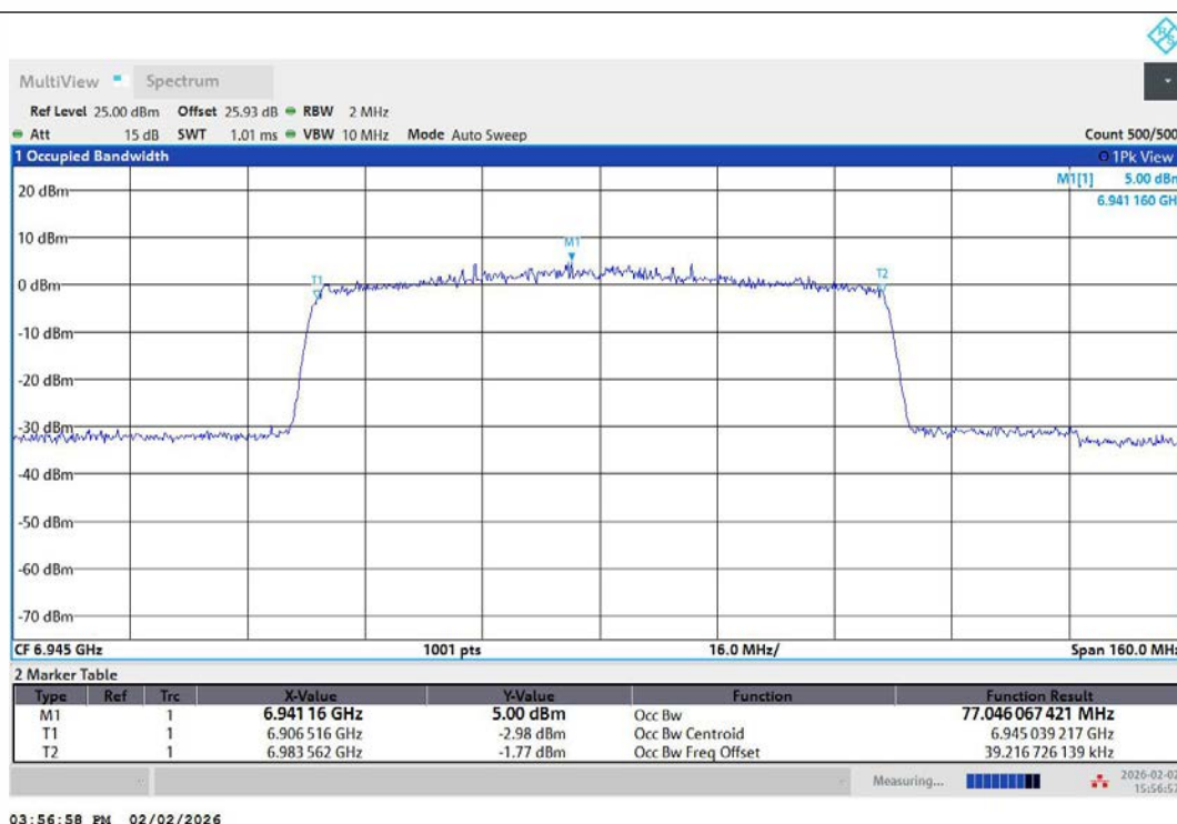
11AX80MIMO-Ant1-6945-PASS
