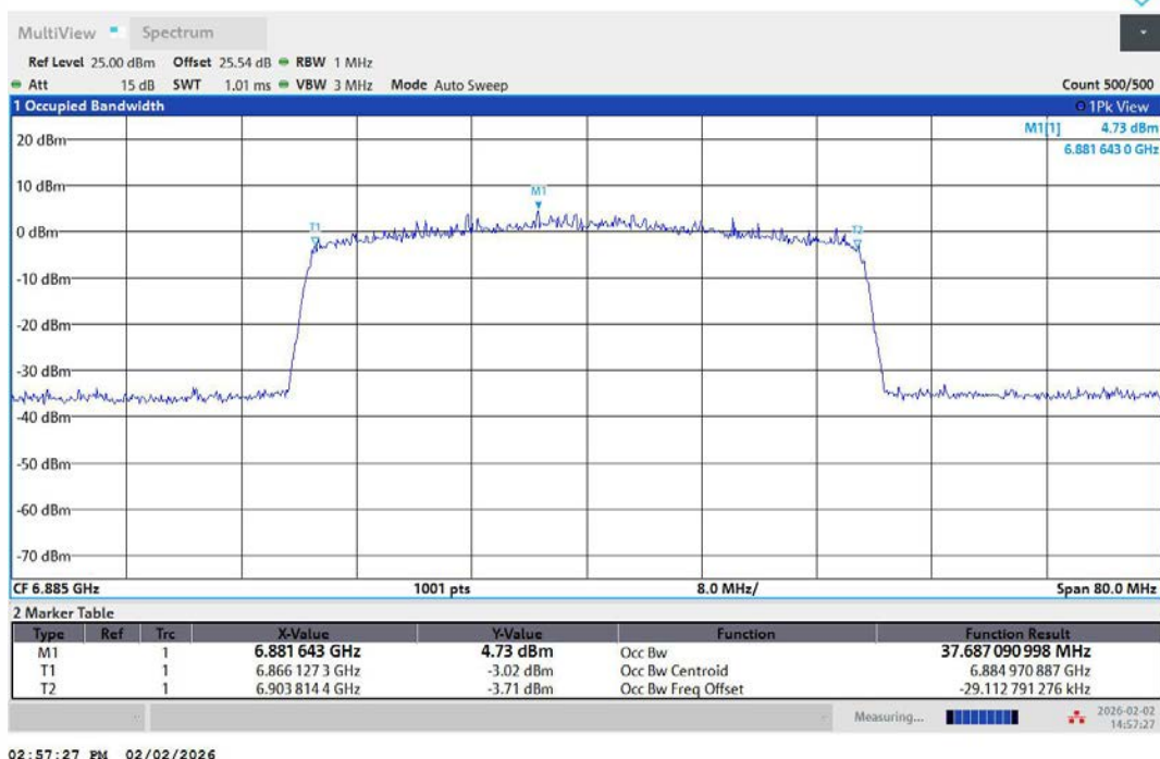
11AX40MIMO-Ant2-6885-PASS
