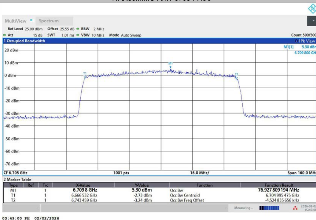
11AX80MIMO-Ant2-6705-PASS
