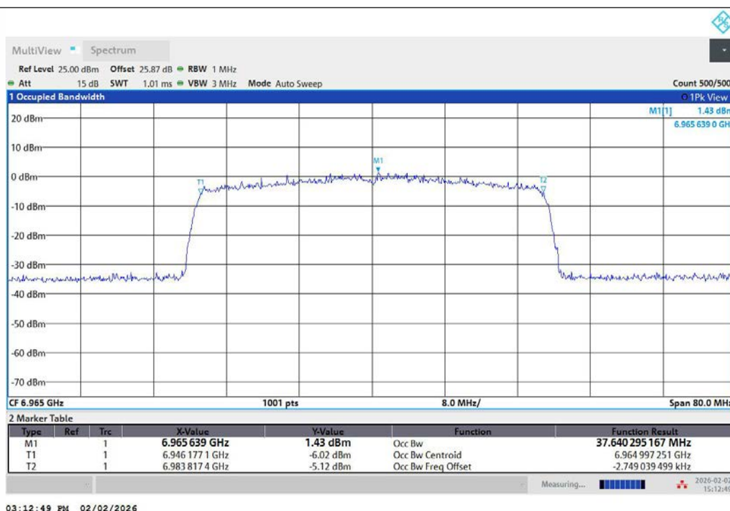
11AX40MIMO-Ant1-6965-PASS
