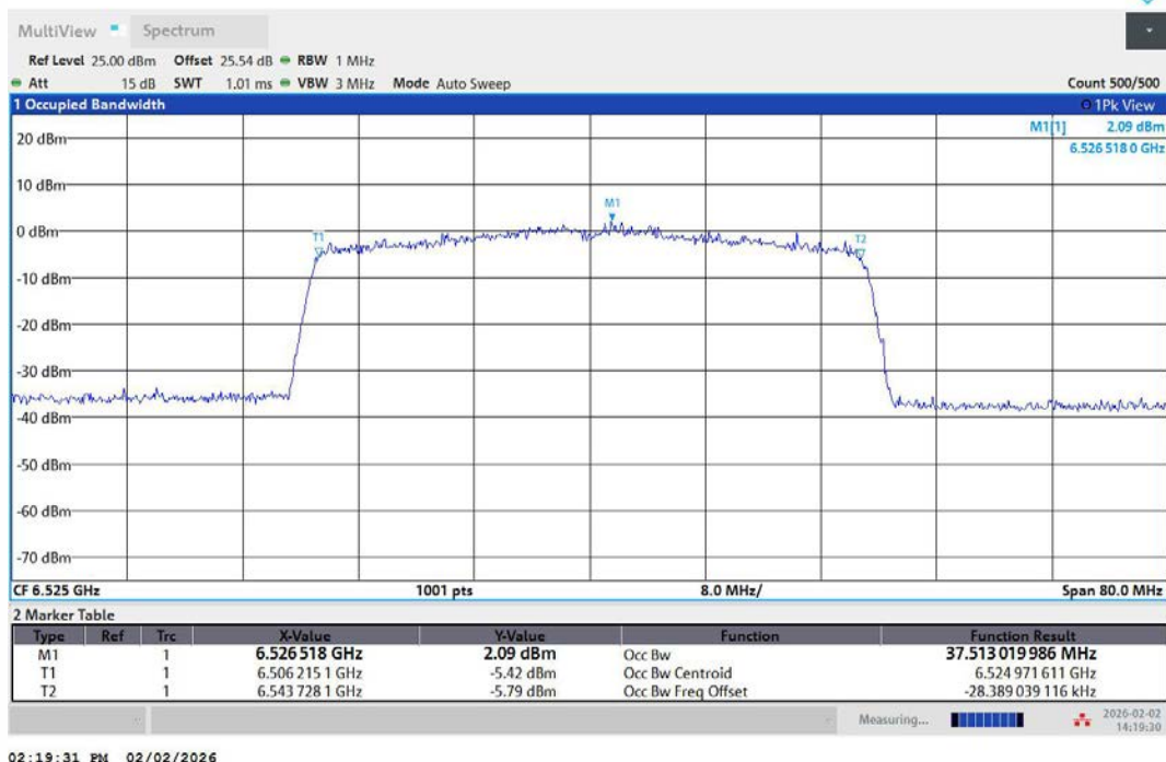
11AX40MIMO-Ant1-6525-PASS
