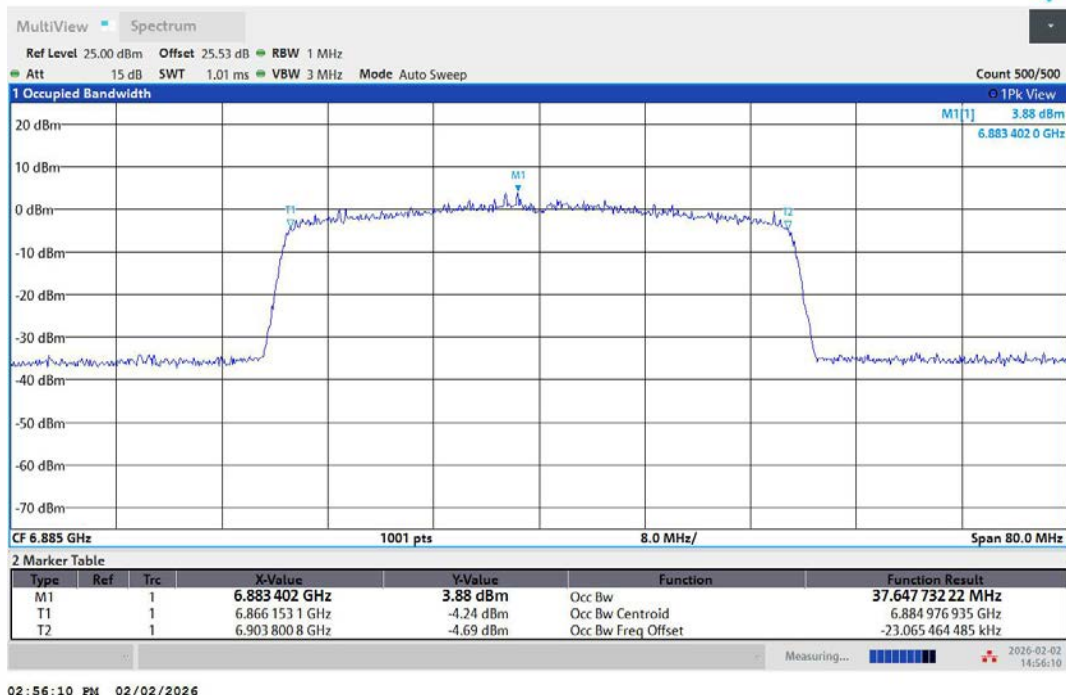
11AX40MIMO-Ant1-6885-PASS
