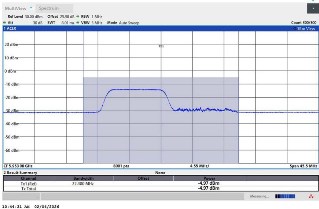
11AX20MIMO-Ant2-5955-106Tone-RU53-PASS
