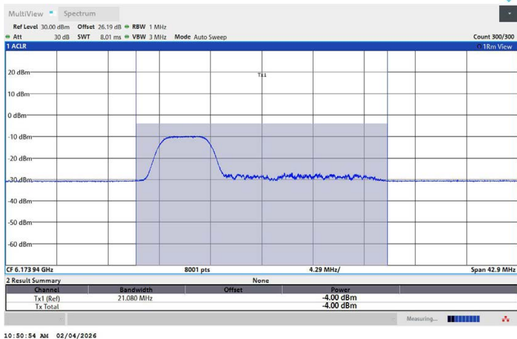
11AX20MIMO-Ant1-6175-52Tone-RU37-PASS
