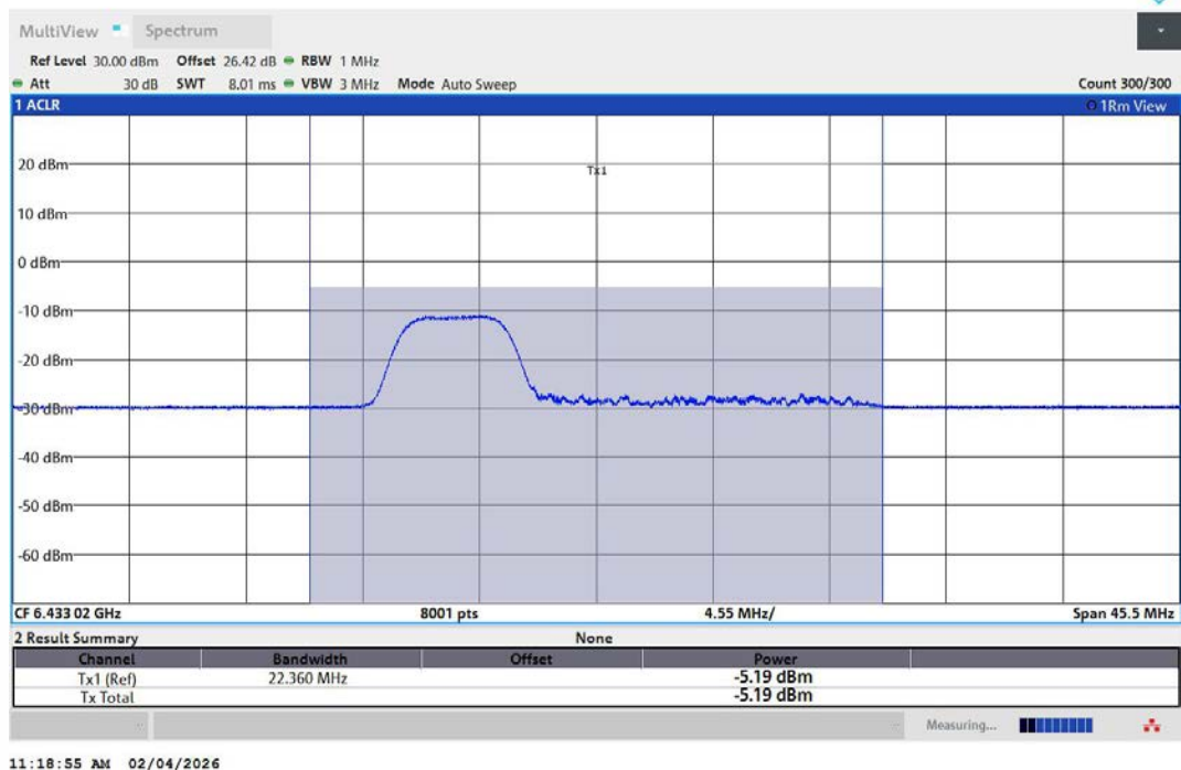
11AX20MIMO-Ant2-6435-52Tone-RU37-PASS
