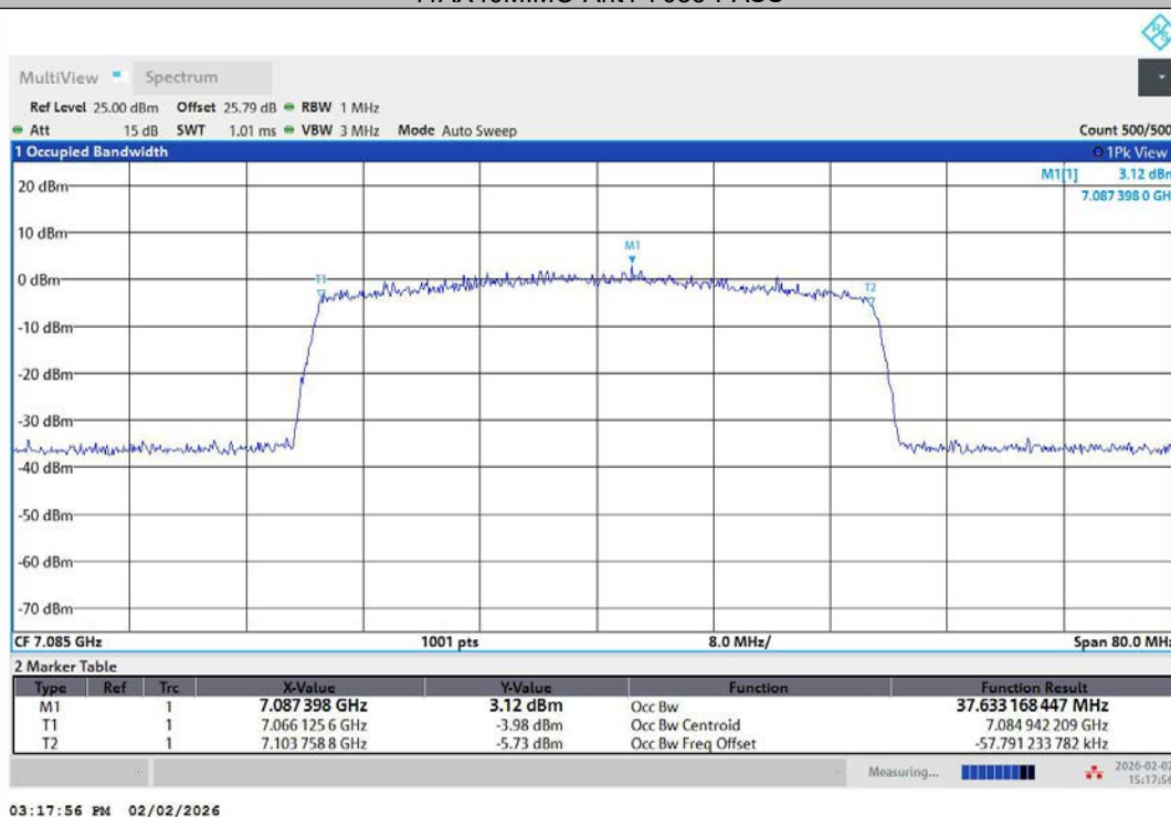
11AX40MIMO-Ant2-7085-PASS
