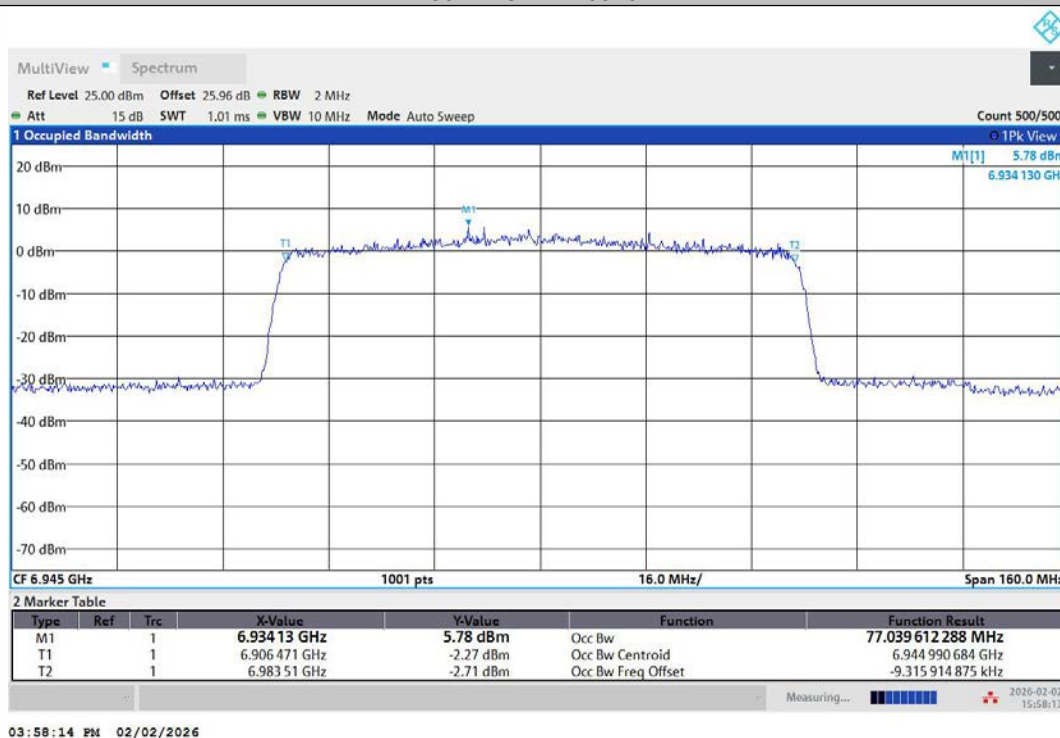
11AX80MIMO-Ant2-6945-PASS
