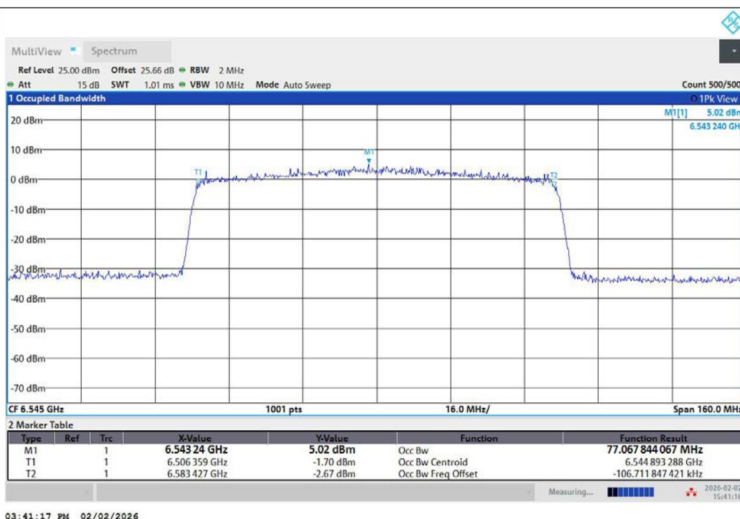
11AX80MIMO-Ant1-6545-PASS
