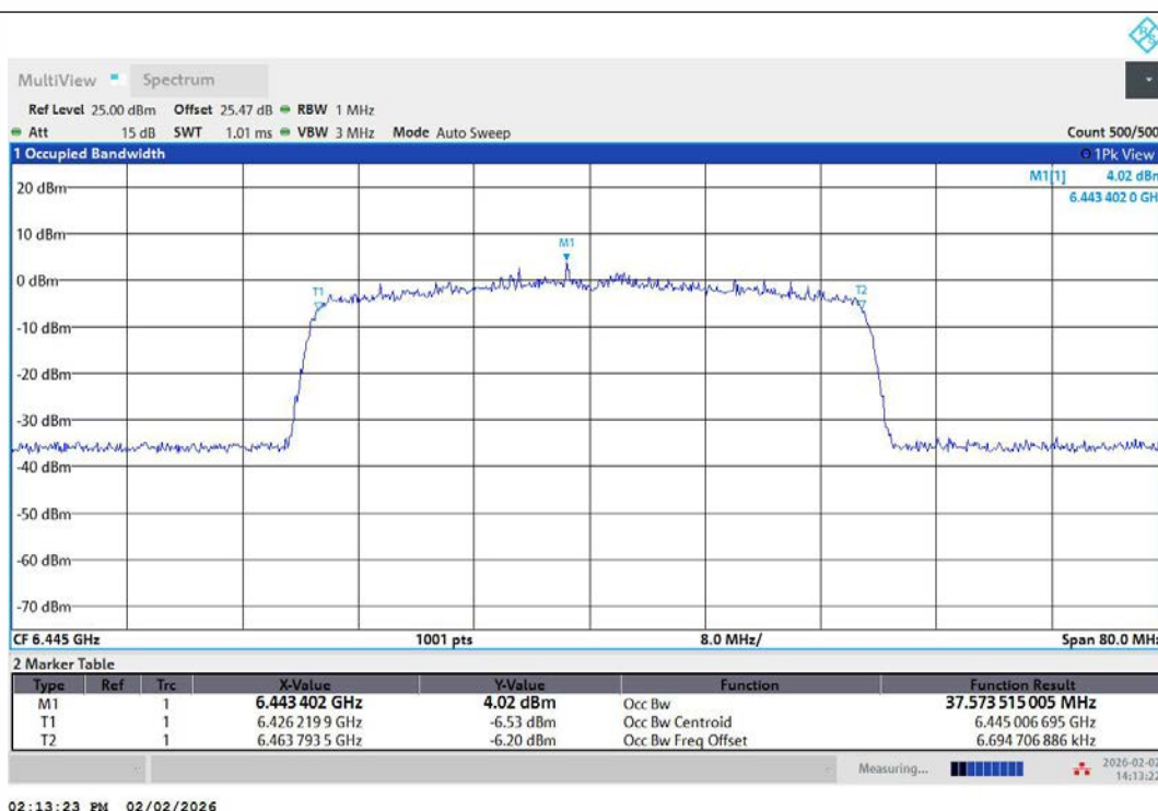
11AX40MIMO-Ant1-6445-PASS
