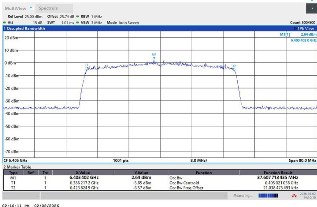
11AX40MIMO-Ant1-6405-PASS
