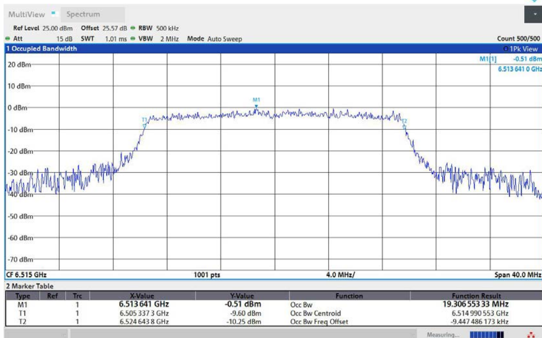
11AX20MIMO-Ant2-6515-PASS
