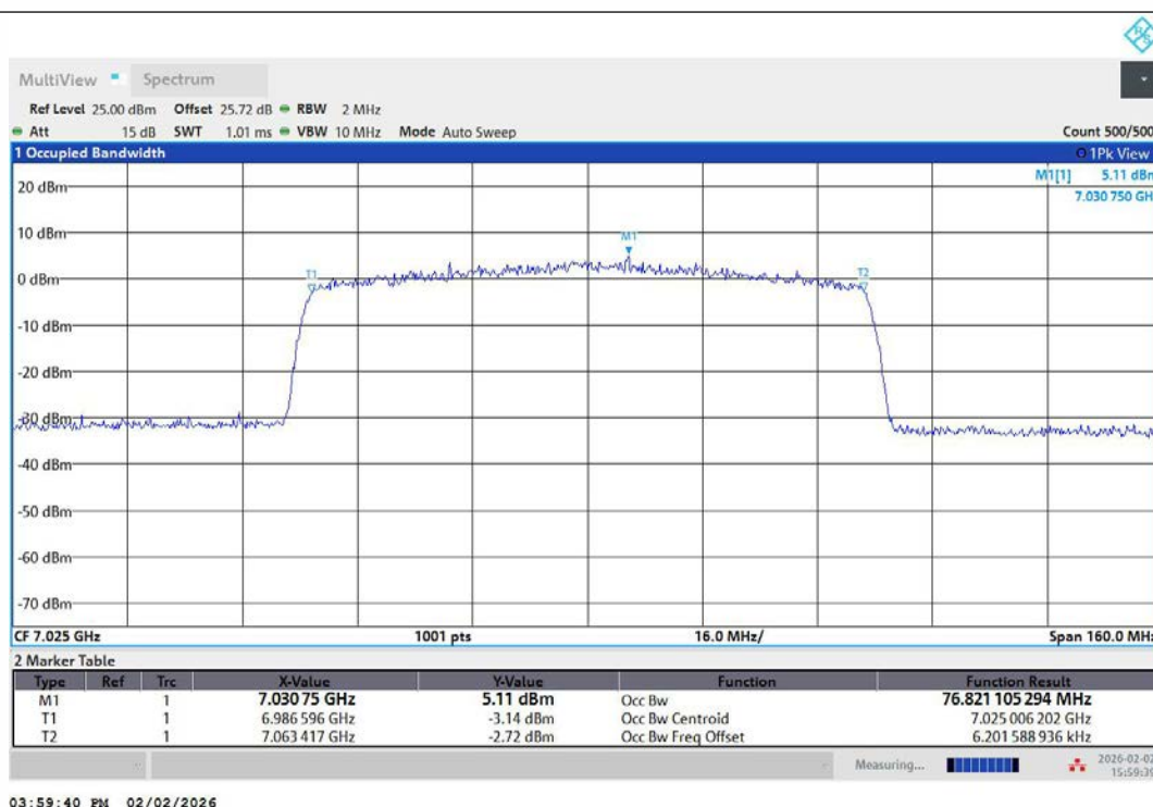
11AX80MIMO-Ant1-7025-PASS
