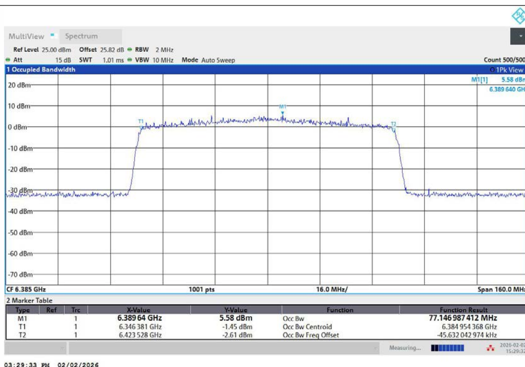
11AX80MIMO-Ant1-6385-PASS
