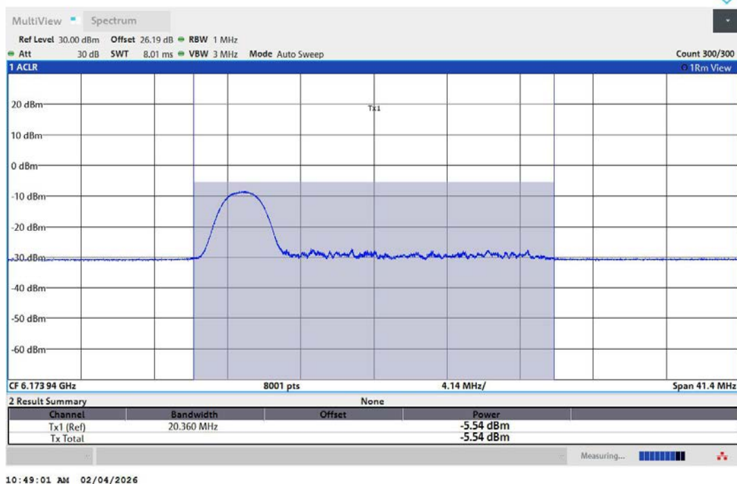
11AX20MIMO-Ant2-6175-26Tone-RU0-PASS
