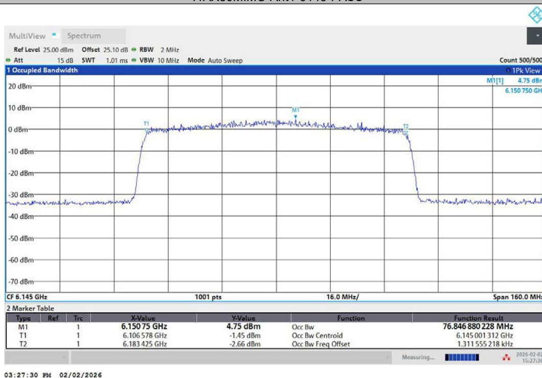
11AX80MIMO-Ant2-6145-PASS
