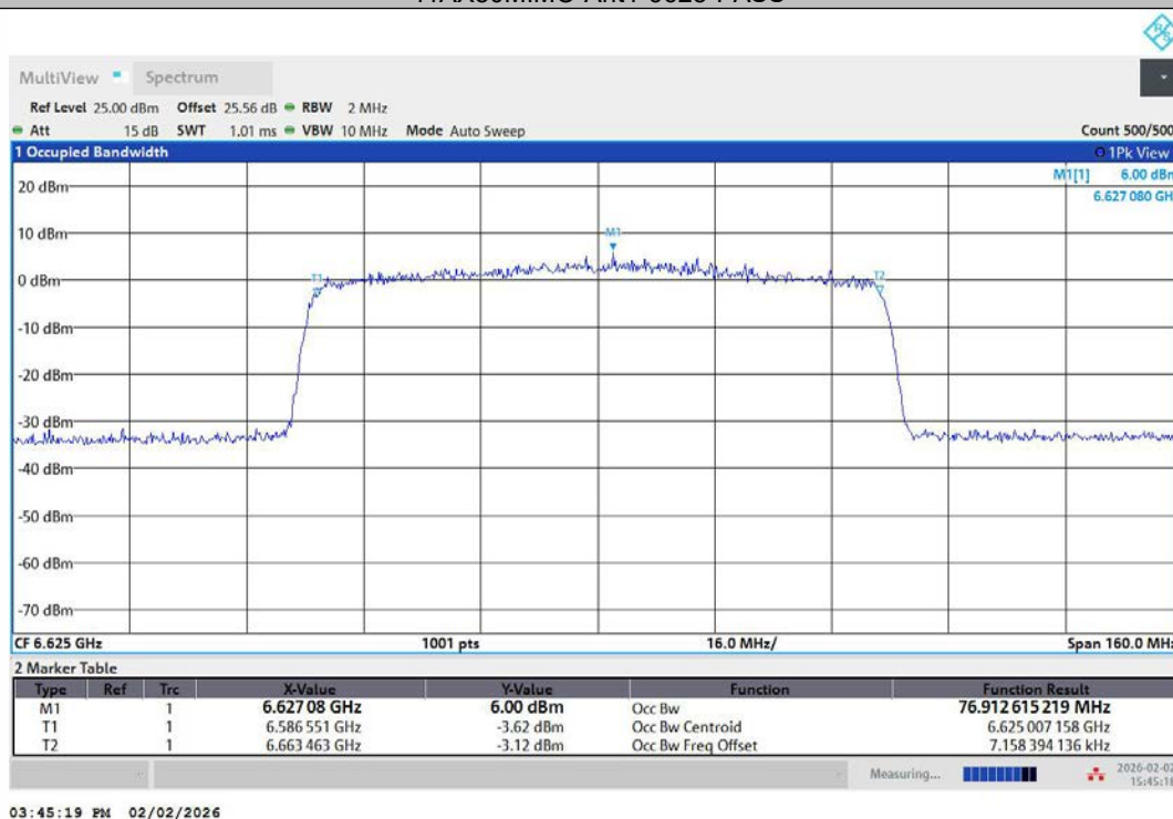
11AX80MIMO-Ant2-6625-PASS
