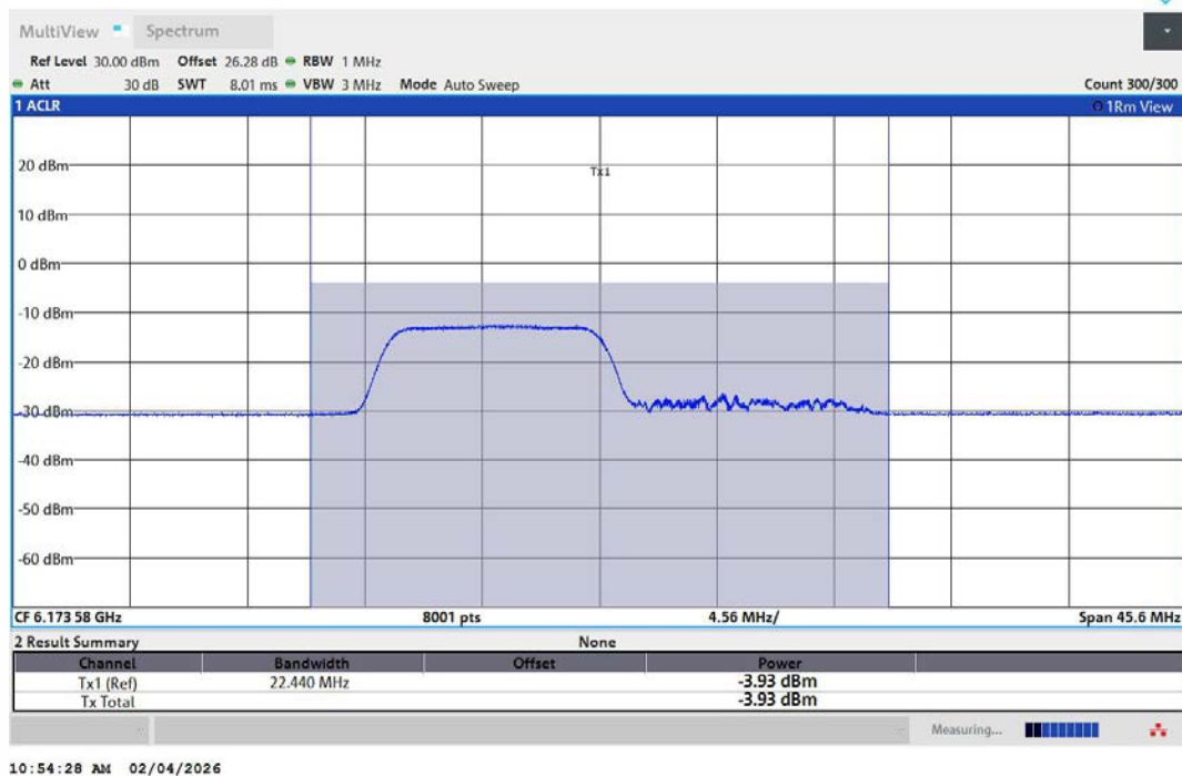
11AX20MIMO-Ant1-6175-106Tone-RU53-PASS
