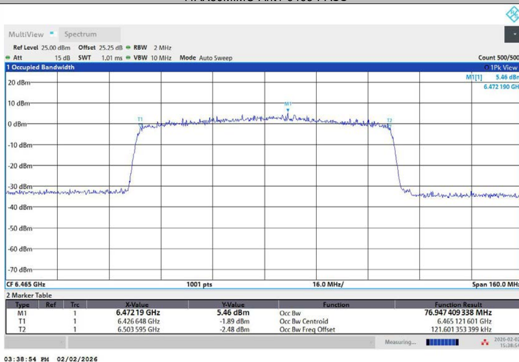
11AX80MIMO-Ant2-6465-PASS
