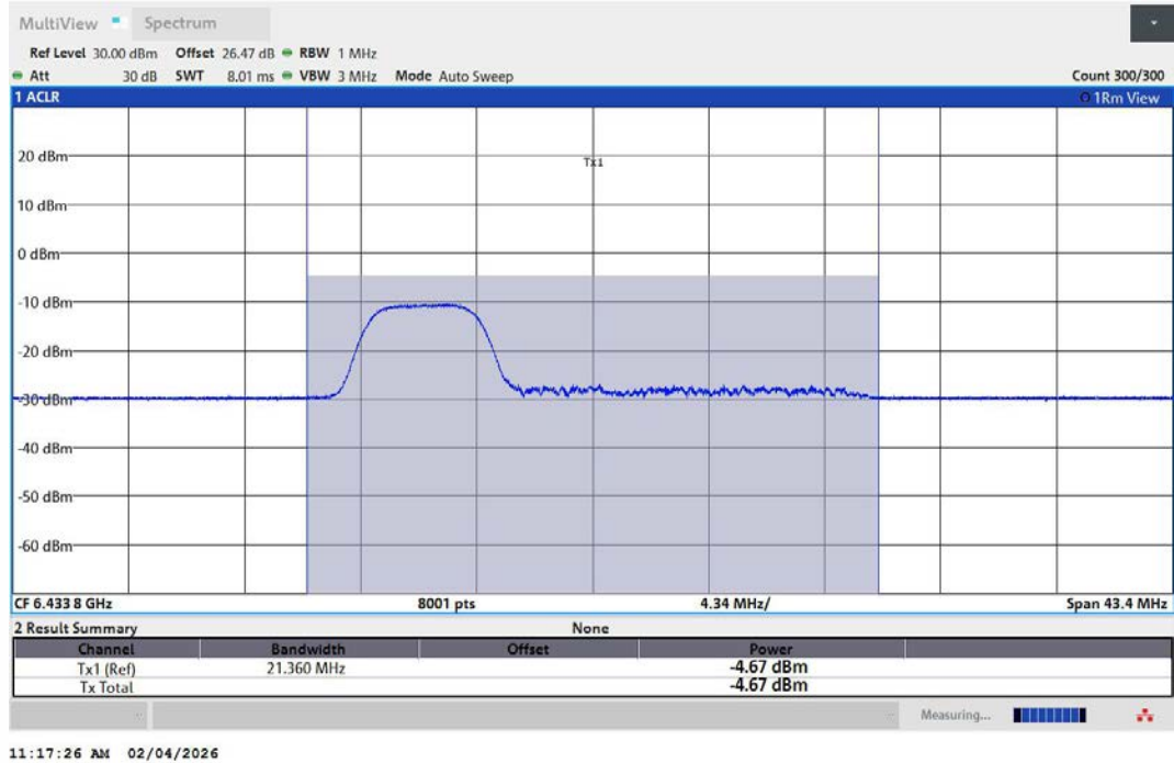
11AX20MIMO-Ant1-6435-52Tone-RU37-PASS
