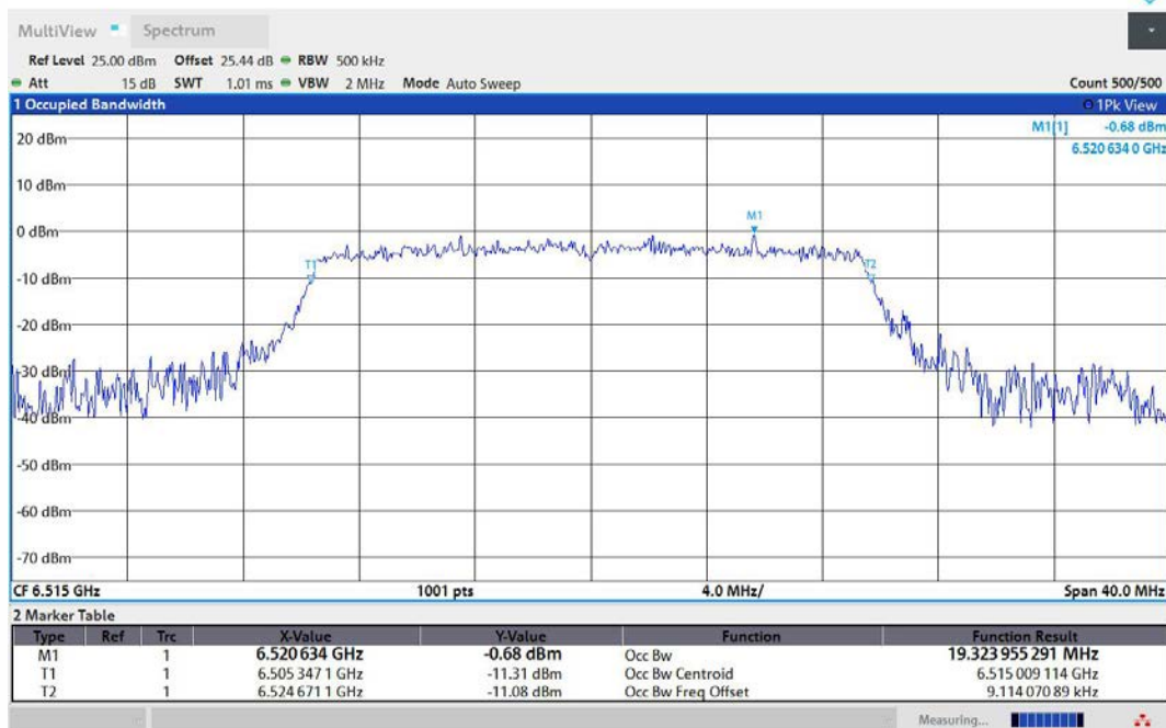
11AX20MIMO-Ant1-6515-PASS
