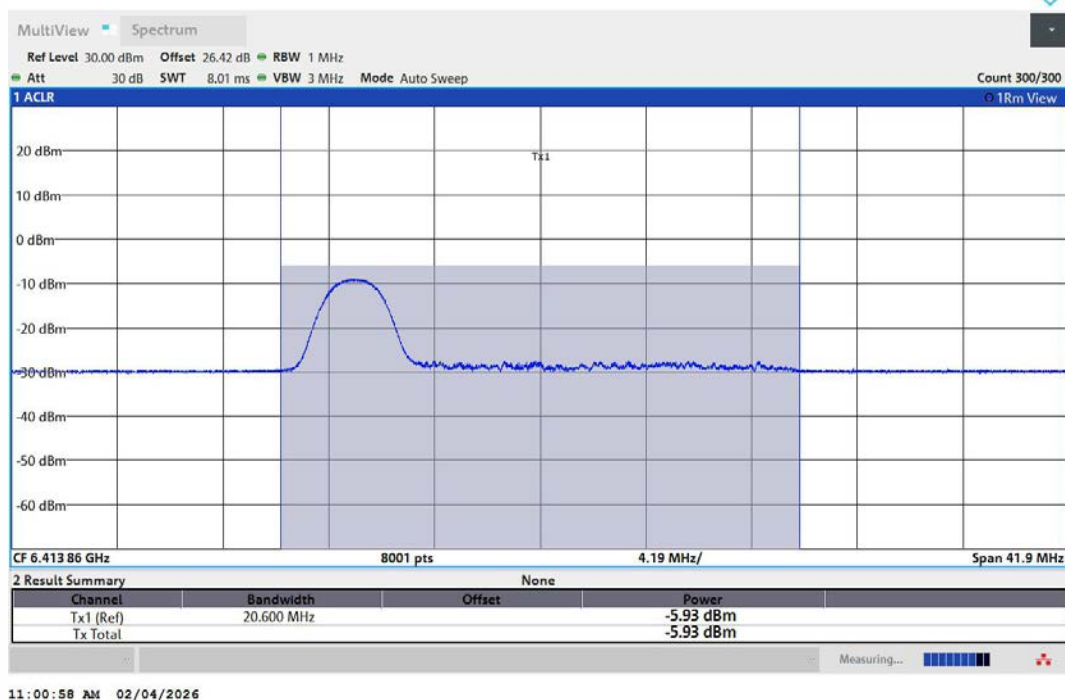
11AX20MIMO-Ant2-6415-26Tone-RU0-PASS
