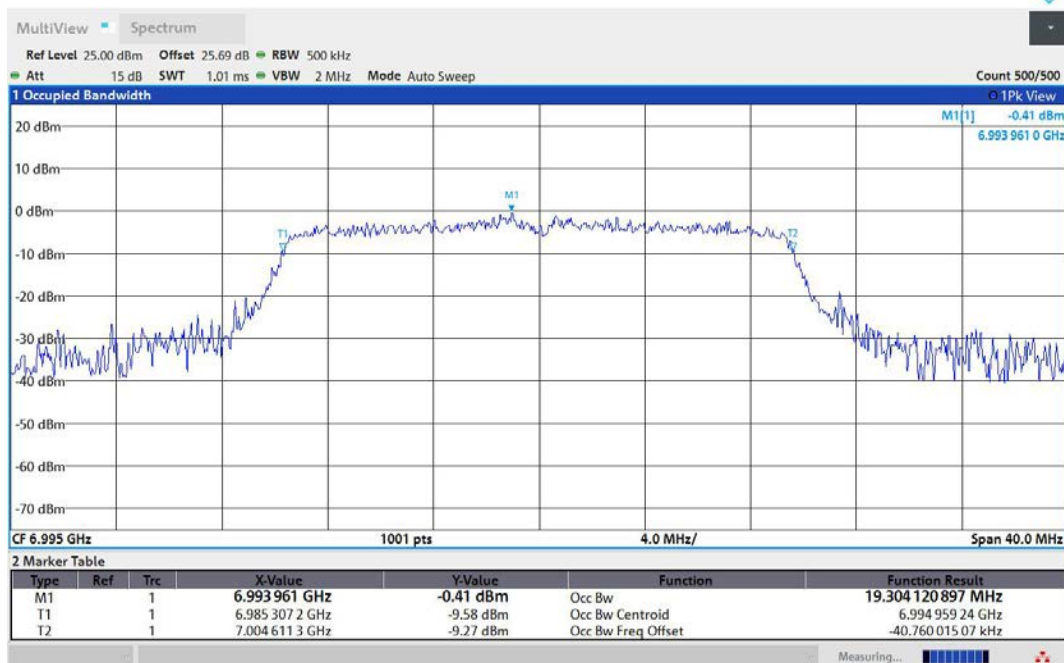
11AX20MIMO-Ant2-6995-PASS
