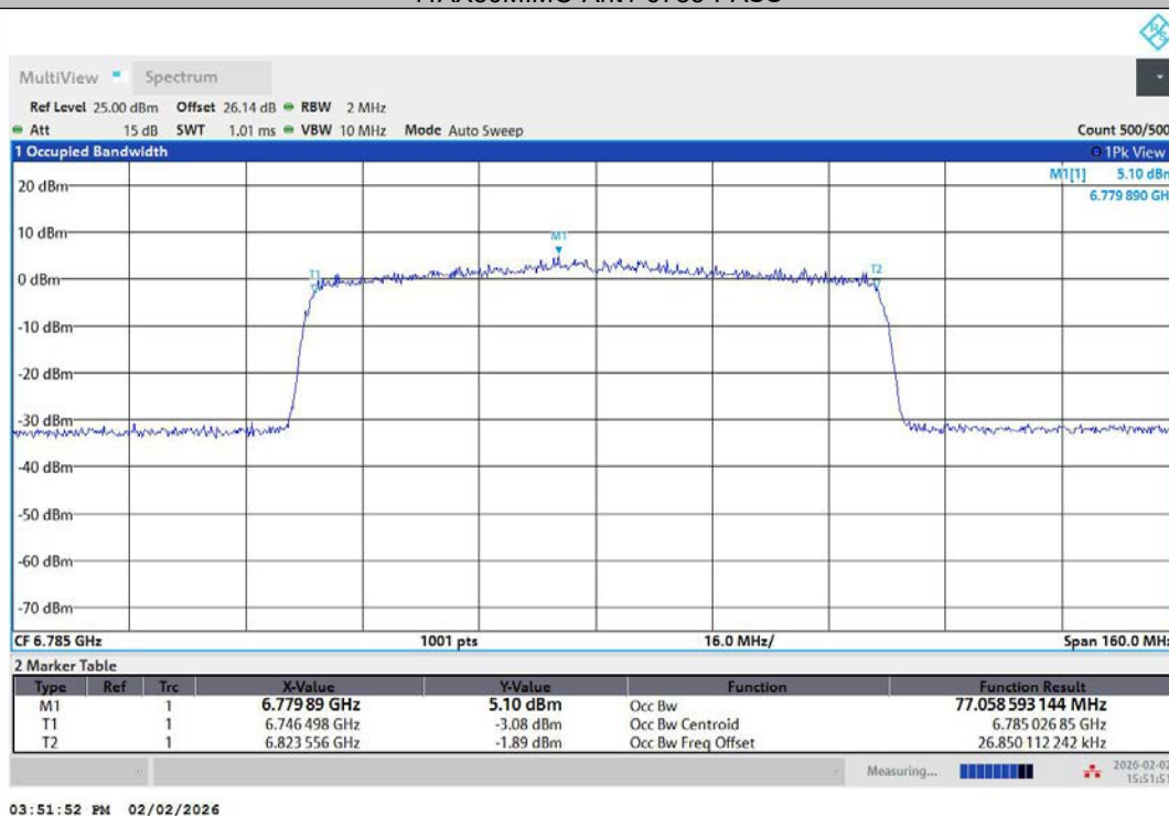
11AX80MIMO-Ant2-6785-PASS
