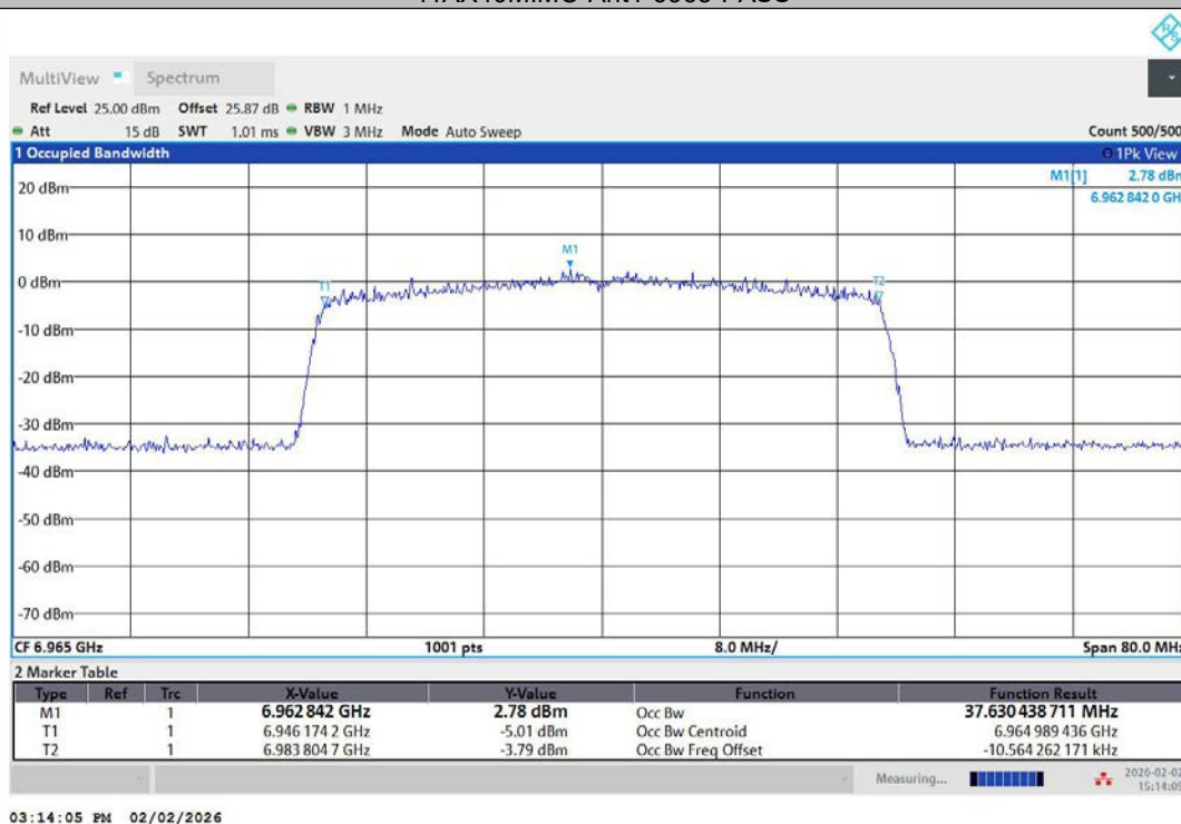
11AX40MIMO-Ant2-6965-PASS
