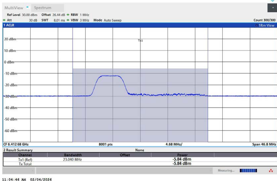
11AX20MIMO-Ant2-6415-52Tone-RU37-PASS
