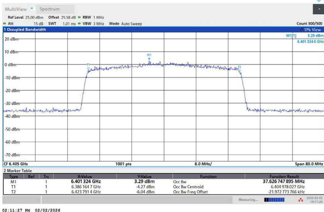
11AX40MIMO-Ant2-6405-PASS
