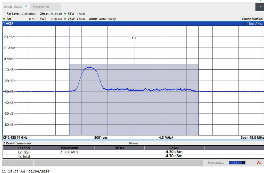
11AX20MIMO-Ant1-6435-26Tone-RU0-PASS
