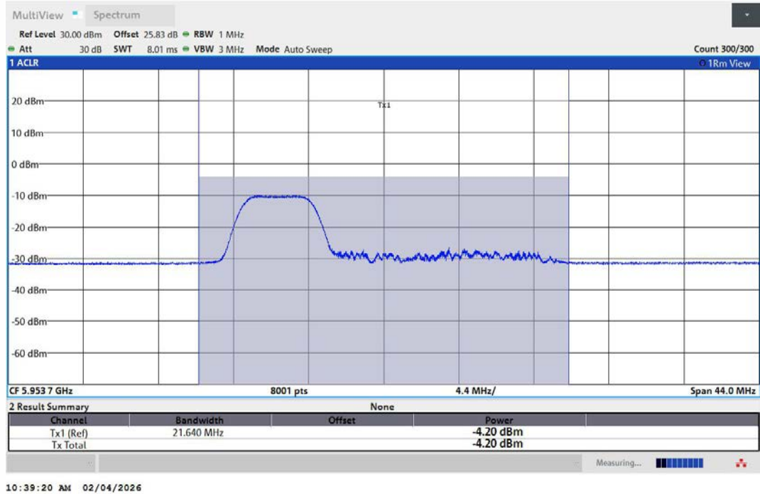
11AX20MIMO-Ant1-5955-52Tone-RU37-PASS
