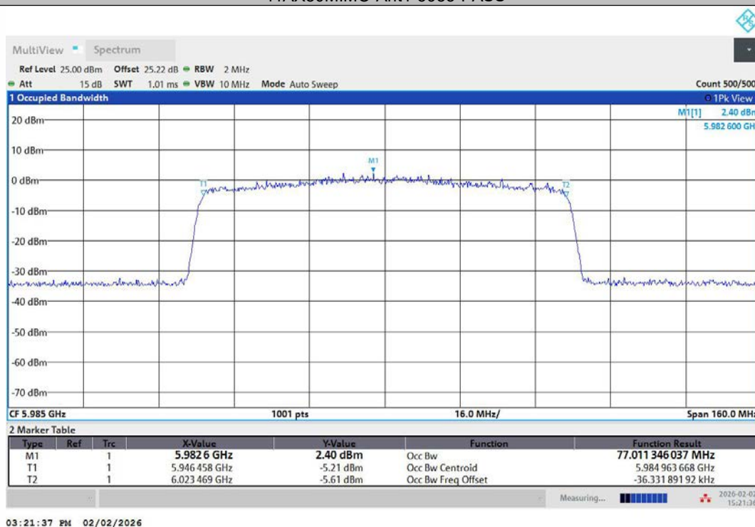
11AX80MIMO-Ant2-5985-PASS
