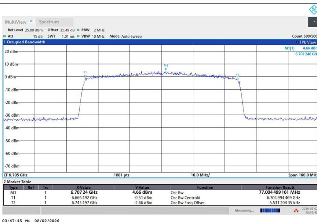
11AX80MIMO-Ant1-6705-PASS
