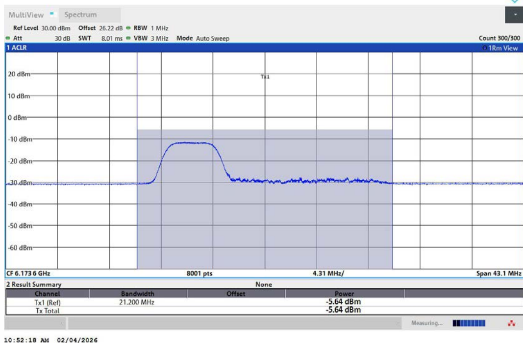
11AX20MIMO-Ant2-6175-52Tone-RU37-PASS
