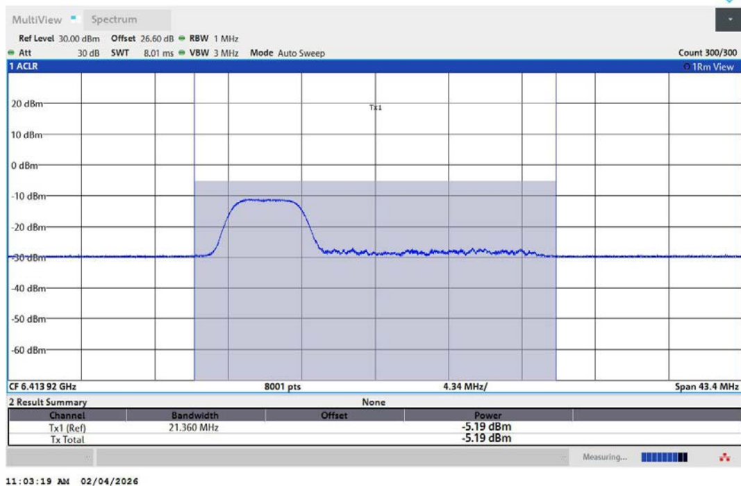
11AX20MIMO-Ant1-6415-52Tone-RU37-PASS
