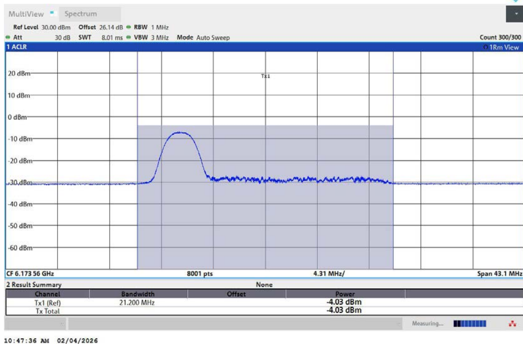
11AX20MIMO-Ant1-6175-26Tone-RU0-PASS
