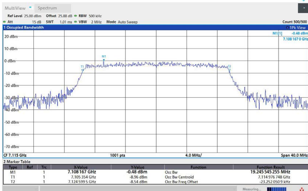
11AX20MIMO-Ant2-7115-PASS
