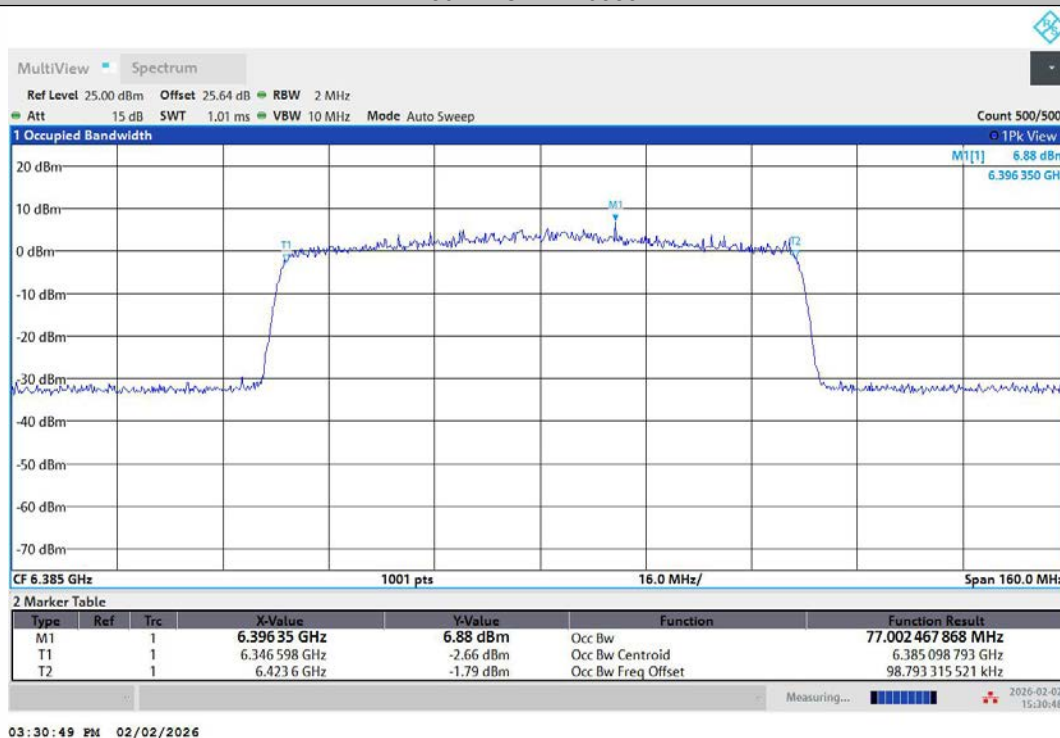
11AX80MIMO-Ant2-6385-PASS
