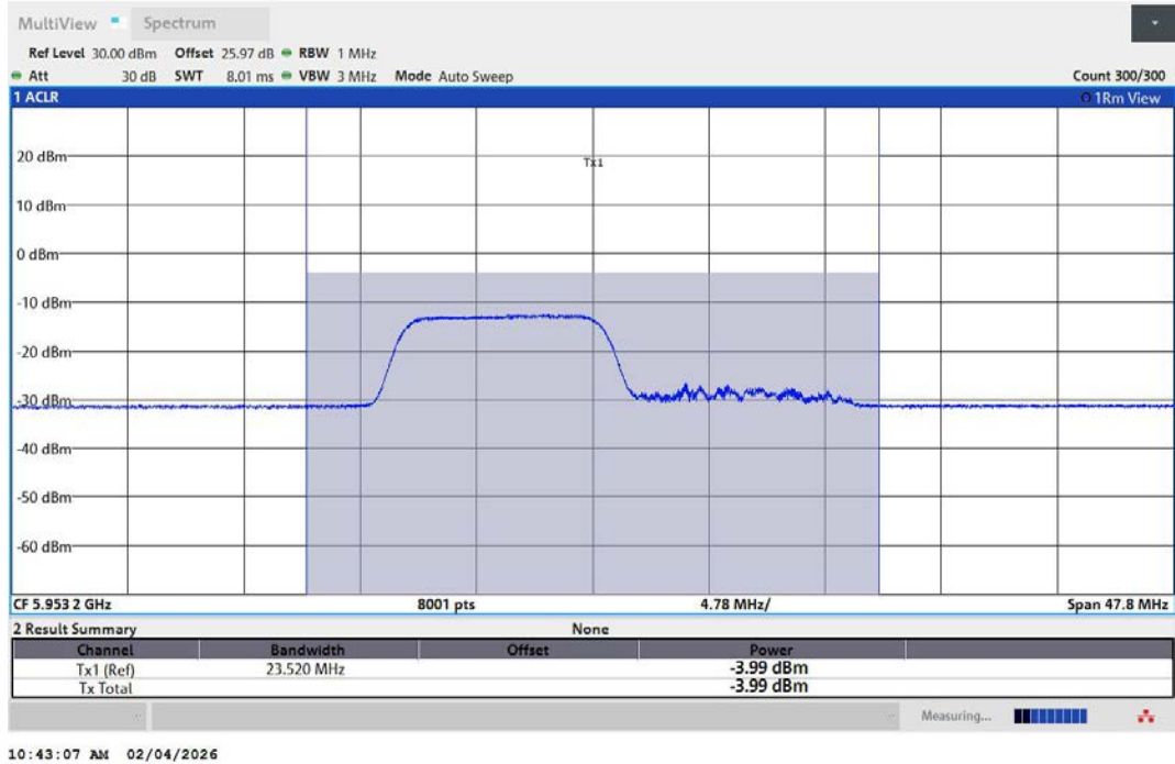
11AX20MIMO-Ant1-5955-106Tone-RU53-PASS
