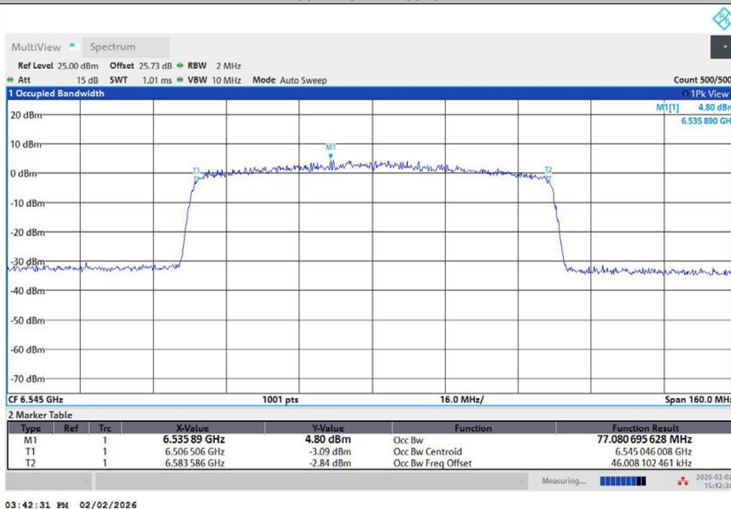
11AX80MIMO-Ant2-6545-PASS
