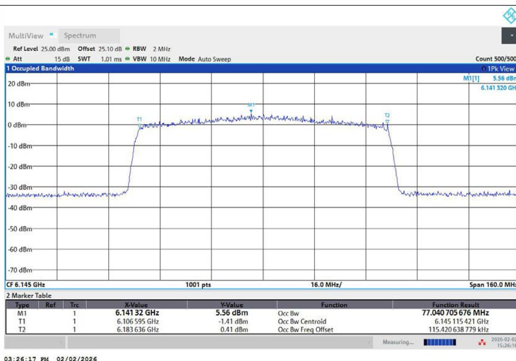
11AX80MIMO-Ant1-6145-PASS
