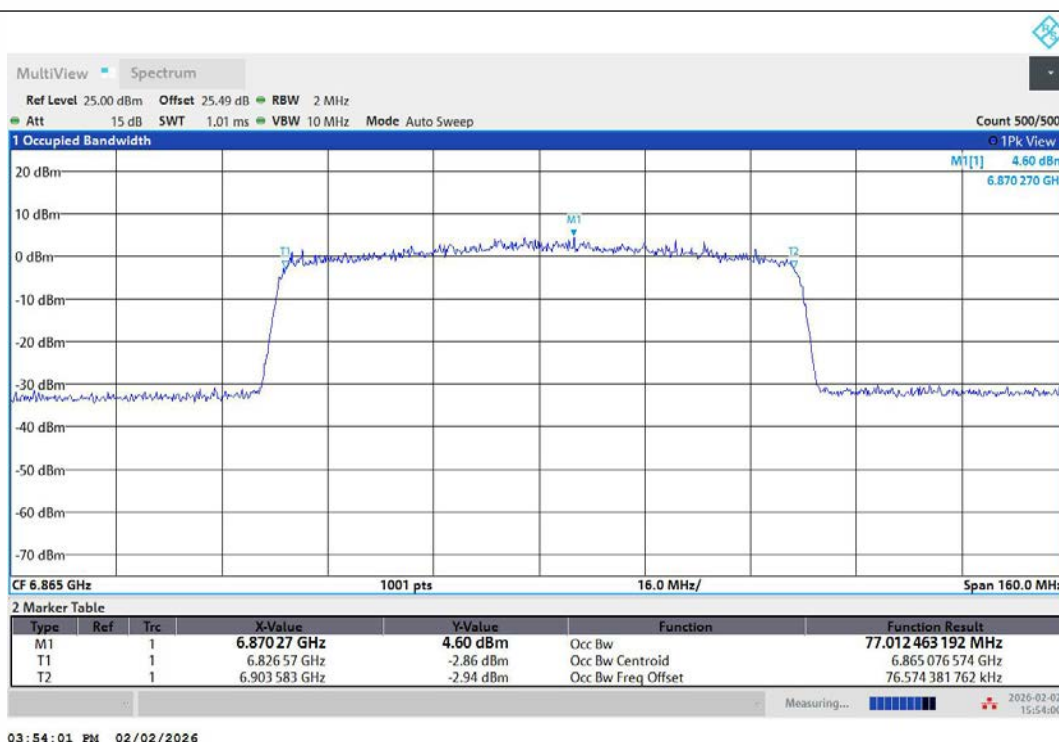
11AX80MIMO-Ant1-6865-PASS
