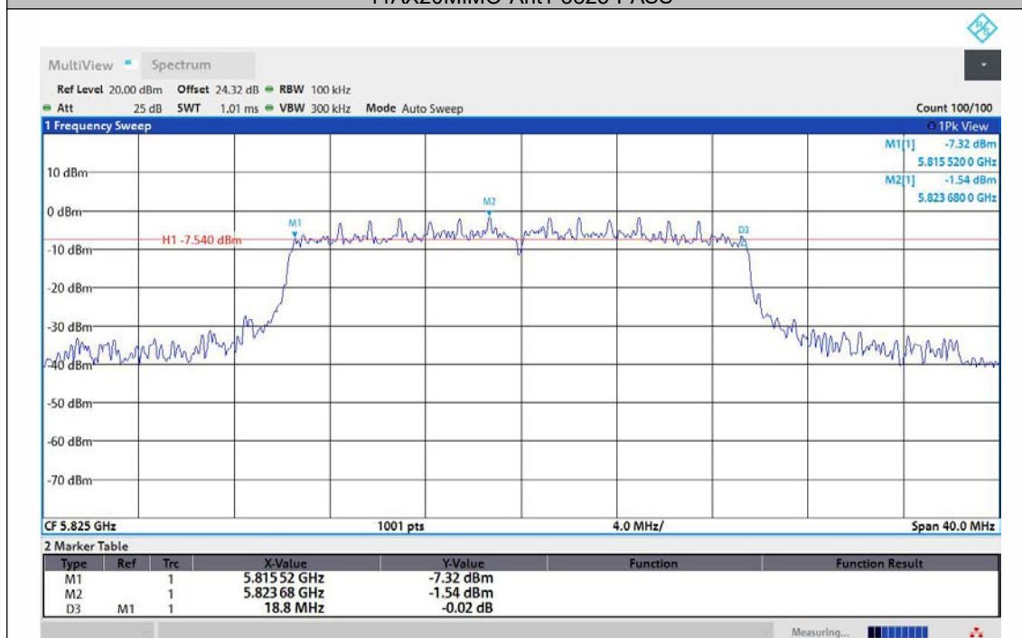
11AX20MIMO-Ant2-5825-PASS
