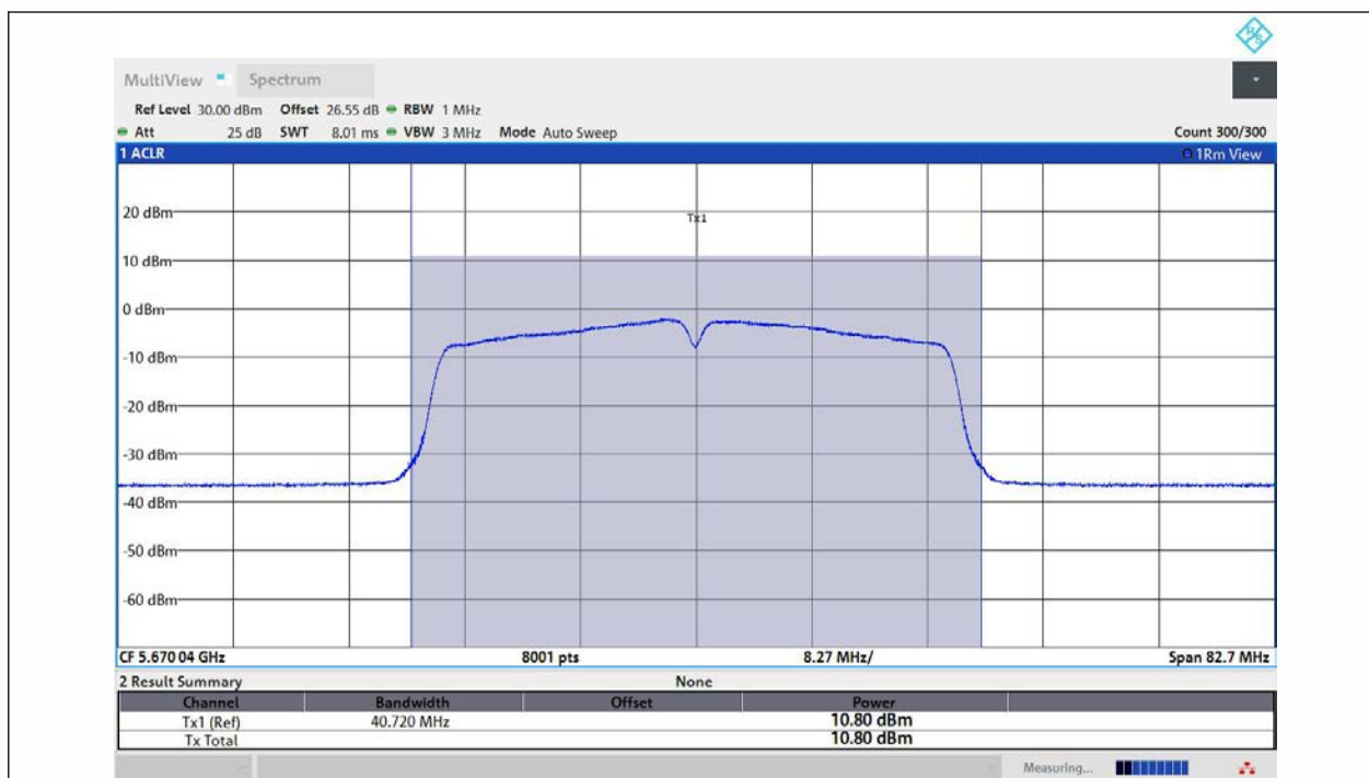
11N40MIMO-Ant1-5670-PASS
