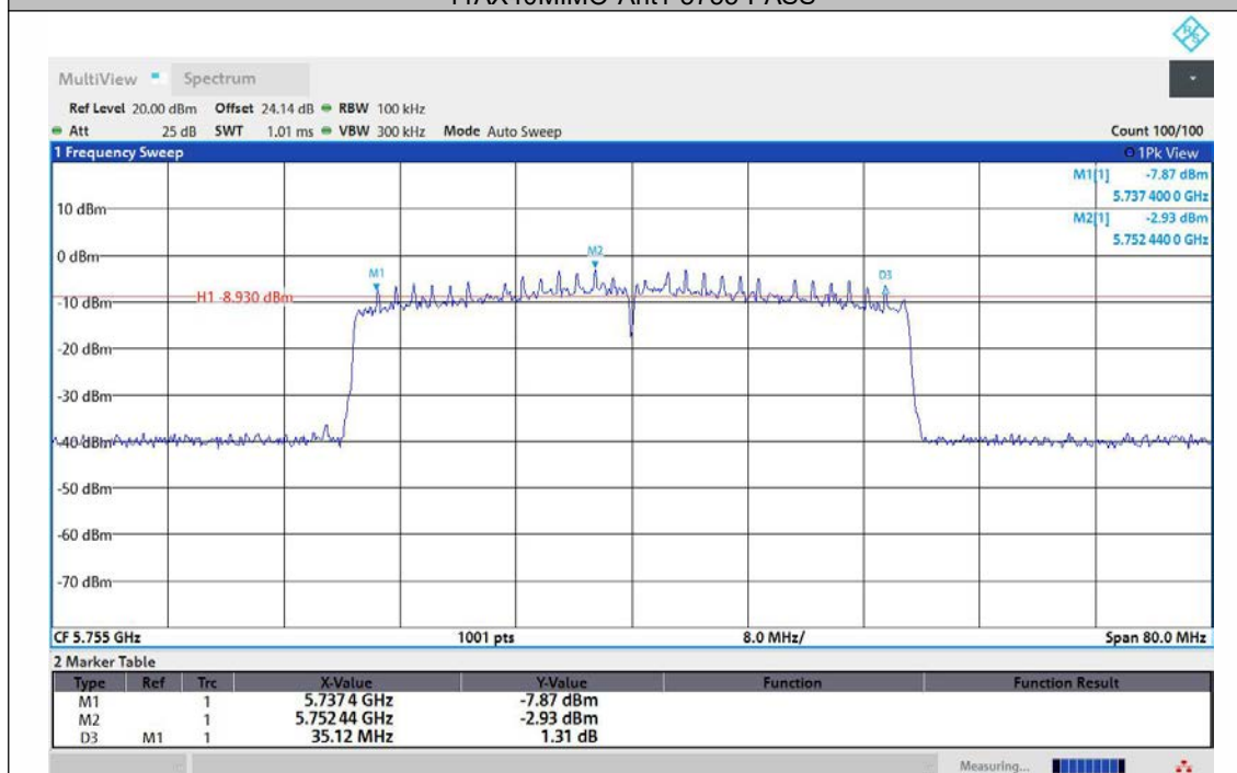
11AX40MIMO-Ant2-5755-PASS
