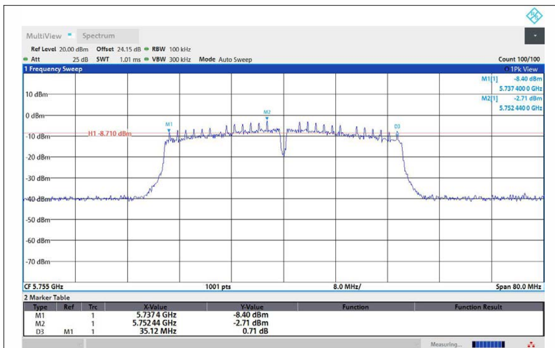
11AC40MIMO-Ant1-5755-PASS
