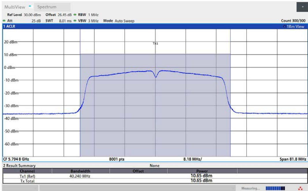
11N40MIMO-Ant2-5795-PASS
