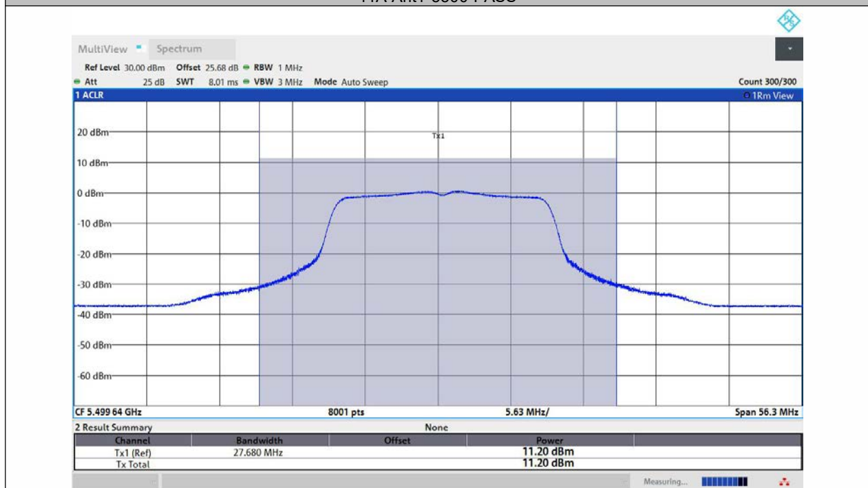
11A-Ant2-5500-PASS
