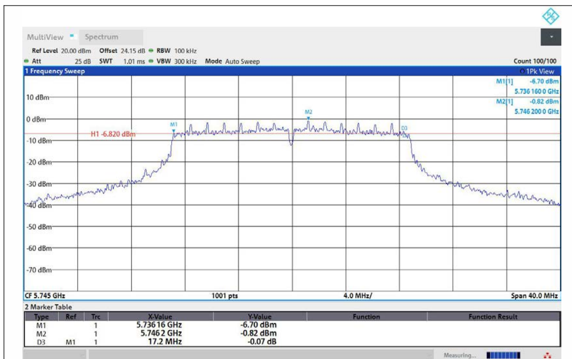
11AC20MIMO-Ant1-5745-PASS
