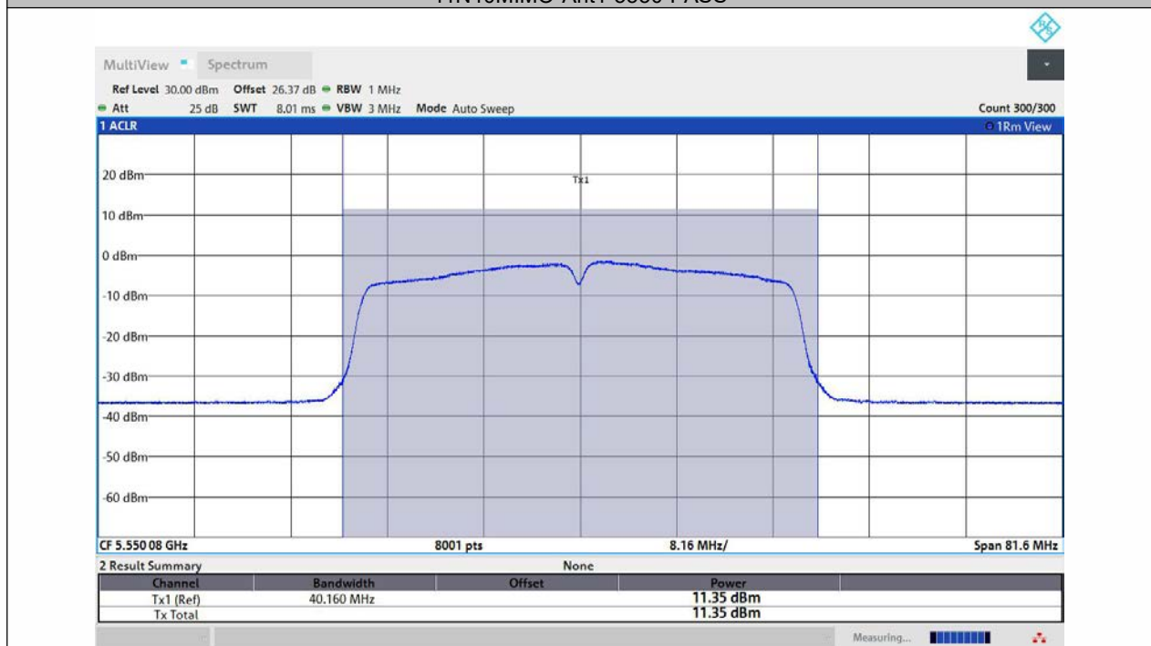
11N40MIMO-Ant2-5550-PASS
