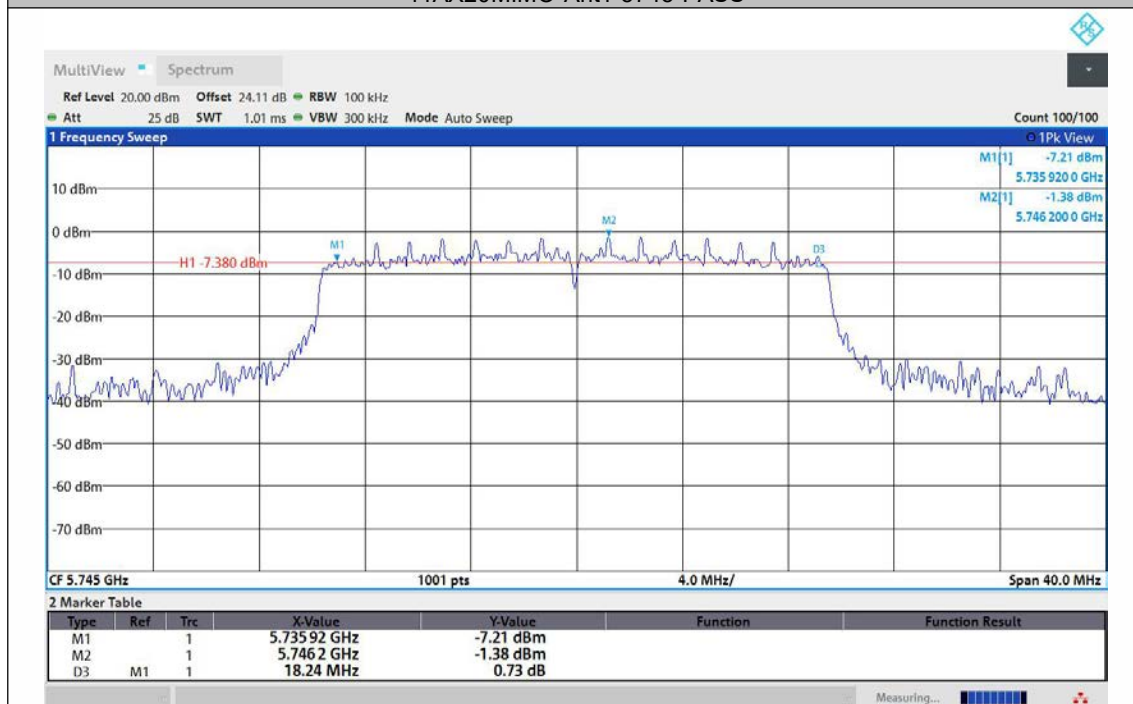
11AX20MIMO-Ant2-5745-PASS
