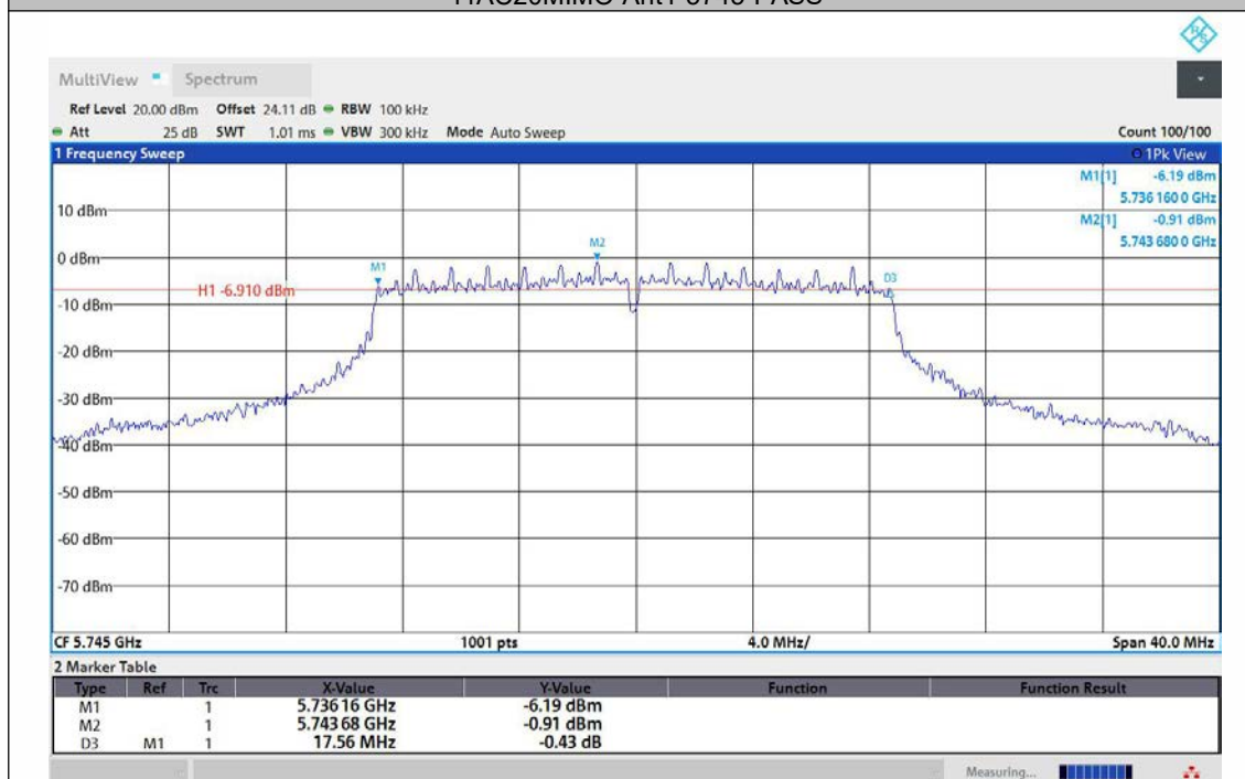
11AC20MIMO-Ant2-5745-PASS
