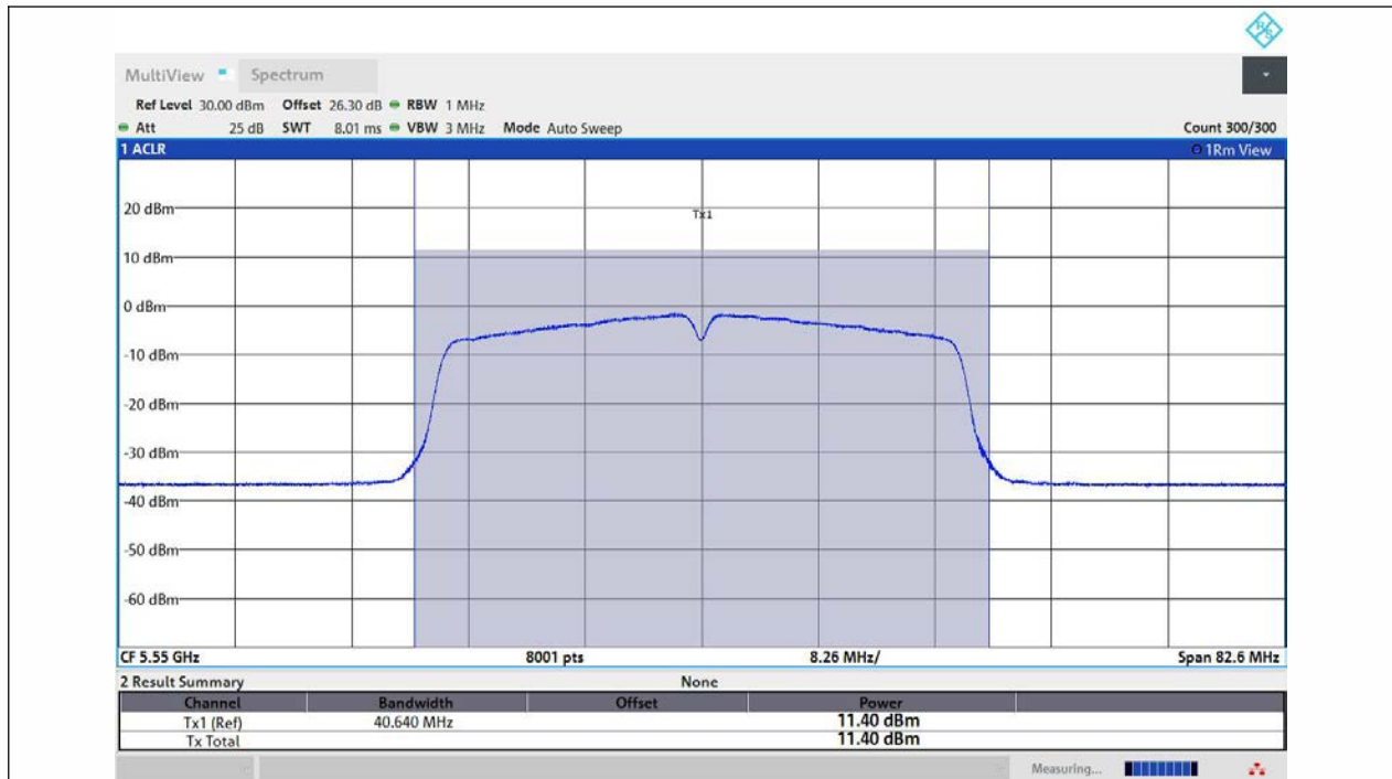
11N40MIMO-Ant1-5550-PASS
