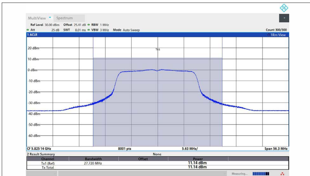
11A-Ant1-5825-PASS
