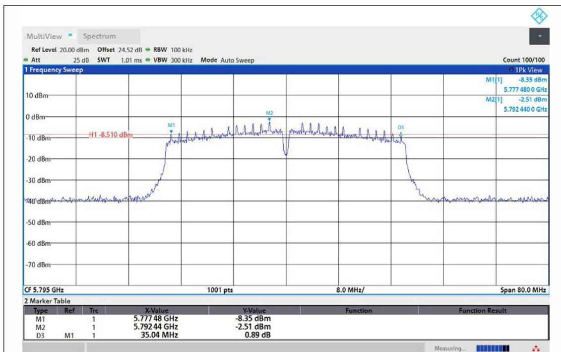
11AC40MIMO-Ant1-5795-PASS
