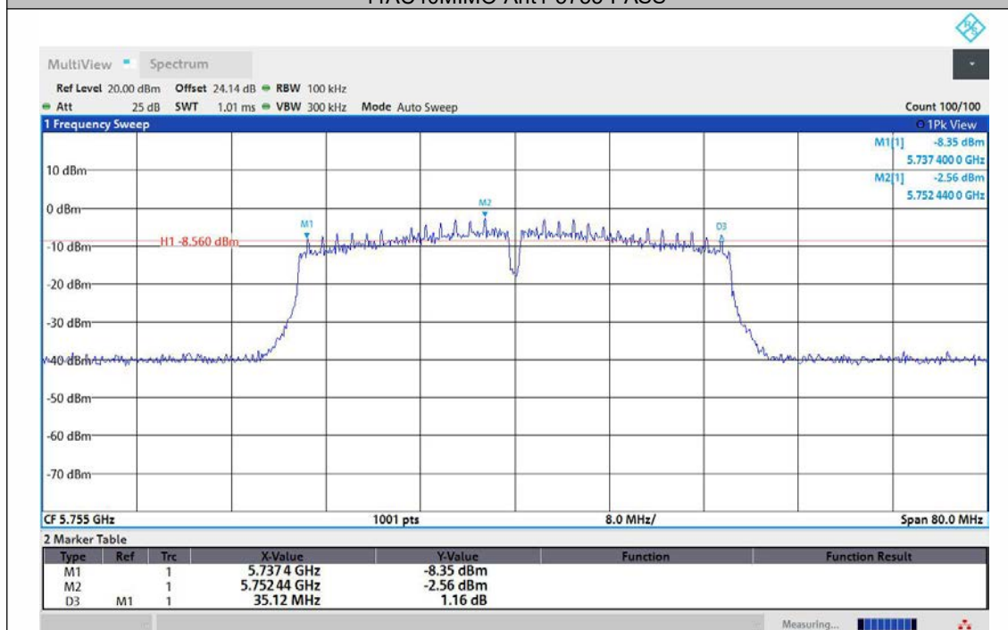
11AC40MIMO-Ant2-5755-PASS
