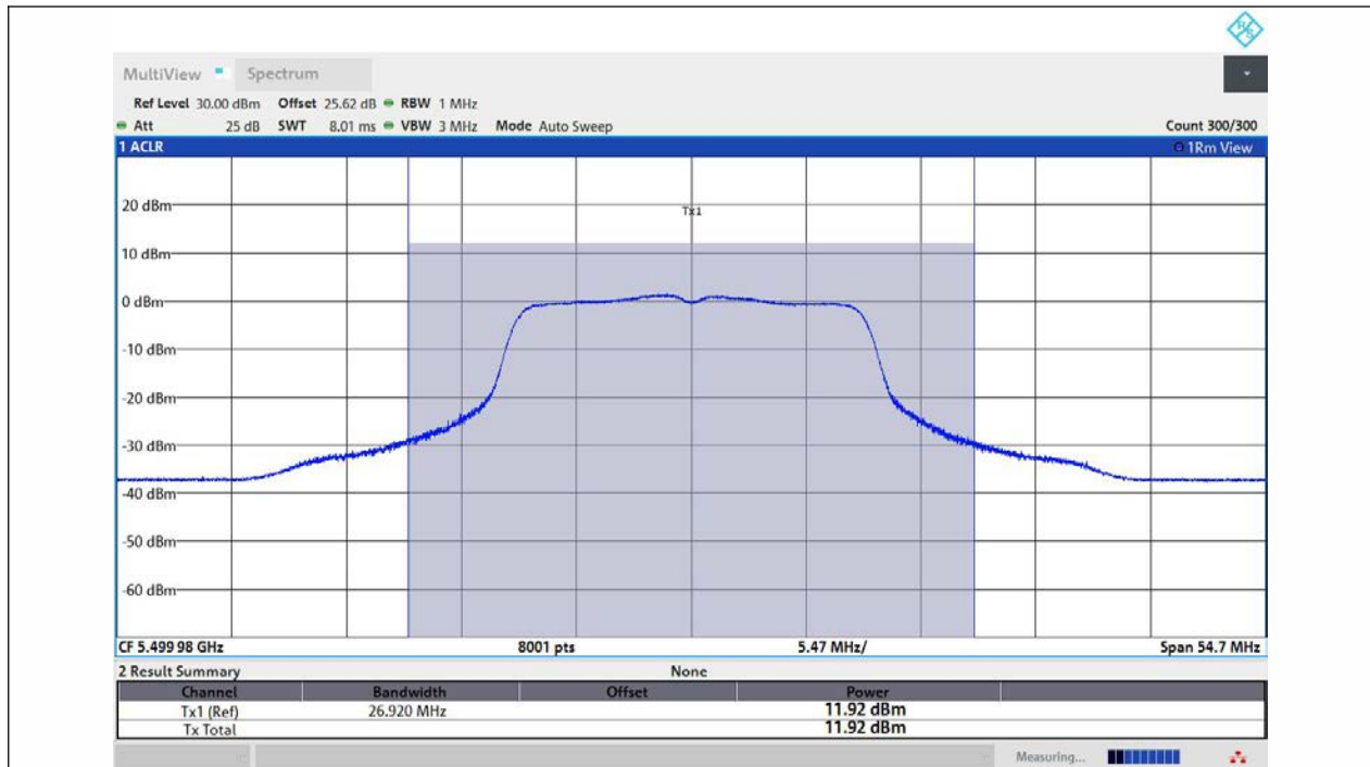
11A-Ant1-5500-PASS
