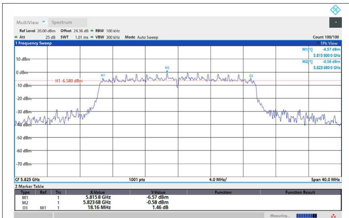
11AX20MIMO-Ant1-5825-PASS
