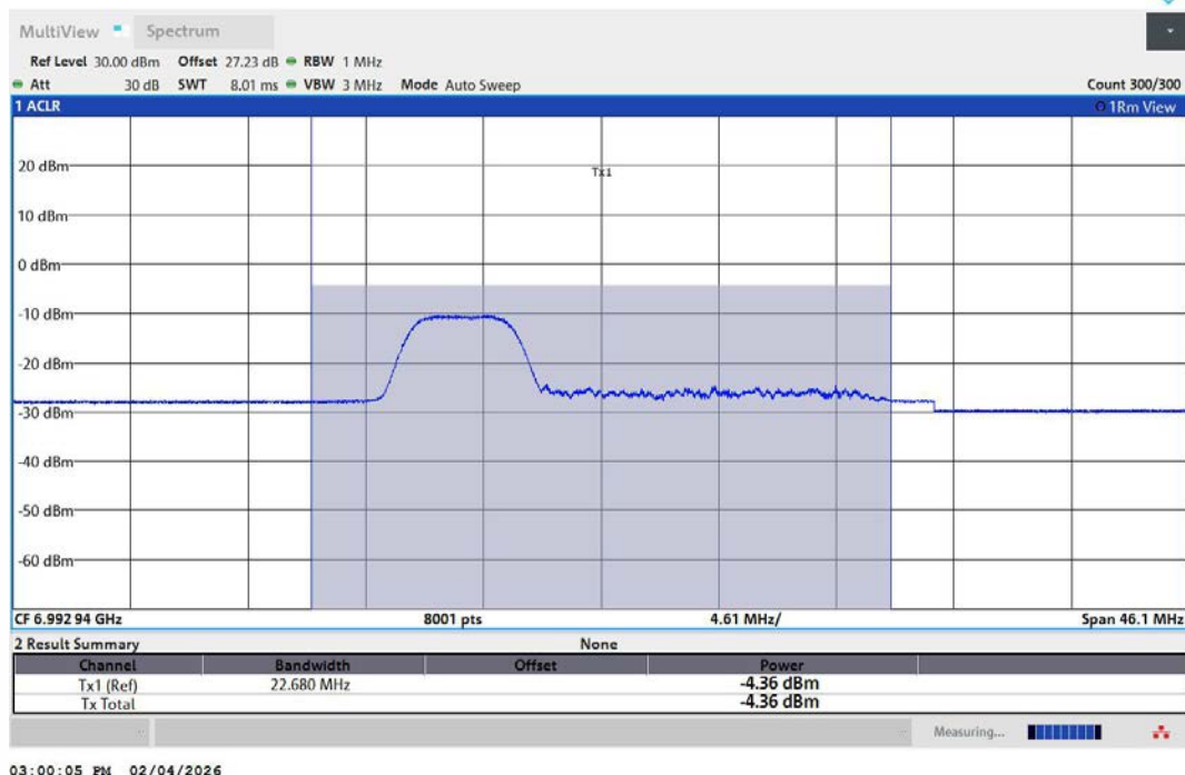
11AX20MIMO-Ant1-6995-52Tone-RU37-PASS
