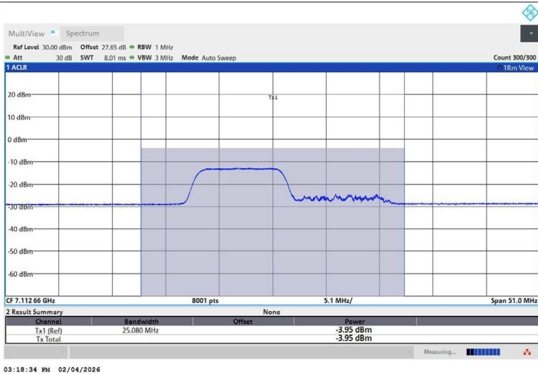
11AX20MIMO-Ant1-7115-106Tone-RU53-PASS
