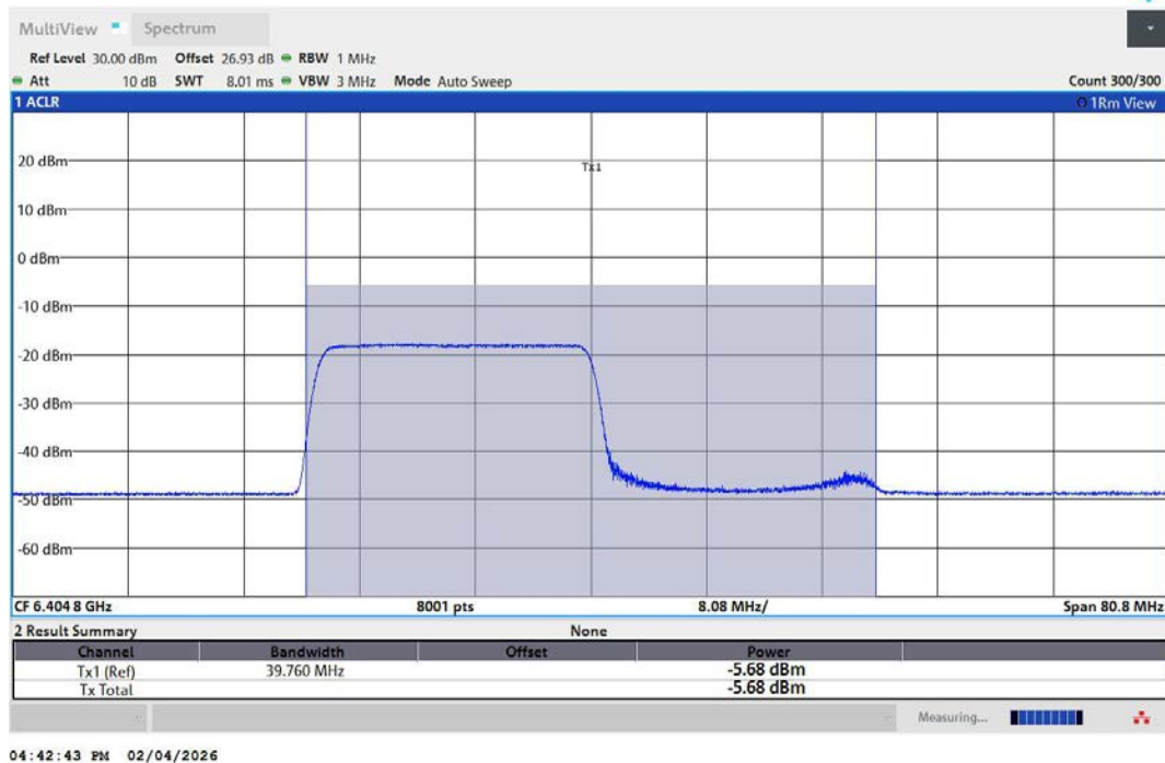
11AX40MIMO-Ant1-6405-242Tone-RU61-PASS
