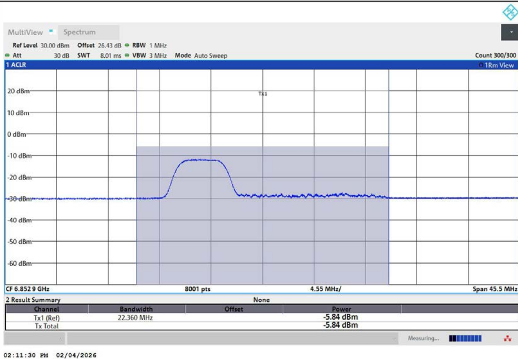
11AX20MIMO-Ant2-6855-52Tone-RU37-PASS
