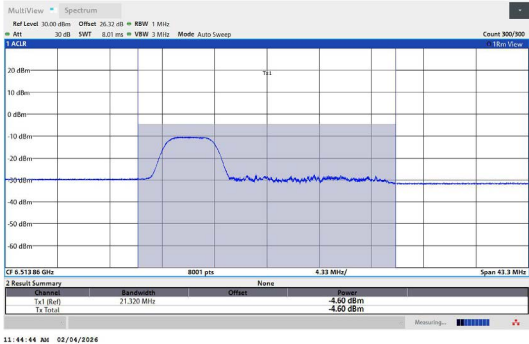
11AX20MIMO-Ant1-6515-52Tone-RU37-PASS
