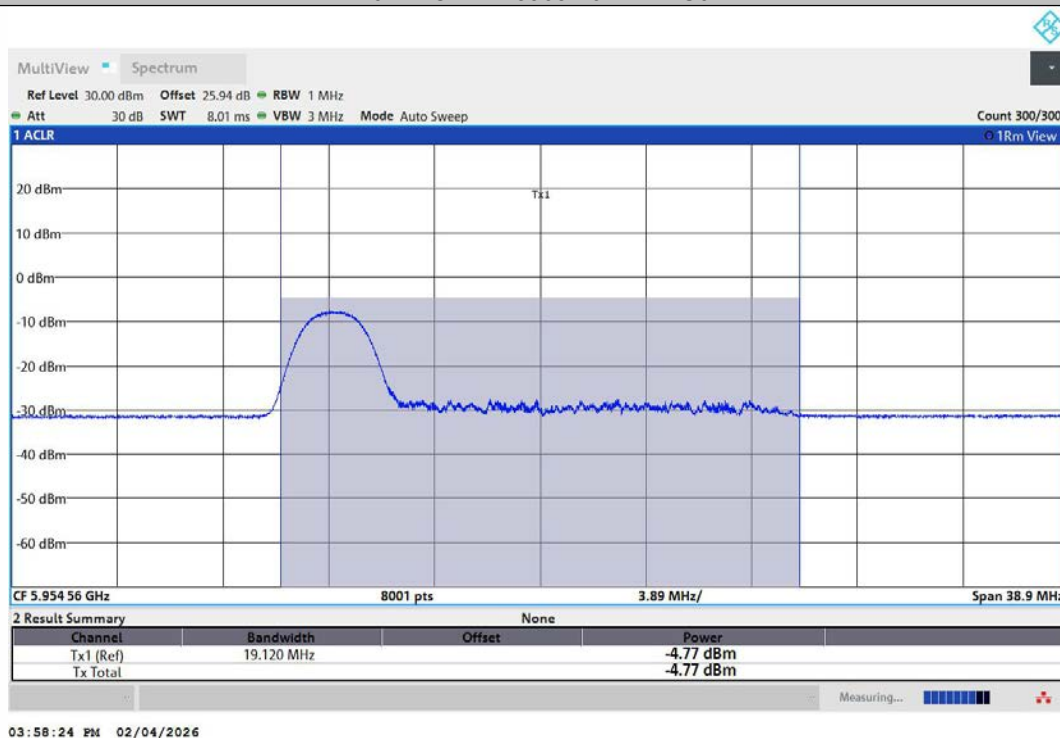
11AX40MIMO-Ant2-5965-26Tone-RU0-PASS
