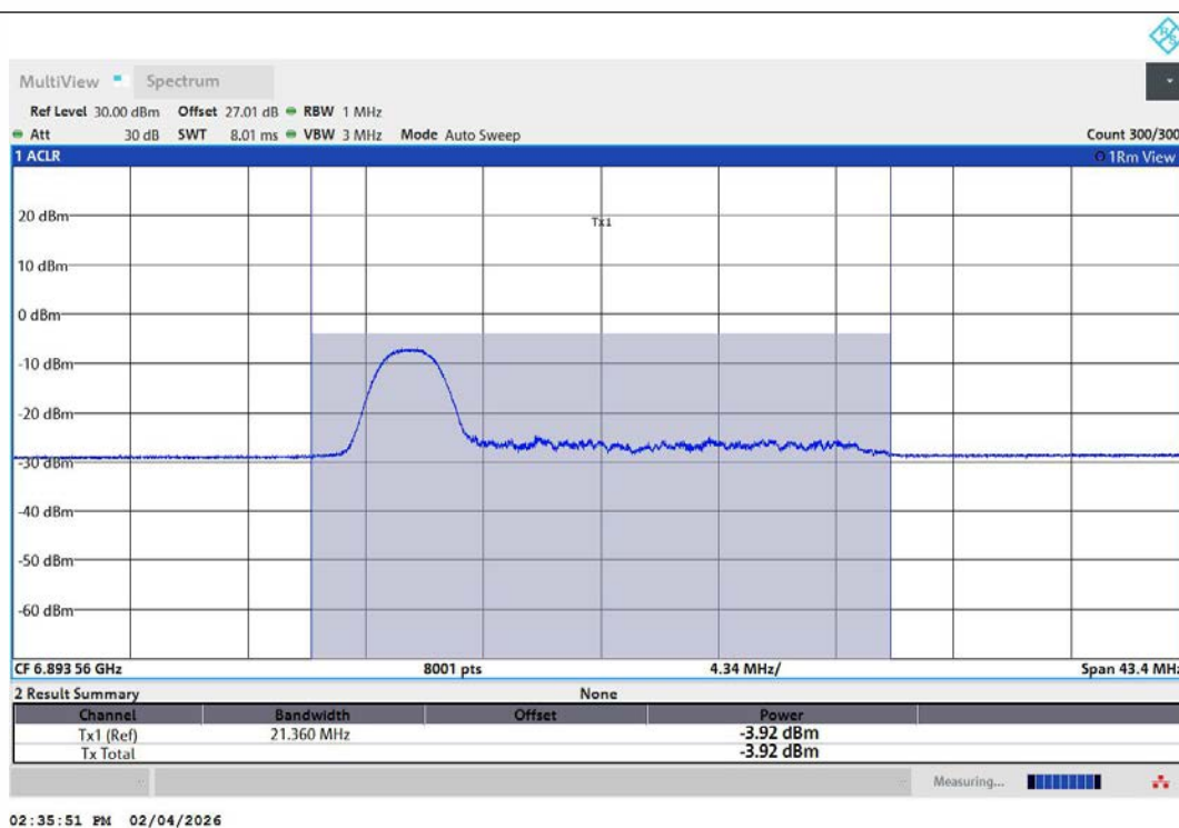
11AX20MIMO-Ant1-6895-26Tone-RU0-PASS
