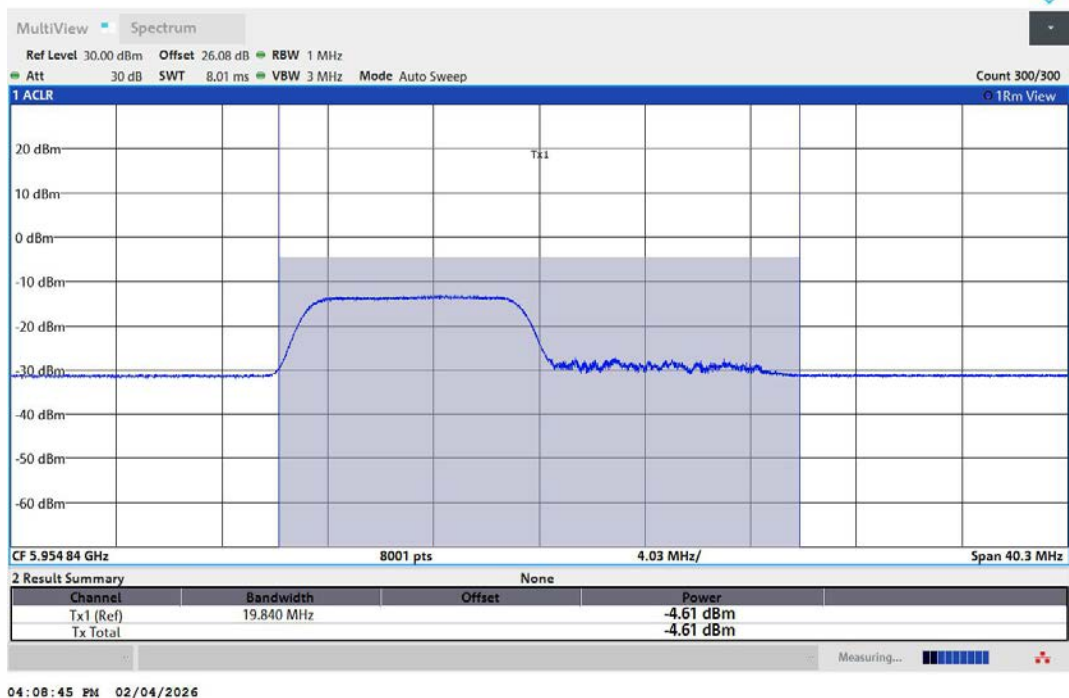
11AX40MIMO-Ant2-5965-106Tone-RU53-PASS
