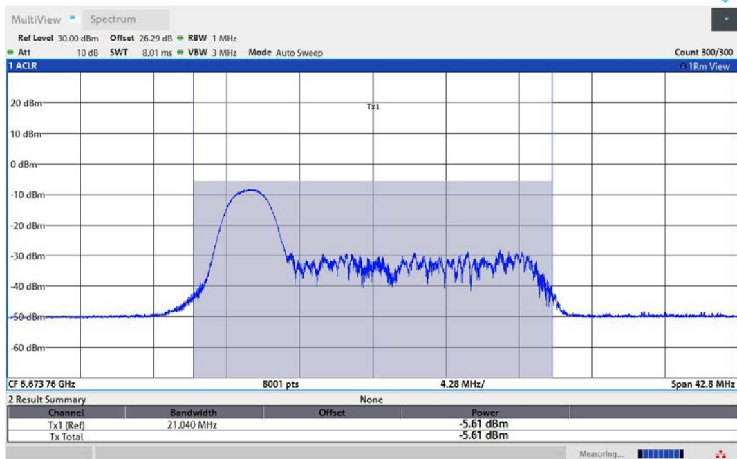
11AX40MIMO-Ant1-6685-26Tone-RU0-PASS
