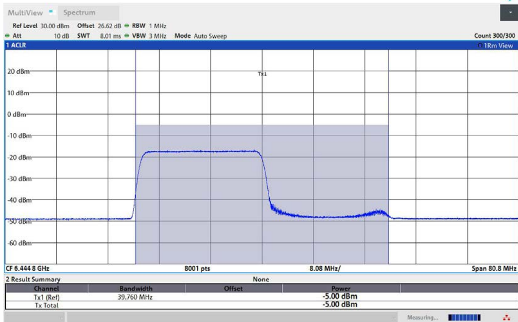
11AX40MIMO-Ant2-6445-242Tone-RU61-PASS
