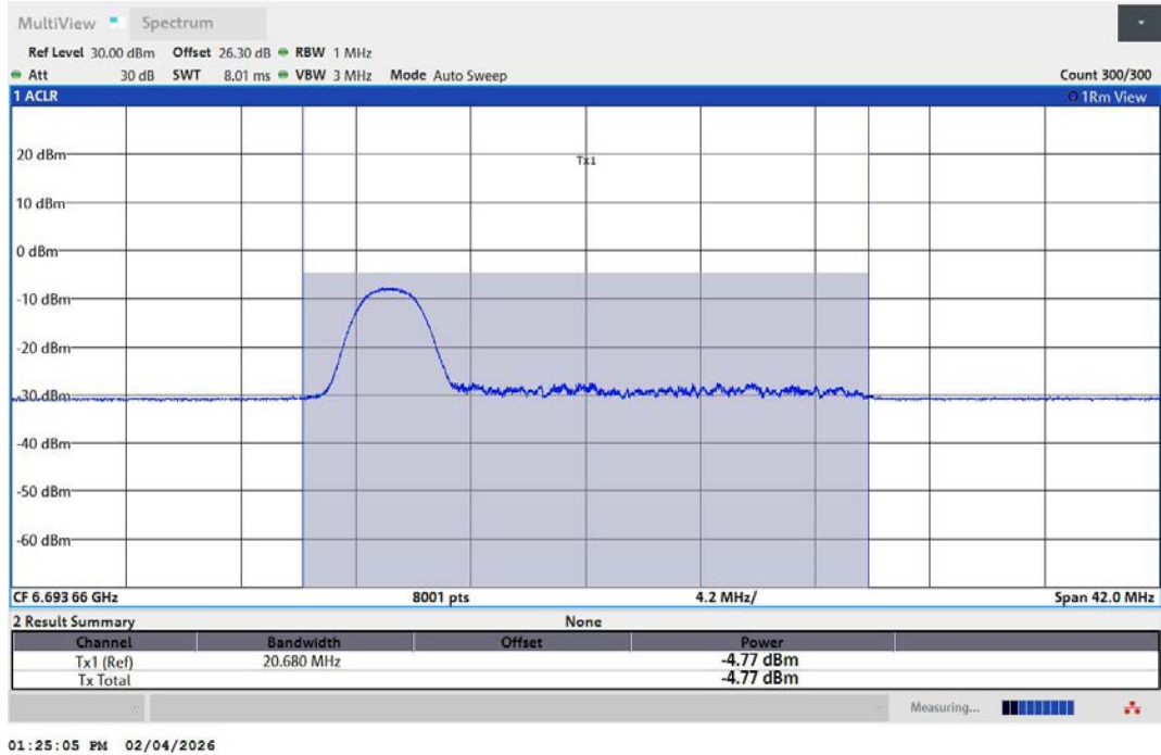
11AX20MIMO-Ant1-6695-26Tone-RU0-PASS
