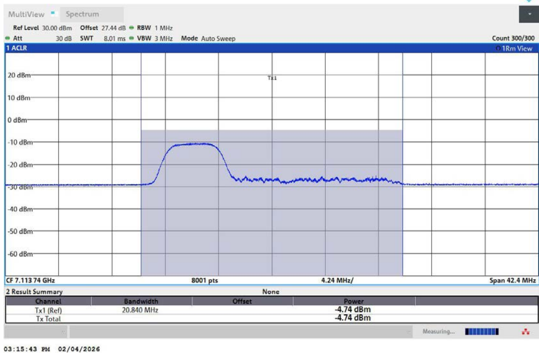
11AX20MIMO-Ant2-7115-52Tone-RU37-PASS
