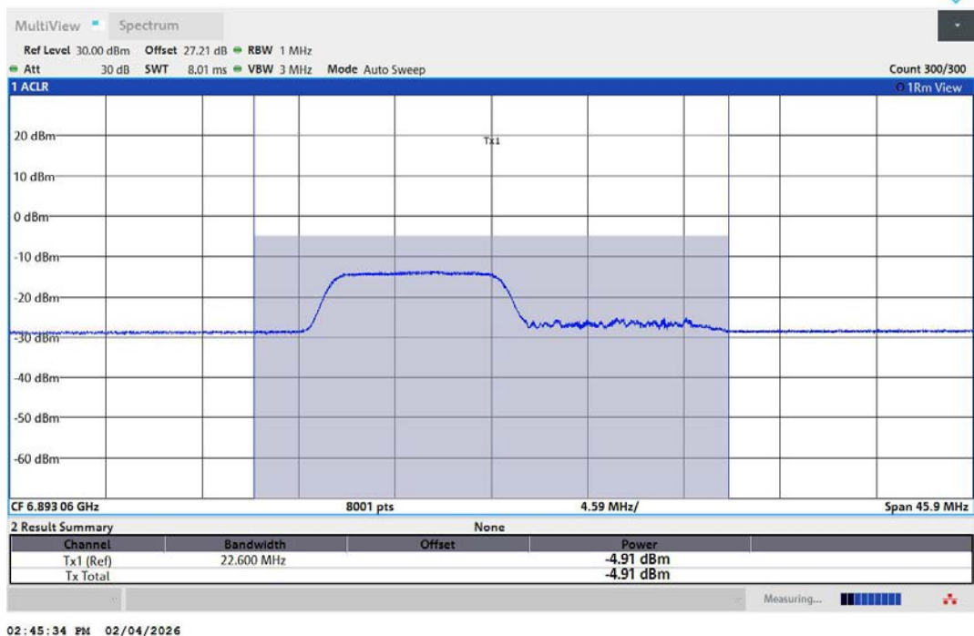
11AX20MIMO-Ant2-6895-106Tone-RU53-PASS
