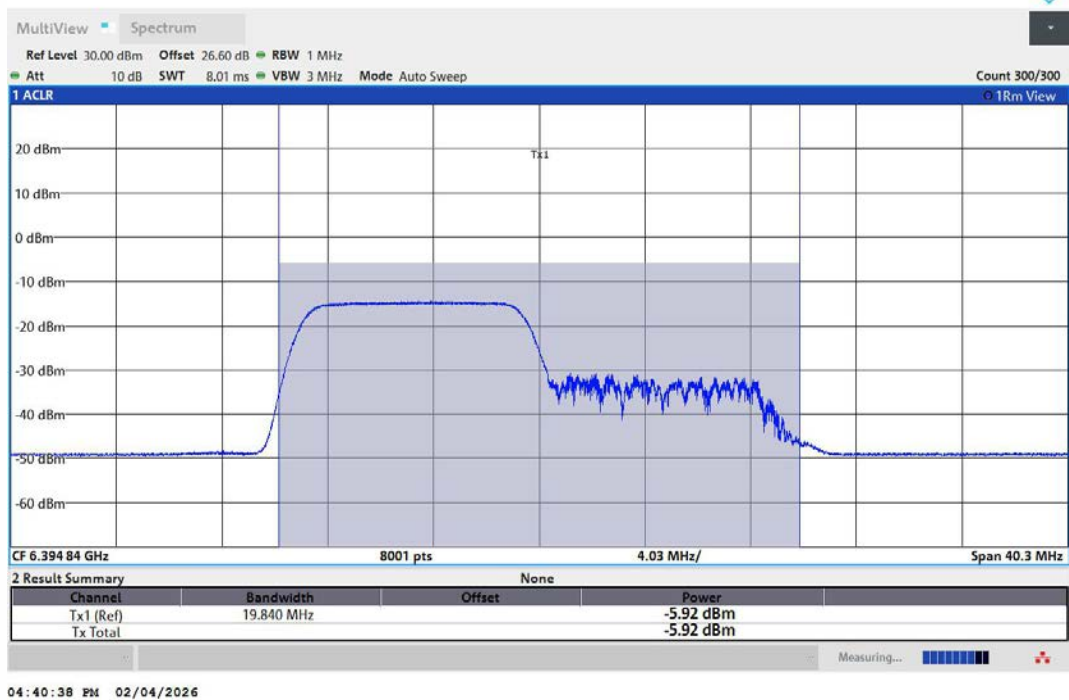
11AX40MIMO-Ant2-6405-106Tone-RU53-PASS
