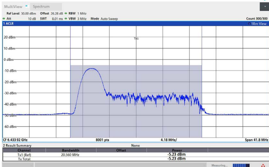
11AX40MIMO-Ant2-6445-26Tone-RU0-PASS
