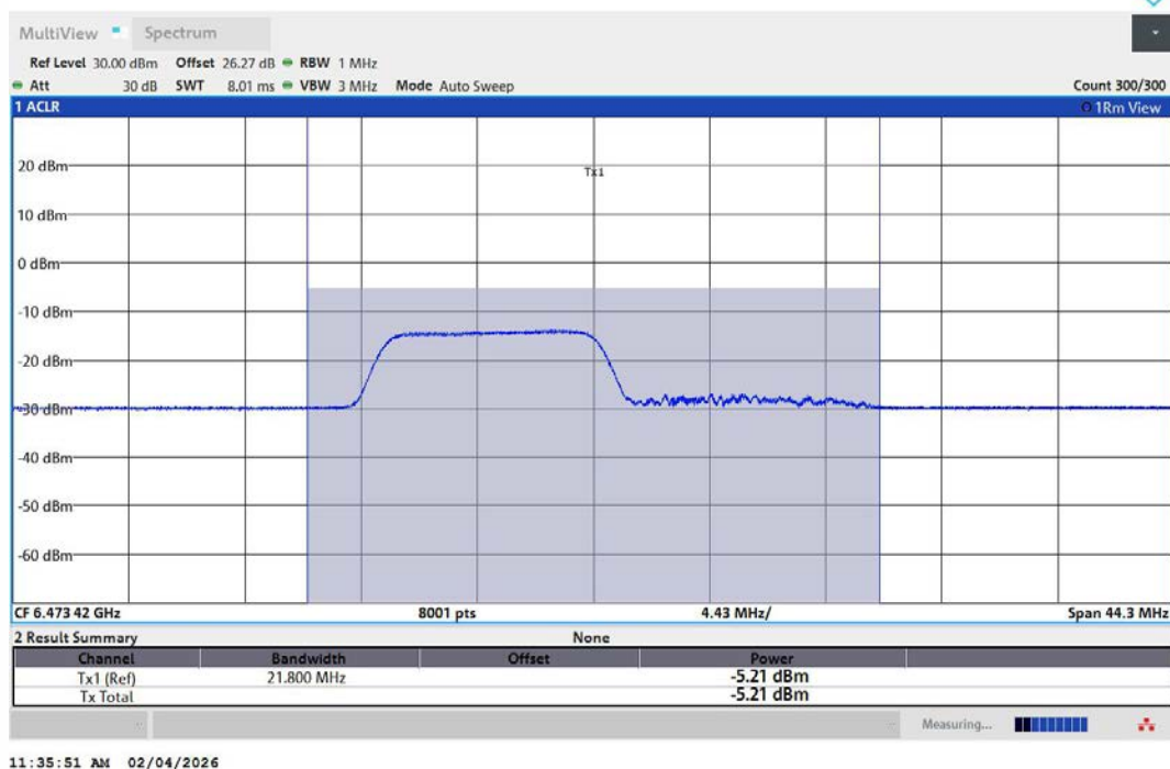
11AX20MIMO-Ant2-6475-106Tone-RU53-PASS
