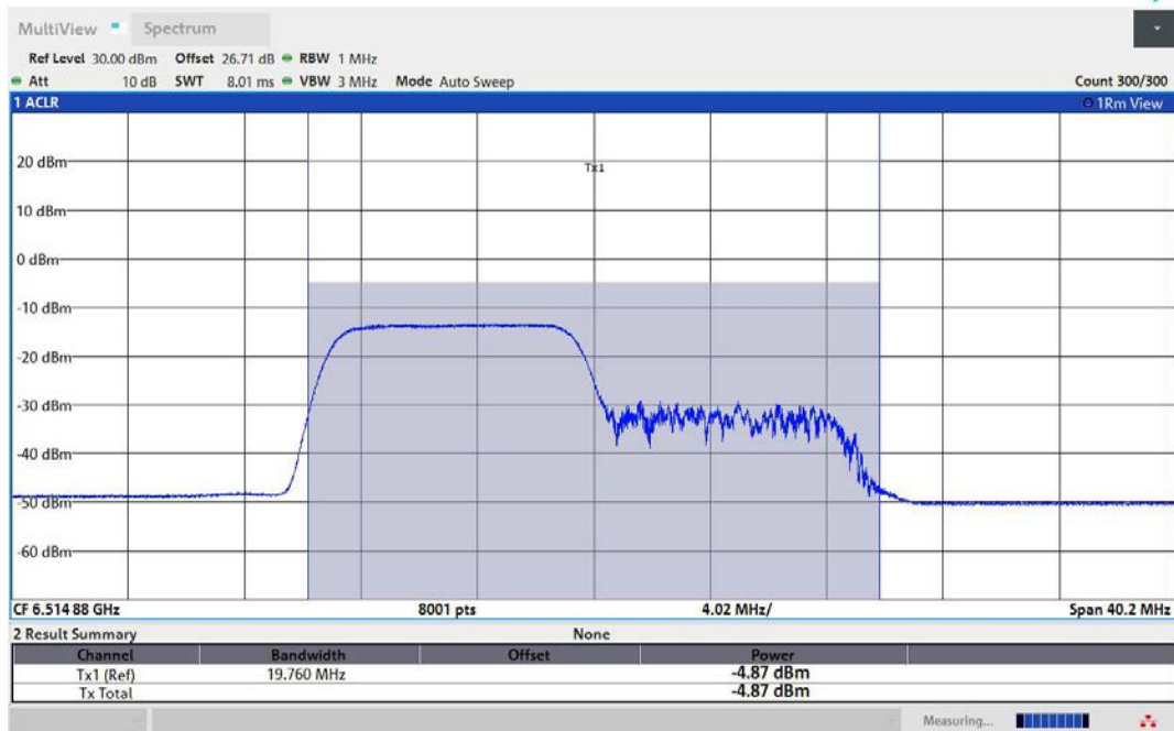
11AX40MIMO-Ant2-6525-106Tone-RU53-PASS
