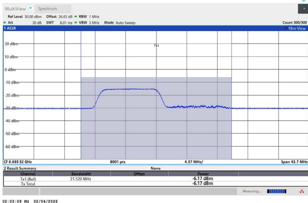
11AX20MIMO-Ant2-6695-106Tone-RU53-PASS
