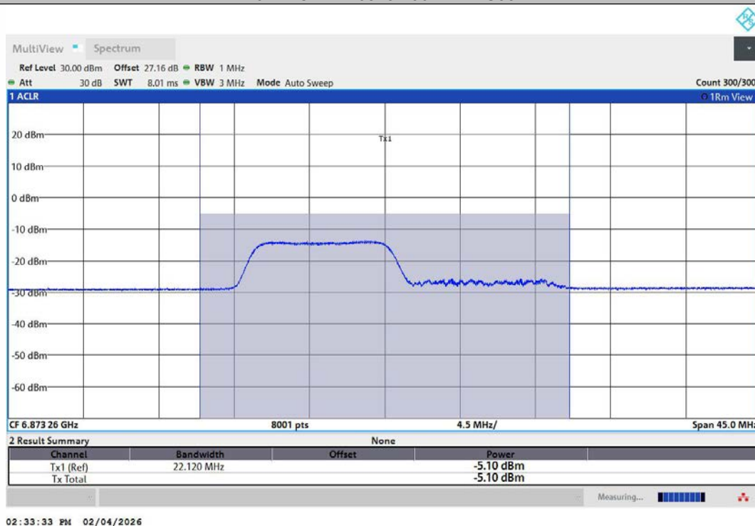
11AX20MIMO-Ant2-6875-106Tone-RU53-PASS
