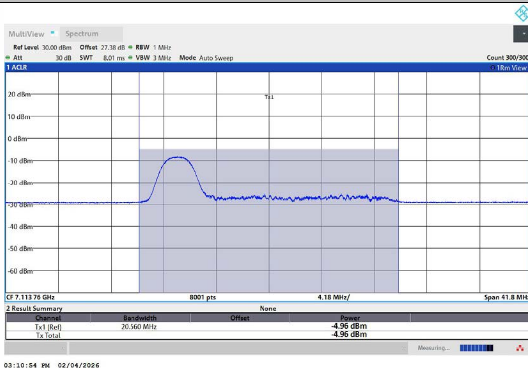
11AX20MIMO-Ant2-7115-26Tone-RU0-PASS
