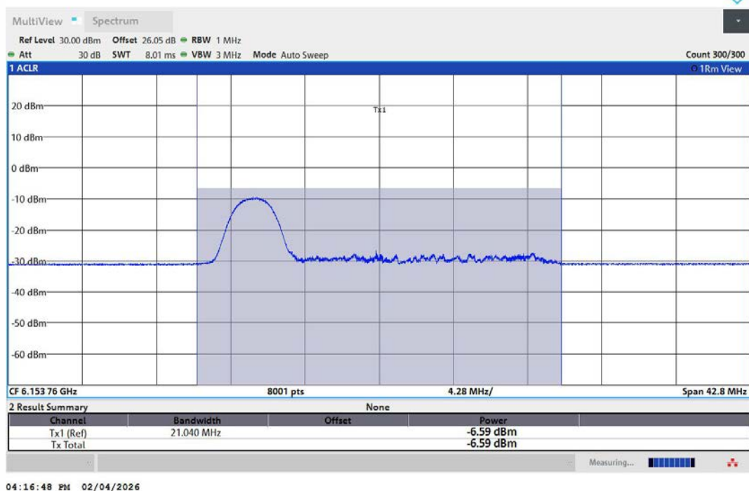
11AX40MIMO-Ant2-6165-26Tone-RU0-PASS
