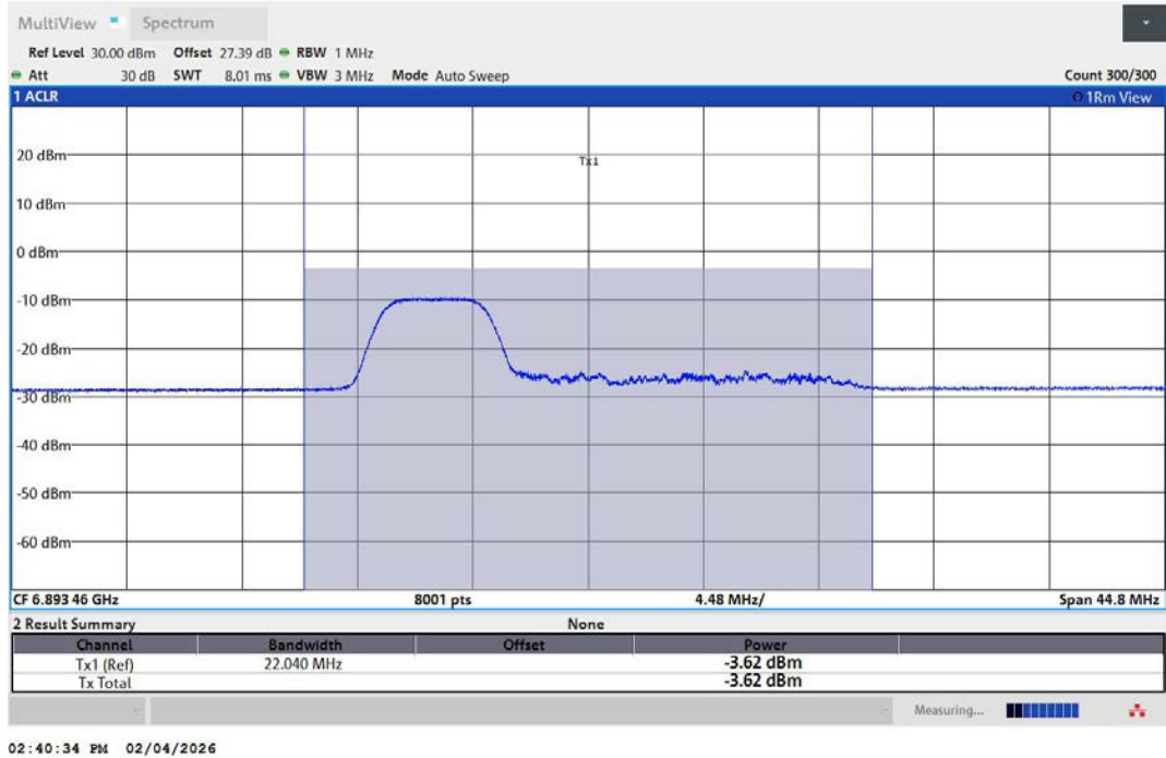
11AX20MIMO-Ant1-6895-52Tone-RU37-PASS
