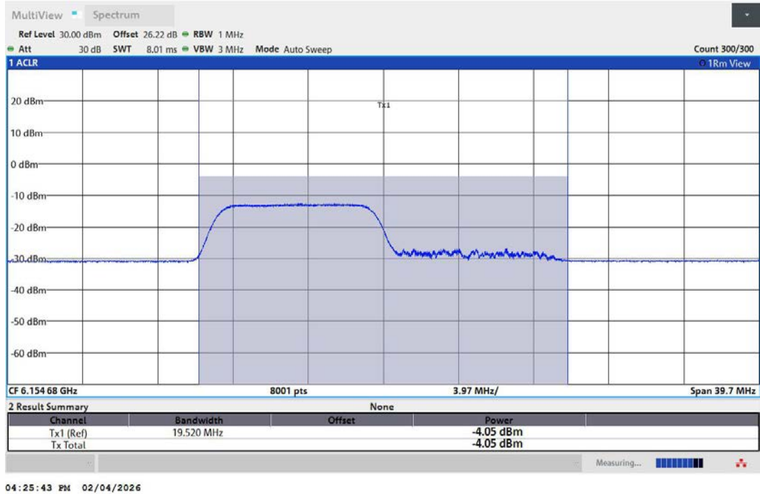
11AX40MIMO-Ant1-6165-106Tone-RU53-PASS
