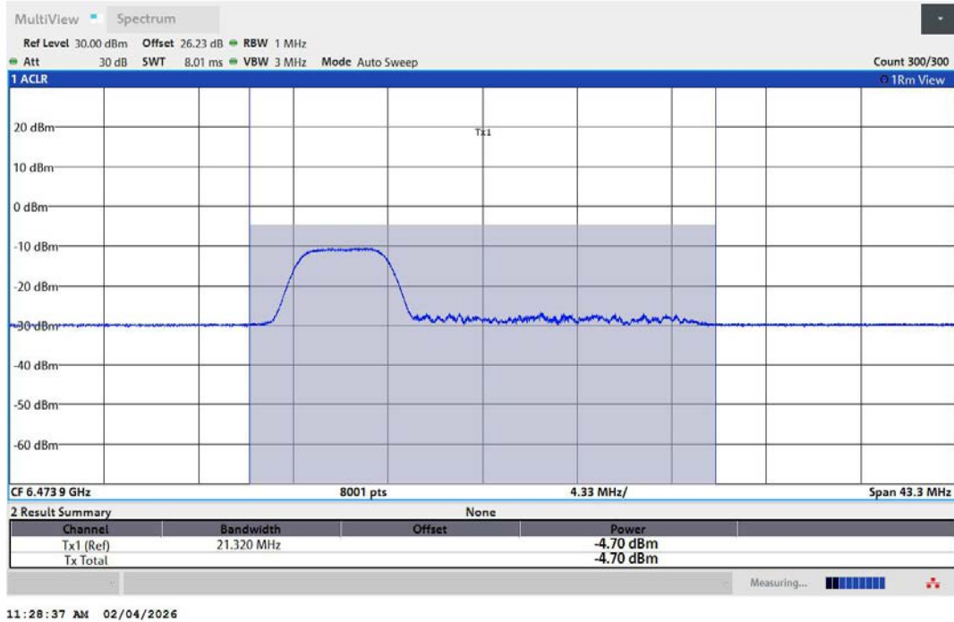
11AX20MIMO-Ant1-6475-52Tone-RU37-PASS
