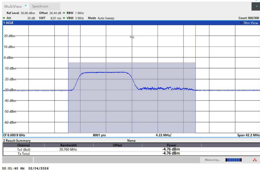
11AX20MIMO-Ant1-6695-106Tone-RU53-PASS
