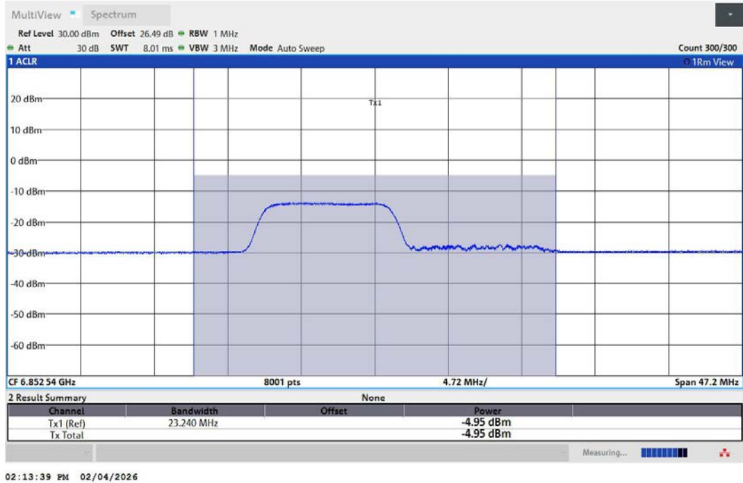
11AX20MIMO-Ant1-6855-106Tone-RU53-PASS
