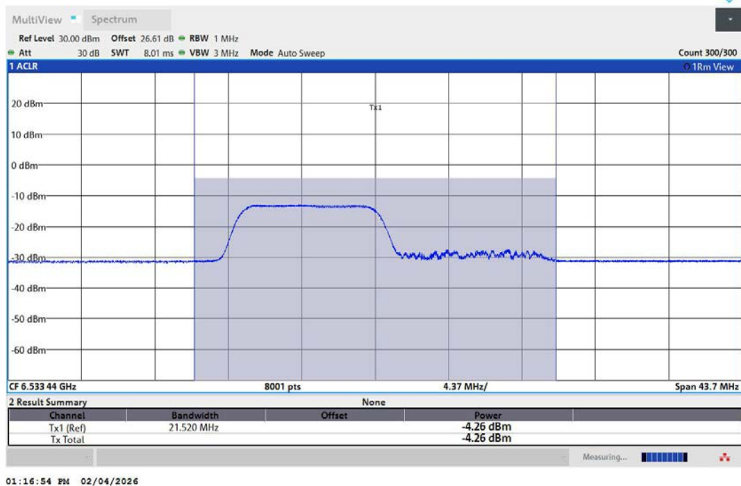
11AX20MIMO-Ant1-6535-106Tone-RU53-PASS
