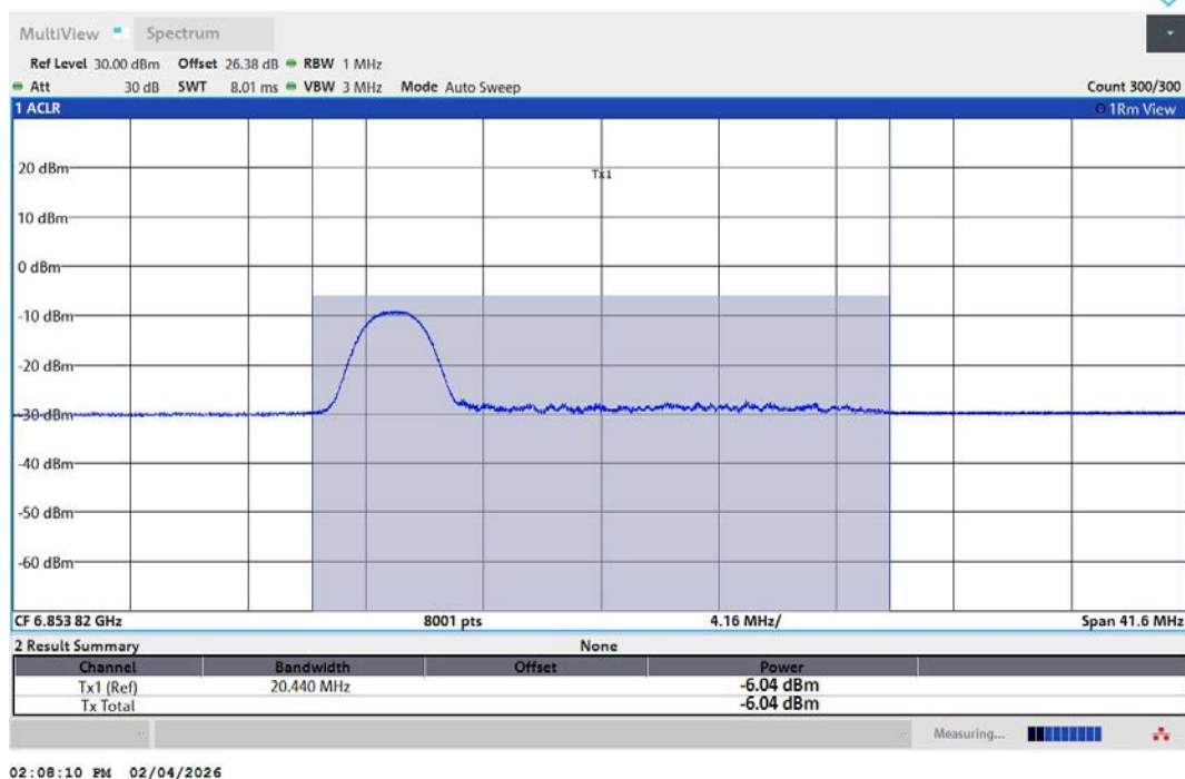
11AX20MIMO-Ant2-6855-26Tone-RU0-PASS
