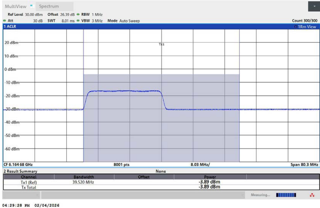
11AX40MIMO-Ant1-6165-242Tone-RU61-PASS
