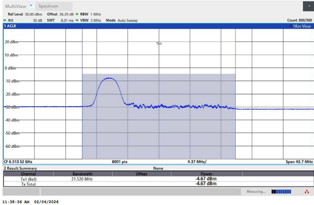
11AX20MIMO-Ant1-6515-26Tone-RU0-PASS
