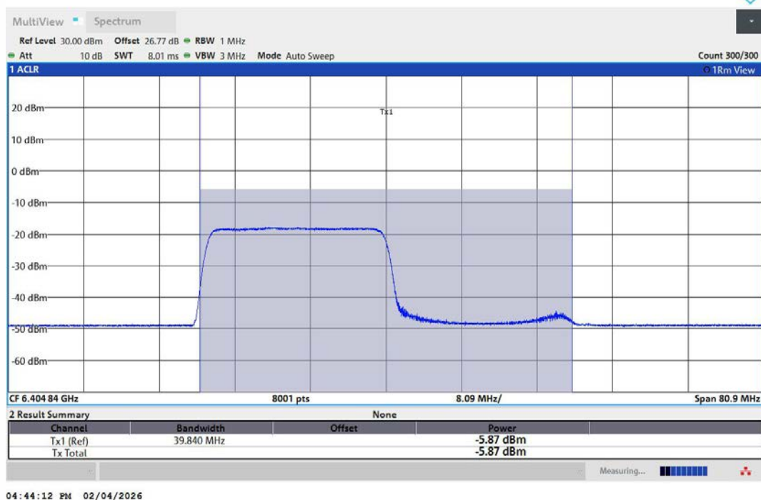
11AX40MIMO-Ant2-6405-242Tone-RU61-PASS
