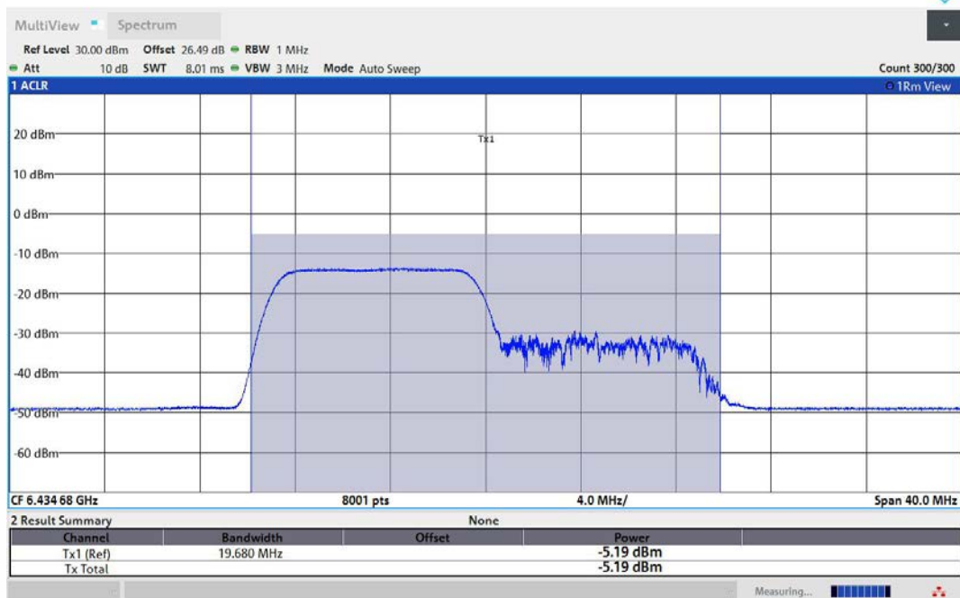
11AX40MIMO-Ant1-6445-106Tone-RU53-PASS
