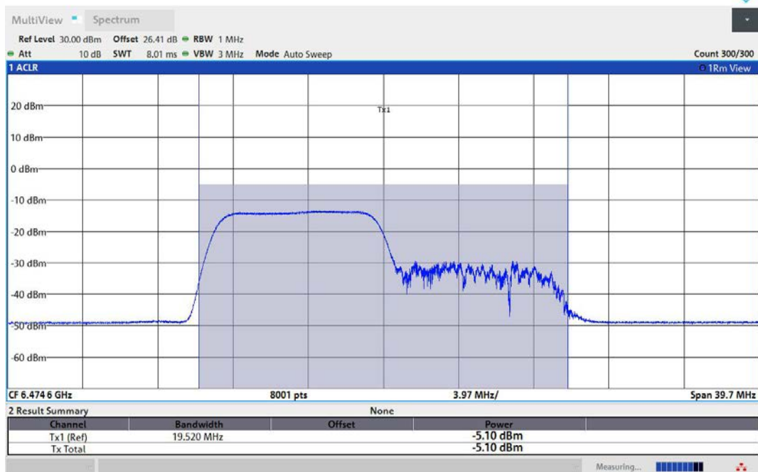
11AX40MIMO-Ant1-6485-106Tone-RU53-PASS
