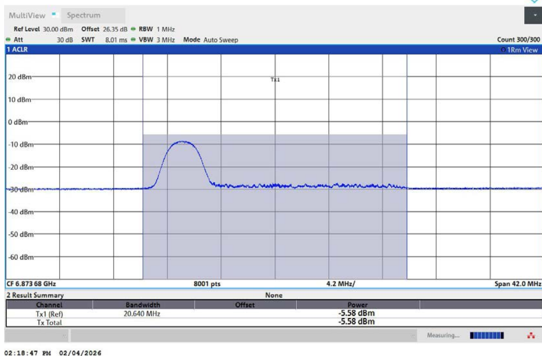
11AX20MIMO-Ant2-6875-26Tone-RU0-PASS
