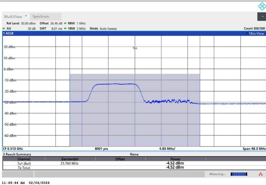
11AX20MIMO-Ant1-6515-106Tone-RU53-PASS
