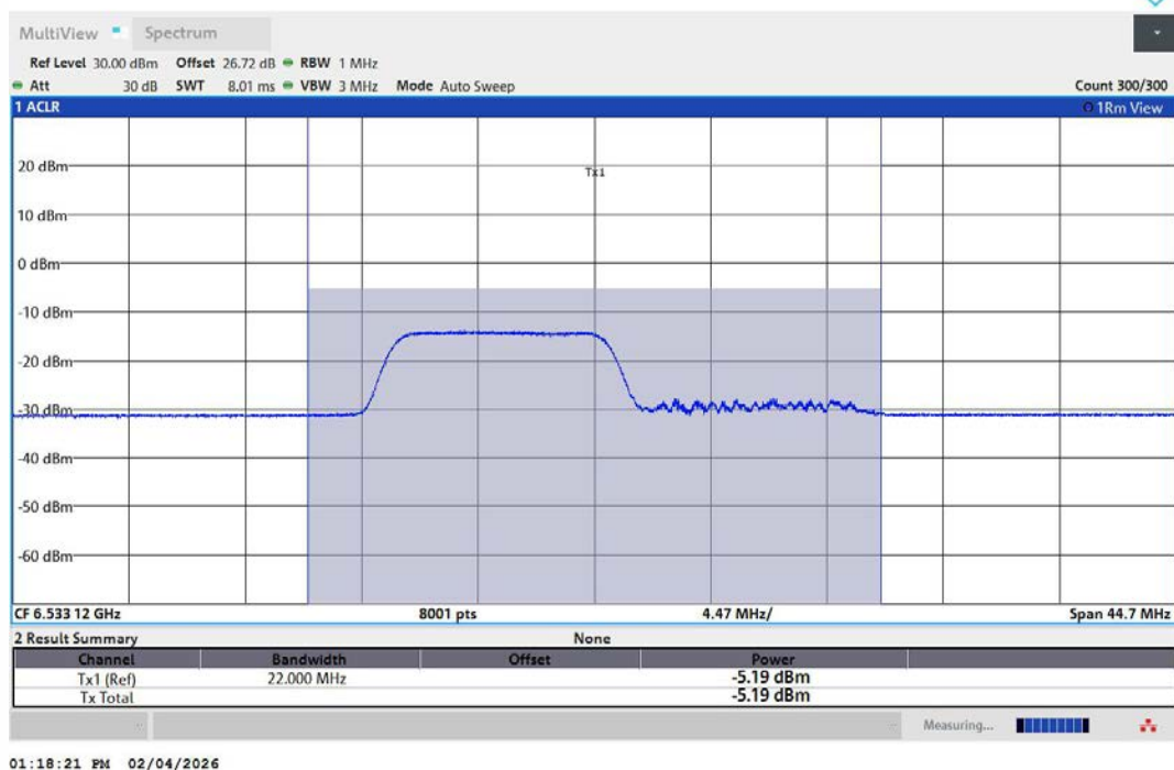
11AX20MIMO-Ant2-6535-106Tone-RU53-PASS
