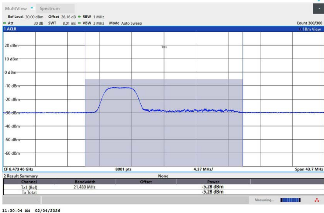
11AX20MIMO-Ant2-6475-52Tone-RU37-PASS
