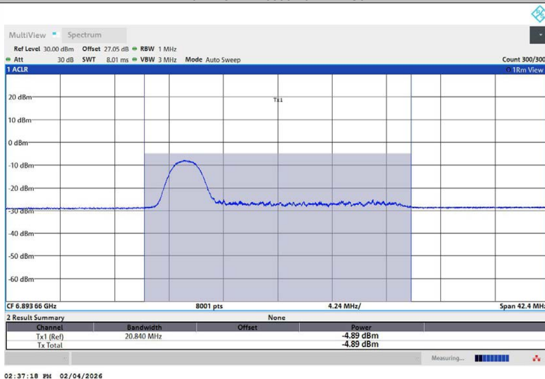
11AX20MIMO-Ant2-6895-26Tone-RU0-PASS
