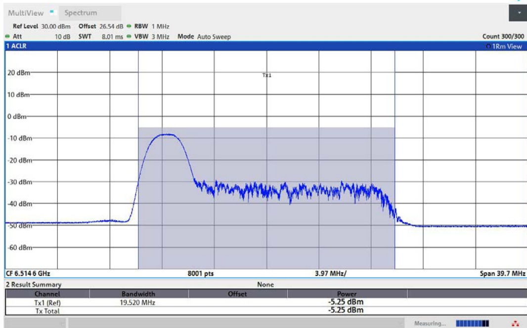
11AX40MIMO-Ant2-6525-26Tone-RU0-PASS
