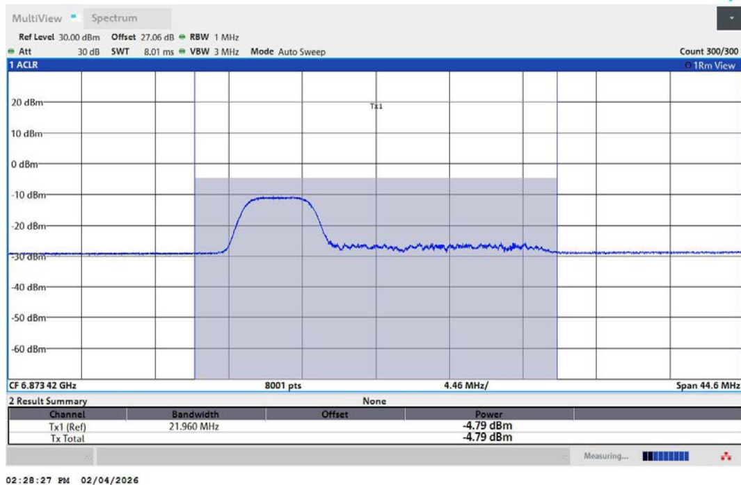
11AX20MIMO-Ant1-6875-52Tone-RU37-PASS
