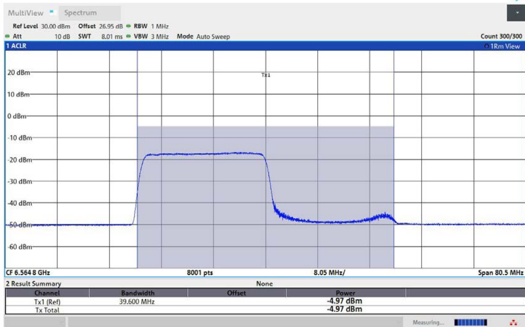
11AX40MIMO-Ant2-6565-242Tone-RU61-PASS
