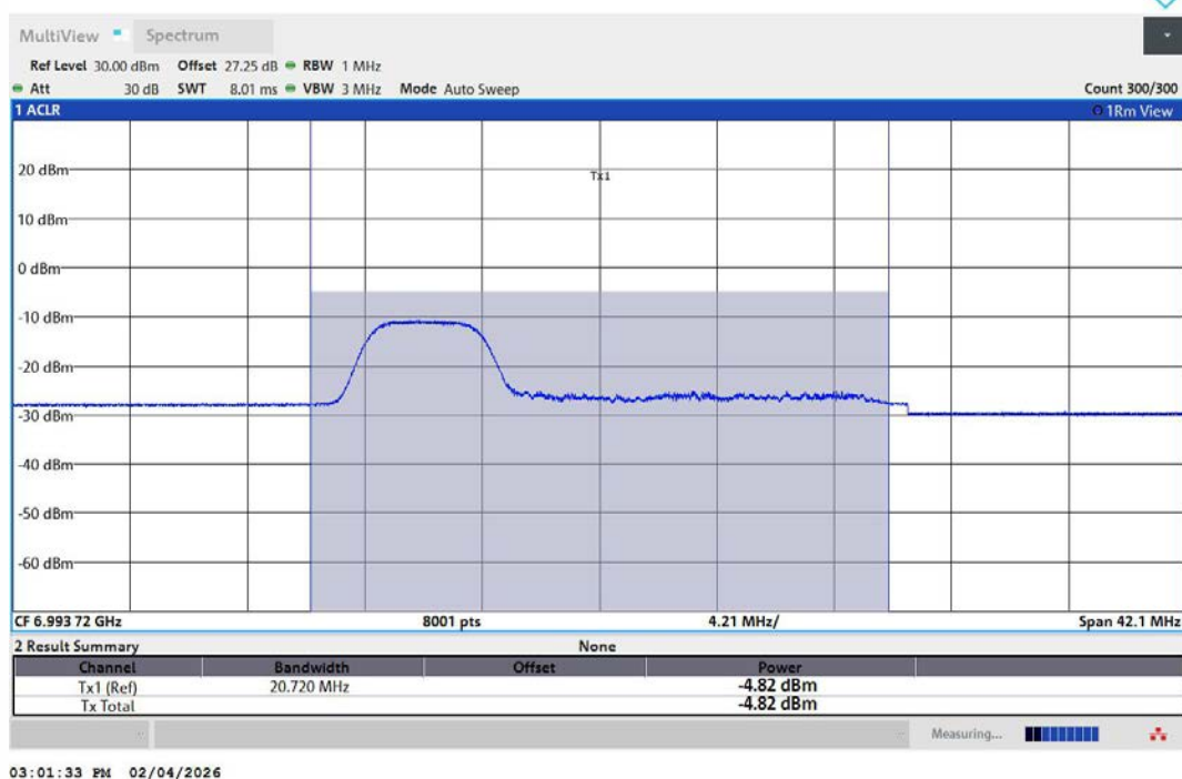
11AX20MIMO-Ant2-6995-52Tone-RU37-PASS
