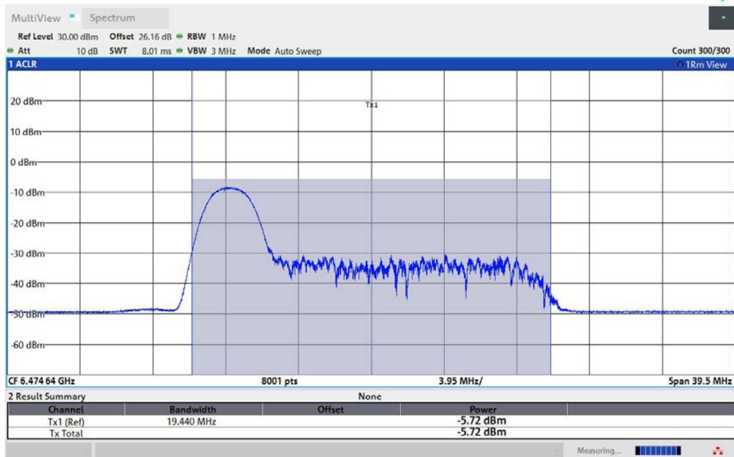
11AX40MIMO-Ant2-6485-26Tone-RU0-PASS
