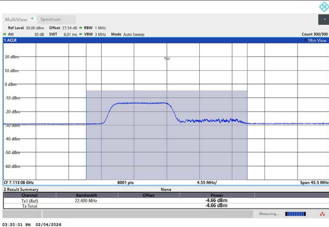
11AX20MIMO-Ant2-7115-106Tone-RU53-PASS
