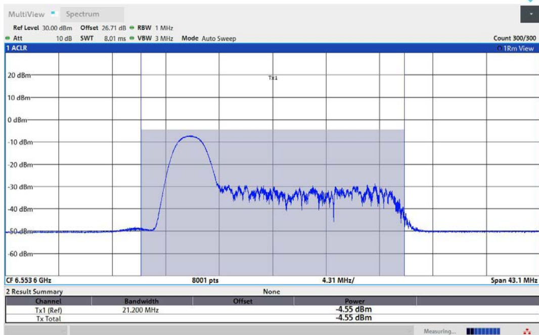
11AX40MIMO-Ant1-6565-26Tone-RU0-PASS
