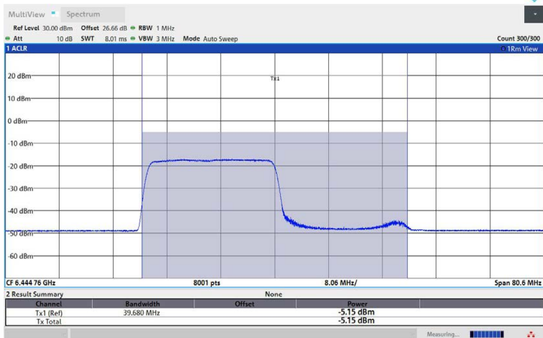
11AX40MIMO-Ant1-6445-242Tone-RU61-PASS
