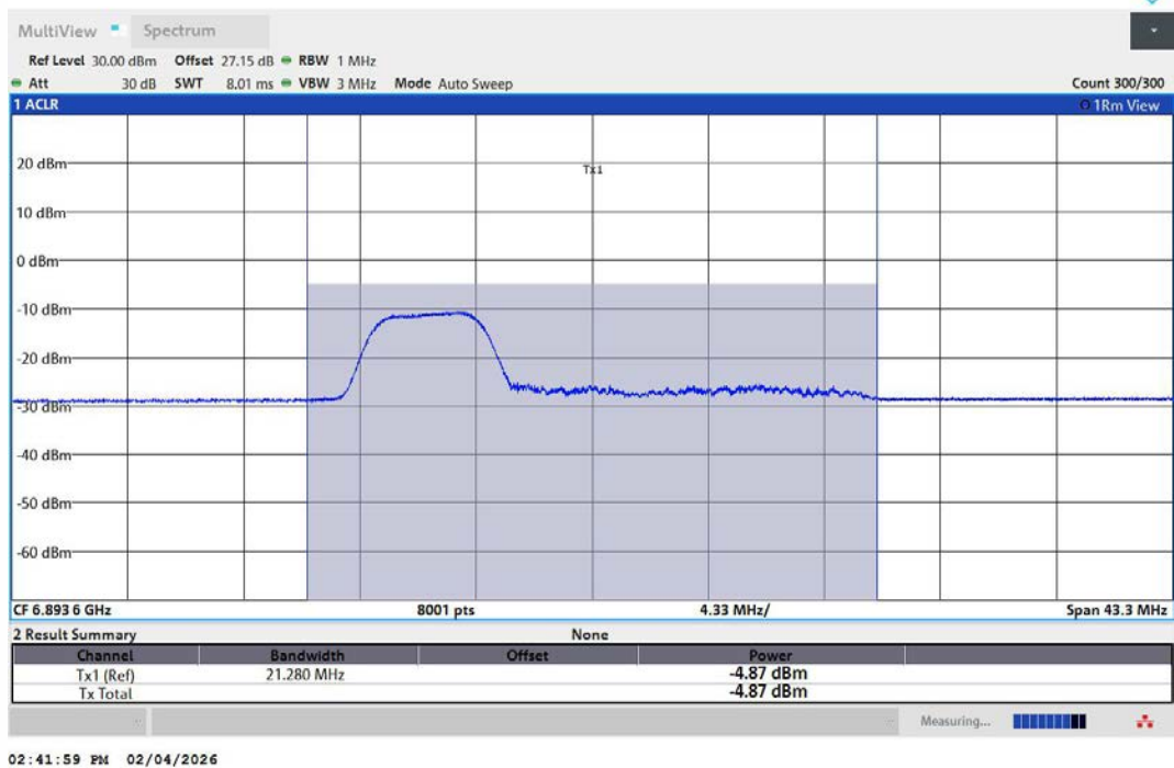
11AX20MIMO-Ant2-6895-52Tone-RU37-PASS
