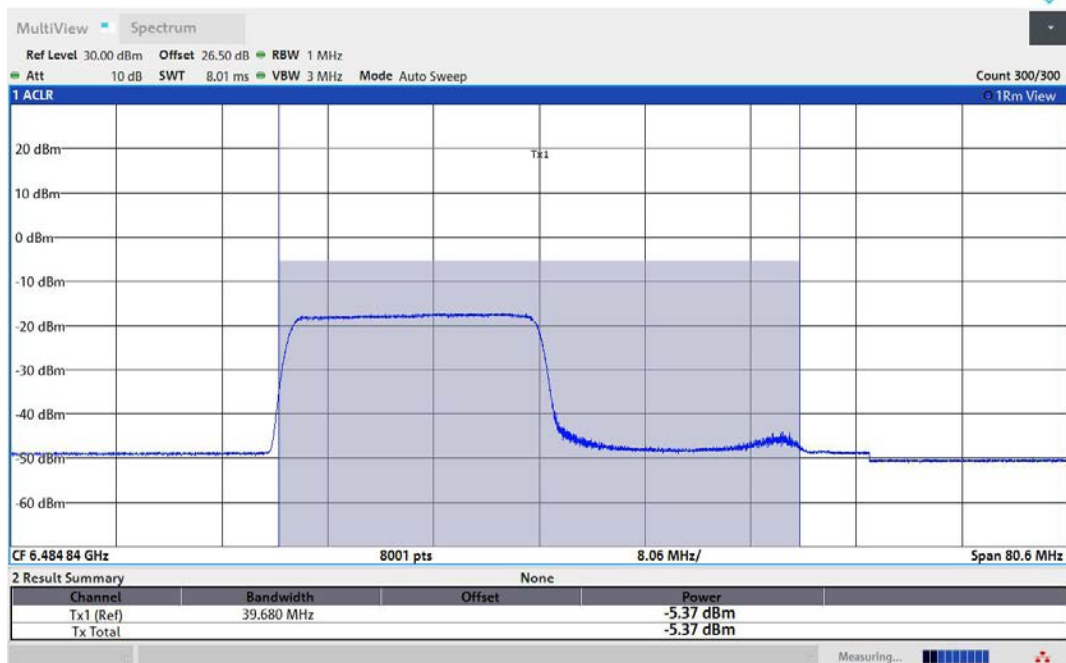
11AX40MIMO-Ant2-6485-242Tone-RU61-PASS
