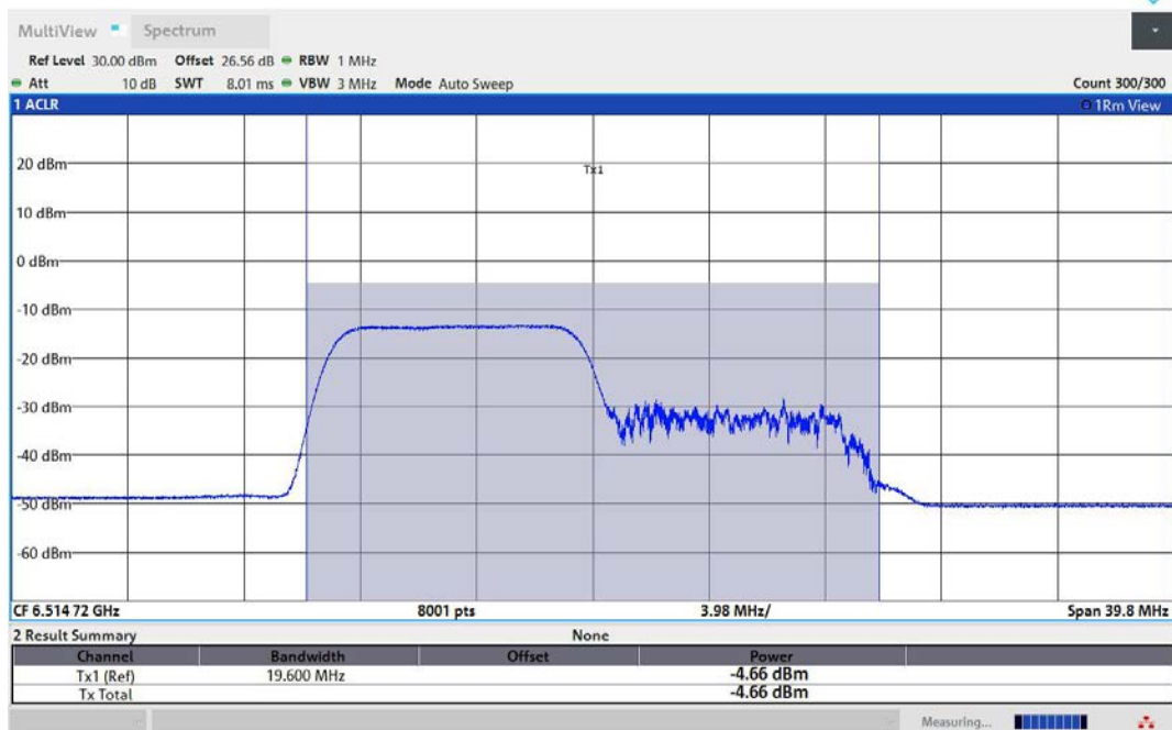
11AX40MIMO-Ant1-6525-106Tone-RU53-PASS
