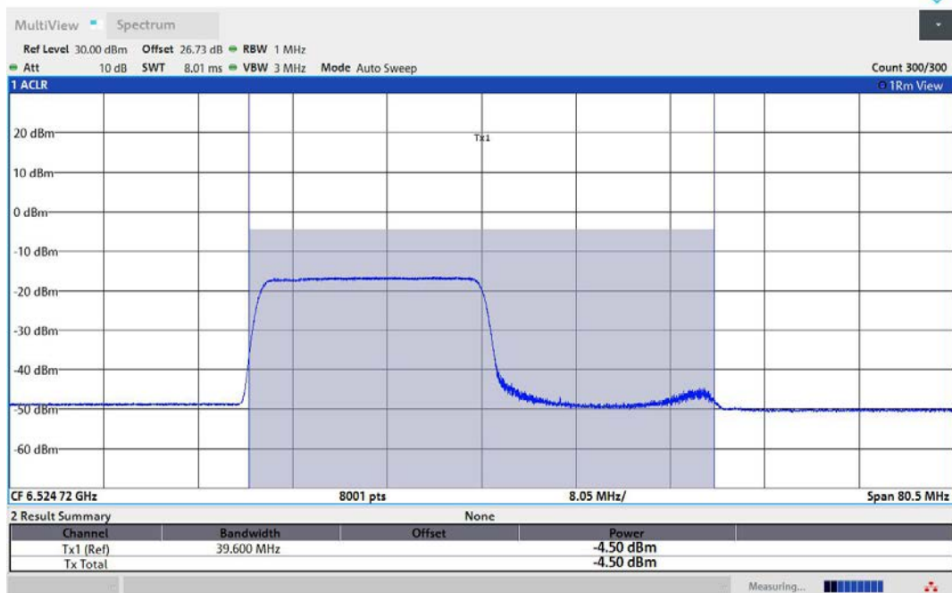
11AX40MIMO-Ant1-6525-242Tone-RU61-PASS
