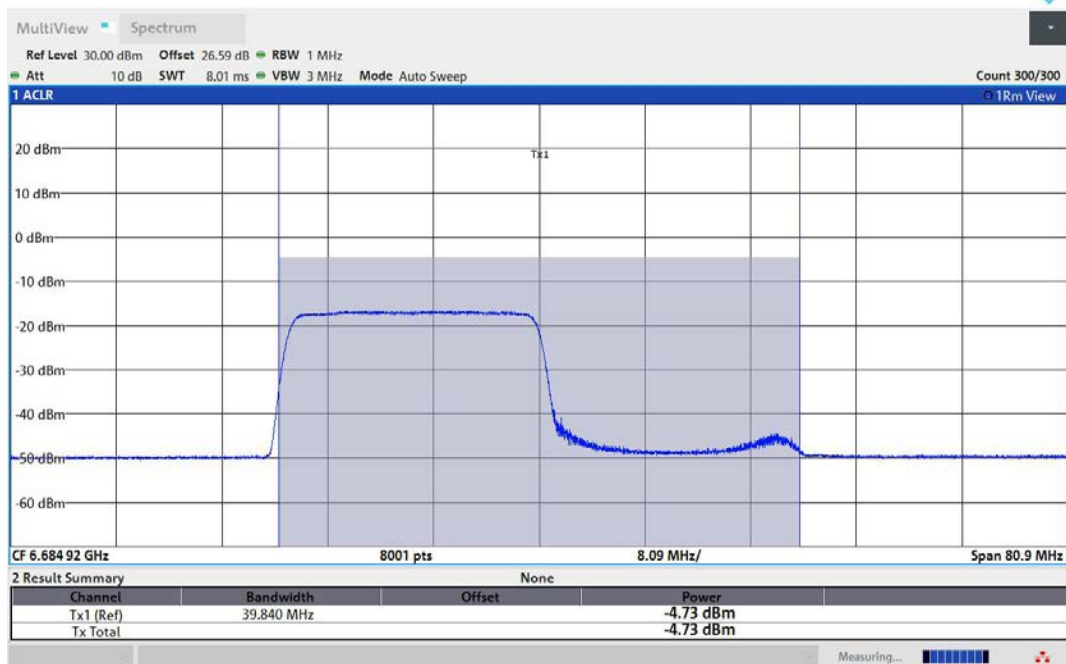
11AX40MIMO-Ant1-6685-242Tone-RU61-PASS
