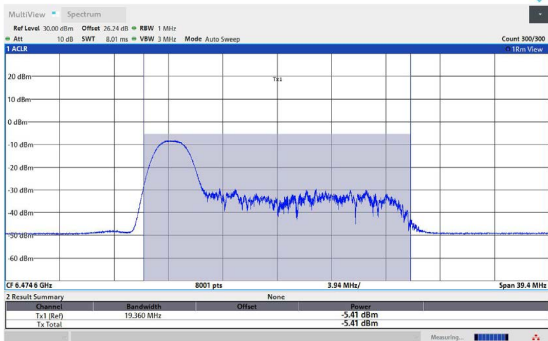
11AX40MIMO-Ant1-6485-26Tone-RU0-PASS
