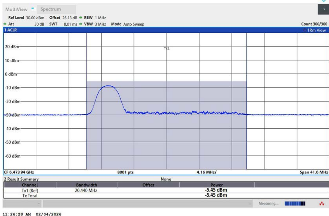
11AX20MIMO-Ant2-6475-26Tone-RU0-PASS
