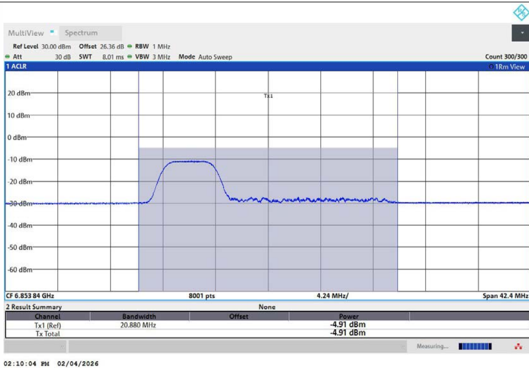
11AX20MIMO-Ant1-6855-52Tone-RU37-PASS
