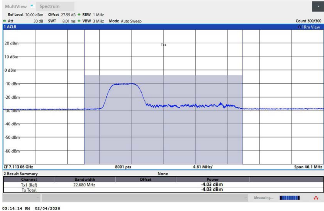
11AX20MIMO-Ant1-7115-52Tone-RU37-PASS
