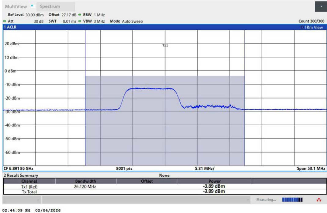
11AX20MIMO-Ant1-6895-106Tone-RU53-PASS
