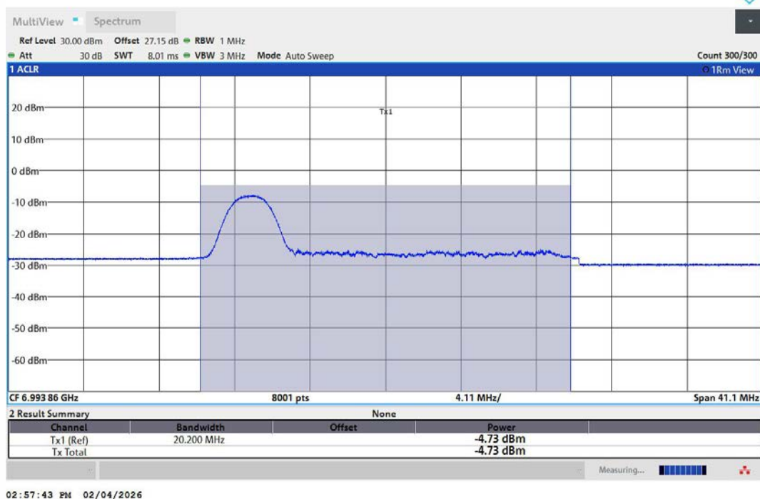
11AX20MIMO-Ant2-6995-26Tone-RU0-PASS
