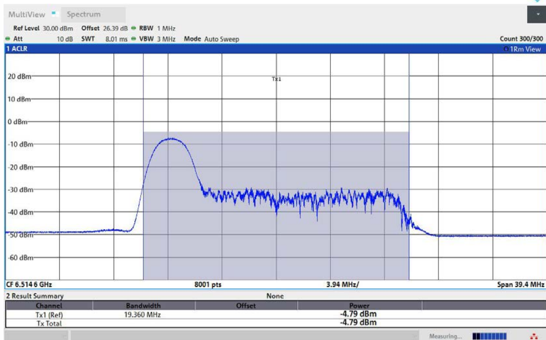
11AX40MIMO-Ant1-6525-26Tone-RU0-PASS
