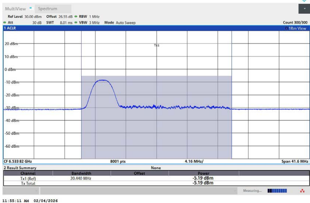
11AX20MIMO-Ant2-6535-26Tone-RU0-PASS
