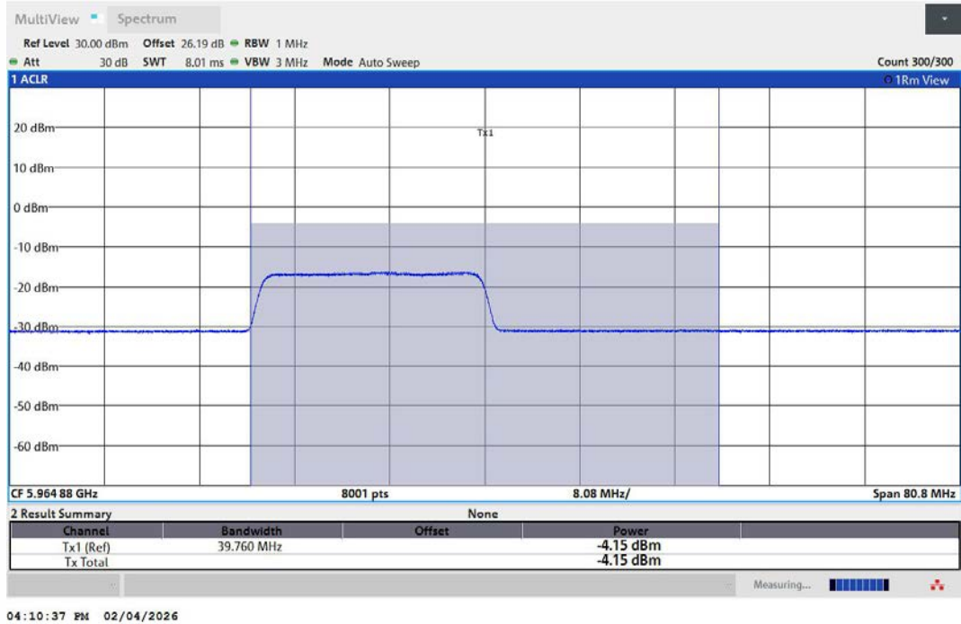
11AX40MIMO-Ant1-5965-242Tone-RU61-PASS
