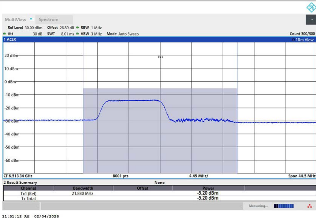
11AX20MIMO-Ant2-6515-106Tone-RU53-PASS
