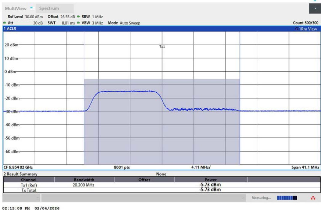
11AX20MIMO-Ant2-6855-106Tone-RU53-PASS
