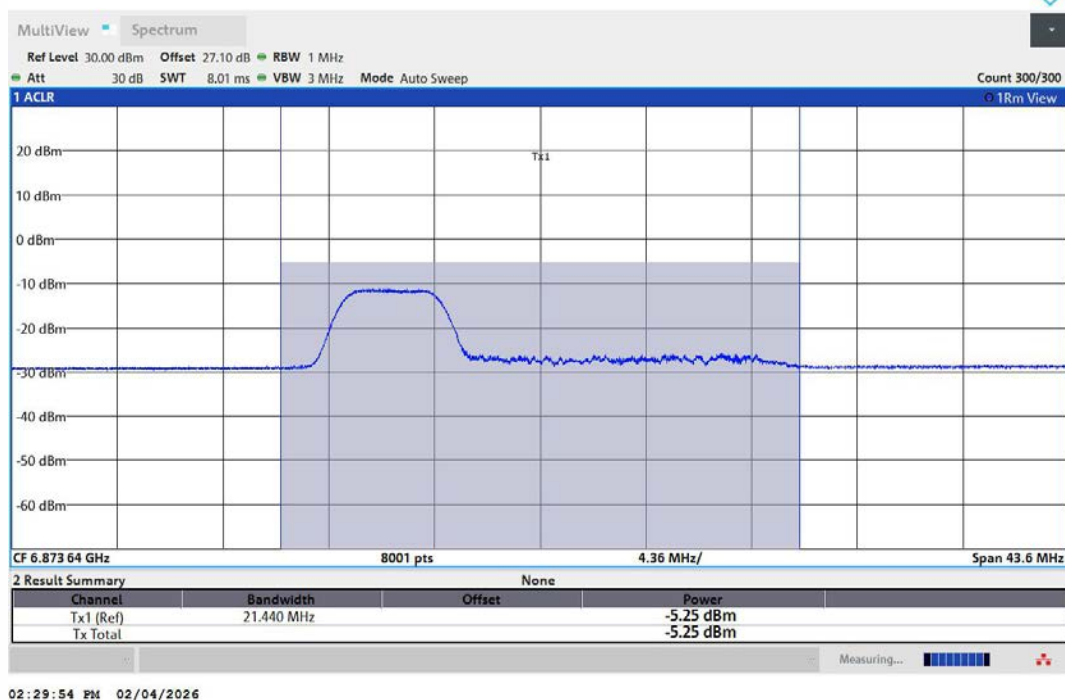
11AX20MIMO-Ant2-6875-52Tone-RU37-PASS
