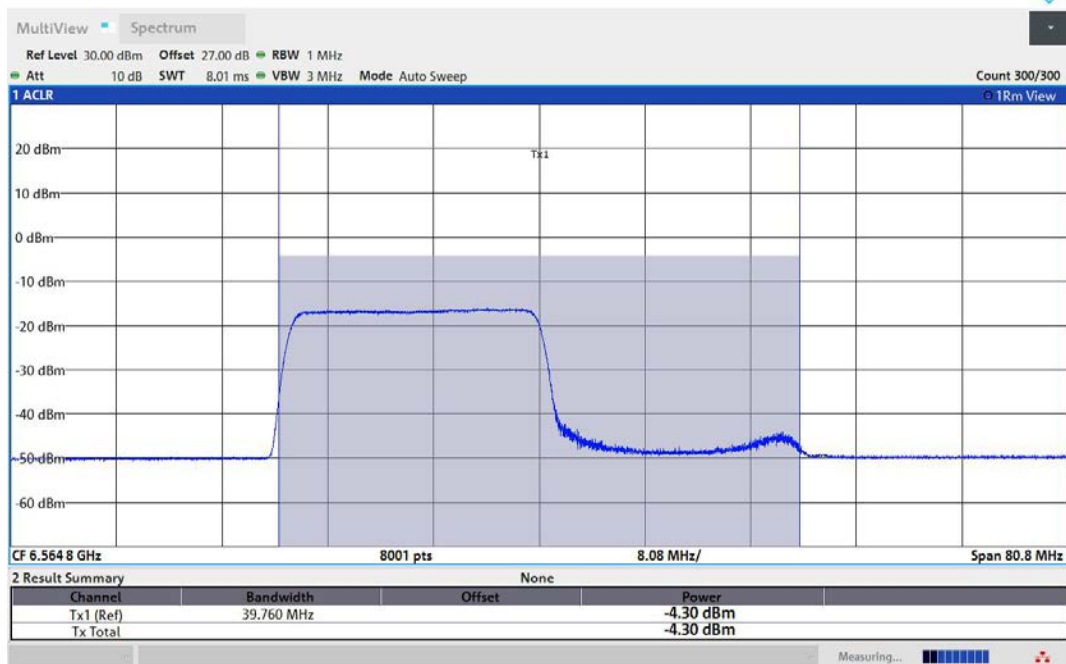
11AX40MIMO-Ant1-6565-242Tone-RU61-PASS
