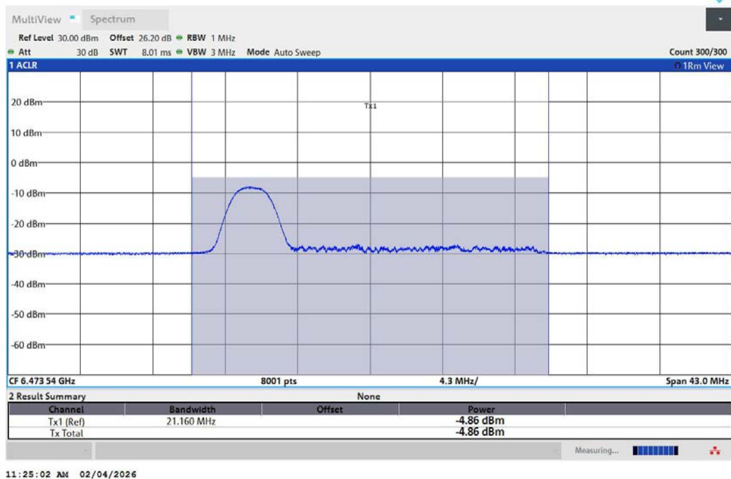
11AX20MIMO-Ant1-6475-26Tone-RU0-PASS
