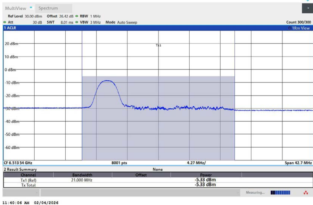
11AX20MIMO-Ant2-6515-26Tone-RU0-PASS
