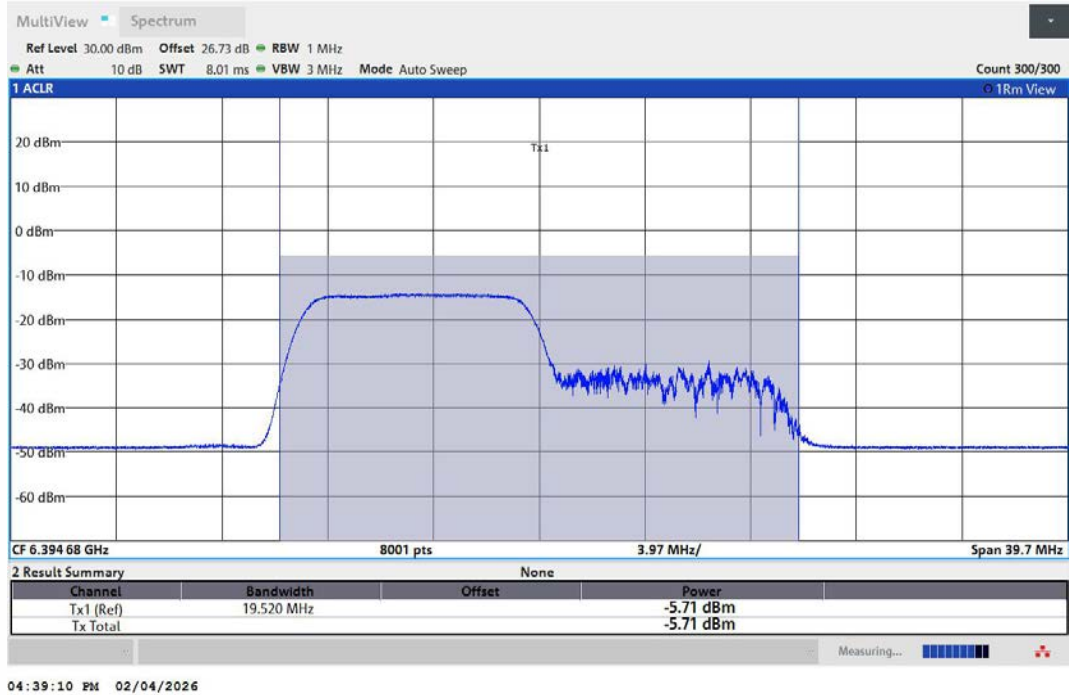
11AX40MIMO-Ant1-6405-106Tone-RU53-PASS
