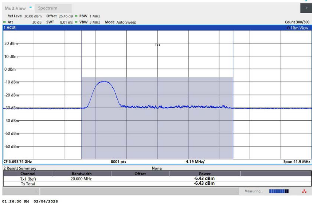
11AX20MIMO-Ant2-6695-26Tone-RU0-PASS
