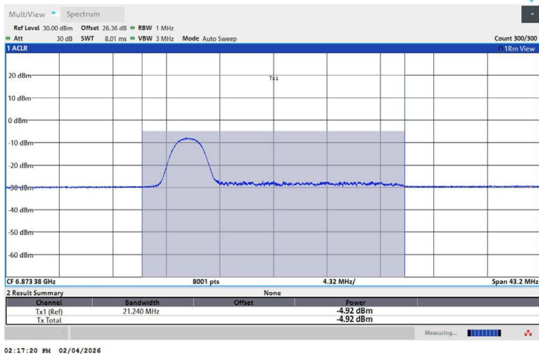
11AX20MIMO-Ant1-6875-26Tone-RU0-PASS
