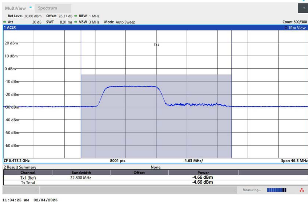
11AX20MIMO-Ant1-6475-106Tone-RU53-PASS
