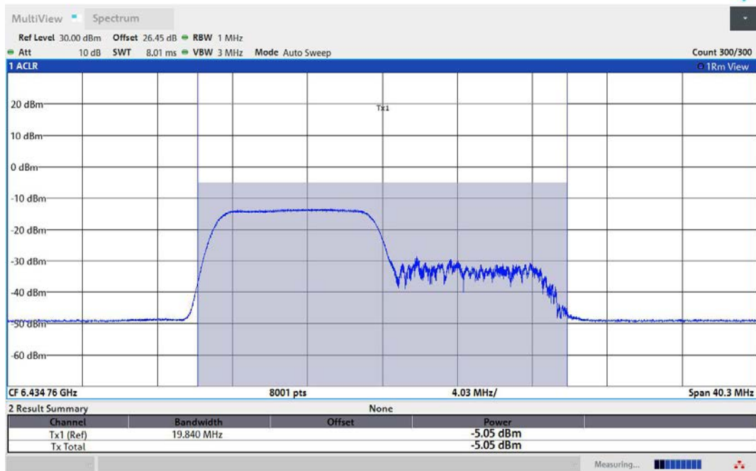
11AX40MIMO-Ant2-6445-106Tone-RU53-PASS
