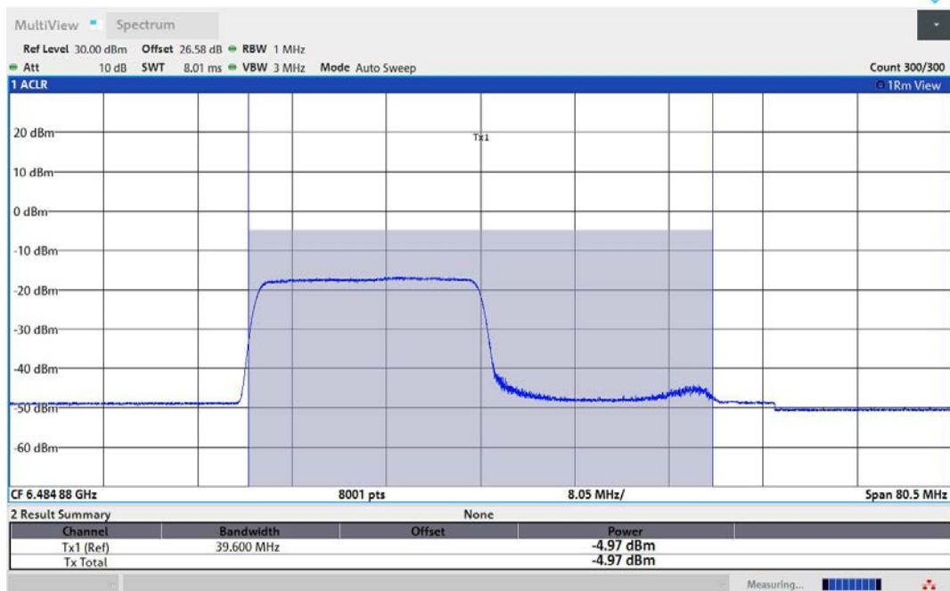
11AX40MIMO-Ant1-6485-242Tone-RU61-PASS
