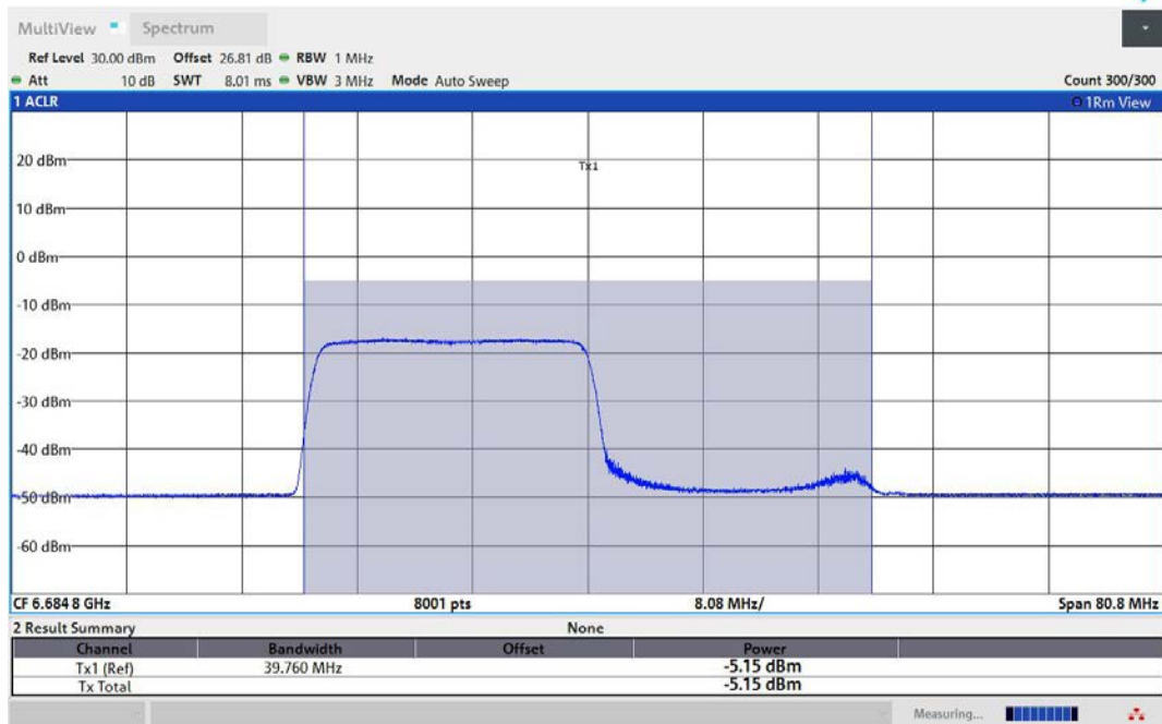
11AX40MIMO-Ant2-6685-242Tone-RU61-PASS
