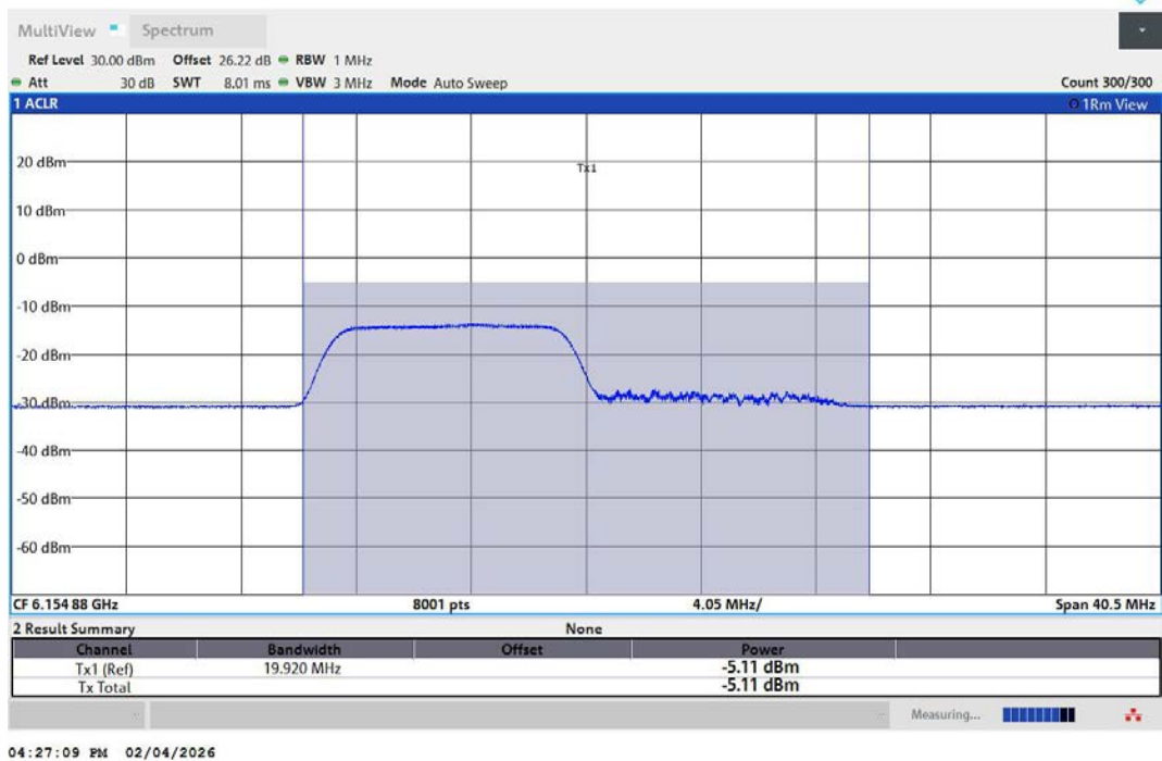
11AX40MIMO-Ant2-6165-106Tone-RU53-PASS
