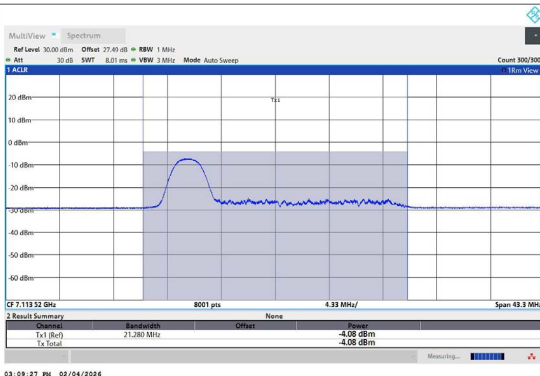
11AX20MIMO-Ant1-7115-26Tone-RU0-PASS
