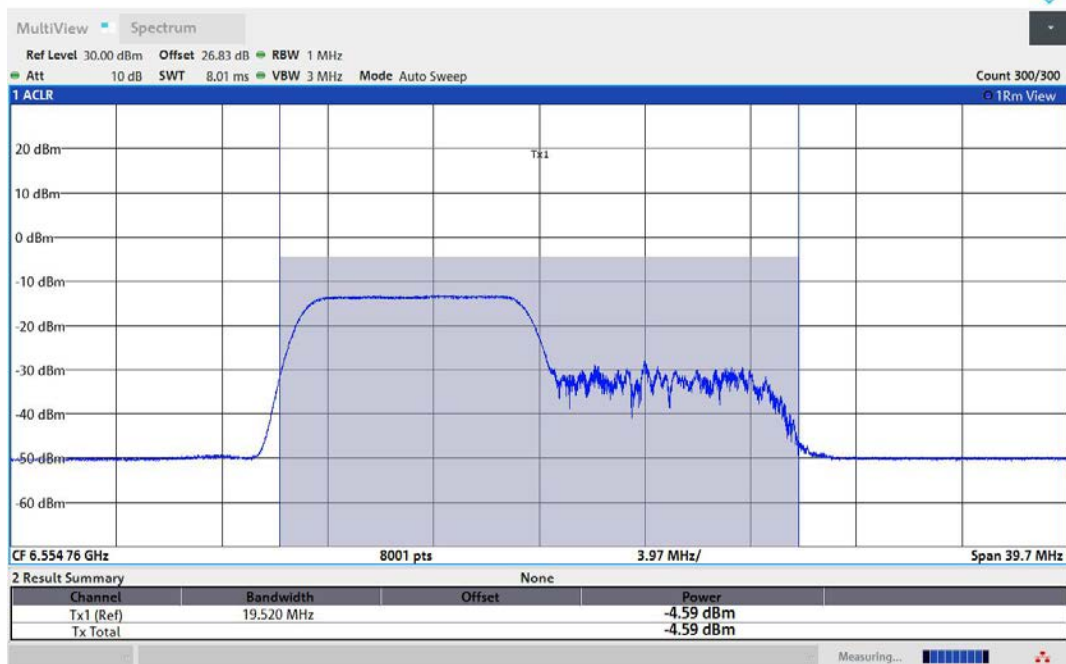
11AX40MIMO-Ant1-6565-106Tone-RU53-PASS
