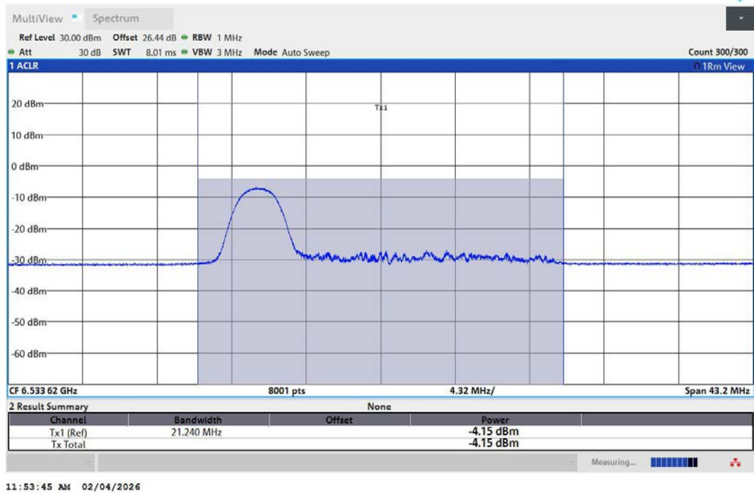
11AX20MIMO-Ant1-6535-26Tone-RU0-PASS
