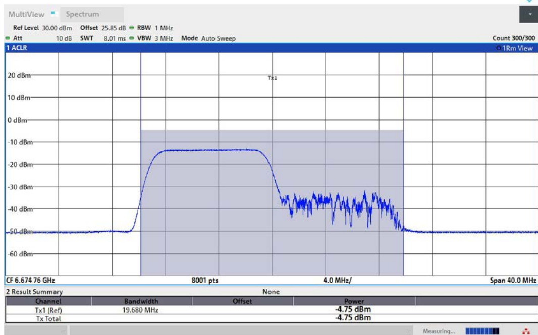
11AX40MIMO-Ant1-6685-106Tone-RU53-PASS
