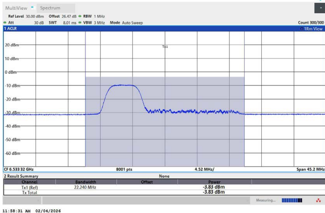
11AX20MIMO-Ant1-6535-52Tone-RU37-PASS
