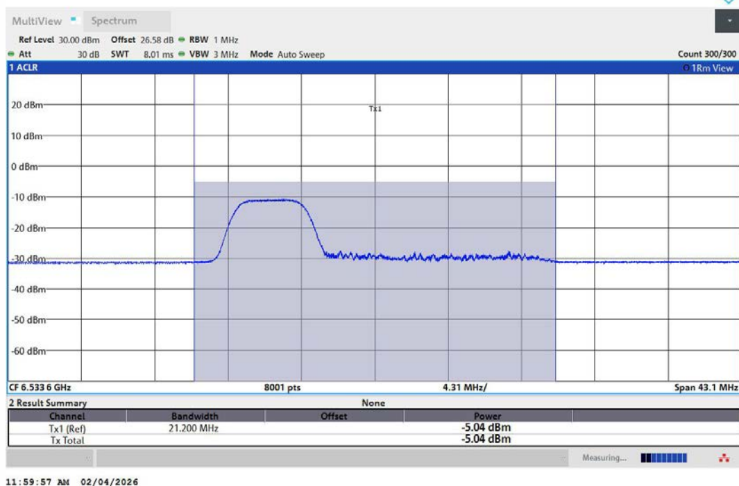
11AX20MIMO-Ant2-6535-52Tone-RU37-PASS
