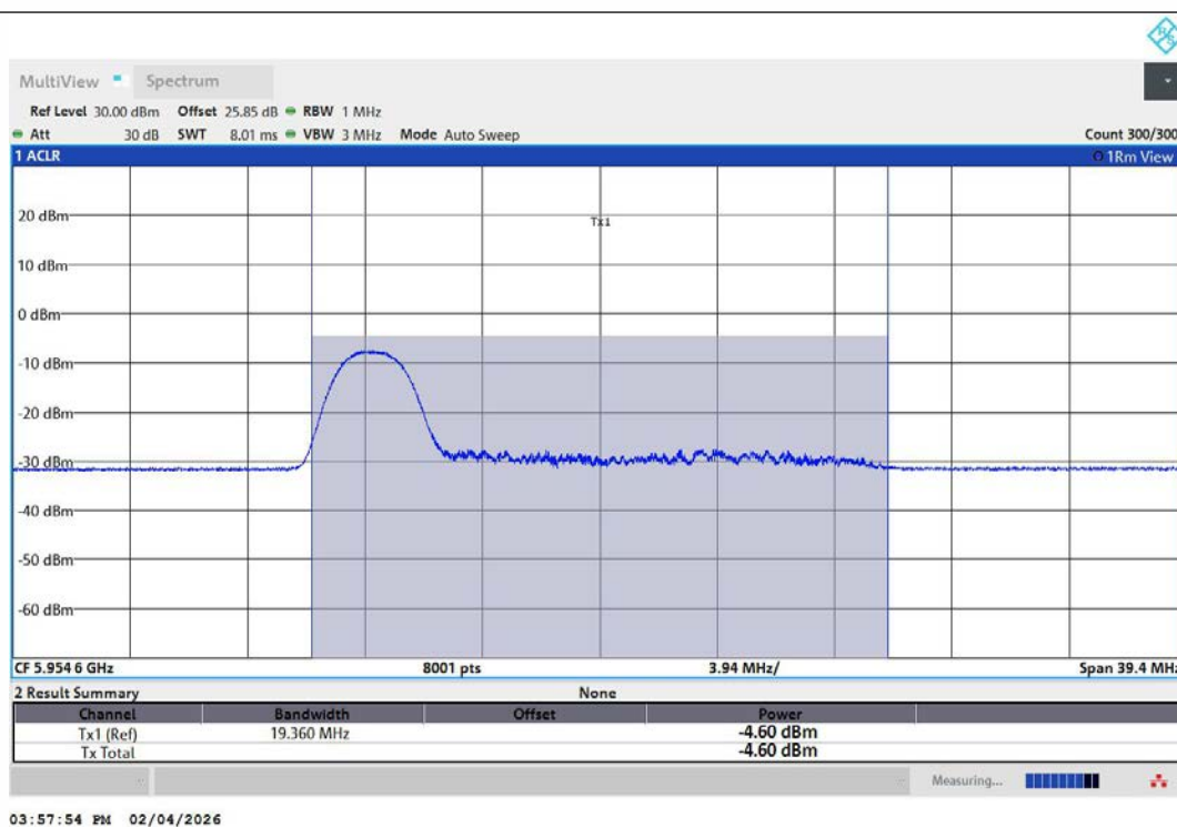
11AX40MIMO-Ant1-5965-26Tone-RU0-PASS
