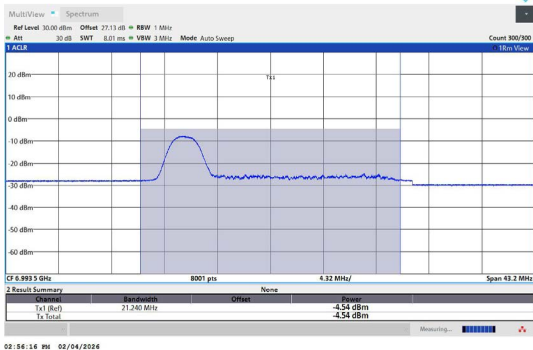
11AX20MIMO-Ant1-6995-26Tone-RU0-PASS
