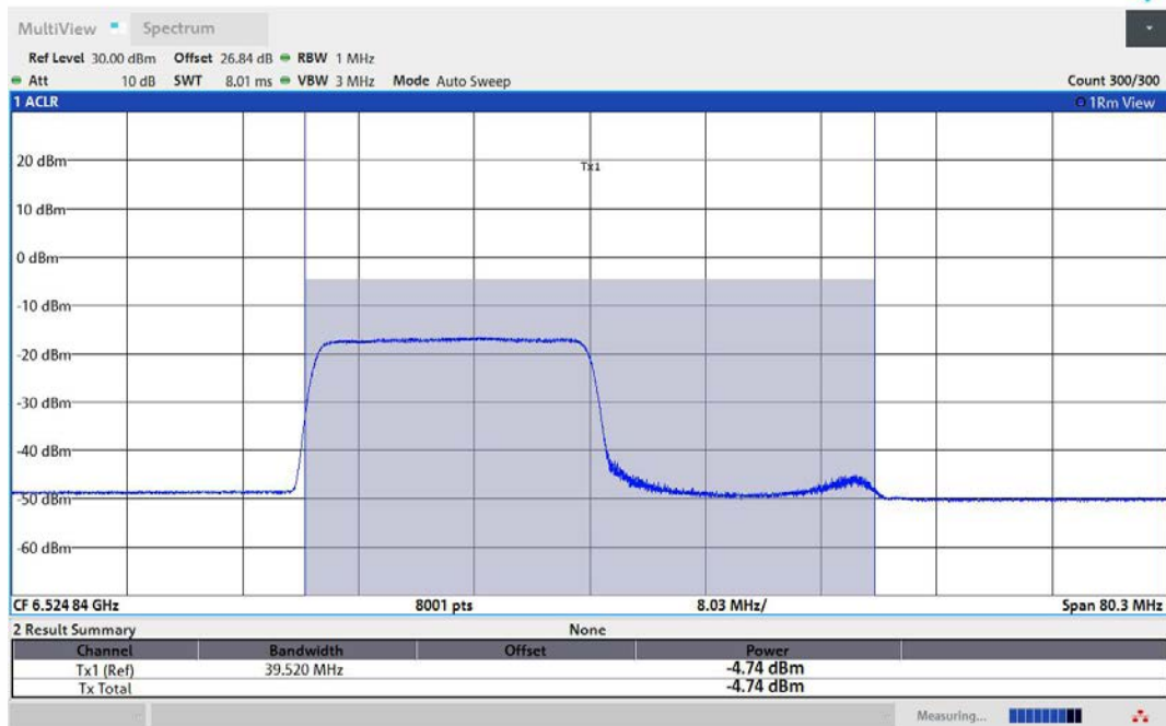
11AX40MIMO-Ant2-6525-242Tone-RU61-PASS
