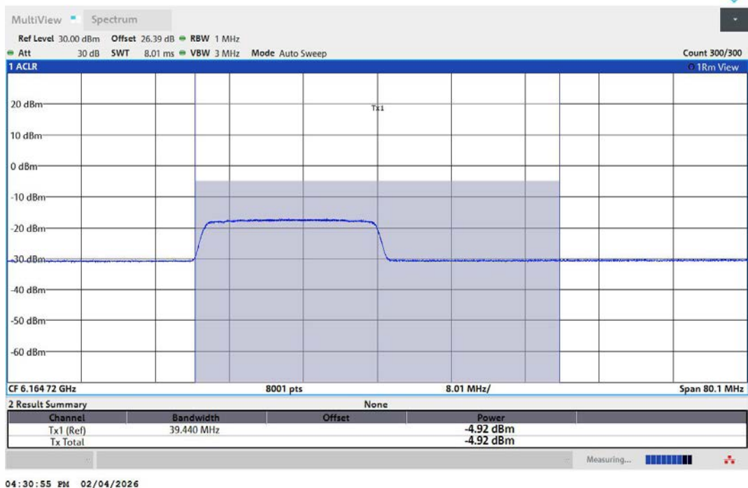
11AX40MIMO-Ant2-6165-242Tone-RU61-PASS
