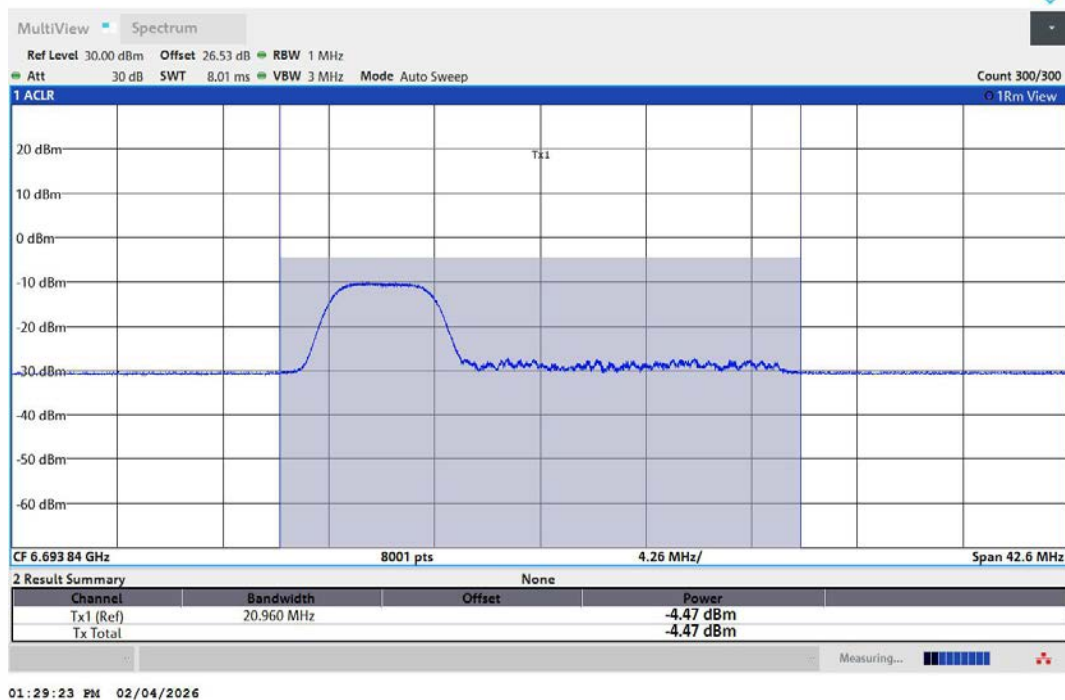
11AX20MIMO-Ant1-6695-52Tone-RU37-PASS
