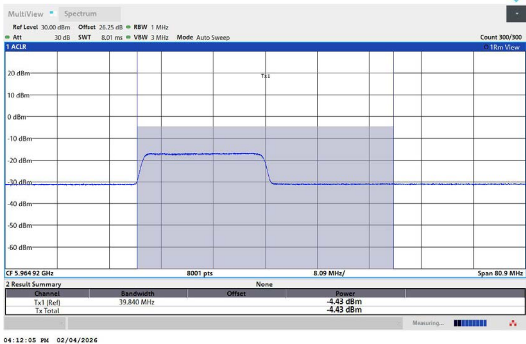
11AX40MIMO-Ant2-5965-242Tone-RU61-PASS
