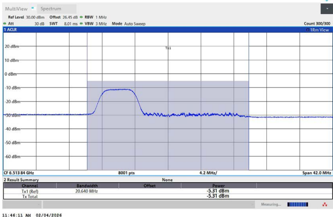
11AX20MIMO-Ant2-6515-52Tone-RU37-PASS
