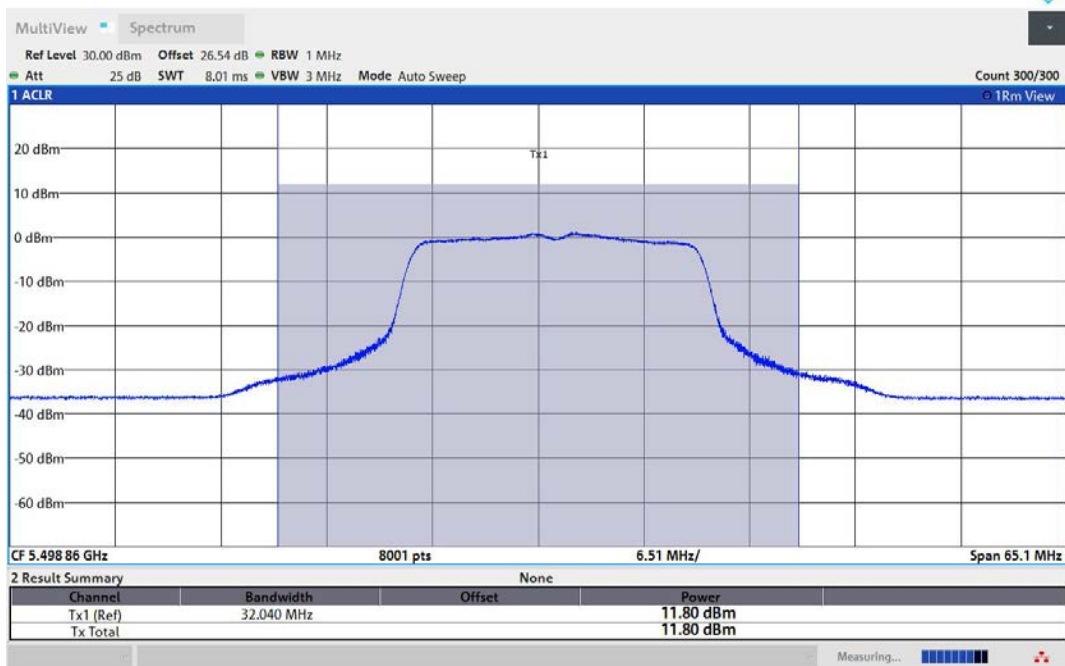
11AC20MIMO-Ant1-5500-PASS
