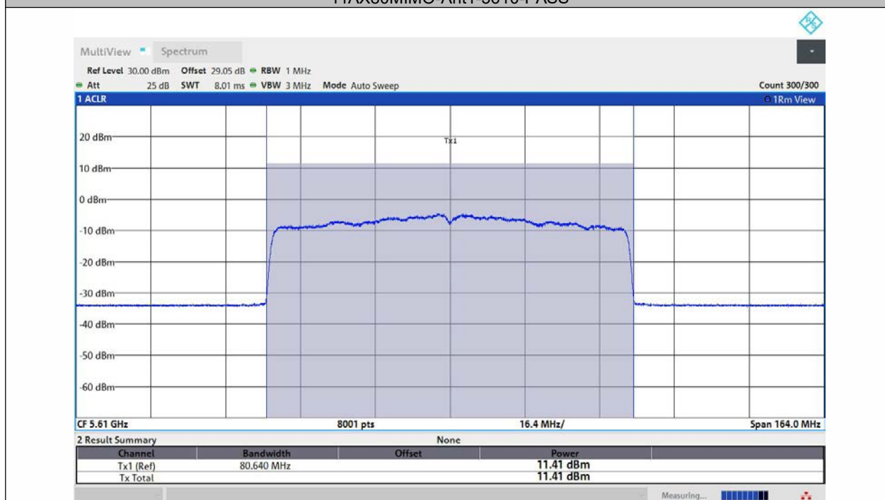
11AX80MIMO-Ant2-5610-PASS
