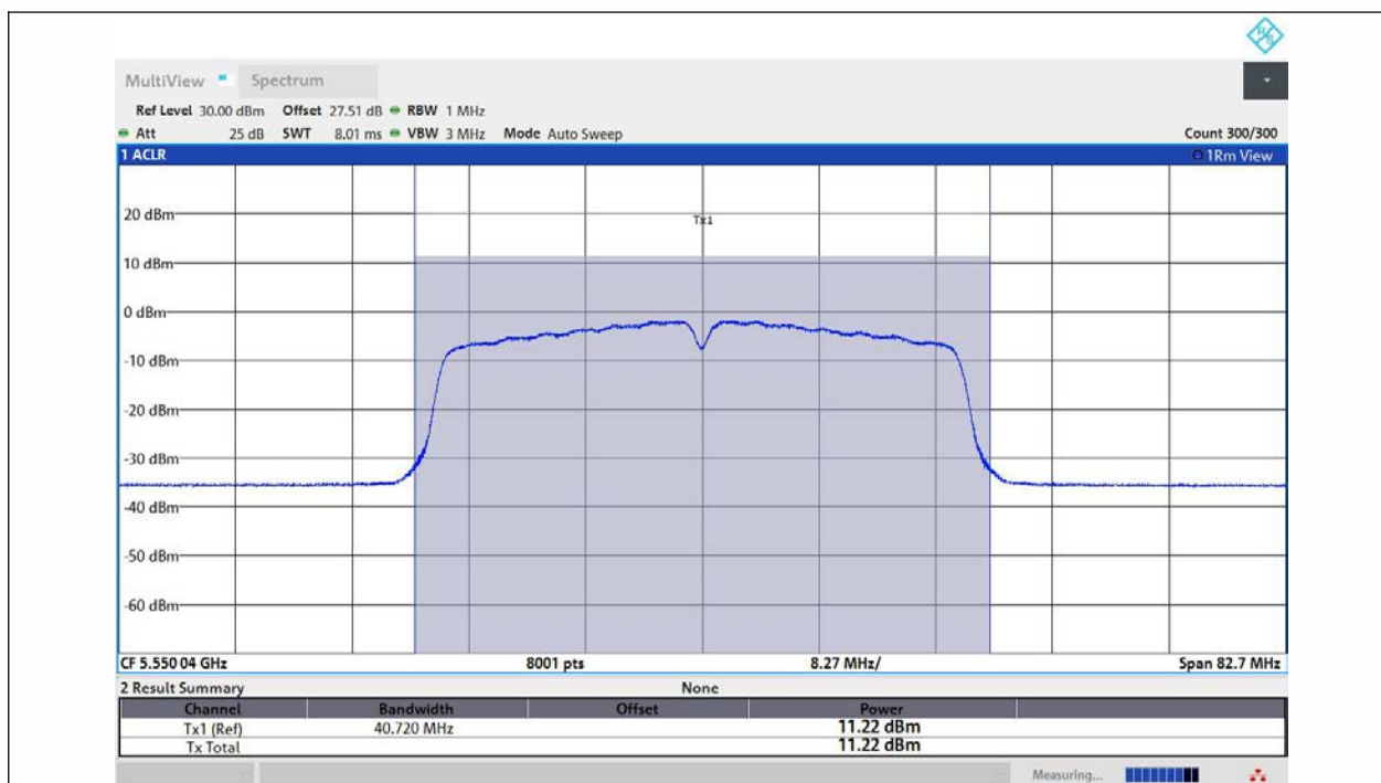
11AC40MIMO-Ant1-5550-PASS
