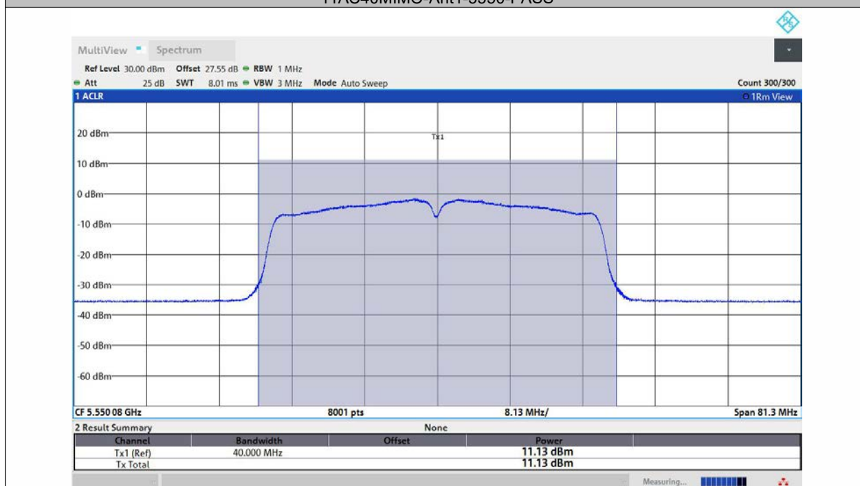
11AC40MIMO-Ant2-5550-PASS
