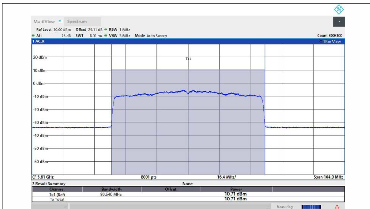
11AX80MIMO-Ant1-5610-PASS
