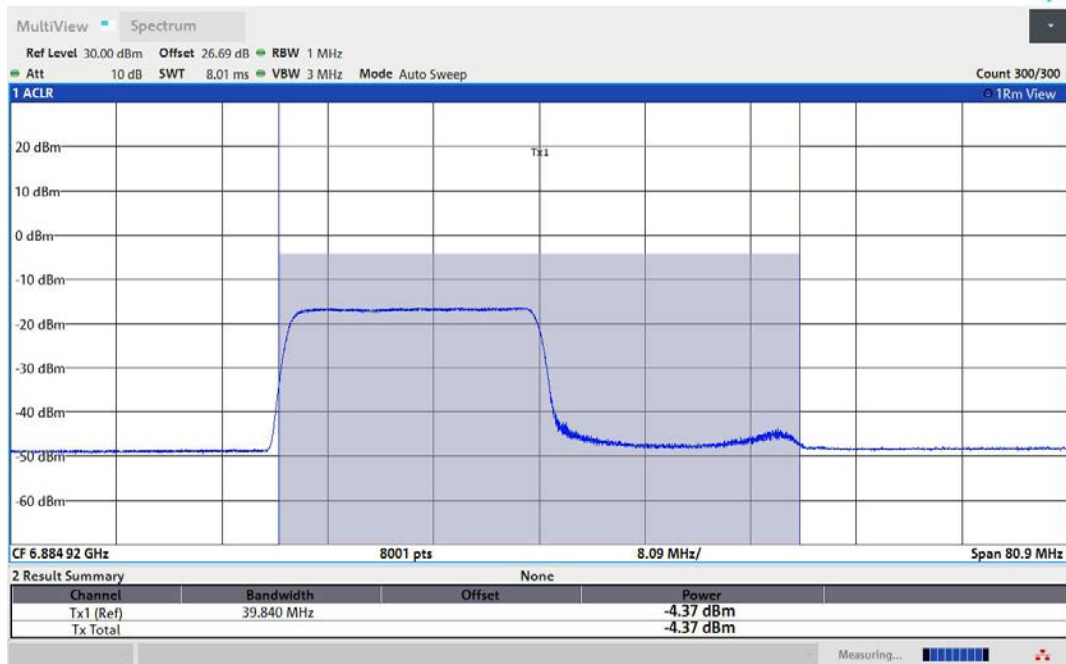
11AX40MIMO-Ant2-6885-242Tone-RU61-PASS
