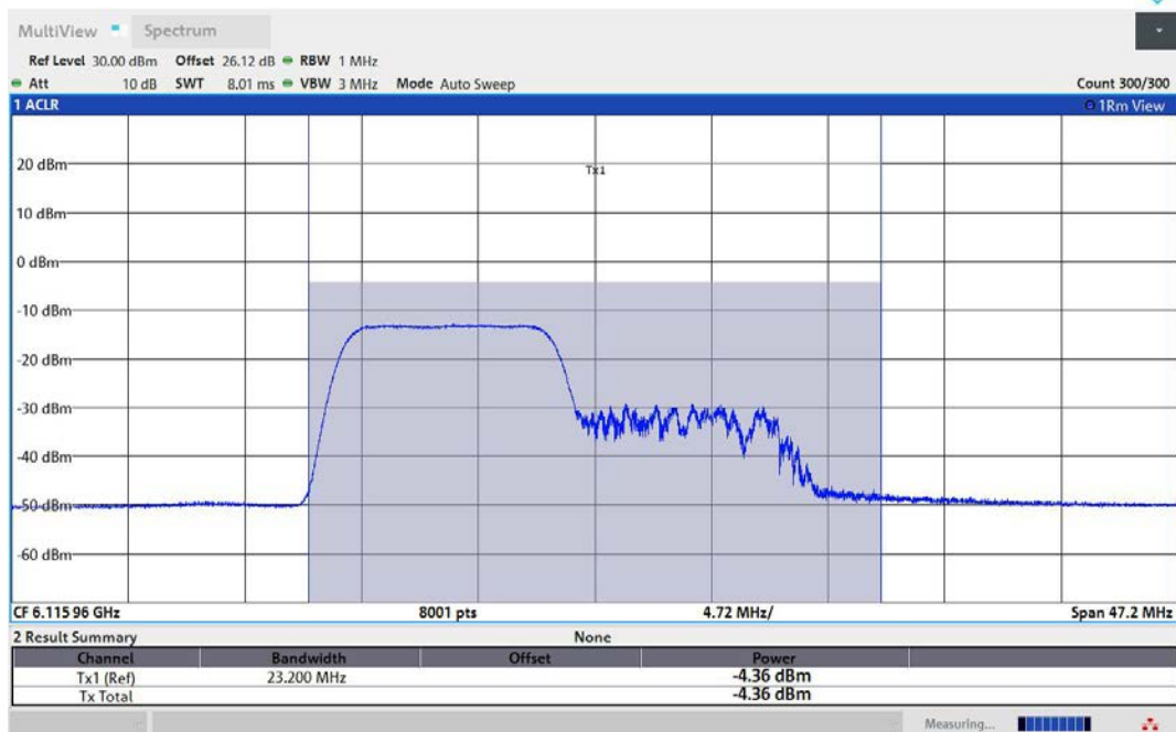
11AX80MIMO-Ant1-6145-106Tone-RU53-PASS
