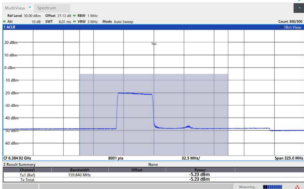
11AX80MIMO-Ant1-6385-484Tone-RU65-PASS
