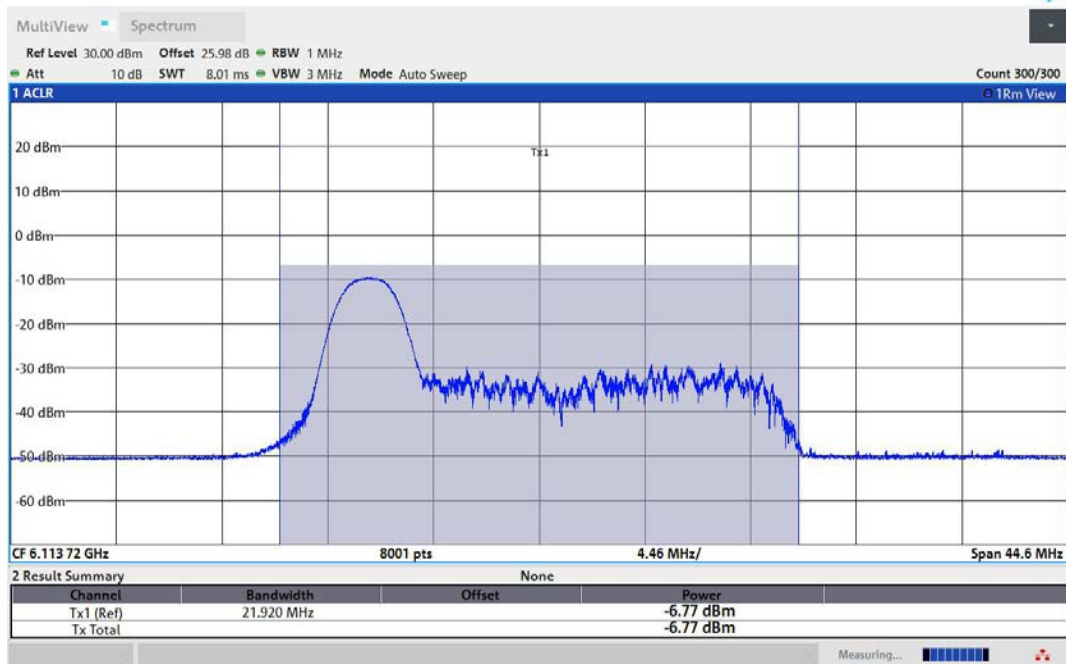
11AX80MIMO-Ant2-6145-26Tone-RU0-PASS
