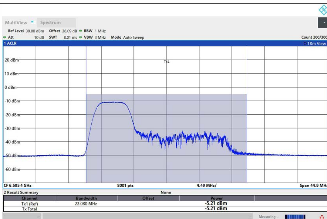
11AX80MIMO-Ant1-6625-52Tone-RU37-PASS
