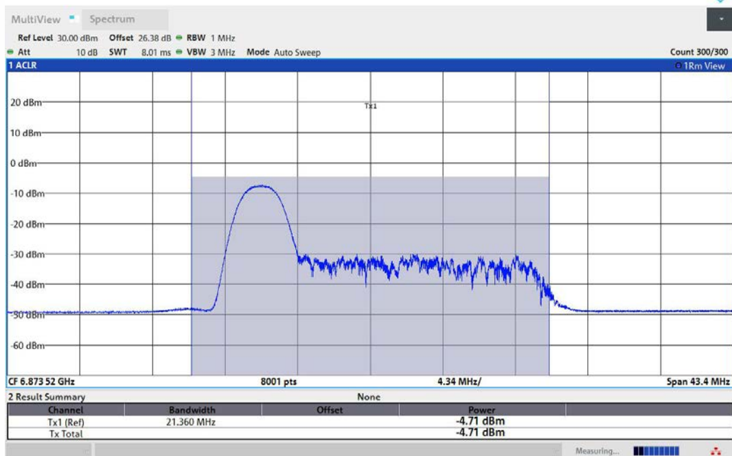
11AX40MIMO-Ant1-6885-26Tone-RU0-PASS
