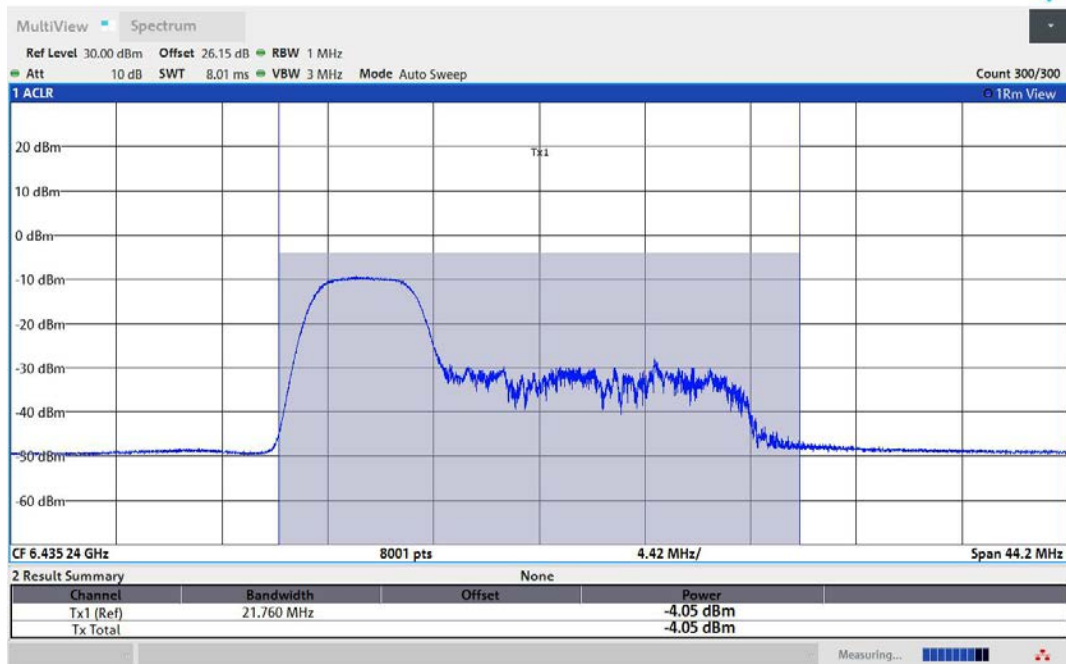
11AX80MIMO-Ant2-6465-52Tone-RU37-PASS
