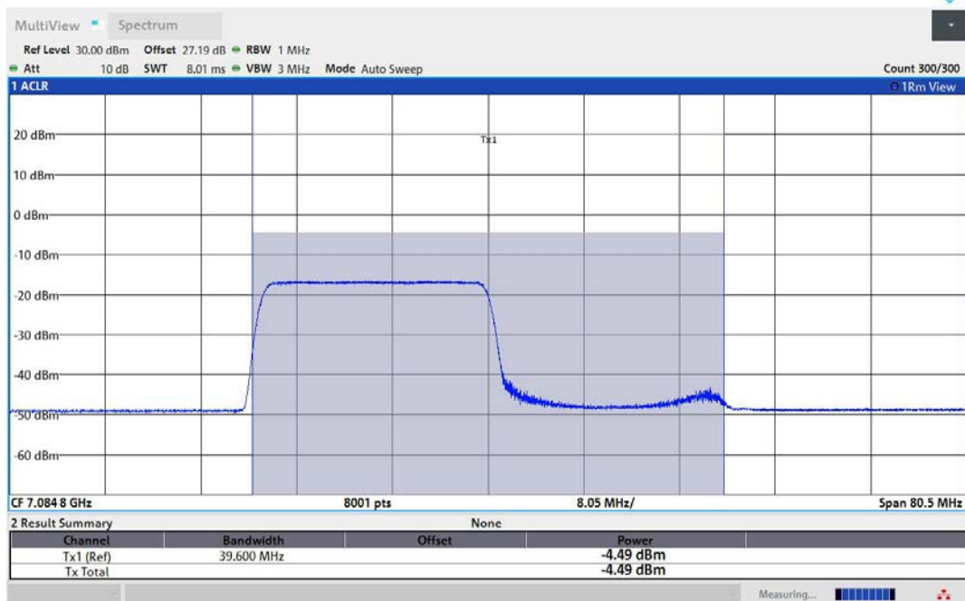
11AX40MIMO-Ant1-7085-242Tone-RU61-PASS
