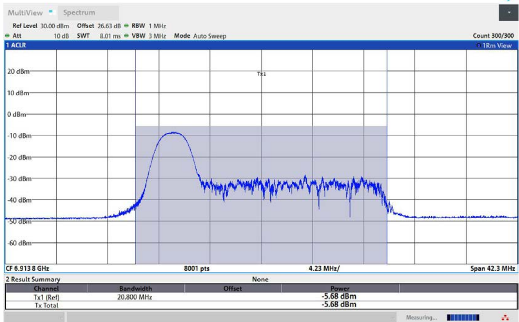
11AX40MIMO-Ant1-6925-26Tone-RU0-PASS
