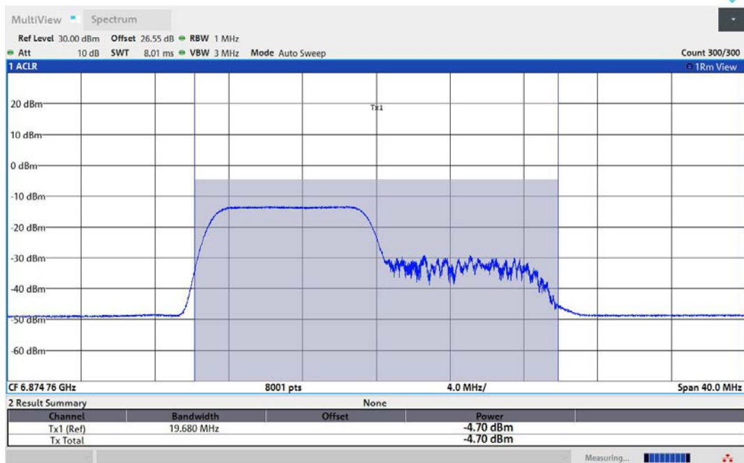
11AX40MIMO-Ant1-6885-106Tone-RU53-PASS
