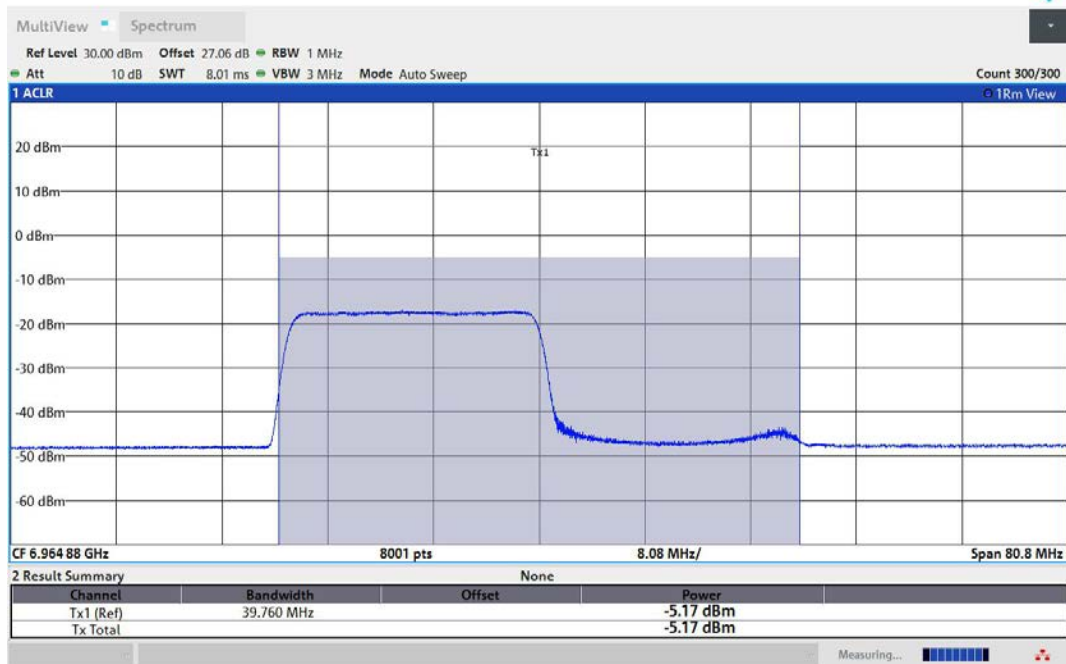
11AX40MIMO-Ant2-6965-242Tone-RU61-PASS
