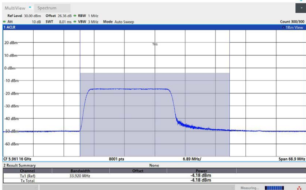
11AX80MIMO-Ant1-5985-242Tone-RU61-PASS
