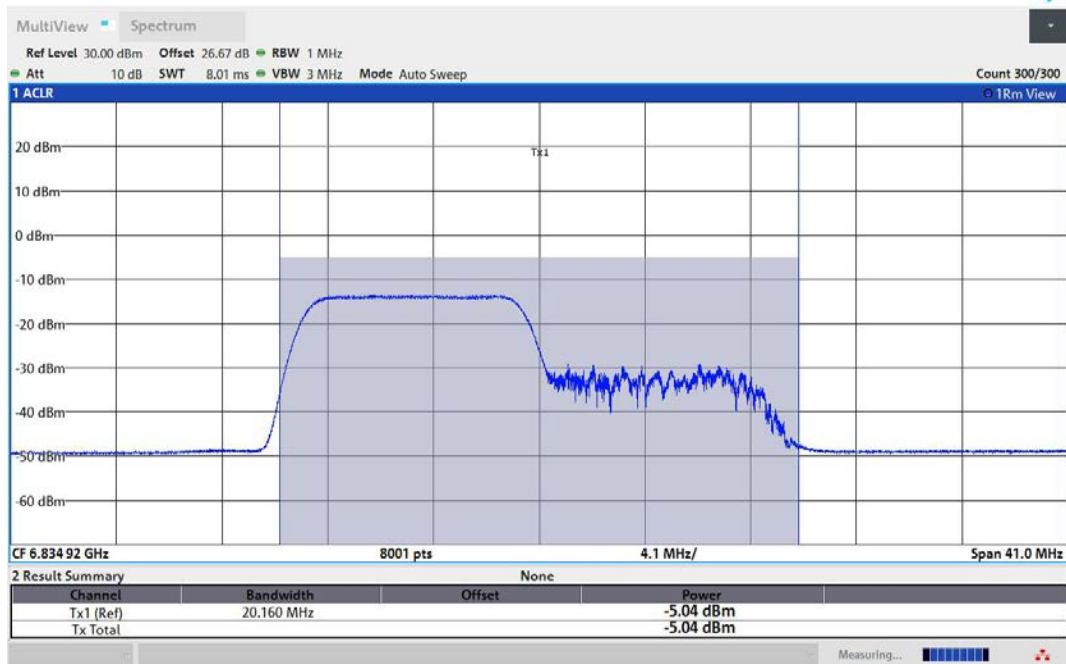
11AX40MIMO-Ant2-6845-106Tone-RU53-PASS
