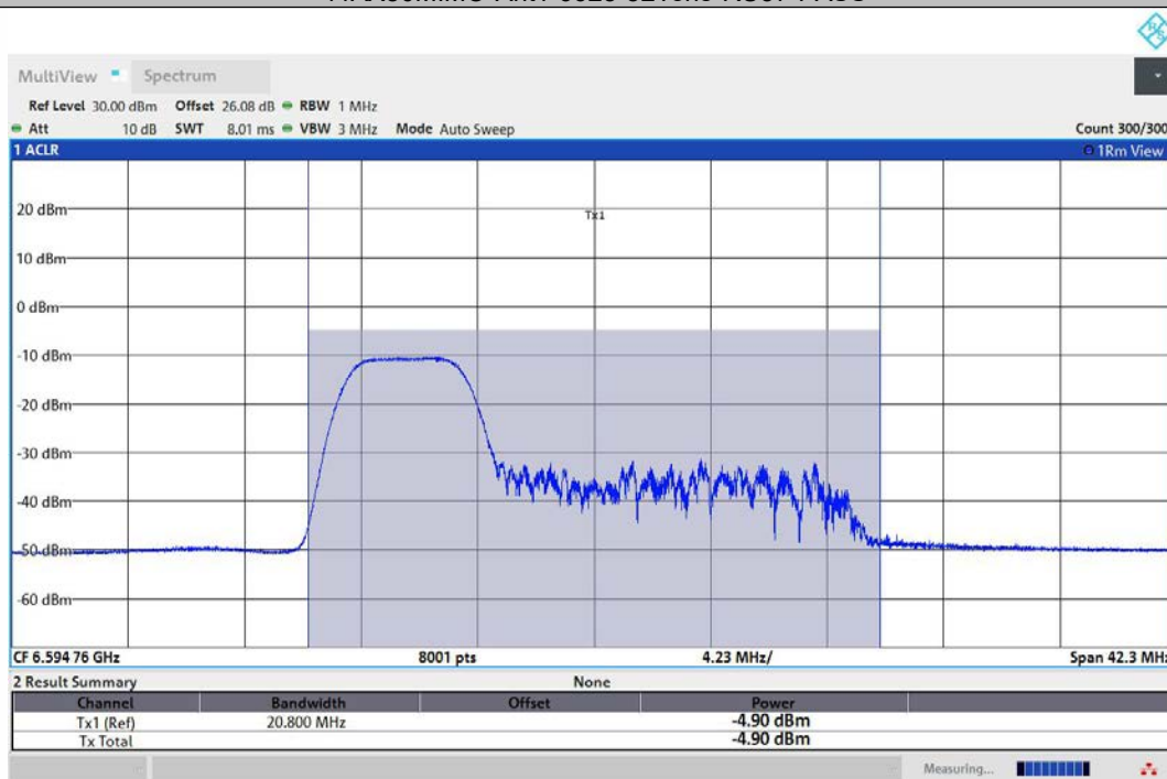
11AX80MIMO-Ant2-6625-52Tone-RU37-PASS
