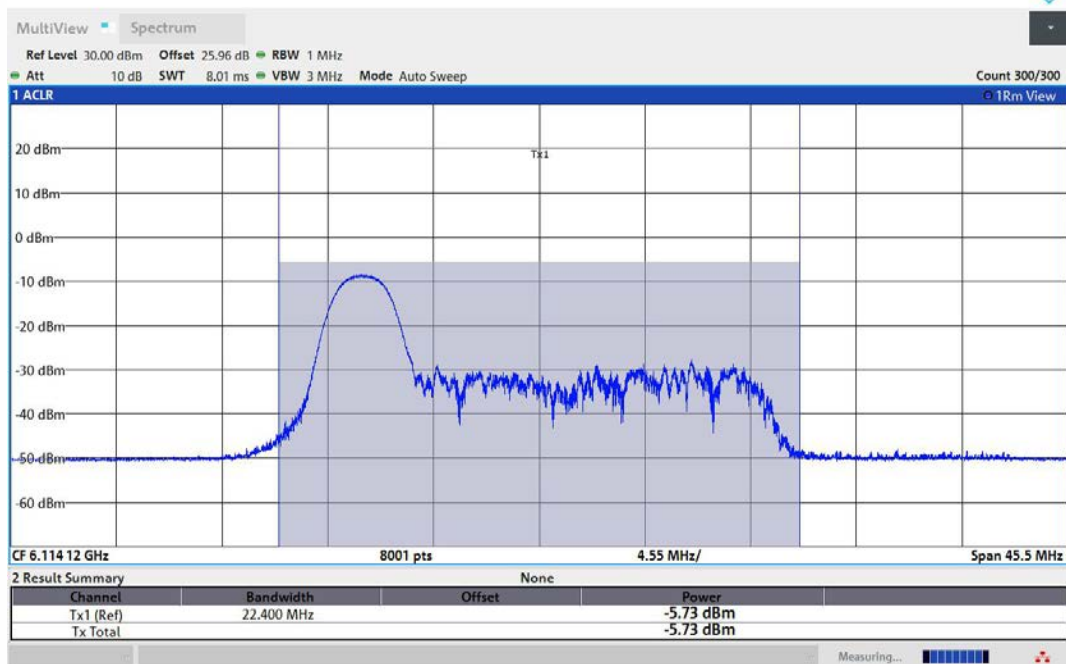
11AX80MIMO-Ant1-6145-26Tone-RU0-PASS
