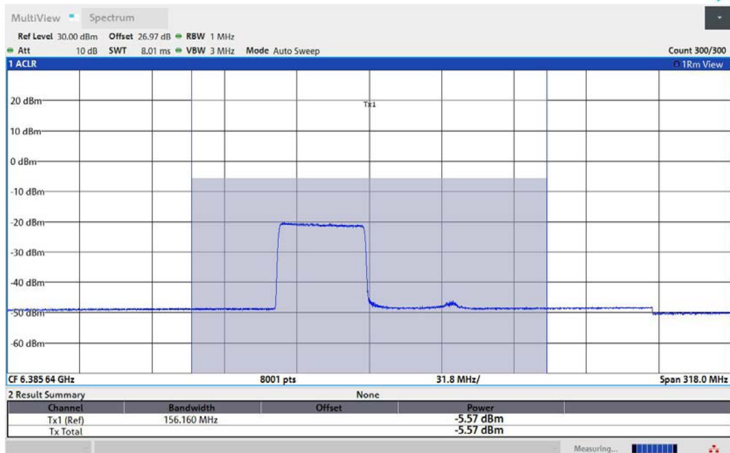
11AX80MIMO-Ant2-6385-484Tone-RU65-PASS
