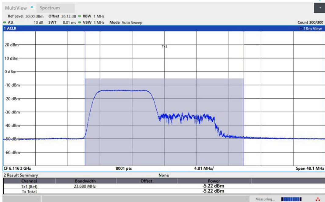
11AX80MIMO-Ant2-6145-106Tone-RU53-PASS
