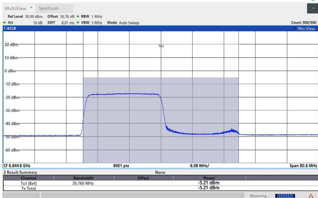
11AX40MIMO-Ant1-6845-242Tone-RU61-PASS
