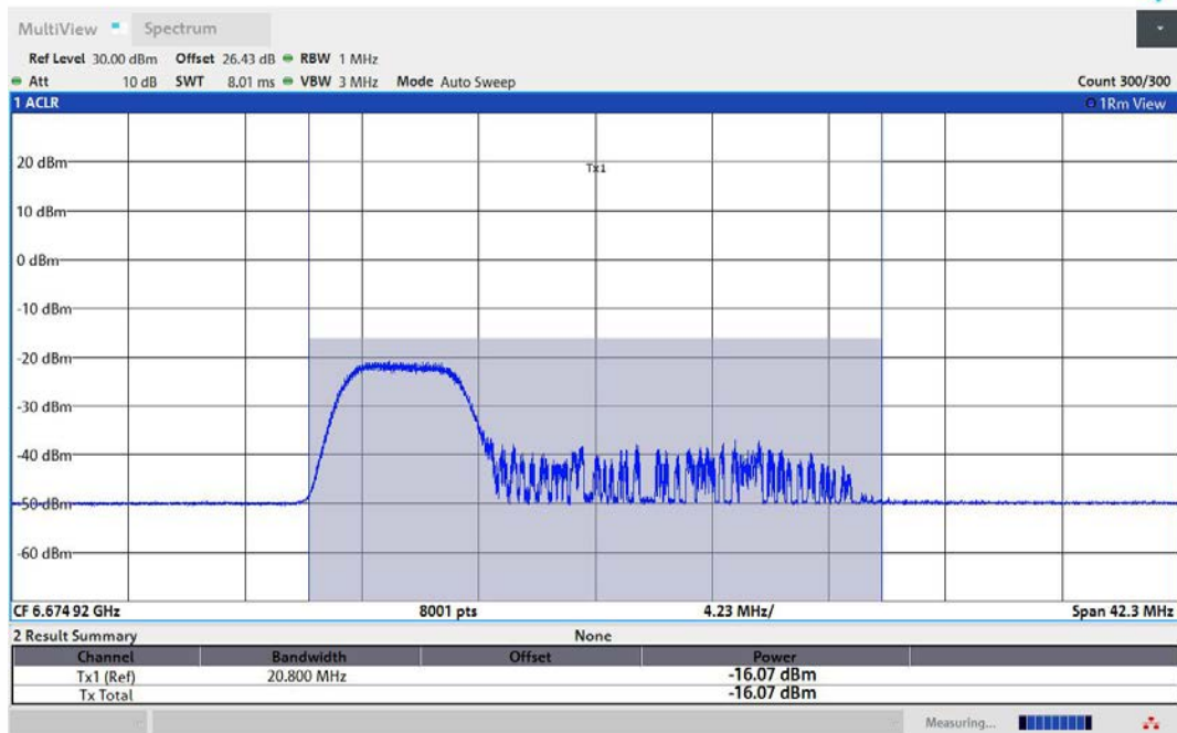
11AX80MIMO-Ant2-6705-52Tone-RU37-PASS
