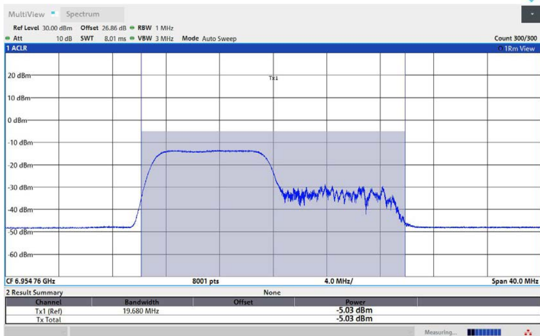
11AX40MIMO-Ant1-6965-106Tone-RU53-PASS
