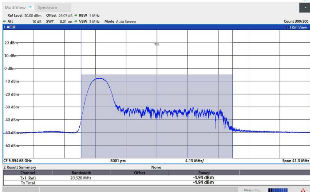
11AX80MIMO-Ant2-5985-26Tone-RU0-PASS
