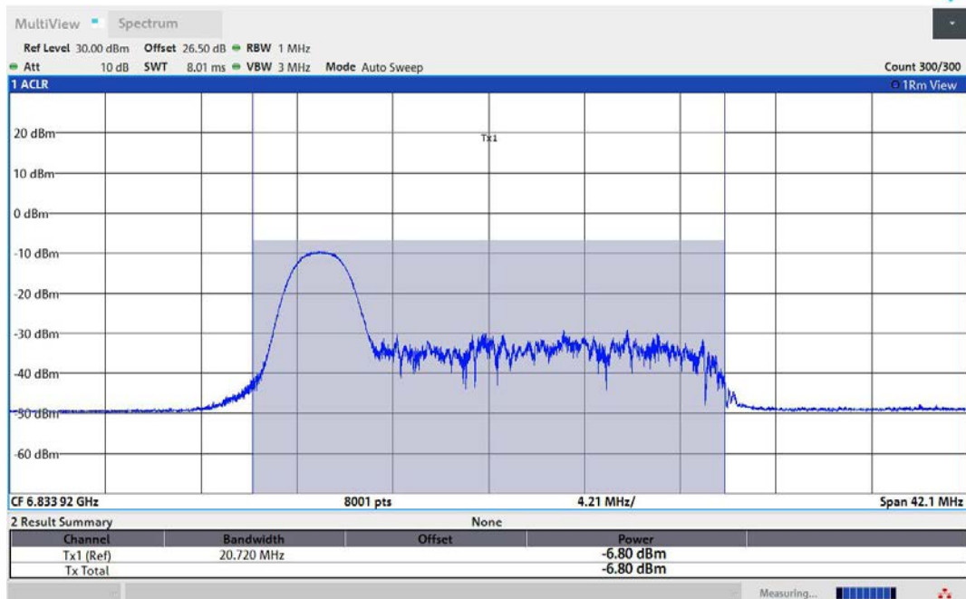
11AX40MIMO-Ant2-6845-26Tone-RU0-PASS
