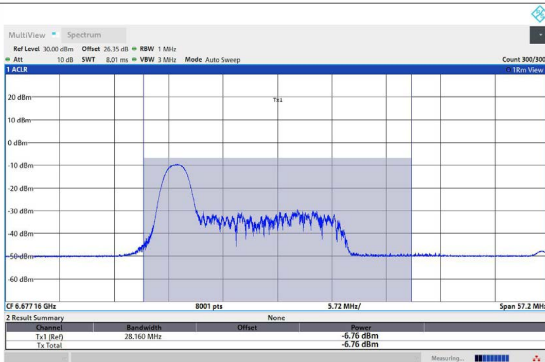
11AX80MIMO-Ant1-6705-26Tone-RU0-PASS
