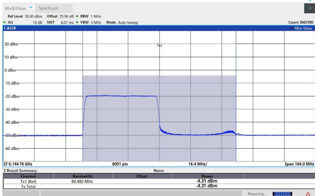
11AX80MIMO-Ant1-6145-484Tone-RU65-PASS
