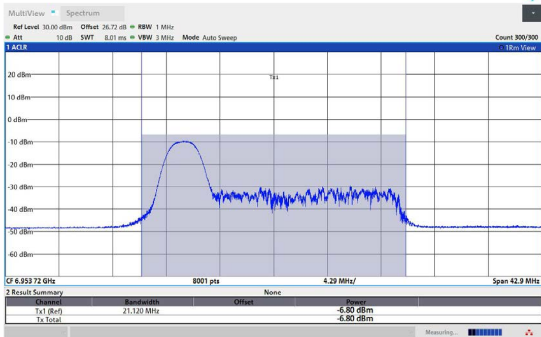
11AX40MIMO-Ant2-6965-26Tone-RU0-PASS
