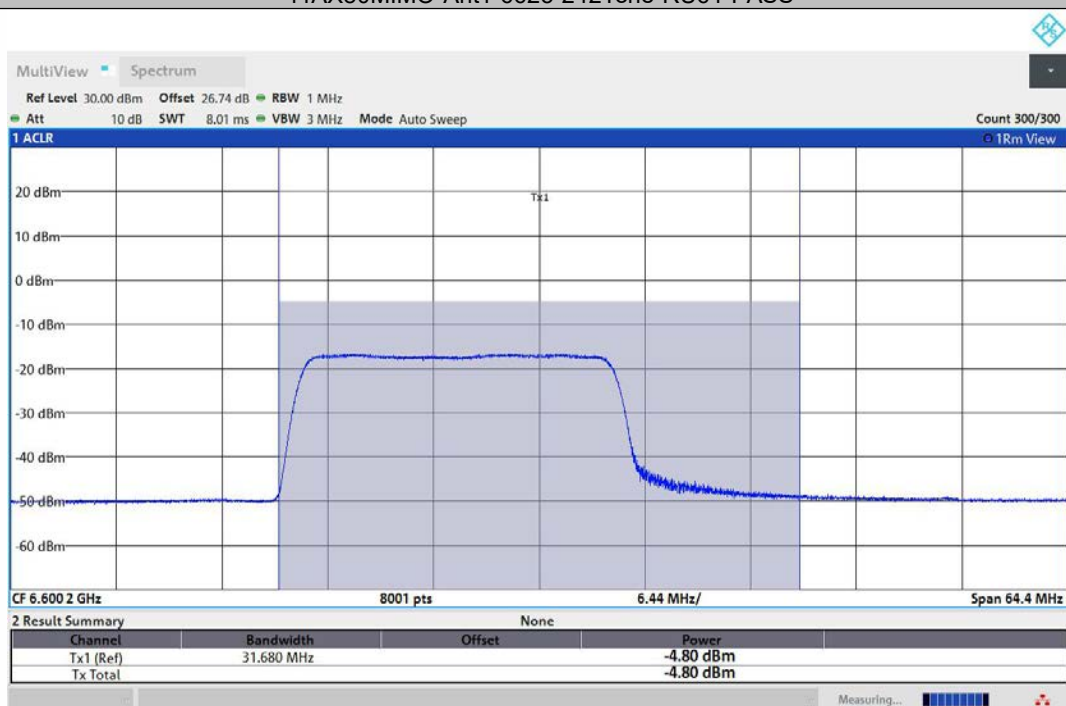
11AX80MIMO-Ant2-6625-242Tone-RU61-PASS
