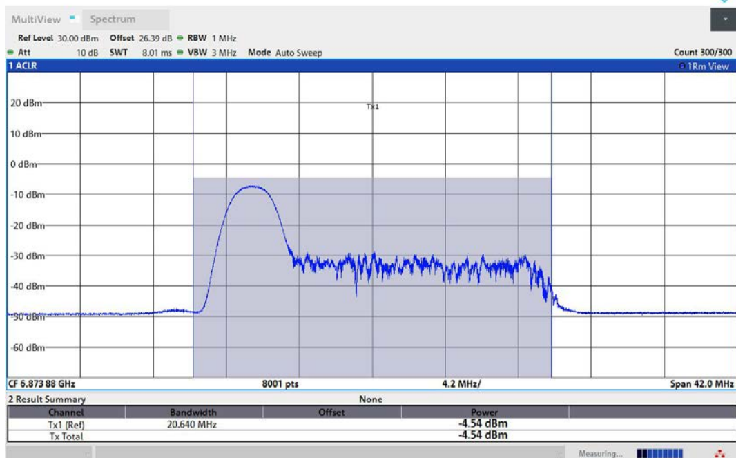
11AX40MIMO-Ant2-6885-26Tone-RU0-PASS
