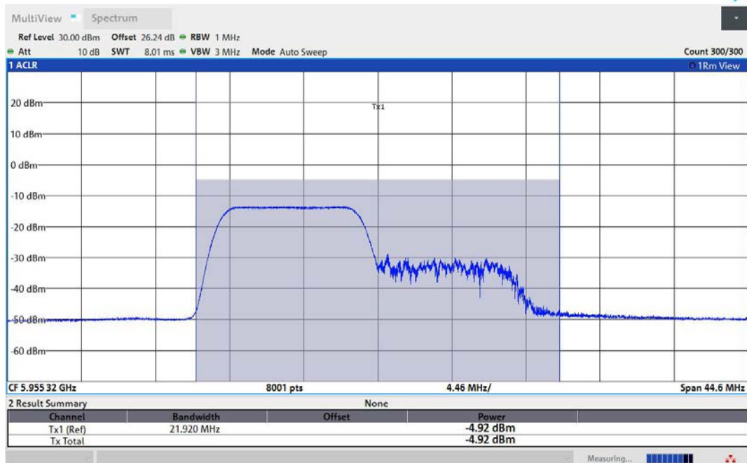
11AX80MIMO-Ant2-5985-106Tone-RU53-PASS
