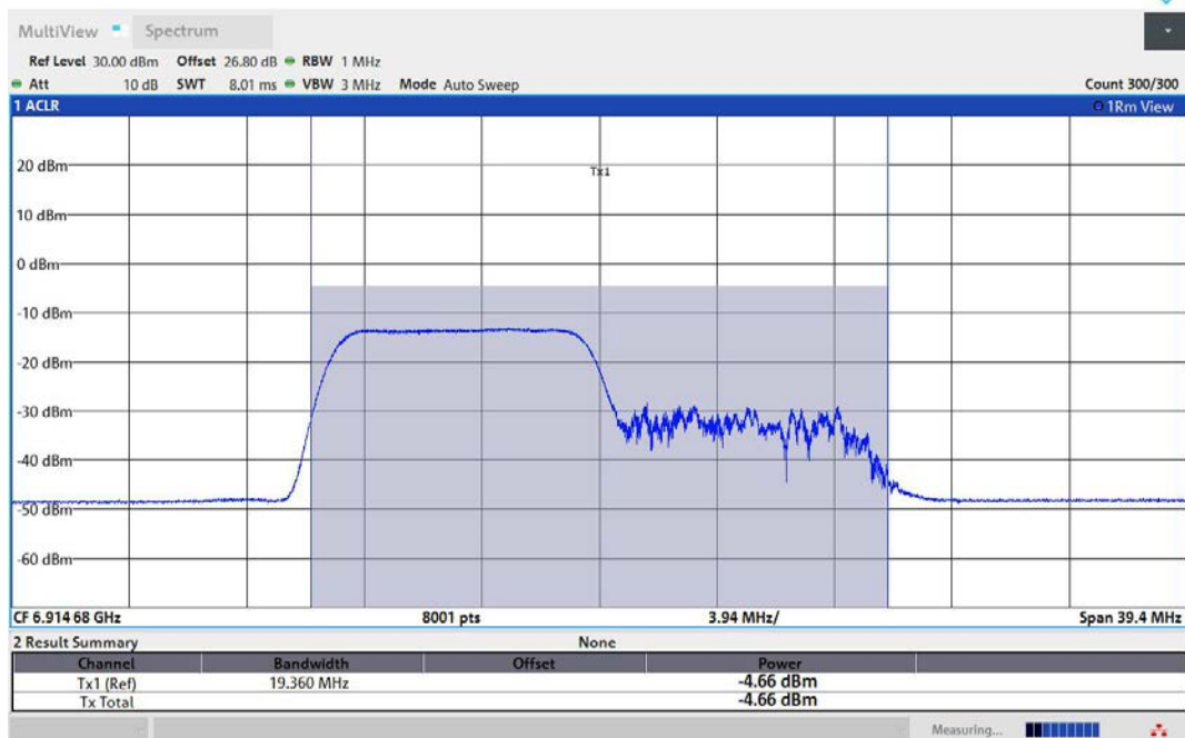
11AX40MIMO-Ant1-6925-106Tone-RU53-PASS
