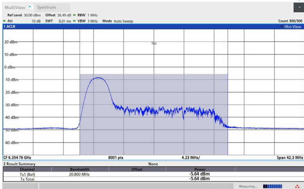
11AX80MIMO-Ant2-6385-26Tone-RU0-PASS
