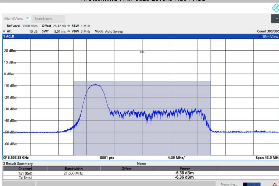
11AX80MIMO-Ant2-6625-26Tone-RU0-PASS
