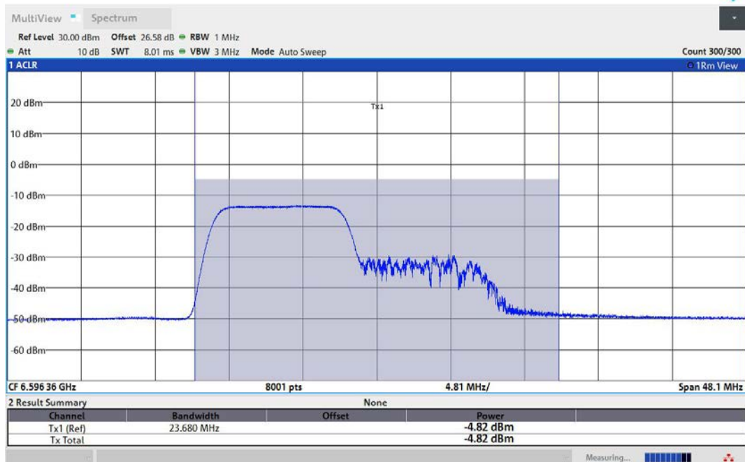
11AX80MIMO-Ant2-6625-106Tone-RU53-PASS
