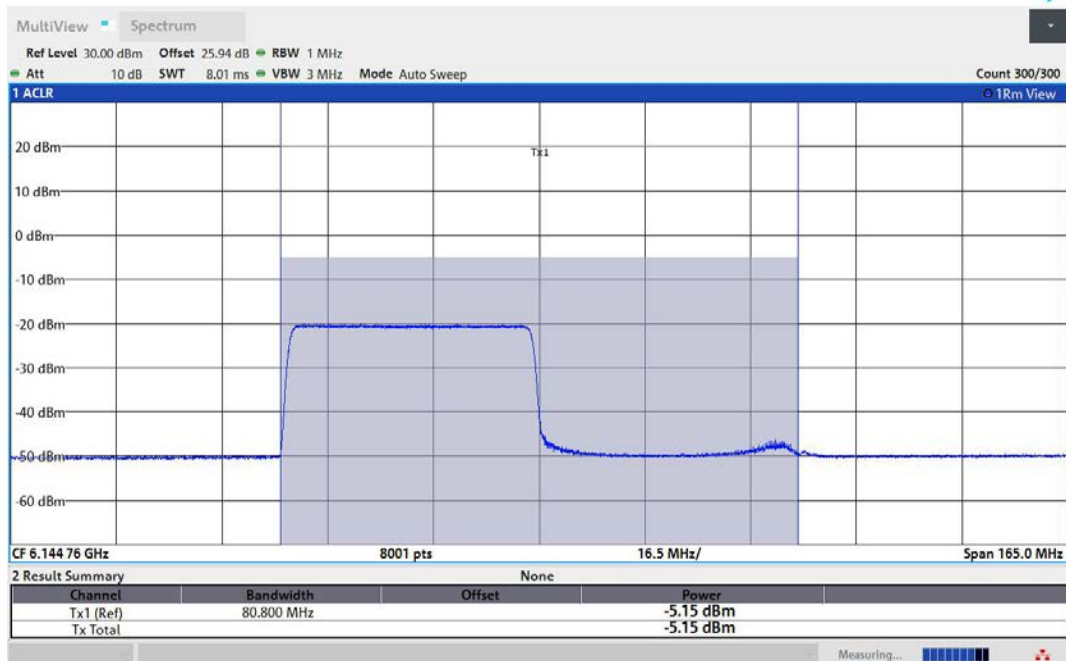
11AX80MIMO-Ant2-6145-484Tone-RU65-PASS
