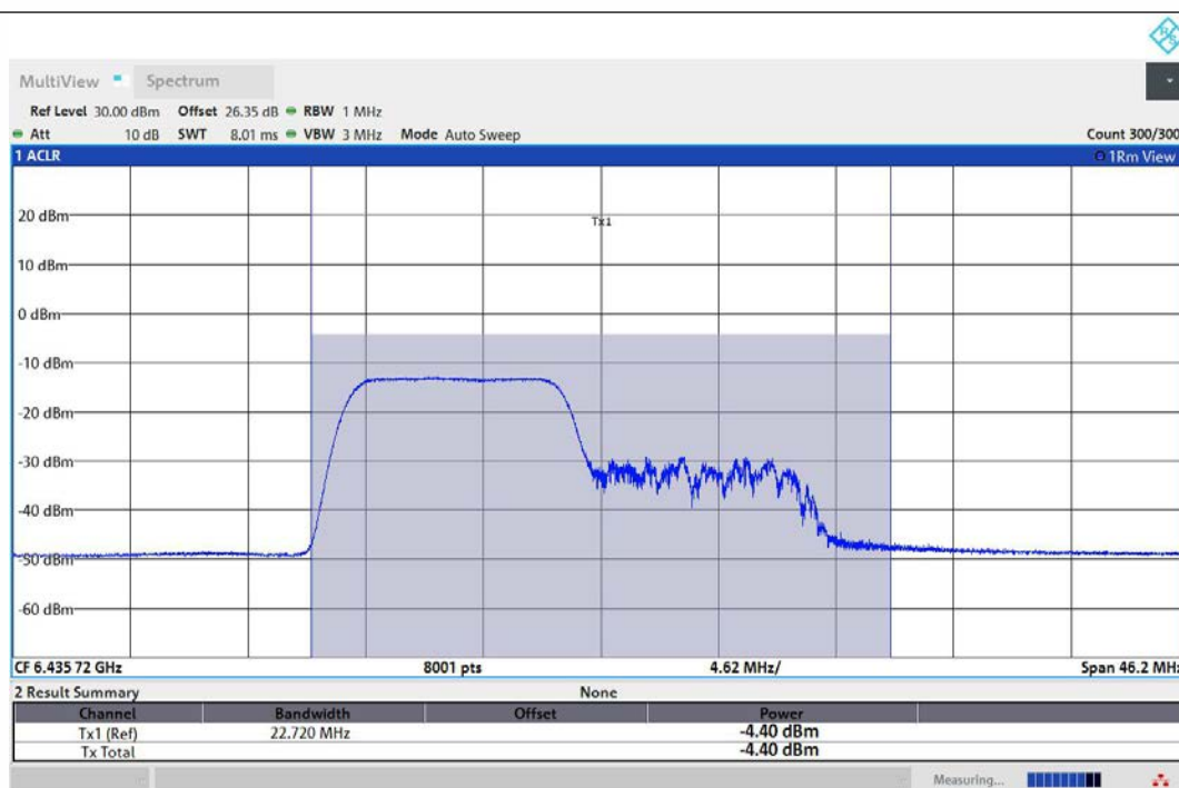
11AX80MIMO-Ant1-6465-106Tone-RU53-PASS
