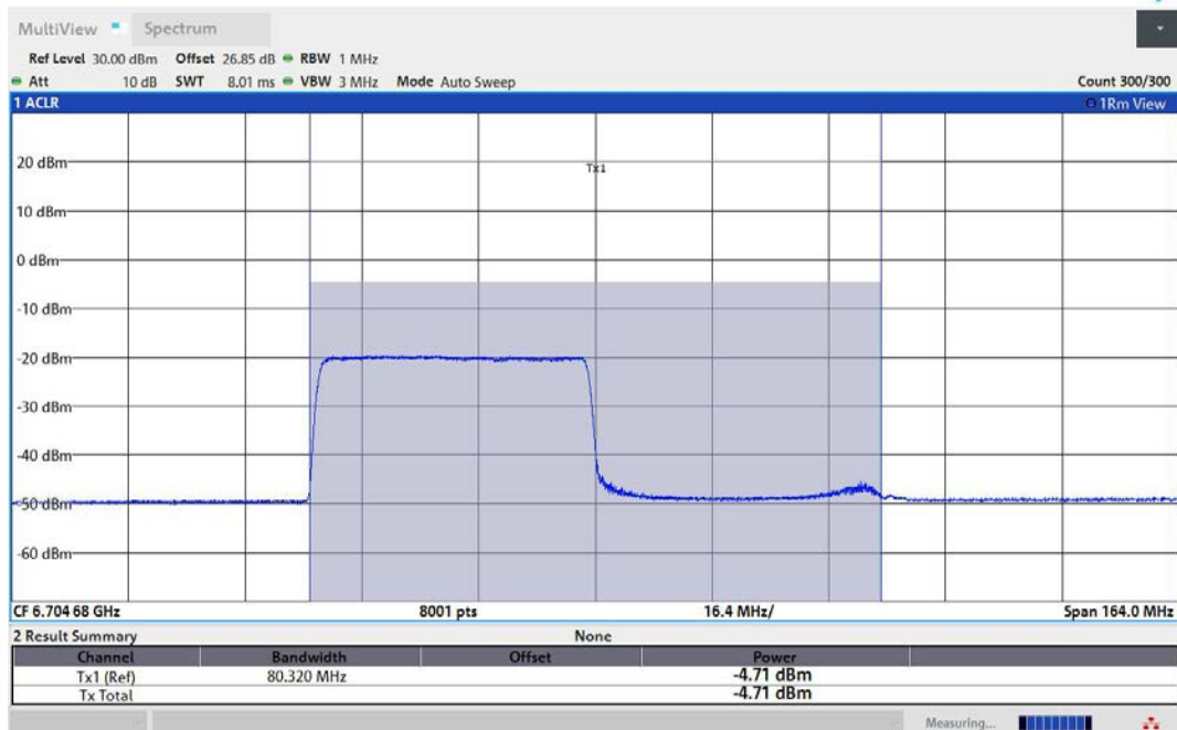
11AX80MIMO-Ant2-6705-484Tone-RU65-PASS
