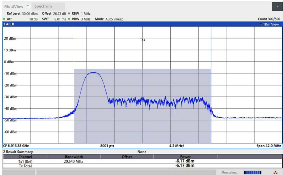
11AX40MIMO-Ant2-6925-26Tone-RU0-PASS
