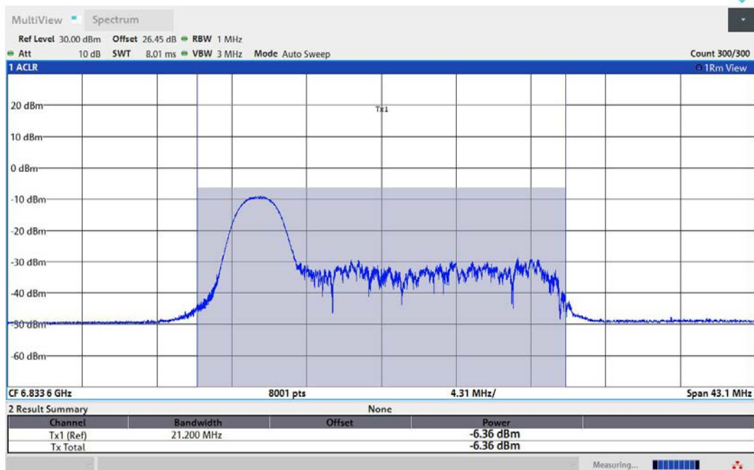
11AX40MIMO-Ant1-6845-26Tone-RU0-PASS
