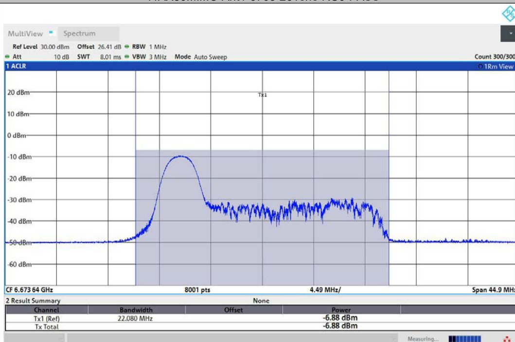
11AX80MIMO-Ant2-6705-26Tone-RU0-PASS
