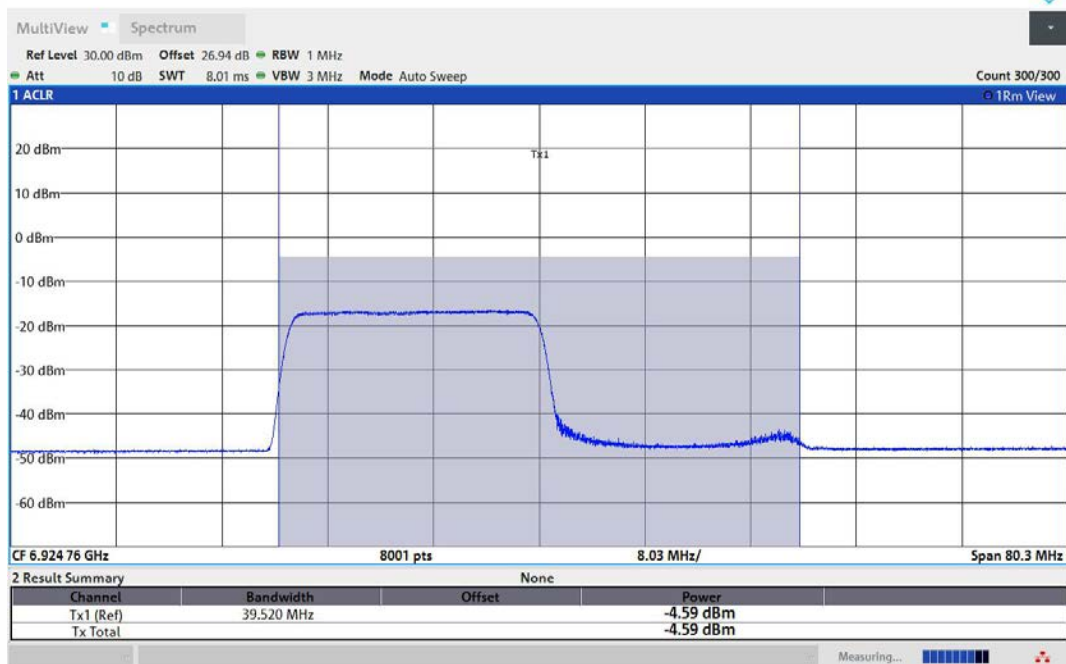
11AX40MIMO-Ant1-6925-242Tone-RU61-PASS
