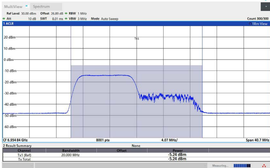
11AX40MIMO-Ant2-6965-106Tone-RU53-PASS
