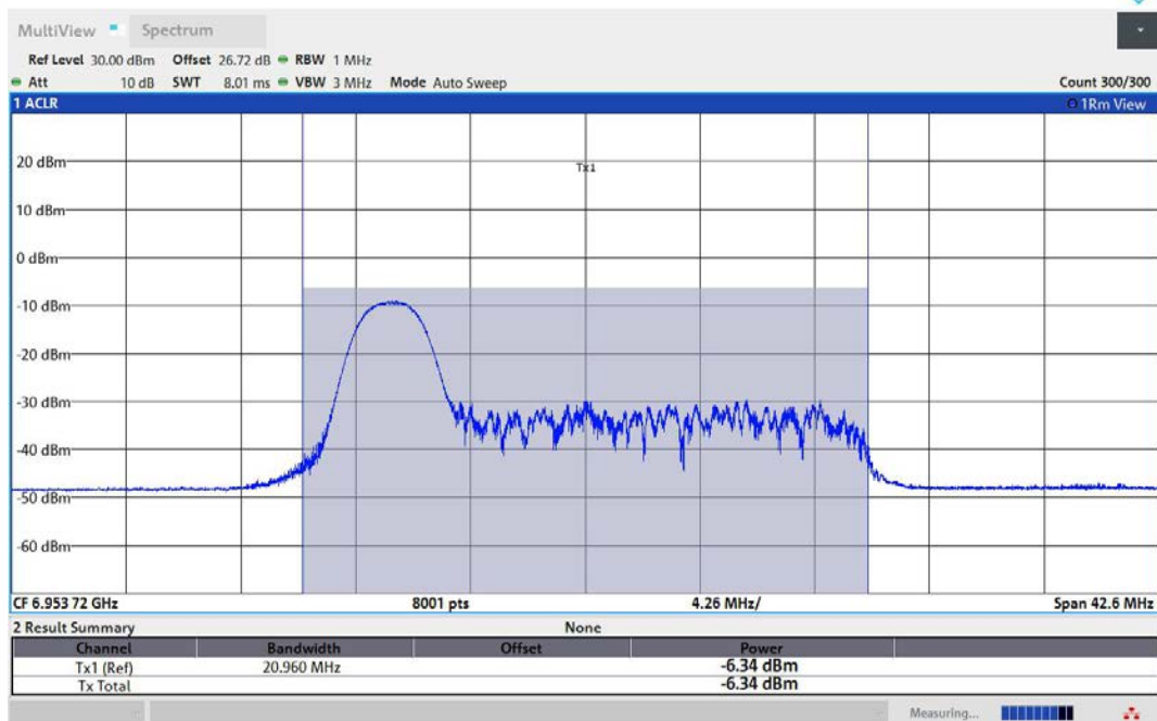
11AX40MIMO-Ant1-6965-26Tone-RU0-PASS
