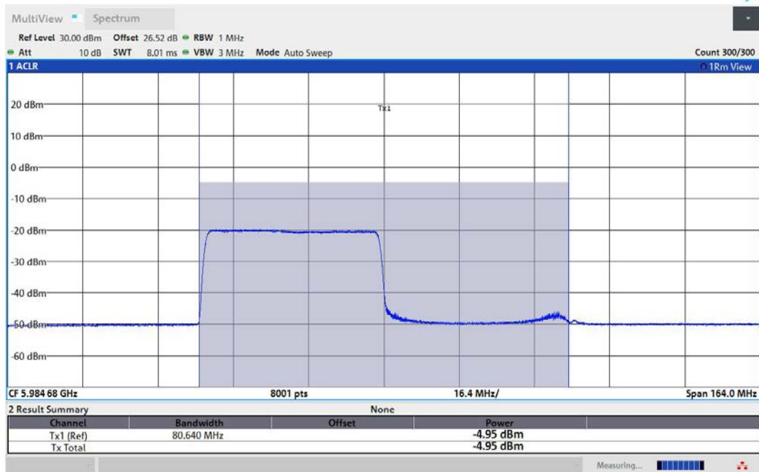
11AX80MIMO-Ant2-5985-484Tone-RU65-PASS
