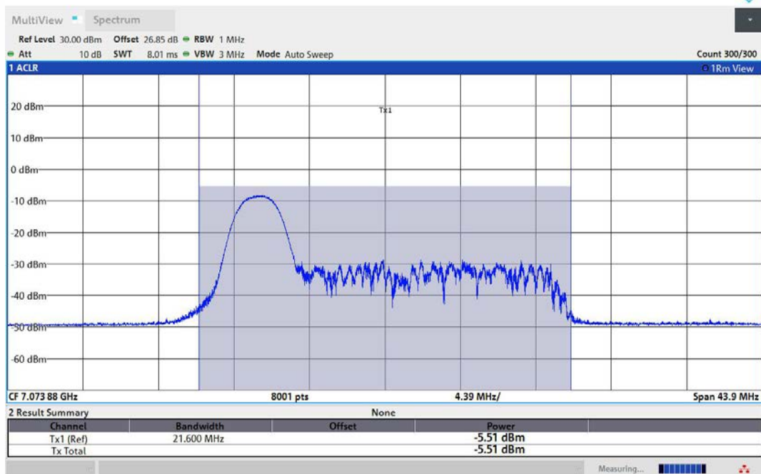
11AX40MIMO-Ant1-7085-26Tone-RU0-PASS
