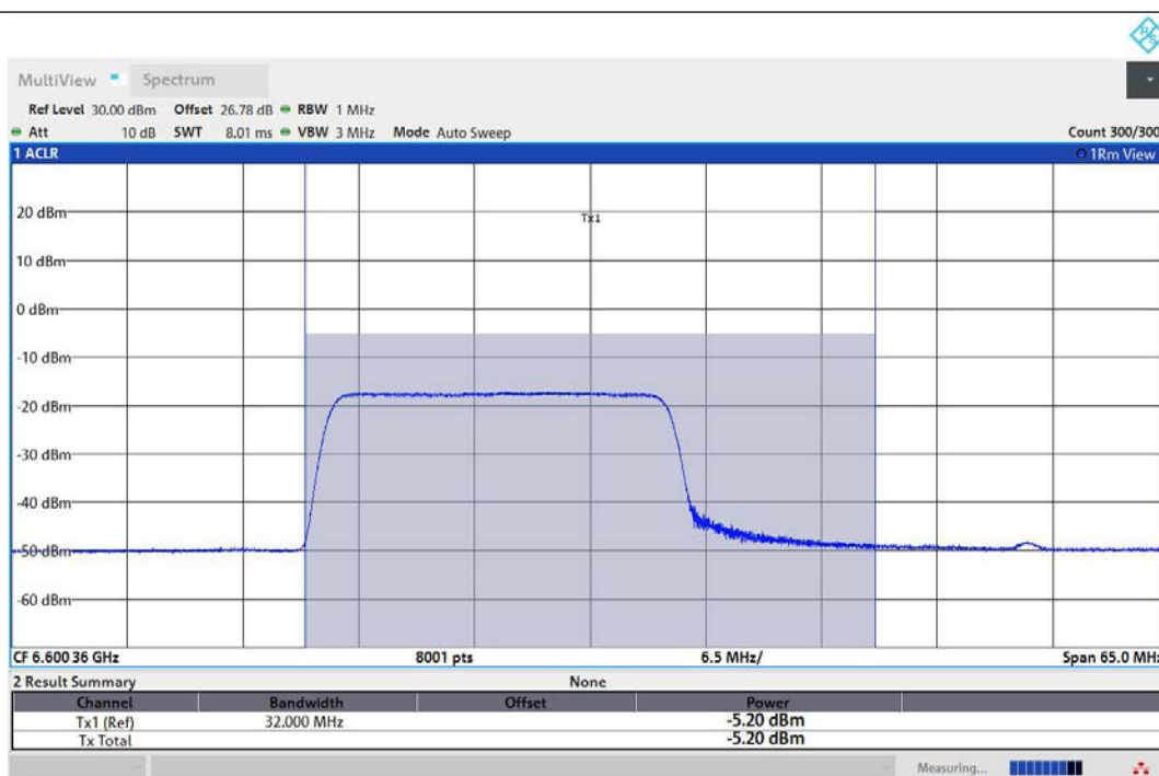
11AX80MIMO-Ant1-6625-242Tone-RU61-PASS
