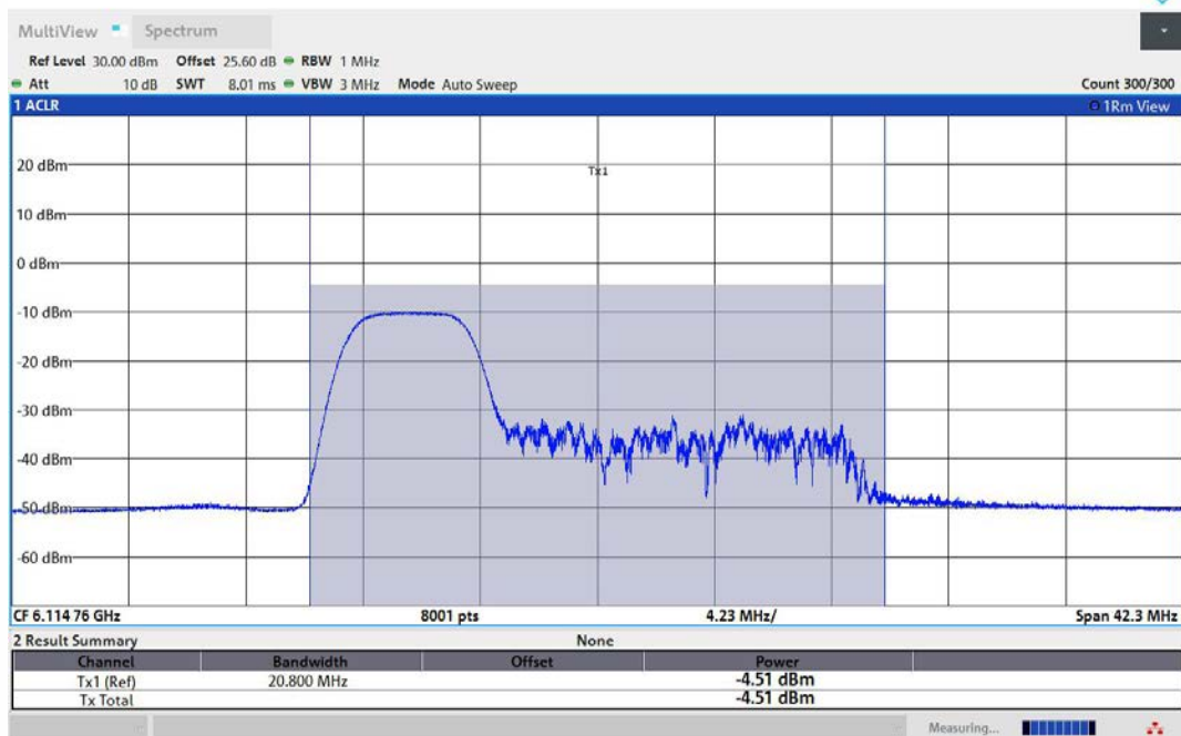
11AX80MIMO-Ant1-6145-52Tone-RU37-PASS
