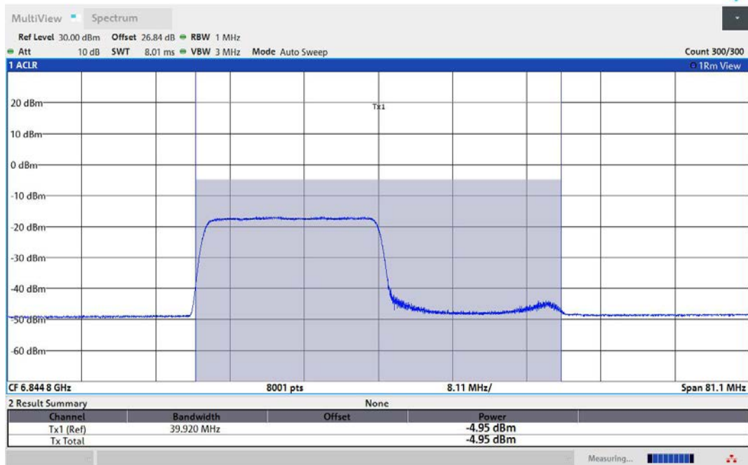
11AX40MIMO-Ant2-6845-242Tone-RU61-PASS
