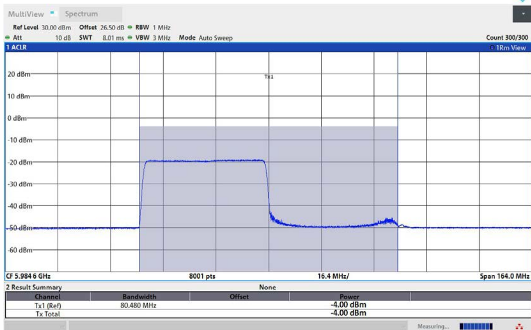
11AX80MIMO-Ant1-5985-484Tone-RU65-PASS
