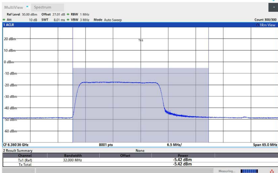
11AX80MIMO-Ant1-6385-242Tone-RU61-PASS
