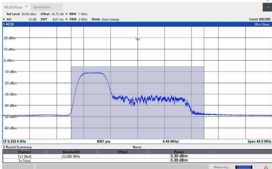
11AX80MIMO-Ant1-6385-52Tone-RU37-PASS
