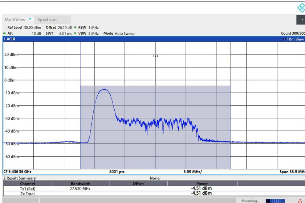
11AX80MIMO-Ant1-6465-26Tone-RU0-PASS
