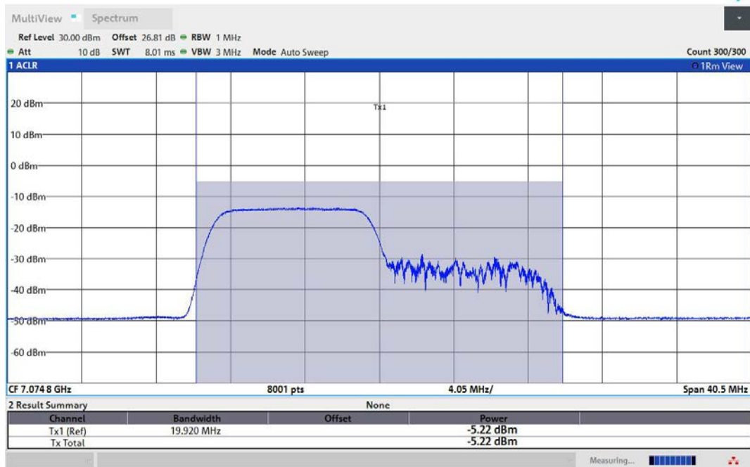
11AX40MIMO-Ant2-7085-106Tone-RU53-PASS
