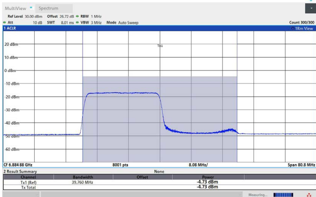
11AX40MIMO-Ant1-6885-242Tone-RU61-PASS
