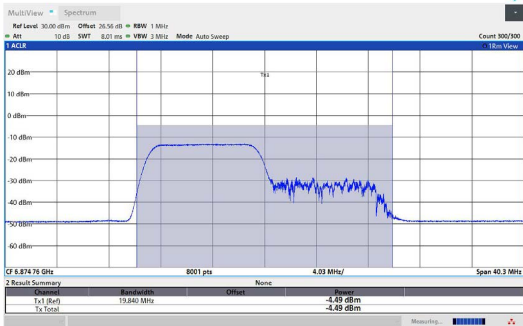
11AX40MIMO-Ant2-6885-106Tone-RU53-PASS
