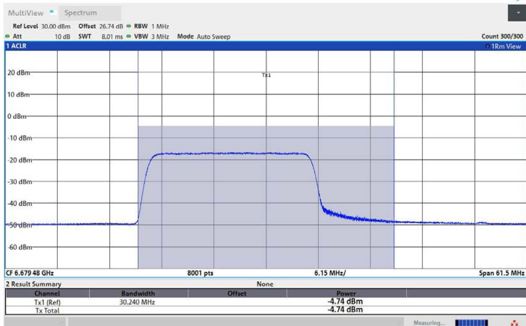
11AX80MIMO-Ant2-6705-242Tone-RU61-PASS
