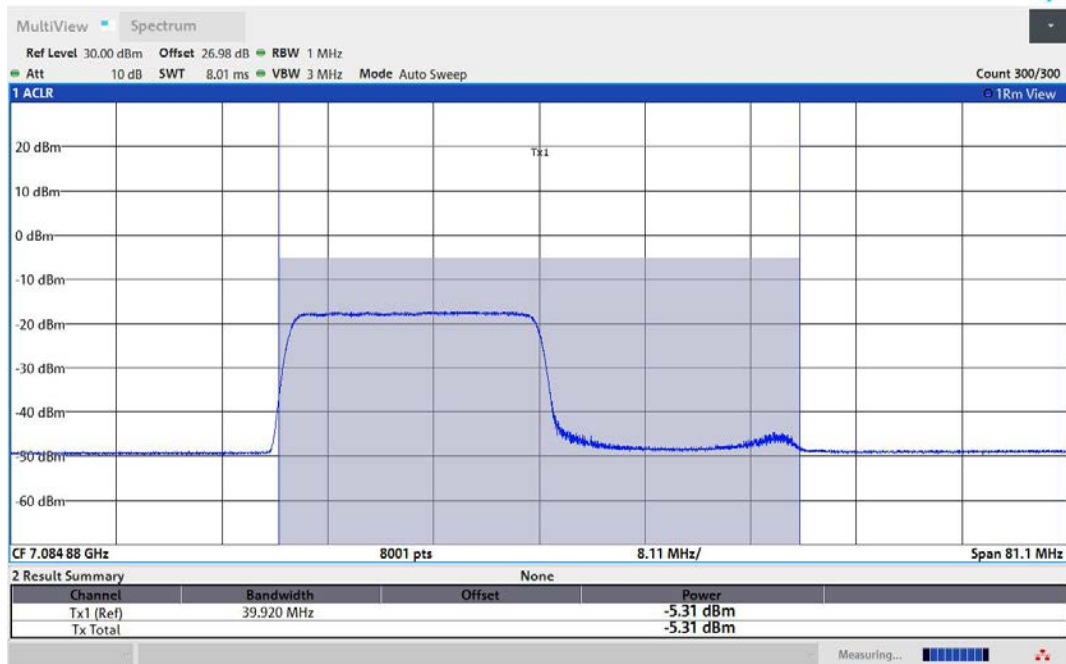
11AX40MIMO-Ant2-7085-242Tone-RU61-PASS
