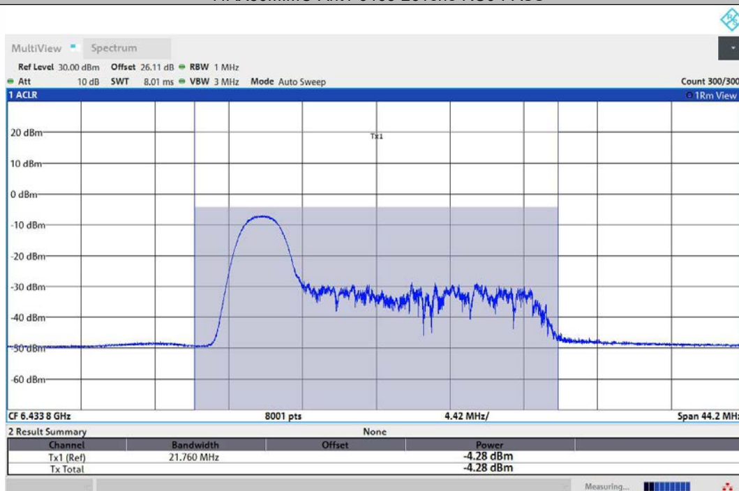
11AX80MIMO-Ant2-6465-26Tone-RU0-PASS
