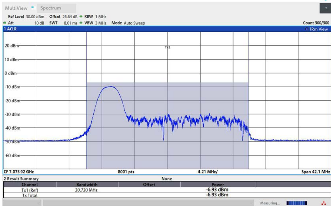
11AX40MIMO-Ant2-7085-26Tone-RU0-PASS
