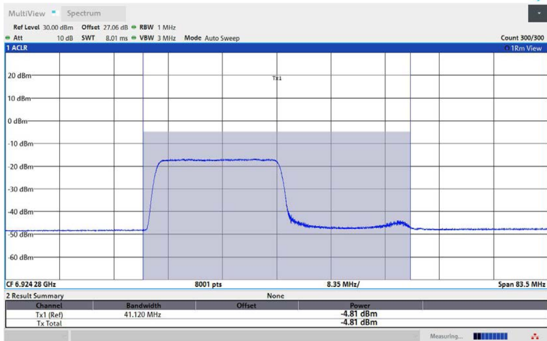
11AX40MIMO-Ant2-6925-242Tone-RU61-PASS
