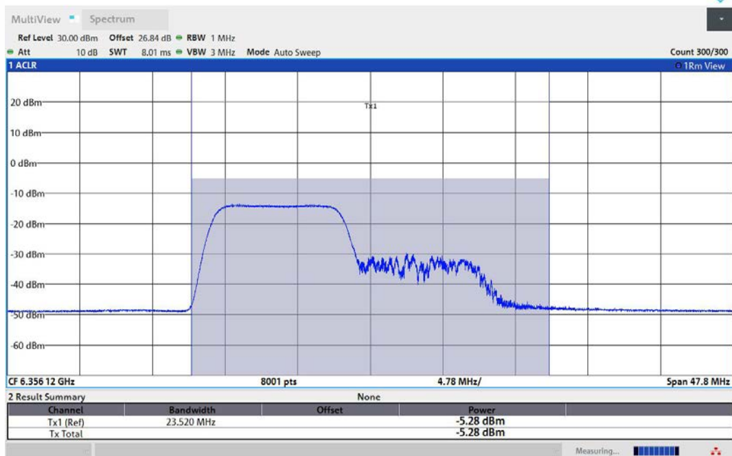
11AX80MIMO-Ant1-6385-106Tone-RU53-PASS
