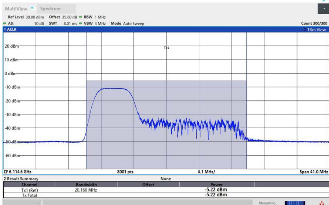
11AX80MIMO-Ant2-6145-52Tone-RU37-PASS
