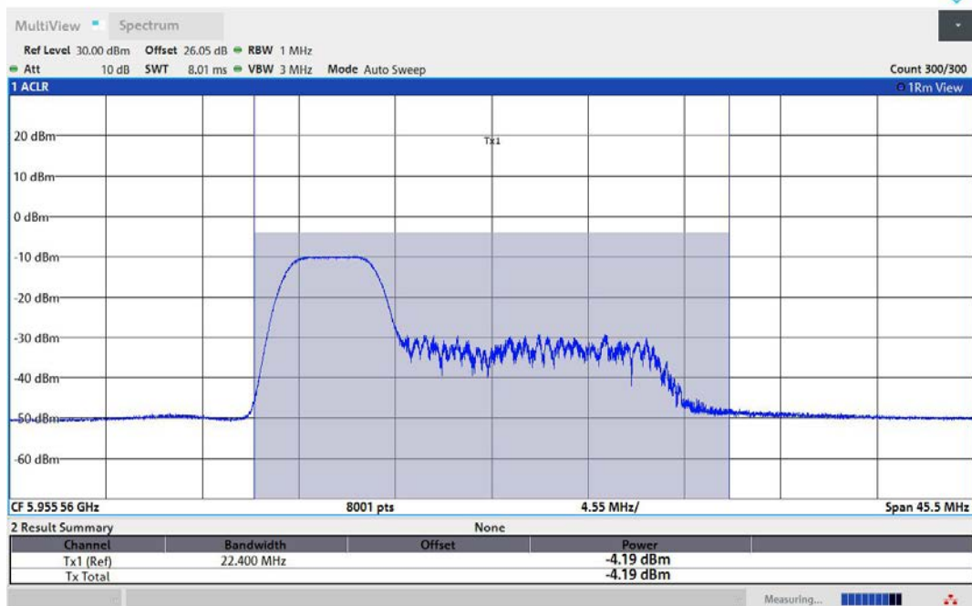
11AX80MIMO-Ant1-5985-52Tone-RU37-PASS
