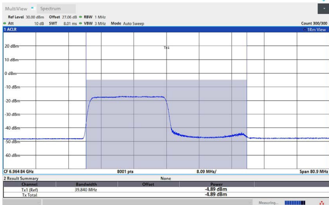
11AX40MIMO-Ant1-6965-242Tone-RU61-PASS
