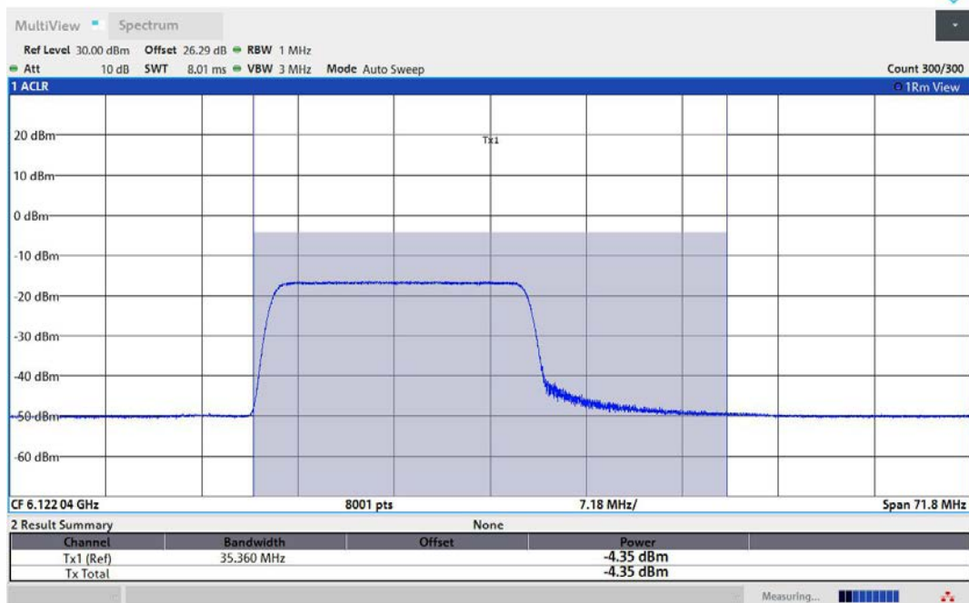
11AX80MIMO-Ant1-6145-242Tone-RU61-PASS
