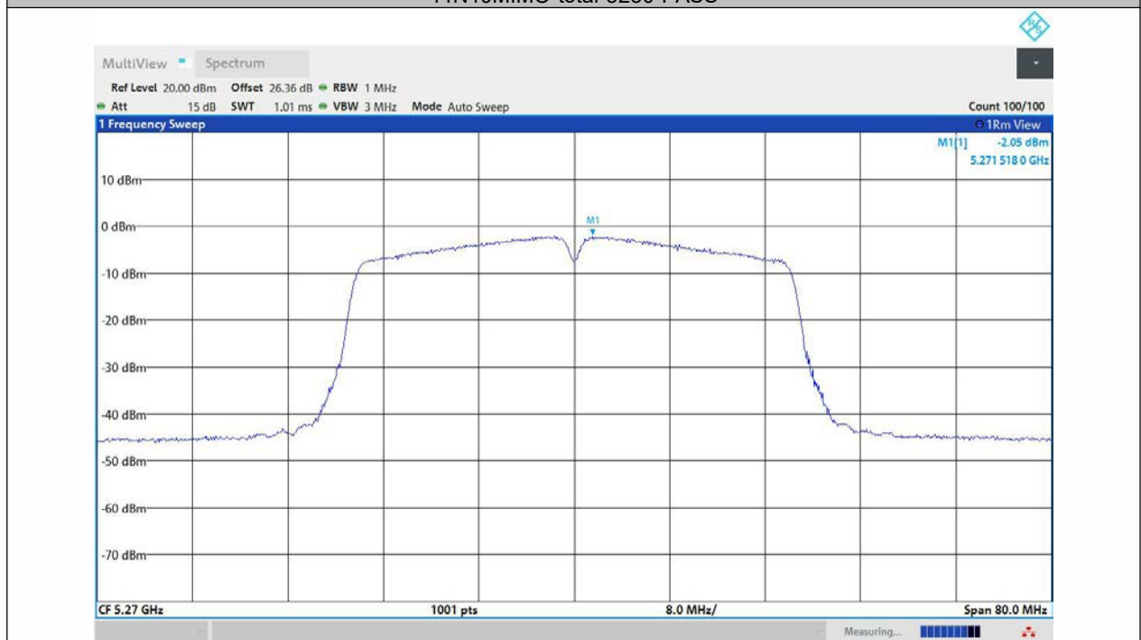
11N40MIMO-Ant1-5270-PASS
