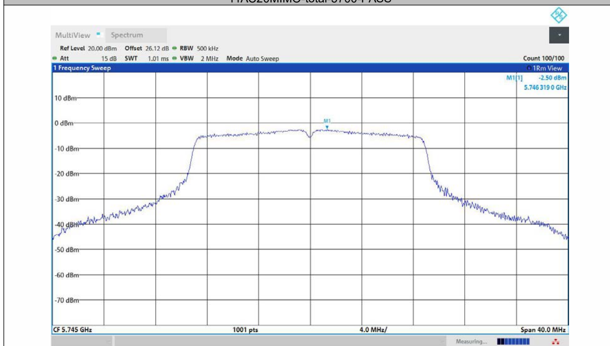
11AC20MIMO-Ant1-5745-PASS
