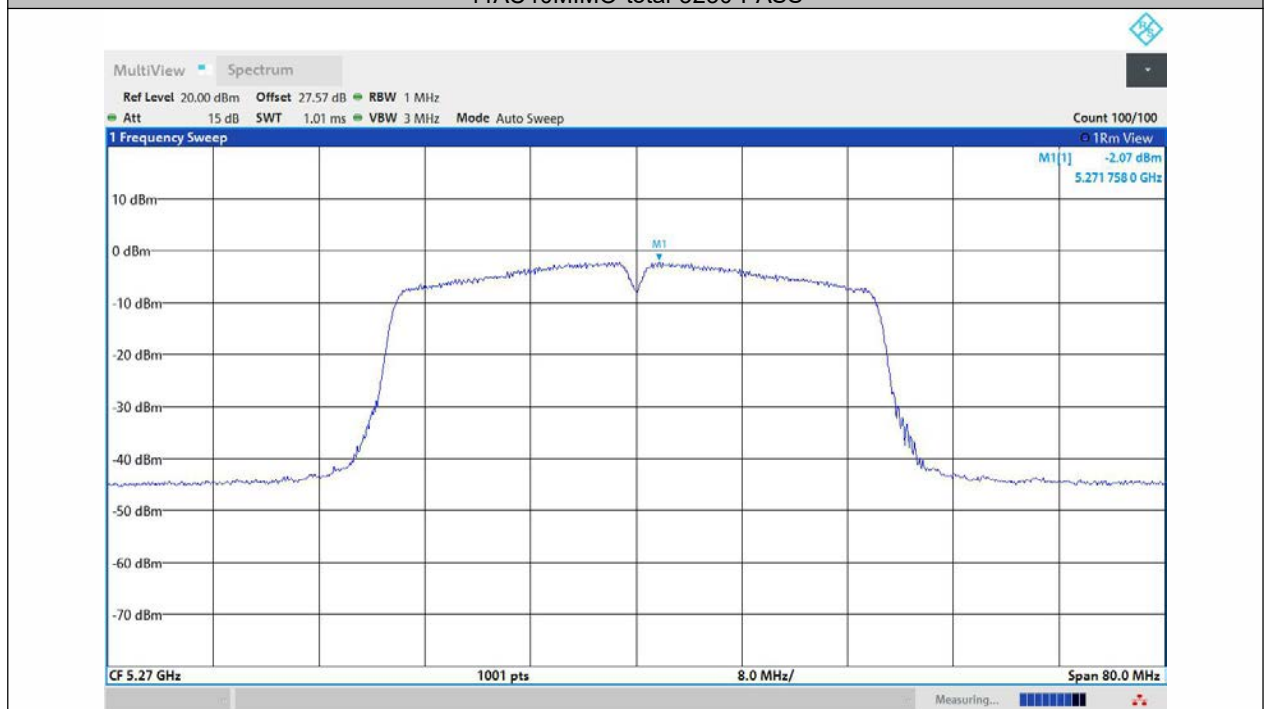
11AC40MIMO-Ant1-5270-PASS
