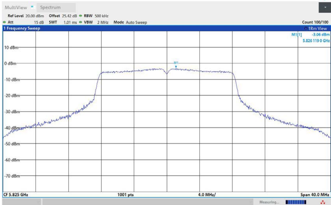
11A-Ant2-5825-PASS
