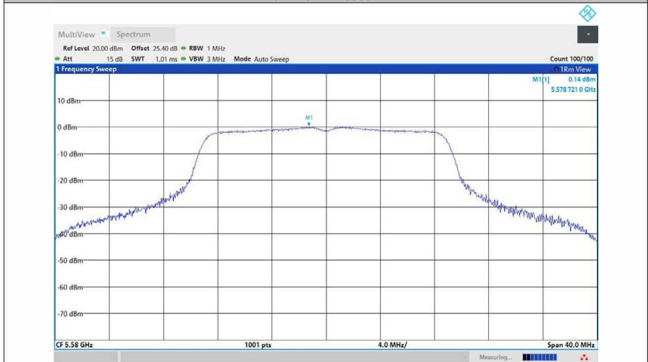
11N20MIMO-Ant1-5580-PASS
