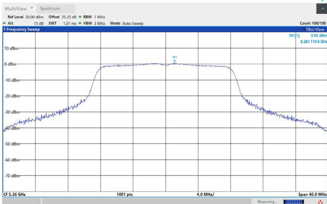
11A-Ant1-5260-PASS
