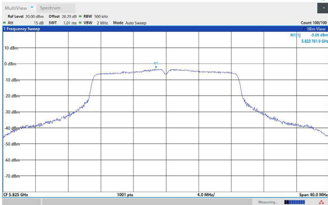
11AC20MIMO-Ant2-5825-PASS
