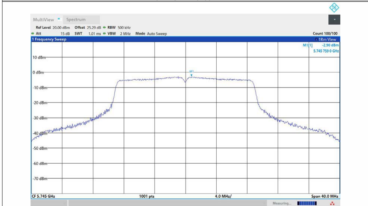
11N20MIMO-Ant1-5745-PASS
