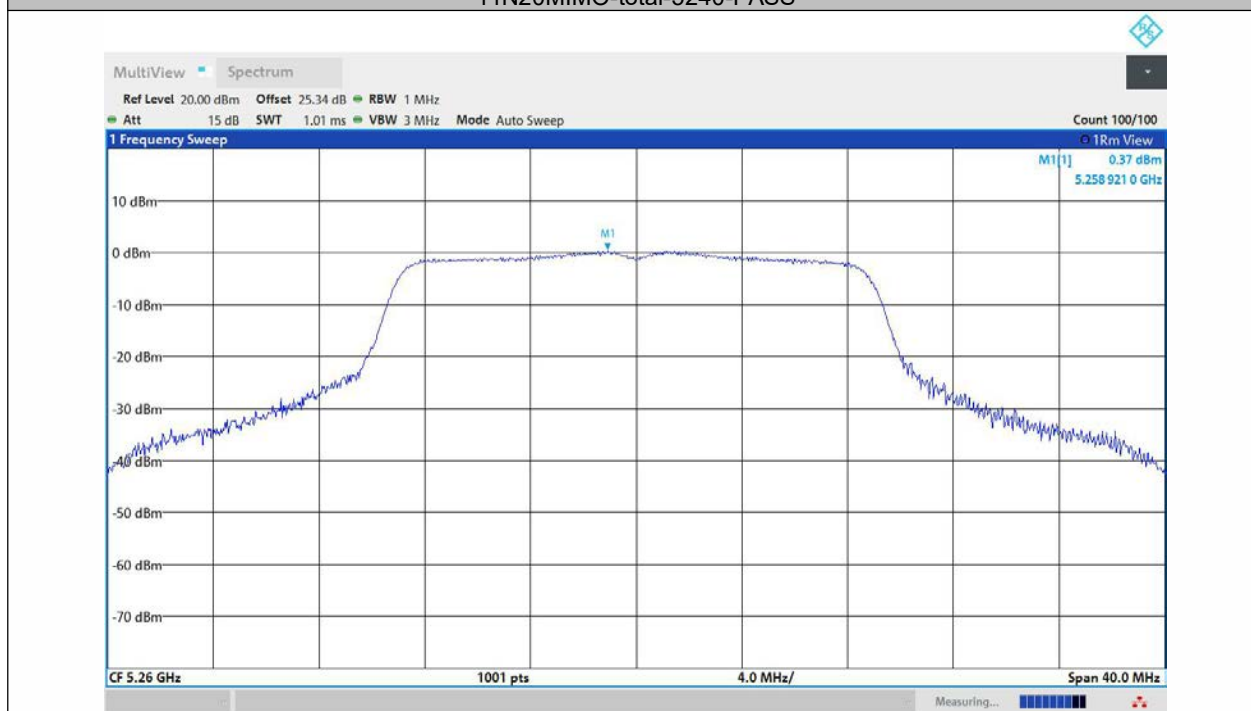
11N20MIMO-Ant1-5260-PASS
