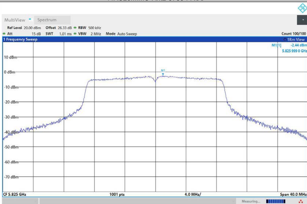
11AC20MIMO-Ant1-5825-PASS
