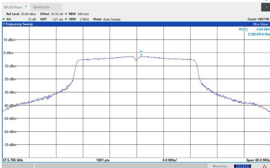
11N20MIMO-Ant2-5785-PASS
