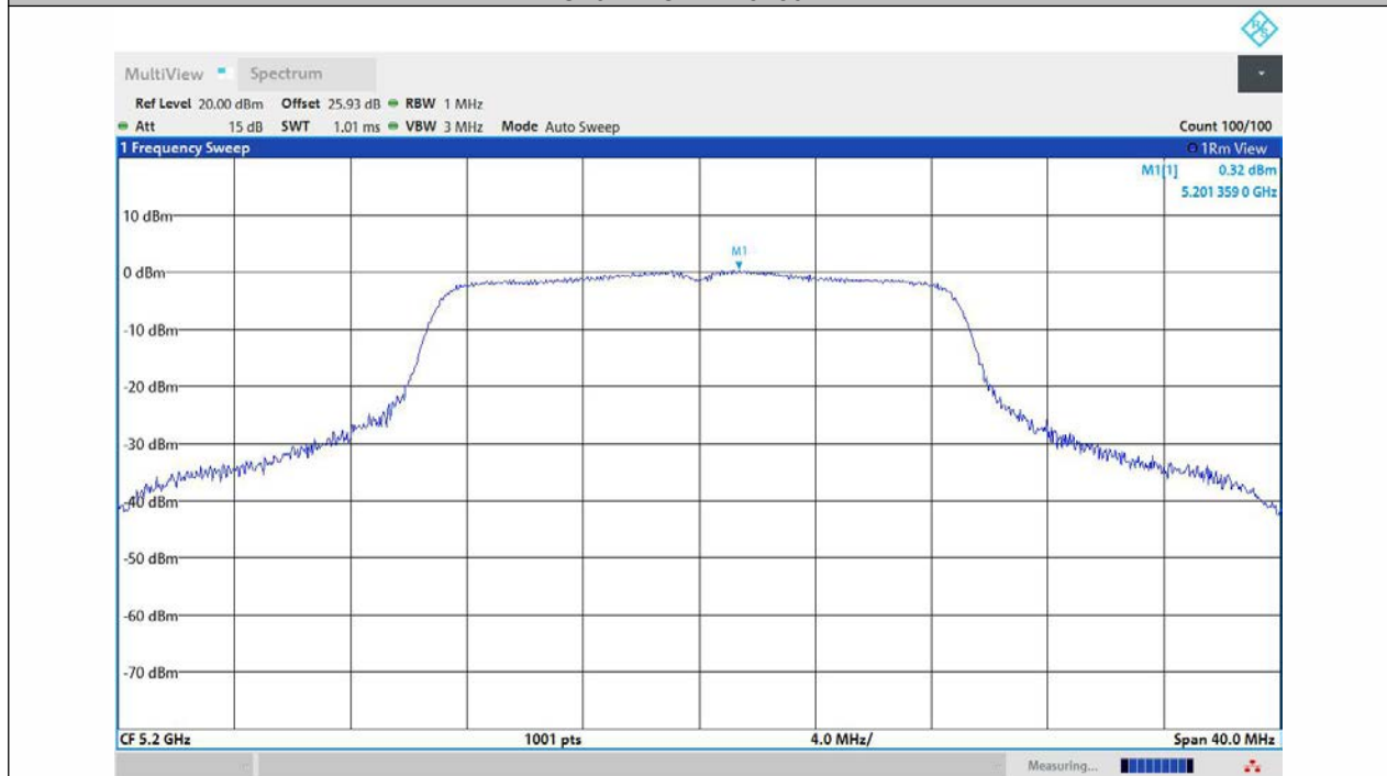
11AC20MIMO-Ant1-5200-PASS
