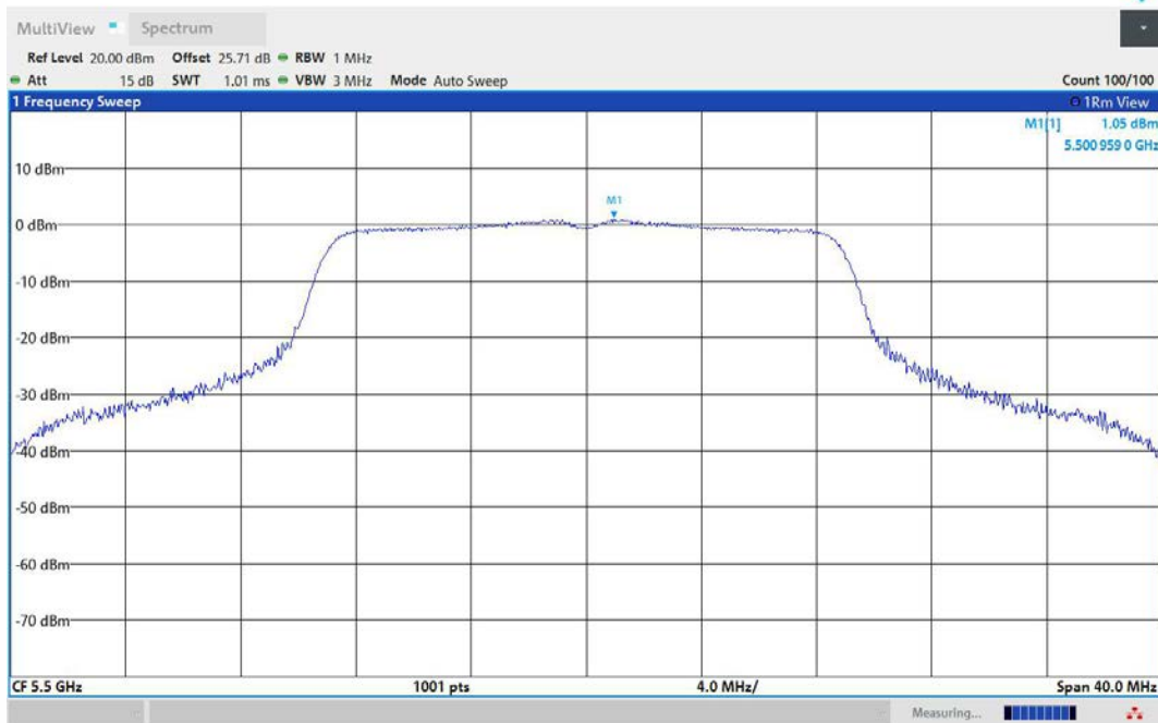
11N20MIMO-Ant1-5500-PASS
