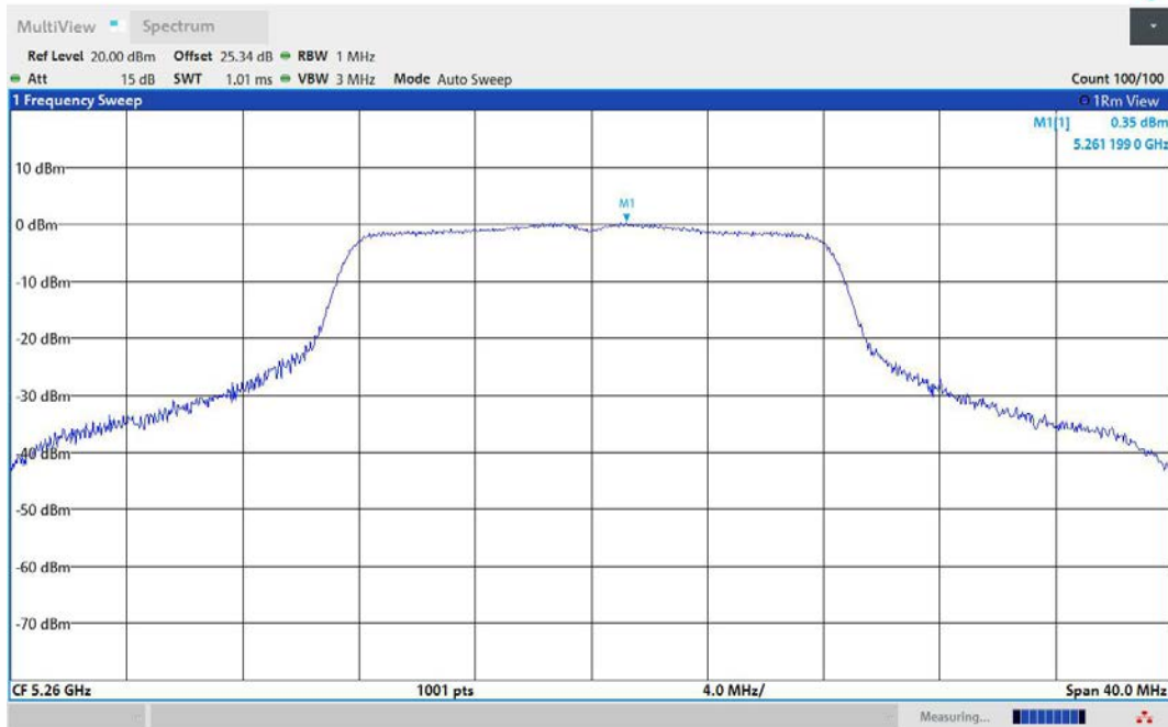
11A-Ant2-5260-PASS
