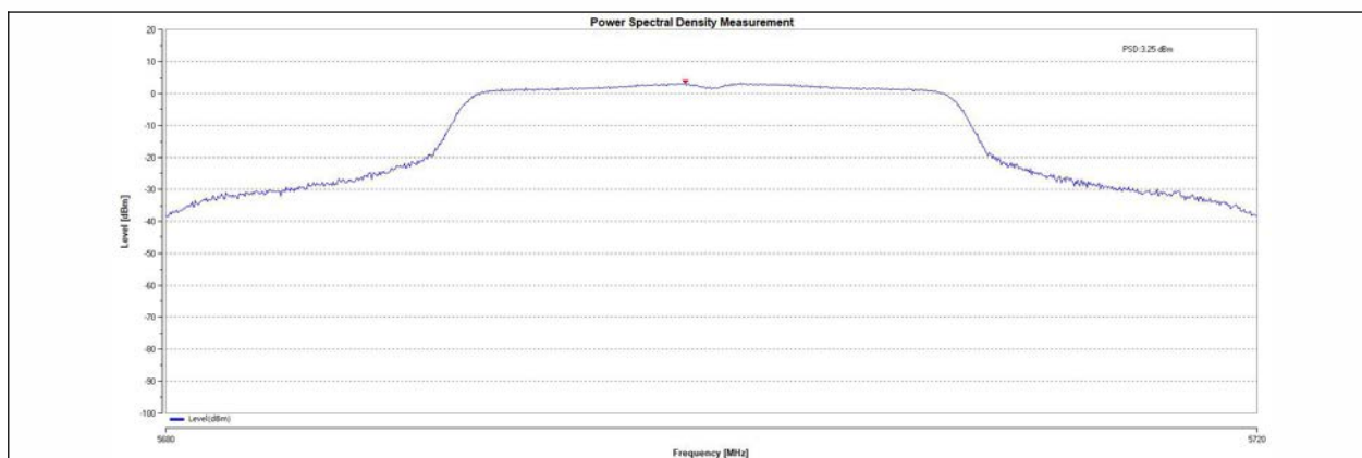
11AC20MIMO-total-5700-PASS
