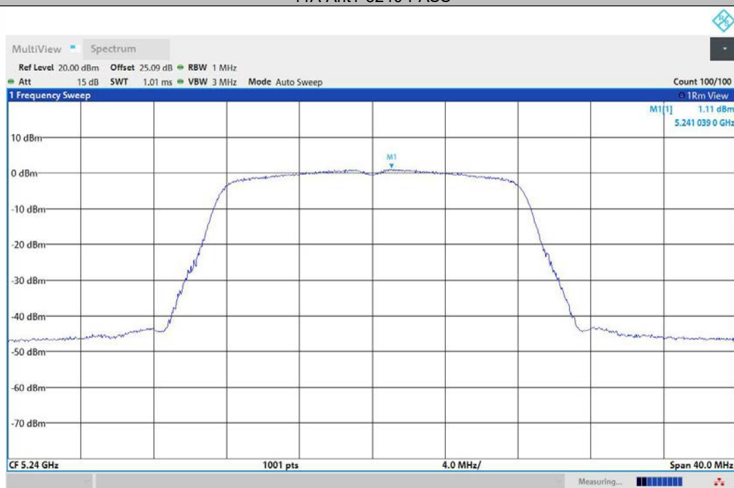
11A-Ant2-5240-PASS
