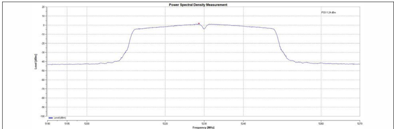
11N40MIMO-total-5230-PASS
