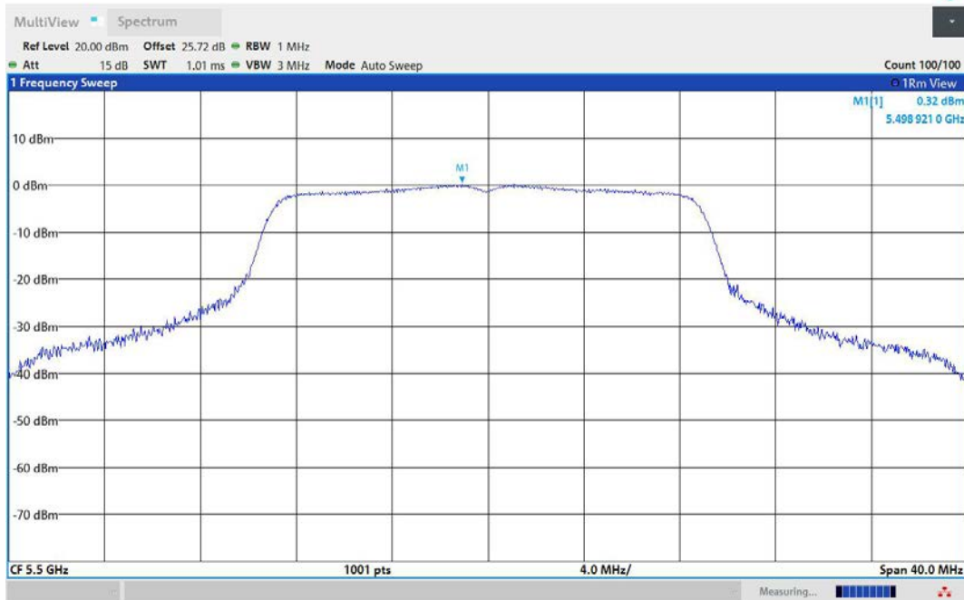
11N20MIMO-Ant2-5500-PASS
