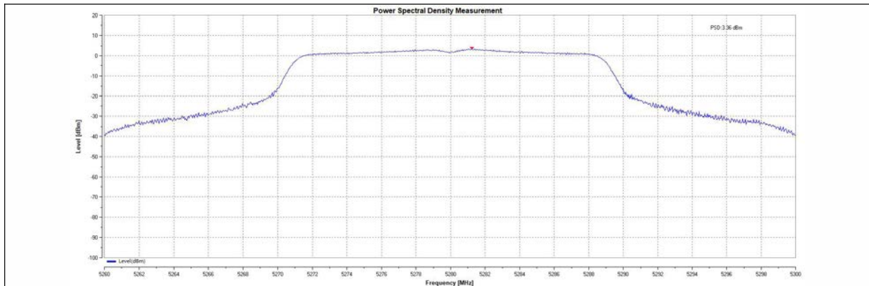
11AC20MIMO-total-5280-PASS
