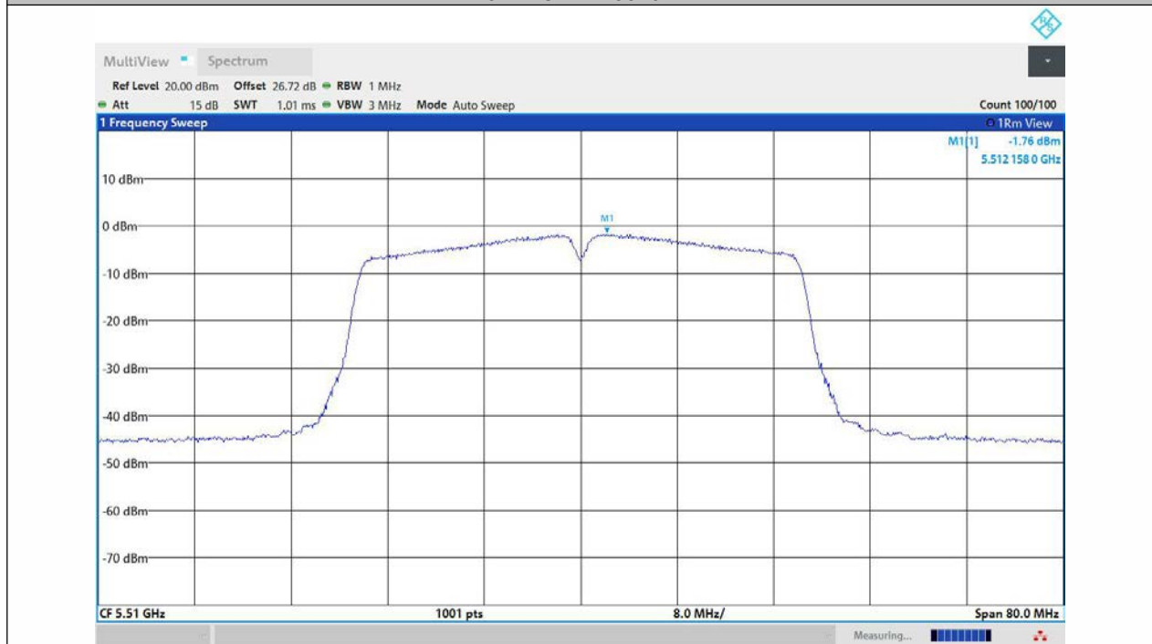
11N40MIMO-Ant1-5510-PASS
