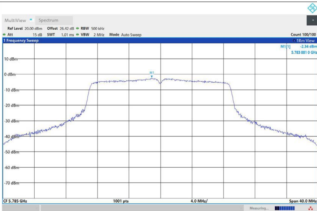
11AC20MIMO-Ant2-5785-PASS
