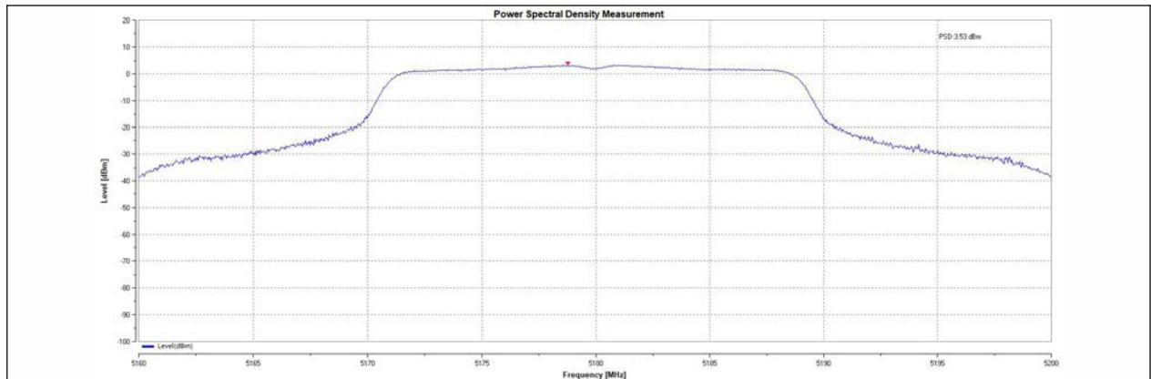
11N20MIMO-total-5180-PASS
