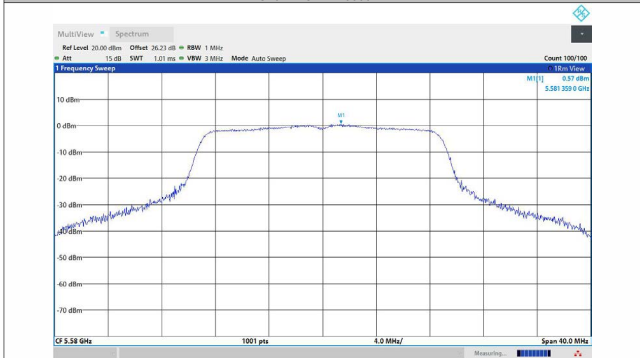
11AC20MIMO-Ant1-5580-PASS
