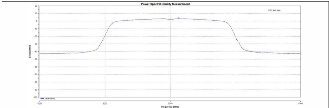
11AC20MIMO-total-5240-PASS
