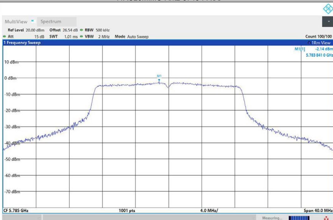
11AC20MIMO-Ant1-5785-PASS
