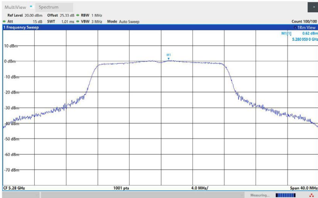
11A-Ant2-5280-PASS
