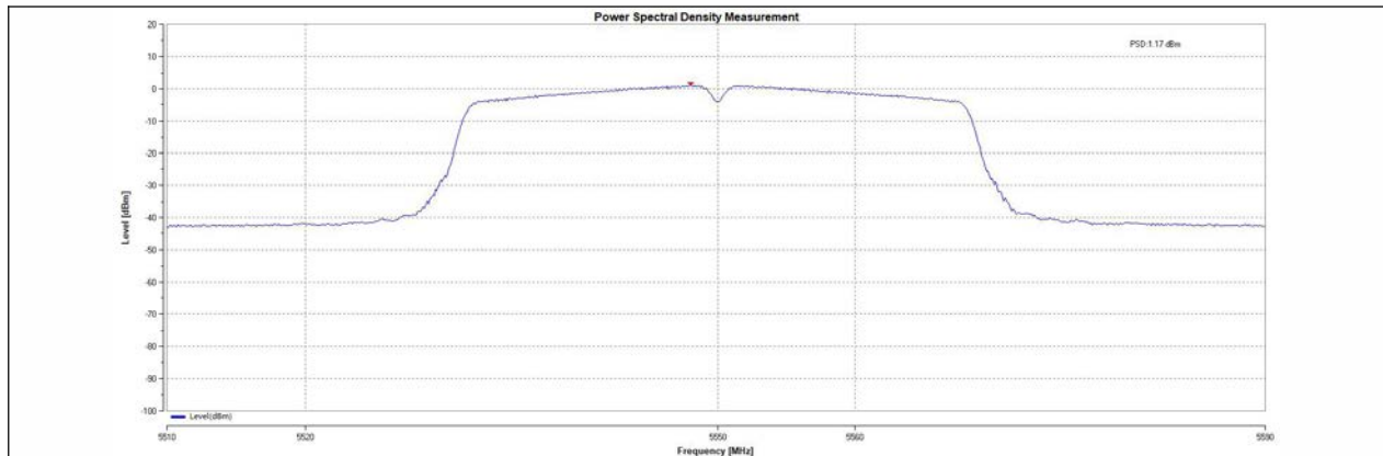
11N40MIMO-total-5550-PASS
