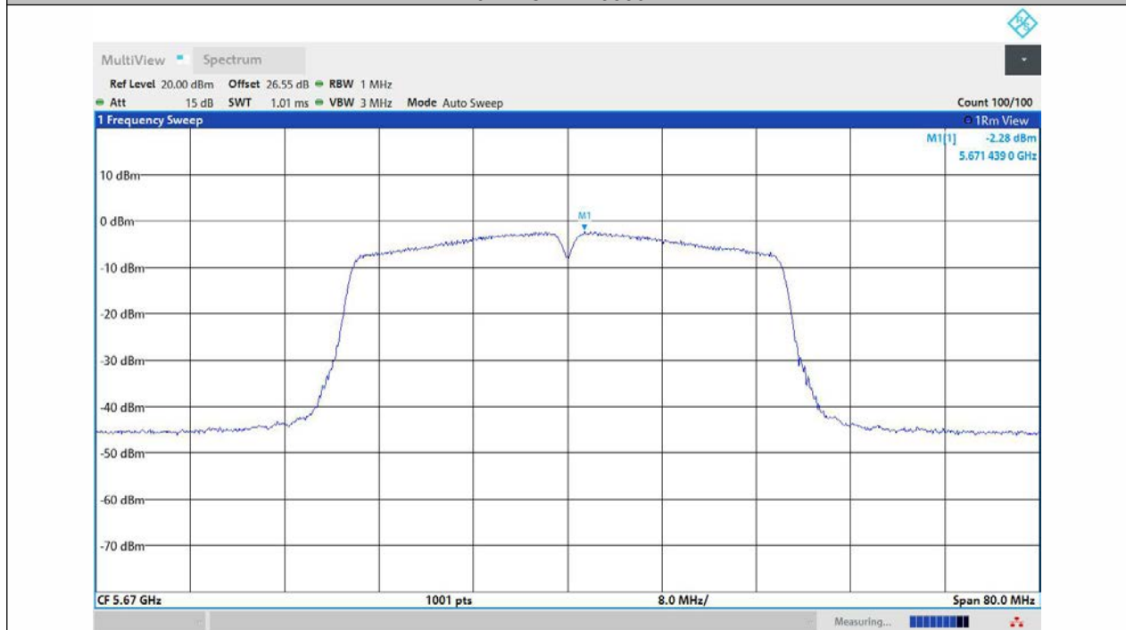
11N40MIMO-Ant1-5670-PASS
