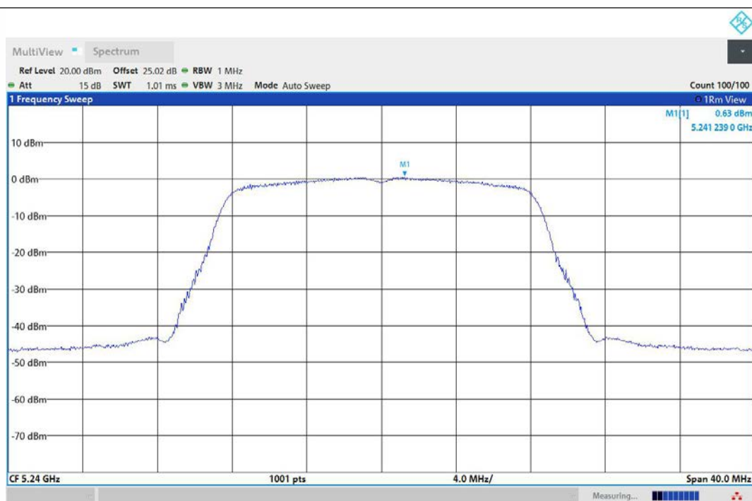
11A-Ant1-5240-PASS
