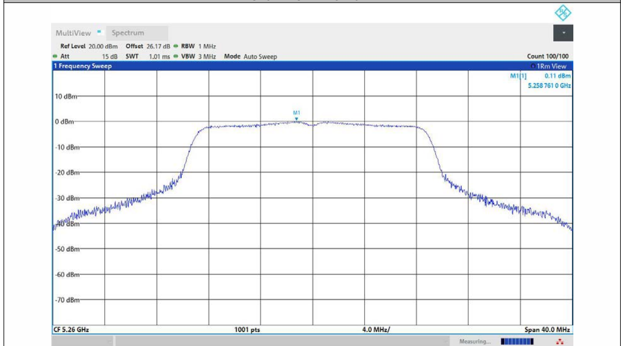
11AC20MIMO-Ant1-5260-PASS
