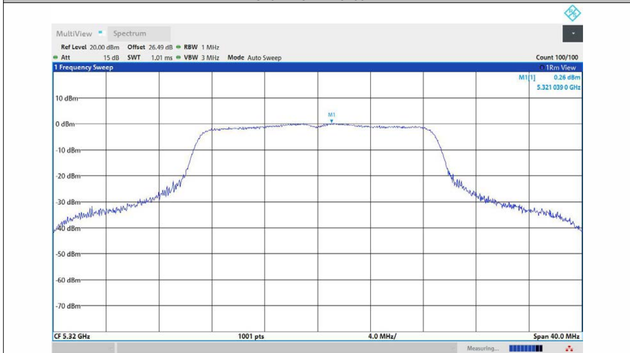
11AC20MIMO-Ant1-5320-PASS
