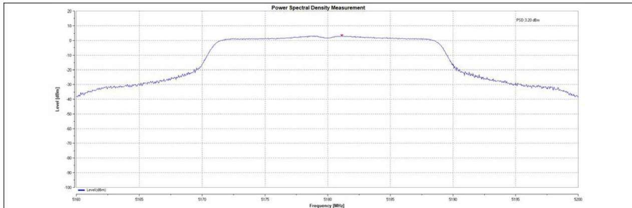
11AC20MIMO-total-5180-PASS
