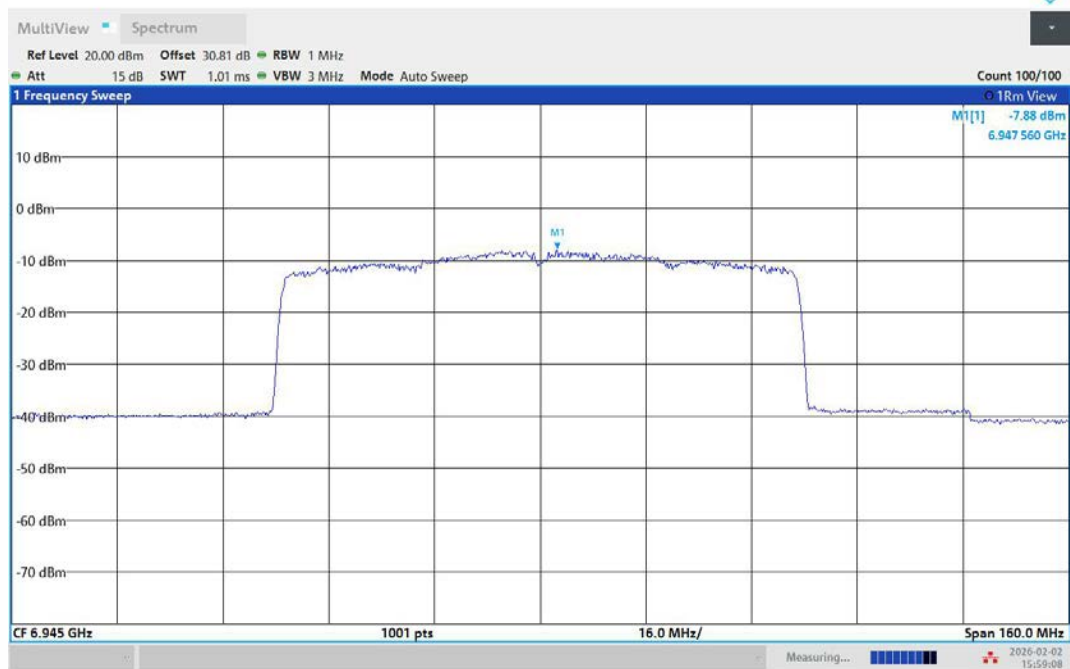
11AX80MIMO-Ant2-6945-PASS
