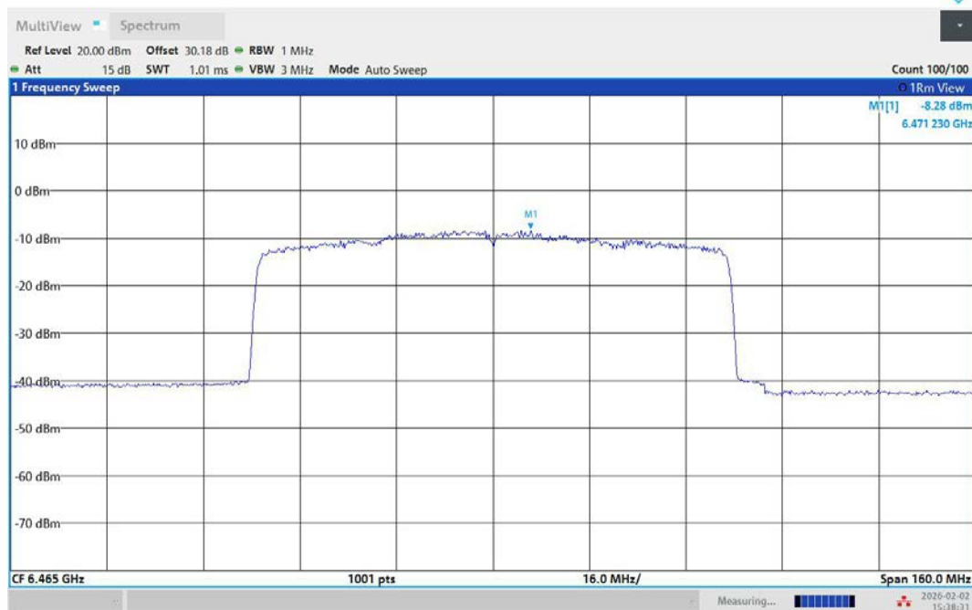
11AX80MIMO-Ant1-6465-PASS
