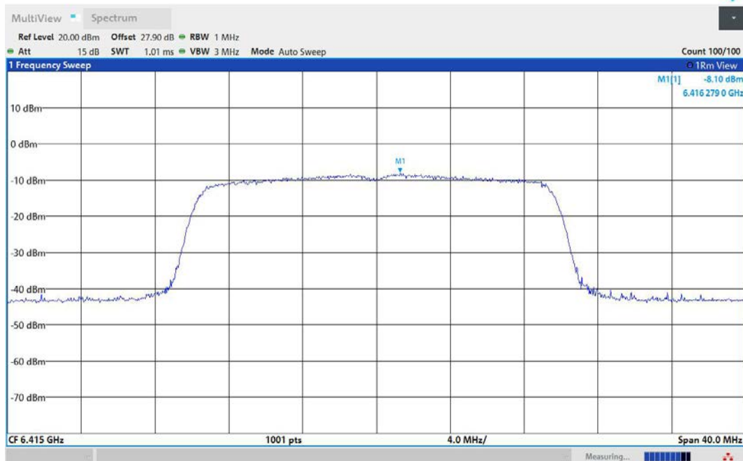
11AX20MIMO-Ant2-6415-PASS
