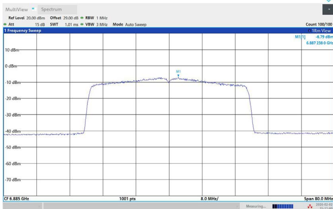
11AX40MIMO-Ant2-6885-PASS
