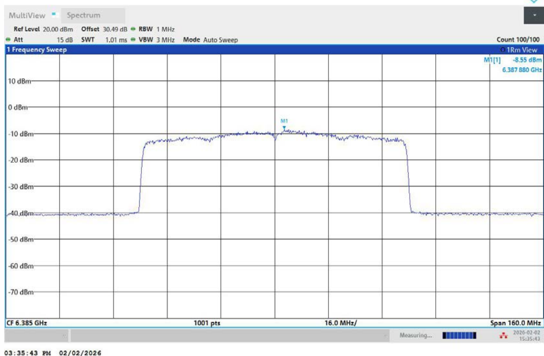
11AX80MIMO-Ant2-6385-PASS
