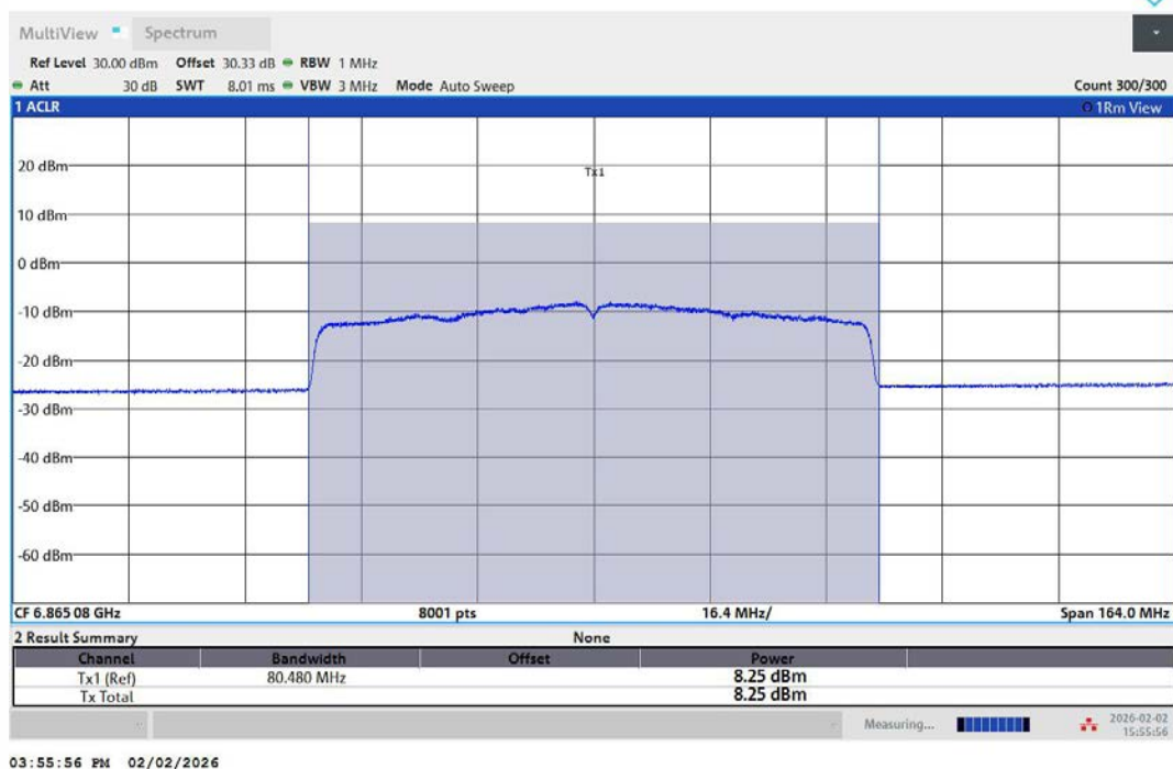
11AX80MIMO-Ant2-6865-PASS
