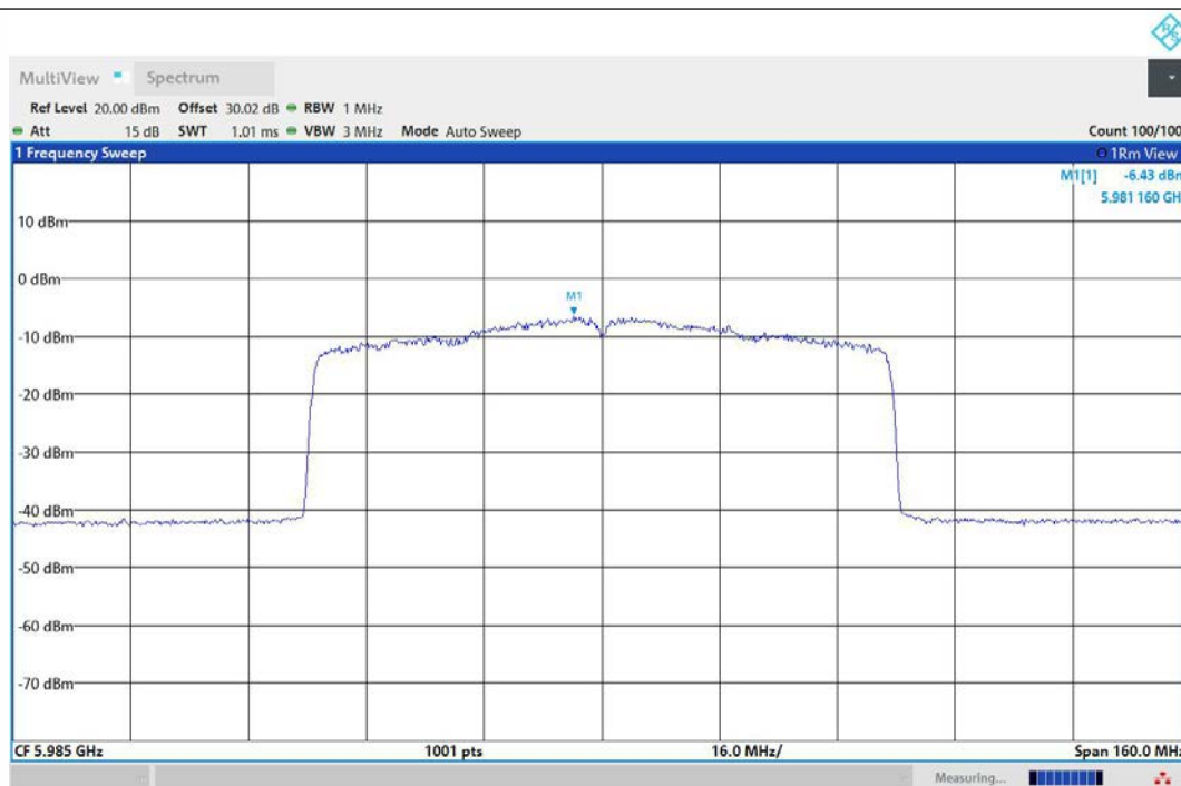
11AX80MIMO-Ant1-5985-PASS
