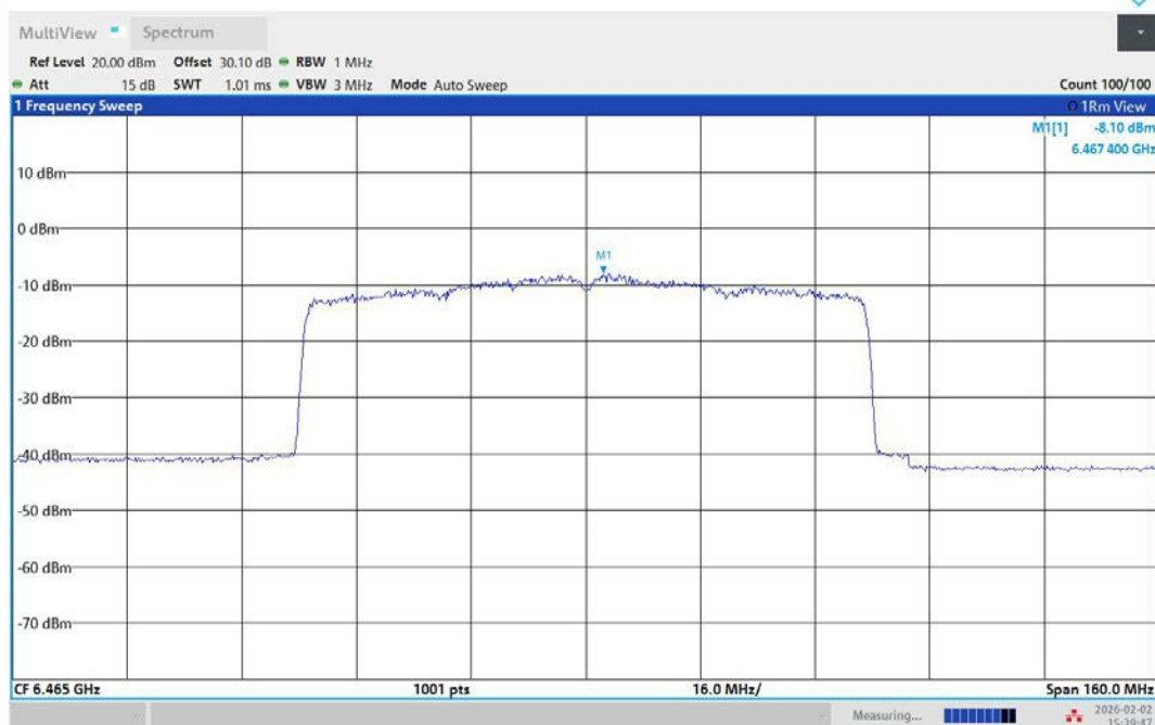
11AX80MIMO-Ant2-6465-PASS
