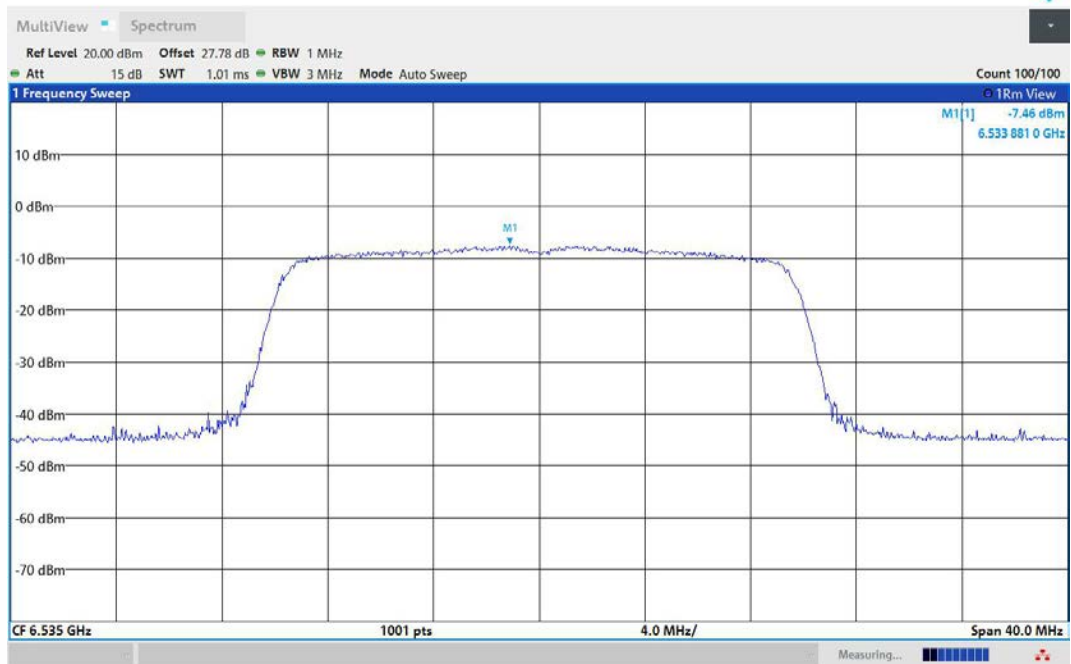
11AX20MIMO-Ant1-6535-PASS
