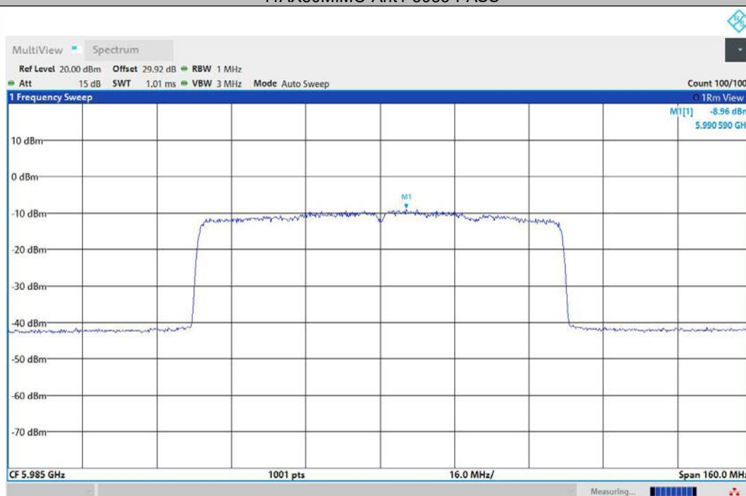
11AX80MIMO-Ant2-5985-PASS
