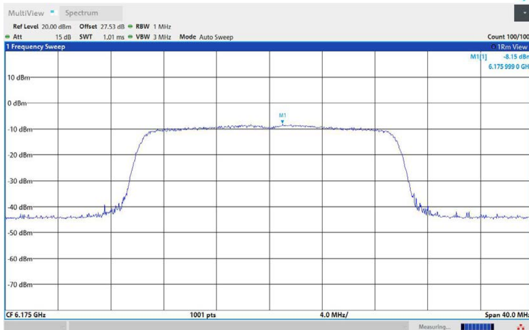
11AX20MIMO-Ant2-6175-PASS
