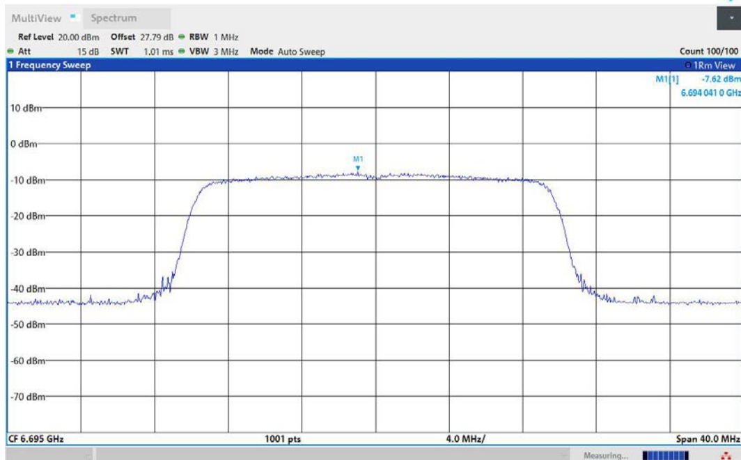
11AX20MIMO-Ant2-6695-PASS
