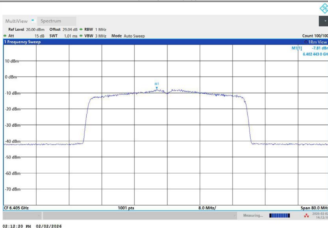
11AX40MIMO-Ant2-6405-PASS
