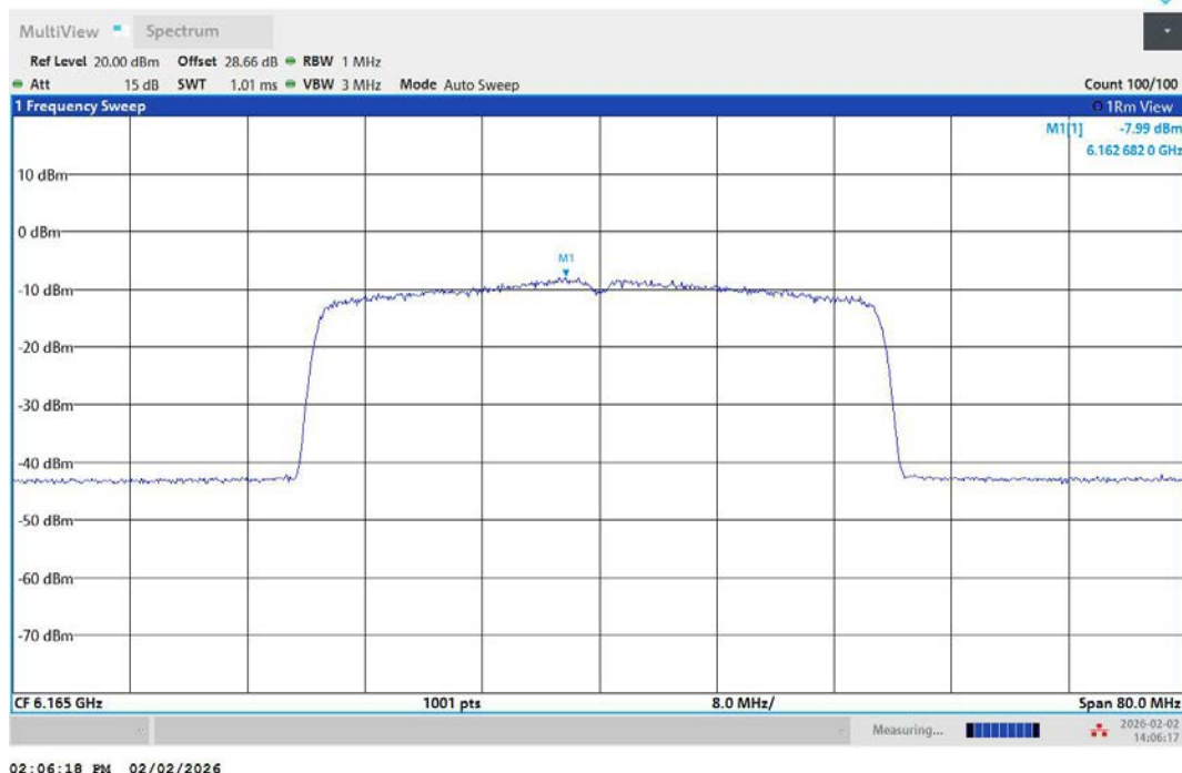
11AX40MIMO-Ant1-6165-PASS
