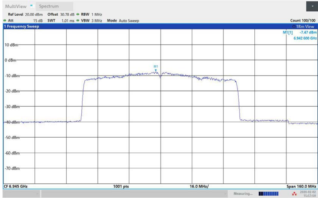
11AX80MIMO-Ant1-6945-PASS
