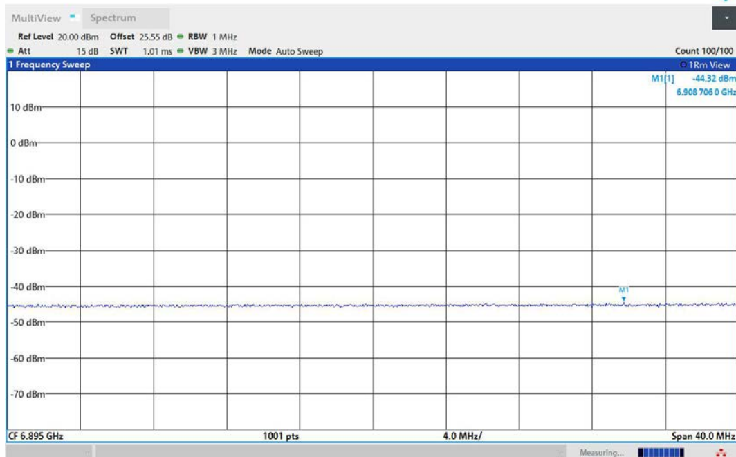
11AX20MIMO-Ant2-6895-PASS
