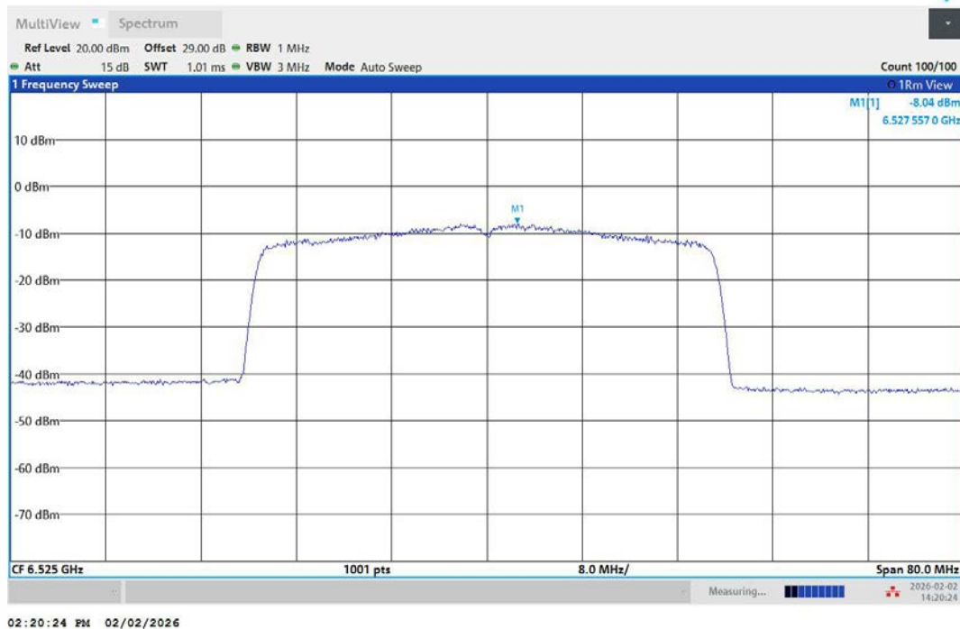
11AX40MIMO-Ant1-6525-PASS
