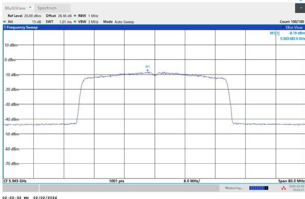
11AX40MIMO-Ant1-5965-PASS
