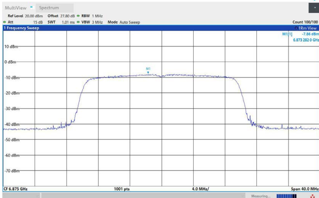
11AX20MIMO-Ant2-6875-PASS
