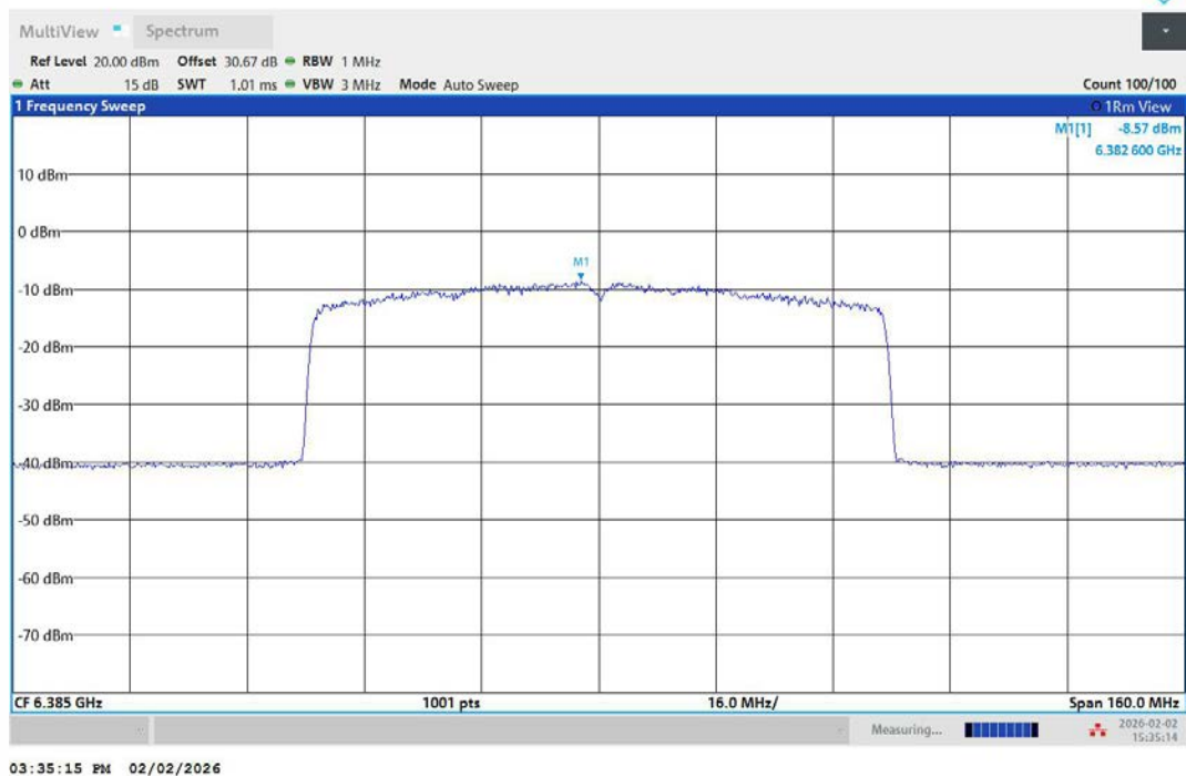
11AX80MIMO-Ant1-6385-PASS
