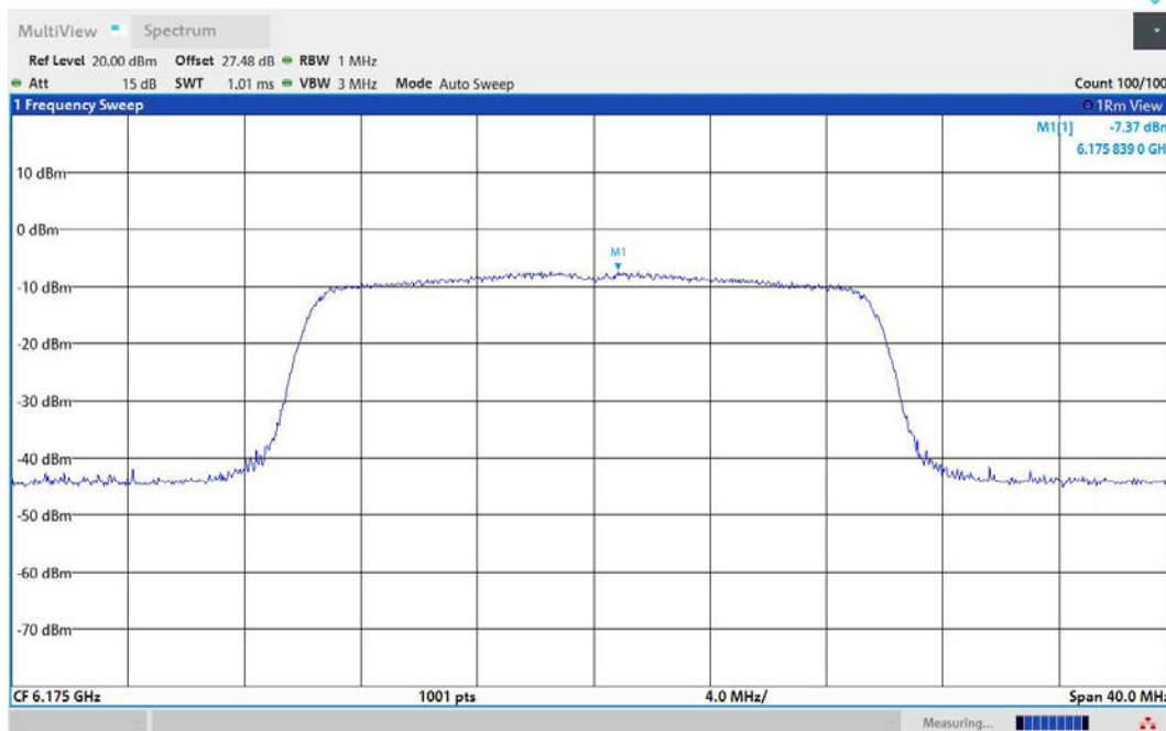
11AX20MIMO-Ant1-6175-PASS
