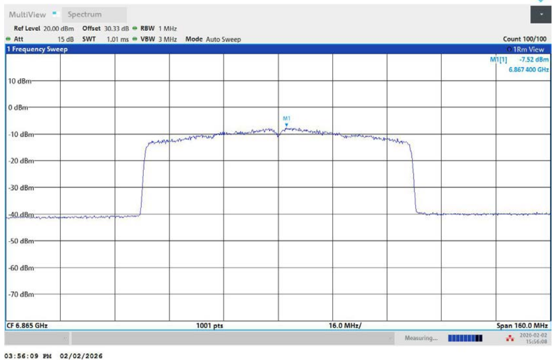
11AX80MIMO-Ant2-6865-PASS
