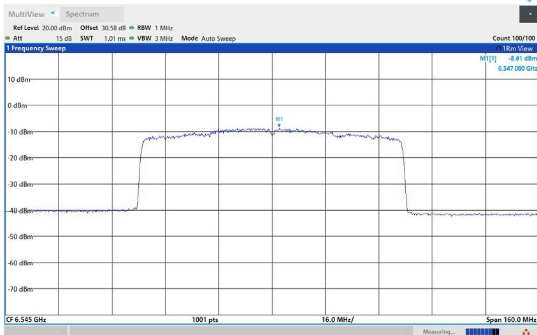
11AX80MIMO-Ant2-6545-PASS
