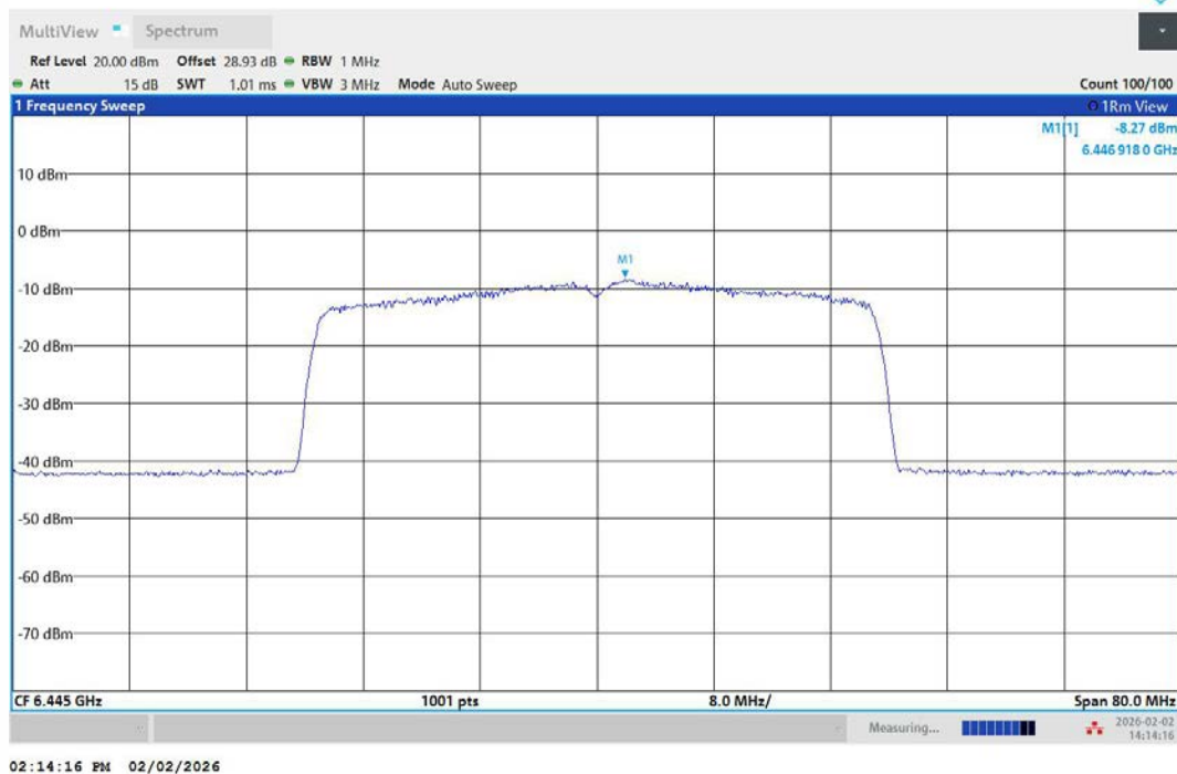
11AX40MIMO-Ant1-6445-PASS
