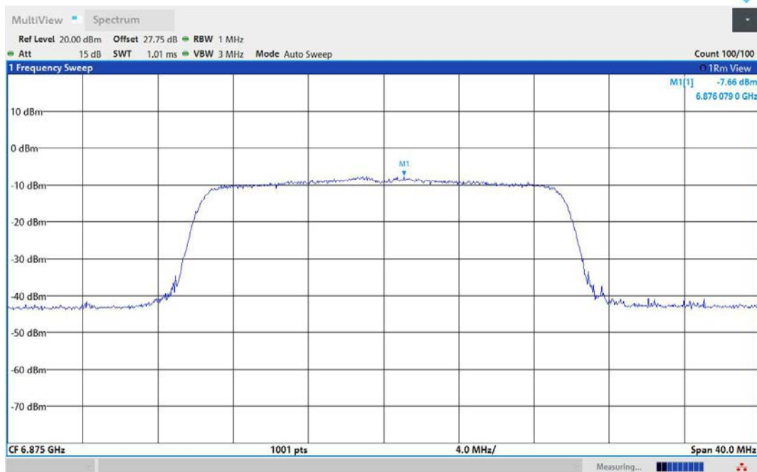
11AX20MIMO-Ant1-6875-PASS
