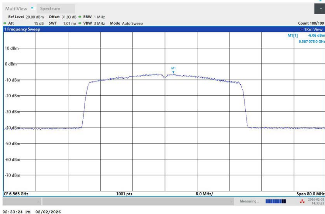
11AX40MIMO-Ant1-6565-PASS
