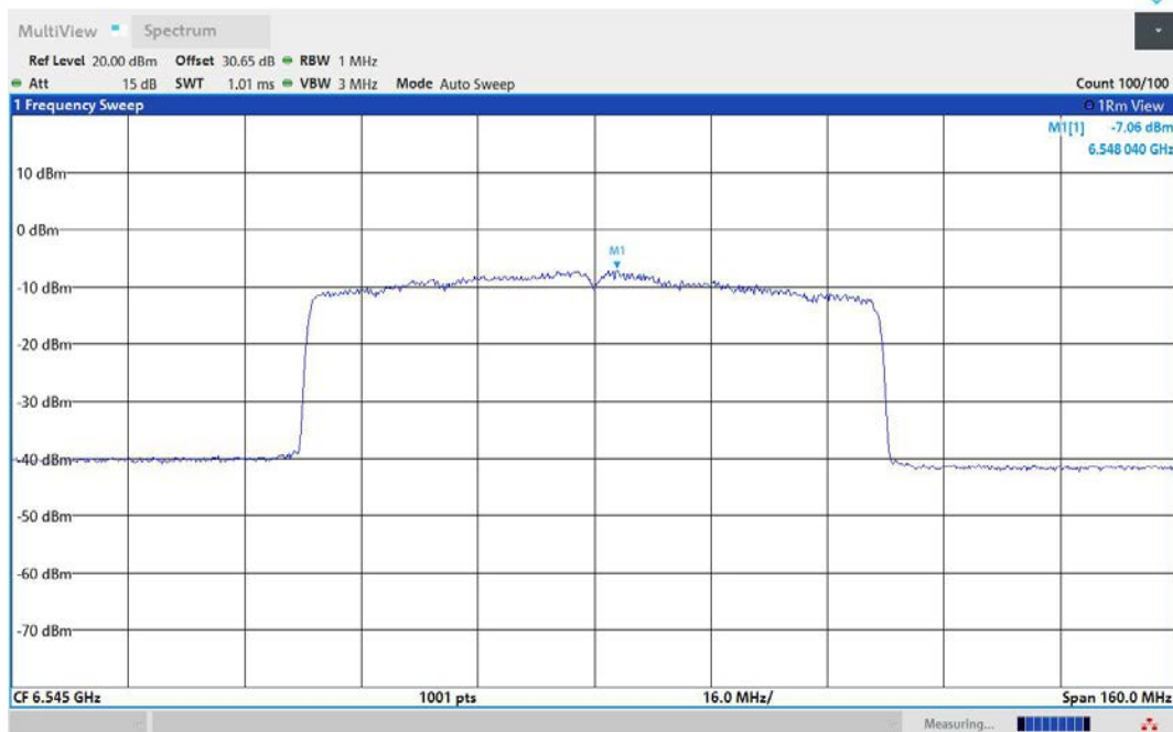
11AX80MIMO-Ant1-6545-PASS
