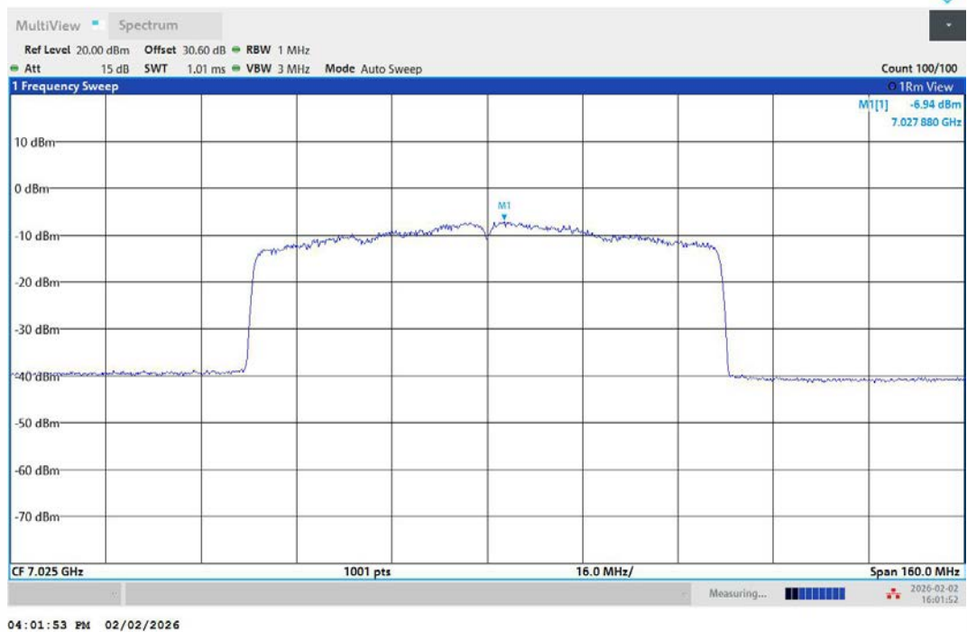
11AX80MIMO-Ant2-7025-PASS
