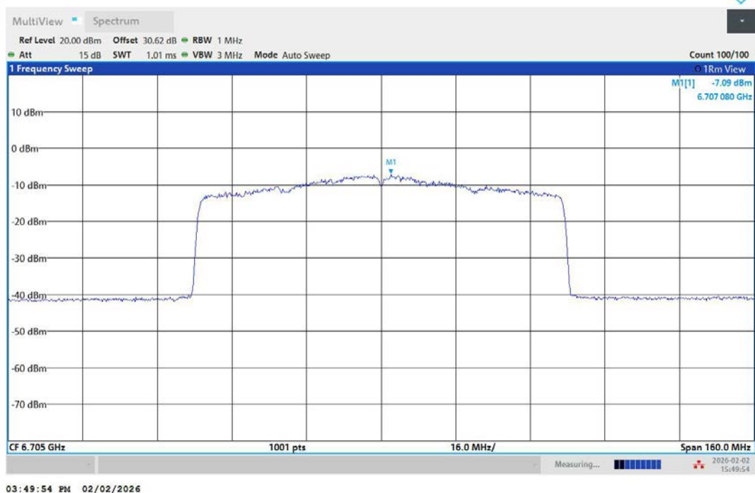
11AX80MIMO-Ant2-6705-PASS
