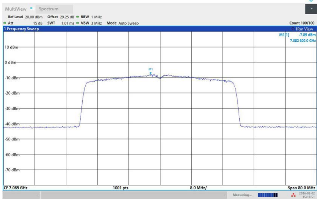
11AX40MIMO-Ant2-7085-PASS
