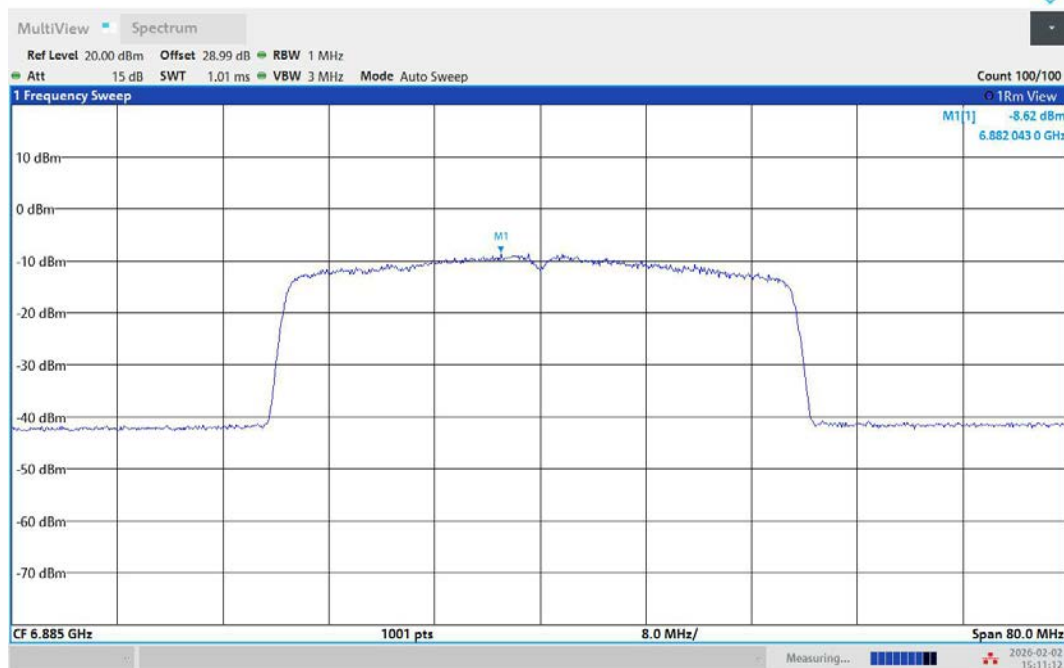
11AX40MIMO-Ant1-6885-PASS
