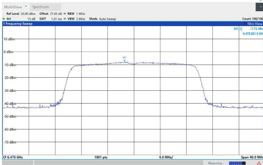
11AX20MIMO-Ant1-6475-PASS
