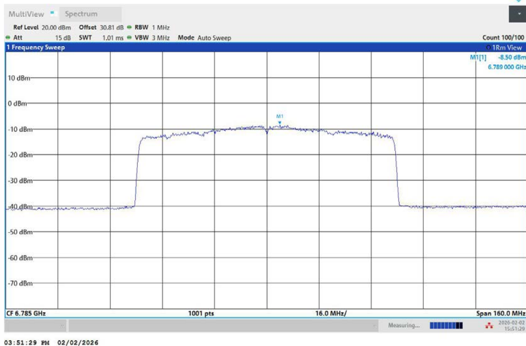
11AX80MIMO-Ant1-6785-PASS
