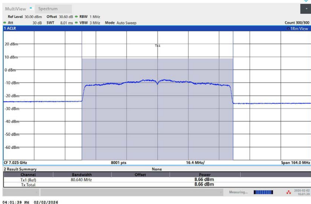
11AX80MIMO-Ant2-7025-PASS
