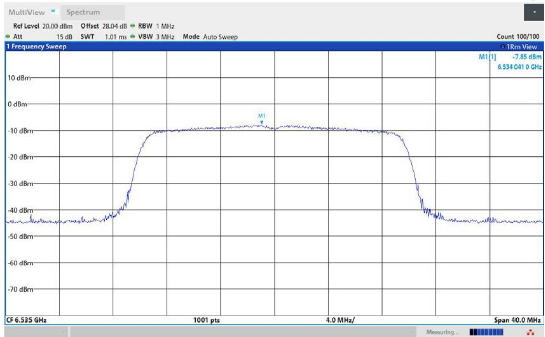
11AX20MIMO-Ant2-6535-PASS
