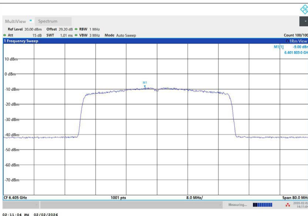
11AX40MIMO-Ant1-6405-PASS
