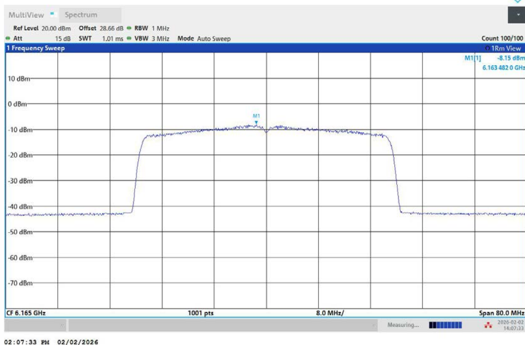
11AX40MIMO-Ant2-6165-PASS
