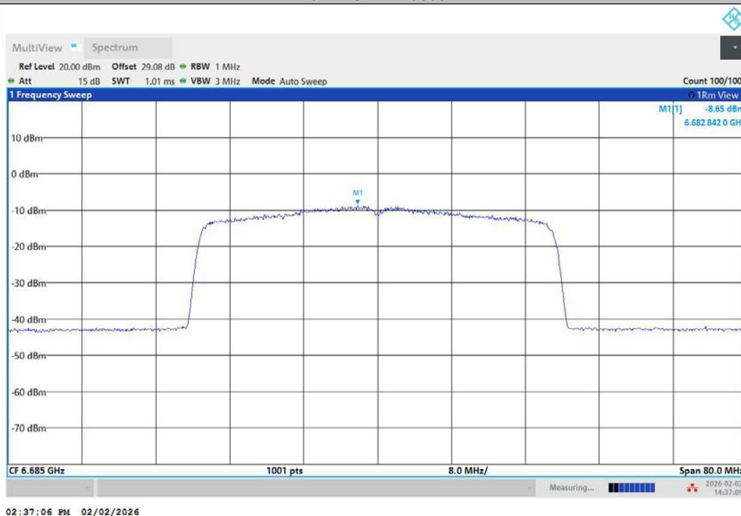
11AX40MIMO-Ant2-6685-PASS
