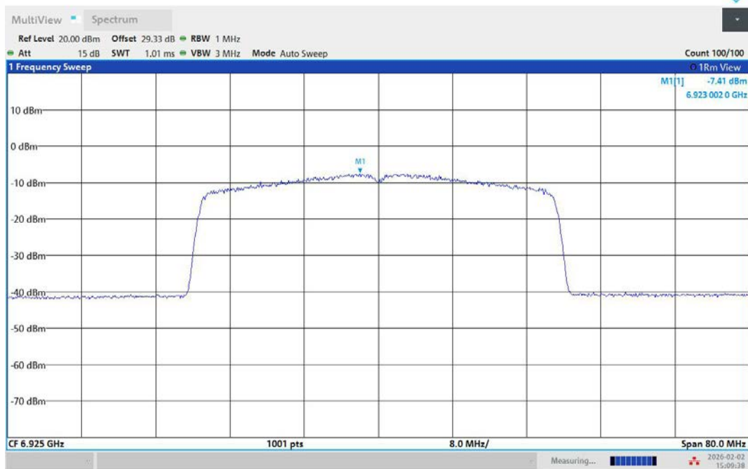
11AX40MIMO-Ant2-6925-PASS
