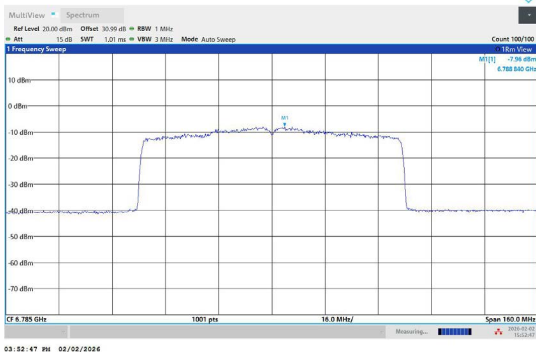
11AX80MIMO-Ant2-6785-PASS
