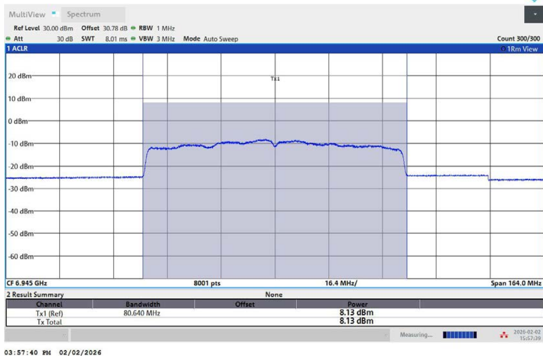
11AX80MIMO-Ant1-6945-PASS
