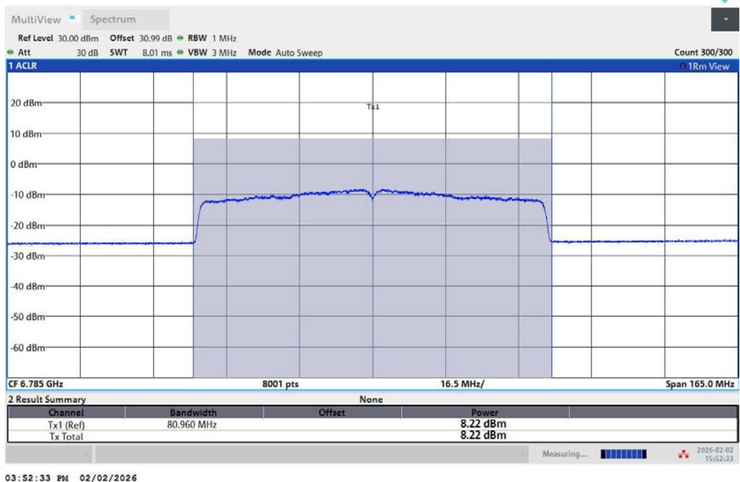
11AX80MIMO-Ant2-6785-PASS
