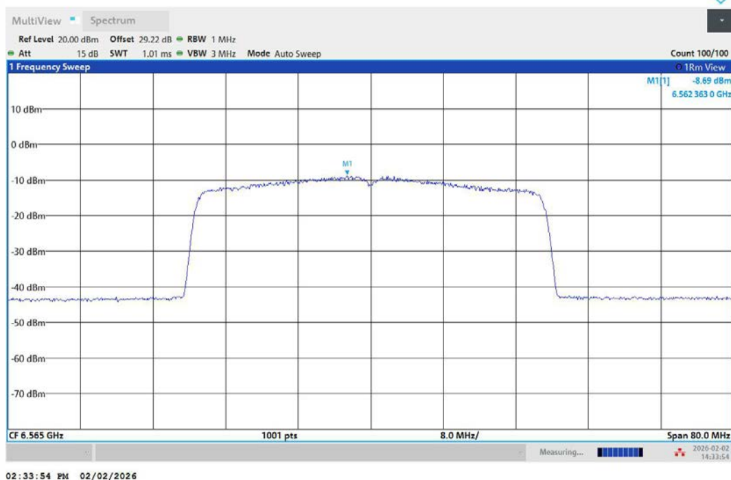
11AX40MIMO-Ant2-6565-PASS
