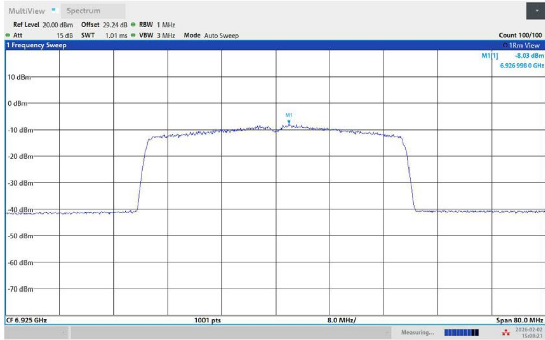
11AX40MIMO-Ant1-6925-PASS
