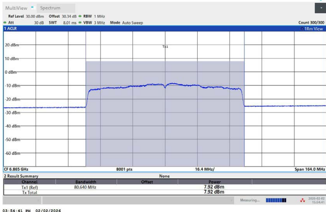
11AX80MIMO-Ant1-6865-PASS
