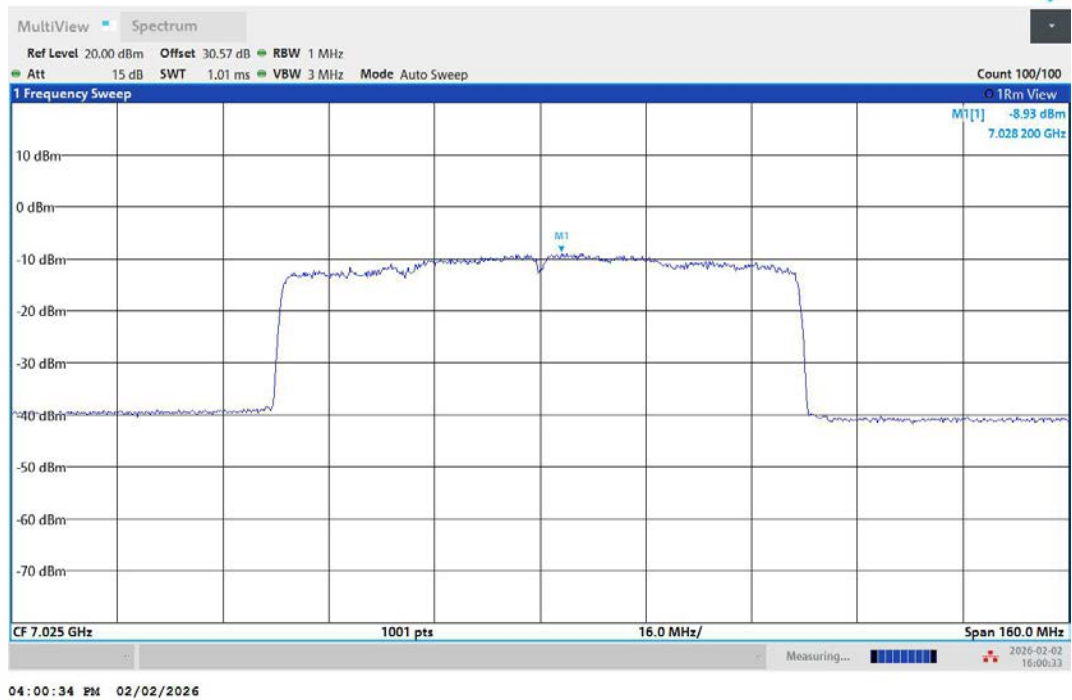
11AX80MIMO-Ant1-7025-PASS
