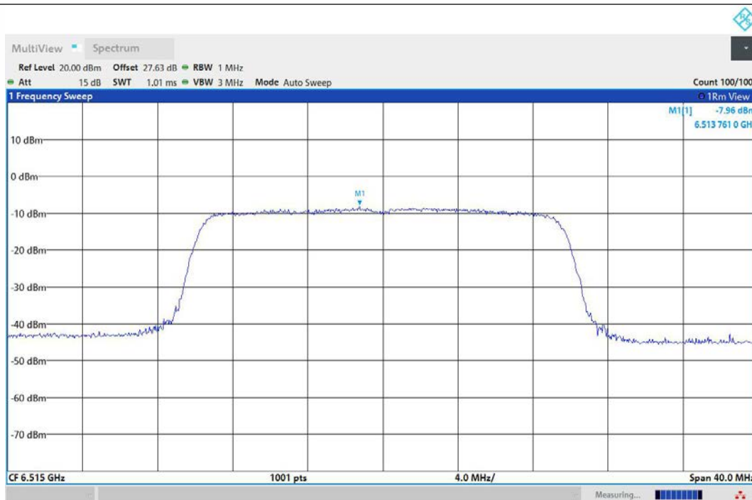
11AX20MIMO-Ant1-6515-PASS
