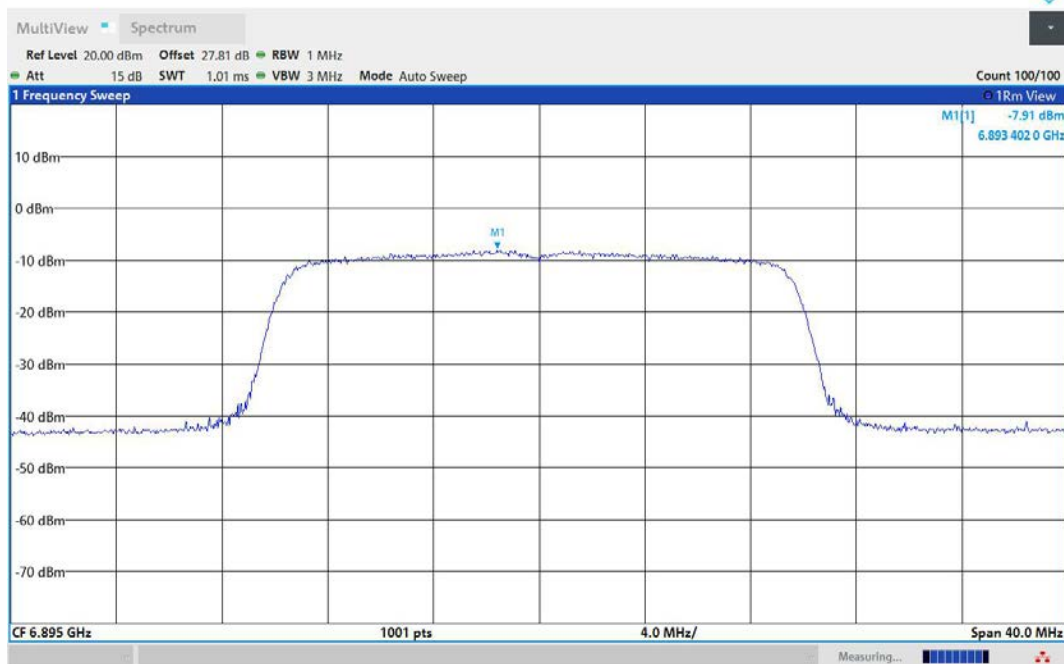
11AX20MIMO-Ant1-6895-PASS
