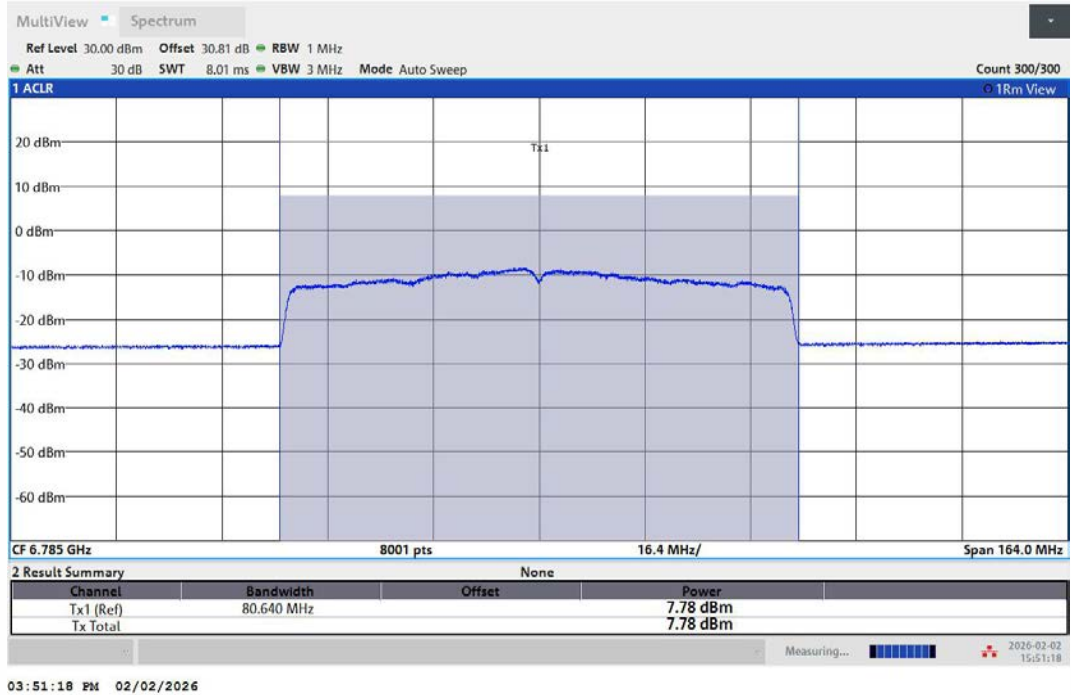
11AX80MIMO-Ant1-6785-PASS
