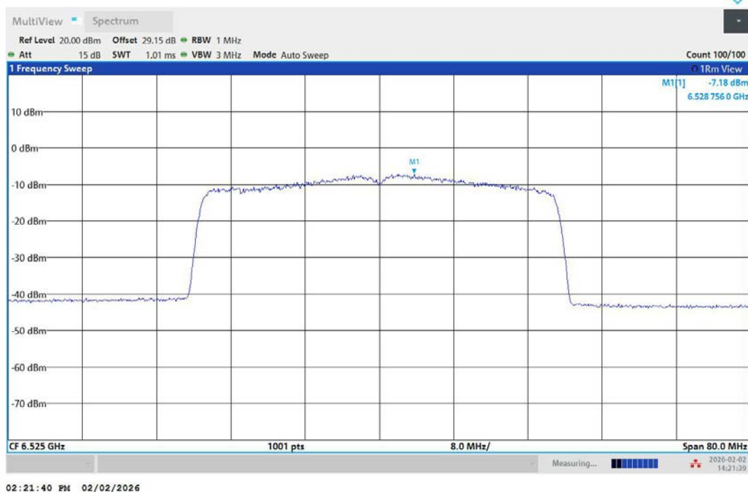
11AX40MIMO-Ant2-6525-PASS
