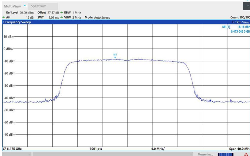
11AX20MIMO-Ant2-6475-PASS
