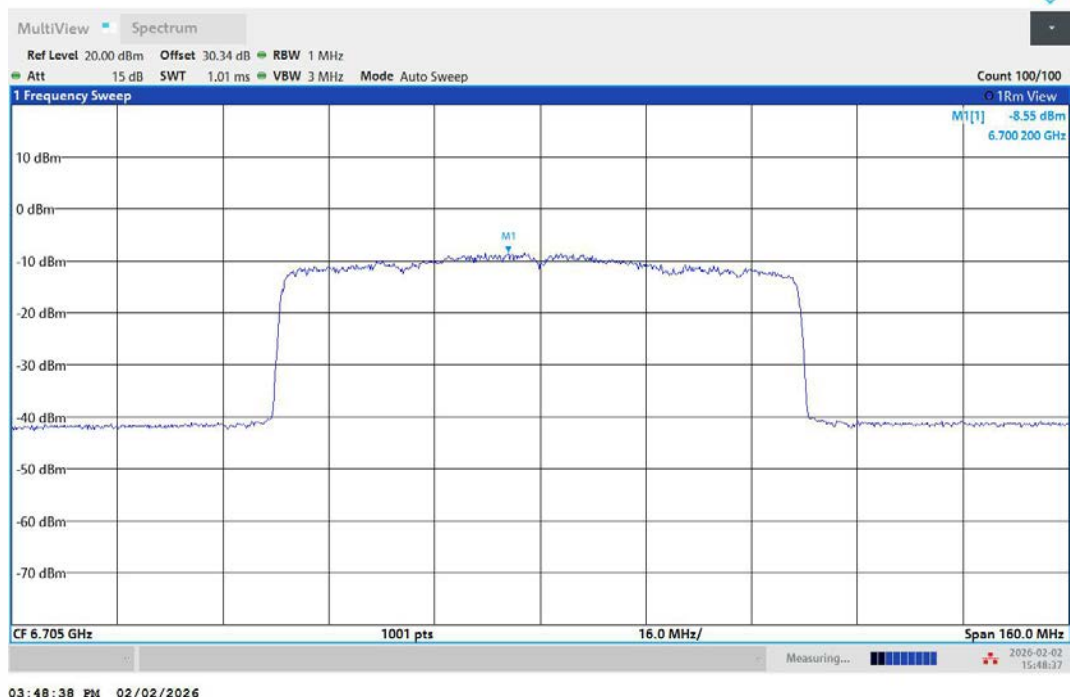
11AX80MIMO-Ant1-6705-PASS
