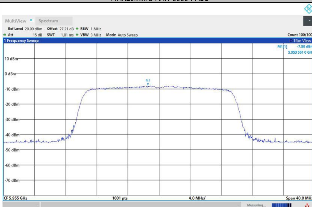
11AX20MIMO-Ant2-5955-PASS
