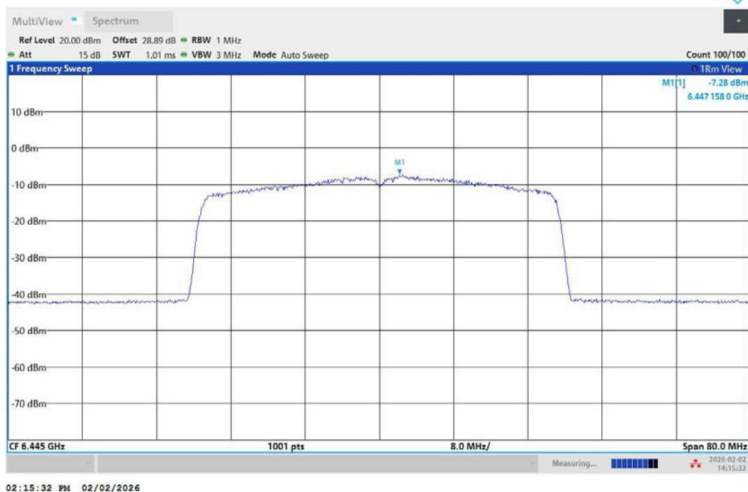
11AX40MIMO-Ant2-6445-PASS
