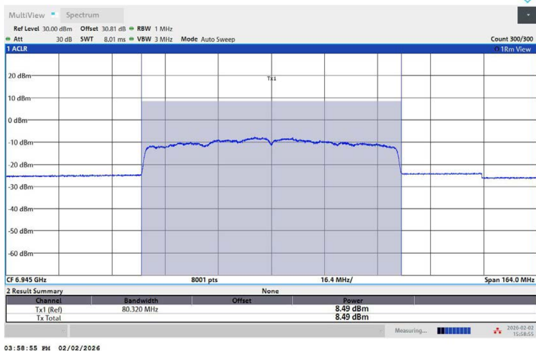
11AX80MIMO-Ant2-6945-PASS
