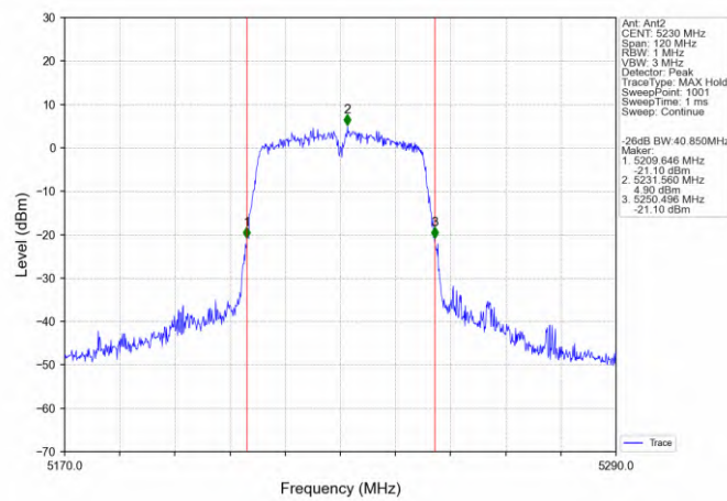
802.11ac(VHT40)_HCH_5230MHz_Ant2_NTNV
