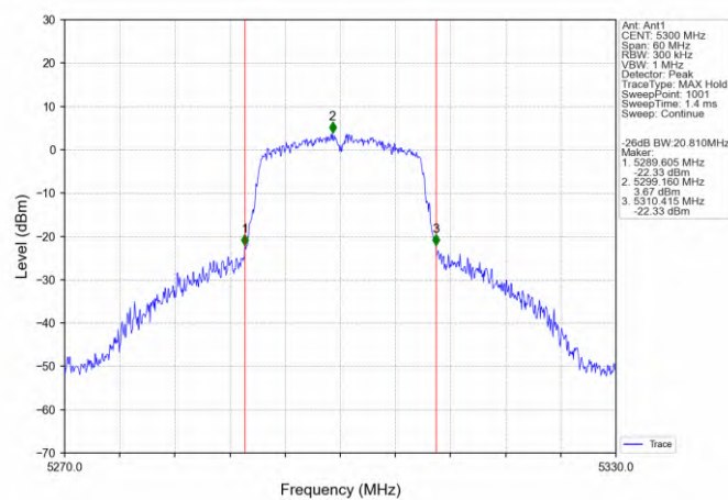
802.11n(HT20)_MCH_5300MHz_Ant1_NTNV
