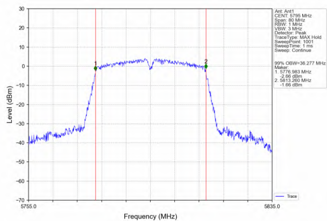
802.11ac(VHT40)_HCH_5795MHz_Ant1_NTNV
