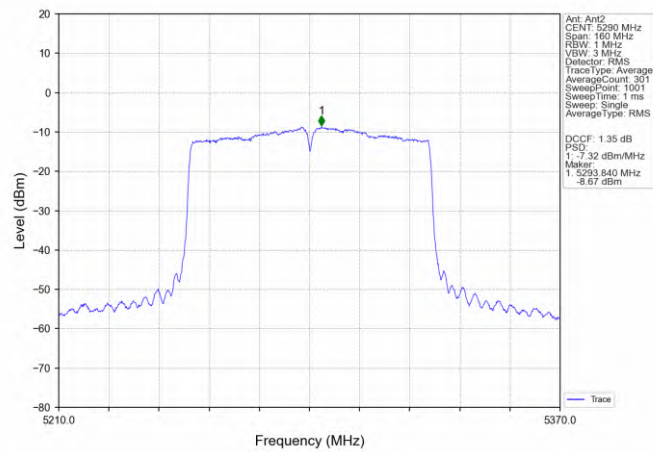
802.11ac(VHT80)_MCH_5290MHz_MIMO_NTNV
