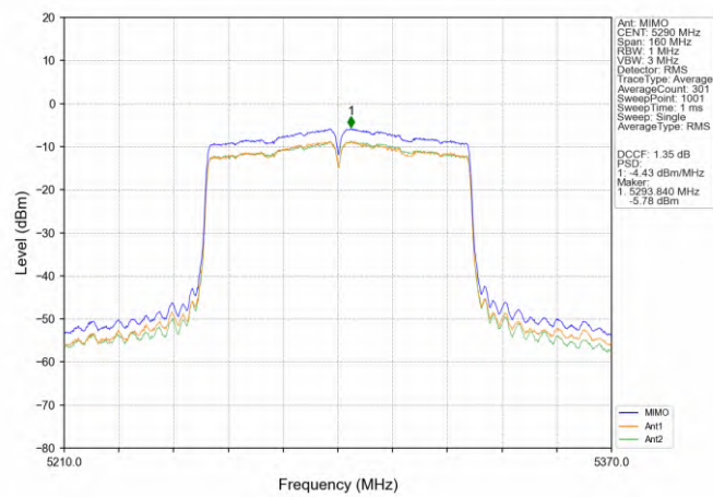
802.11ac(VHT80)_MCH_5290MHz_MIMO_NTNV
