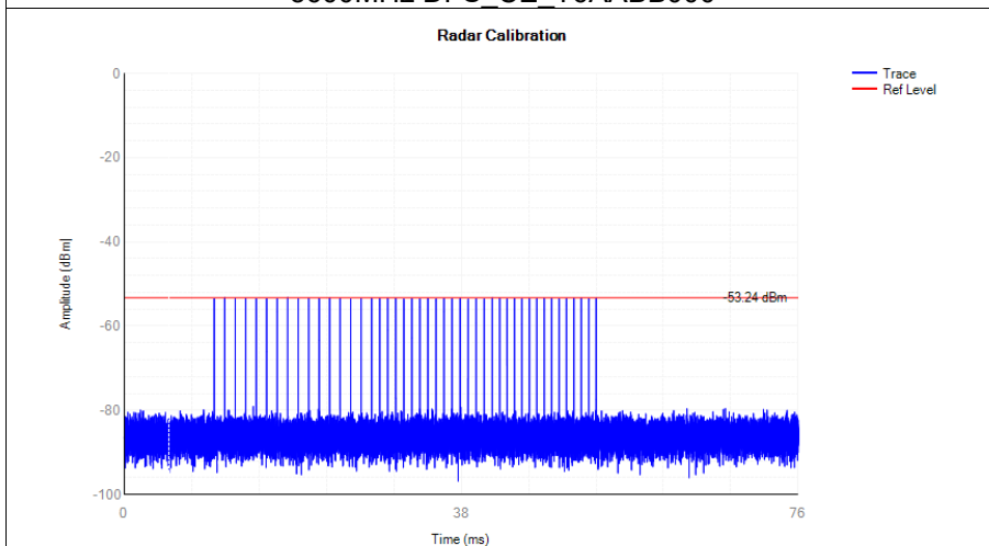
5600MHz DFS_CE_T6ABAB000
