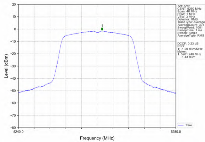
802.11n(HT20)_LCH_5260MHz_MIMO_NTNV
