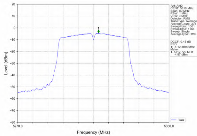
802.11n(HT40)_HCH_5310MHz_MIMO_NTNV
