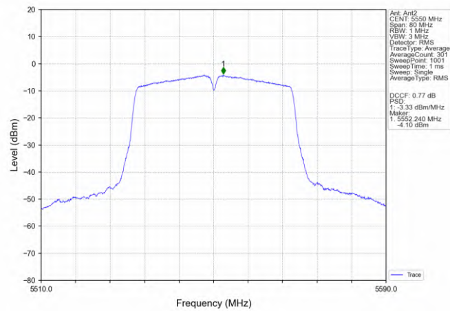
802.11ac(VHT40)_MCH_5550MHz_MIMO_NTNV
