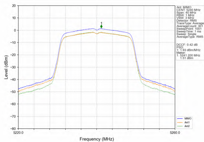
802.11ac(VHT20)_HCH_5240MHz_MIMO_NTNV
