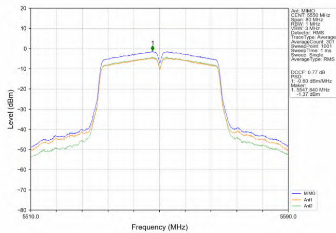
802.11ac(VHT40)_MCH_5550MHz_MIMO_NTNV
