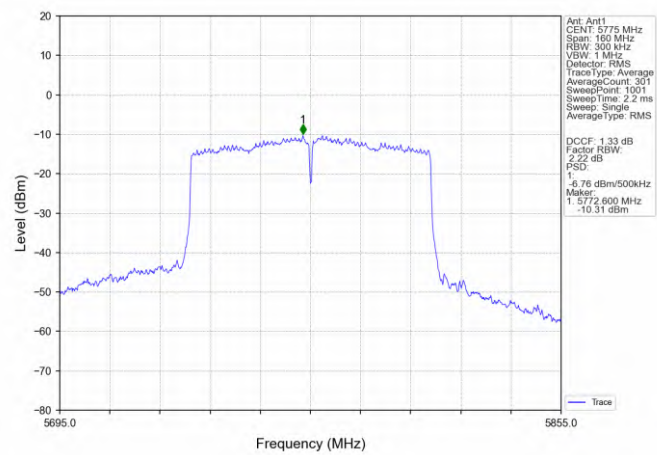
802.11ac(VHT80)_MCH_5775MHz_Ant1_NTNV
