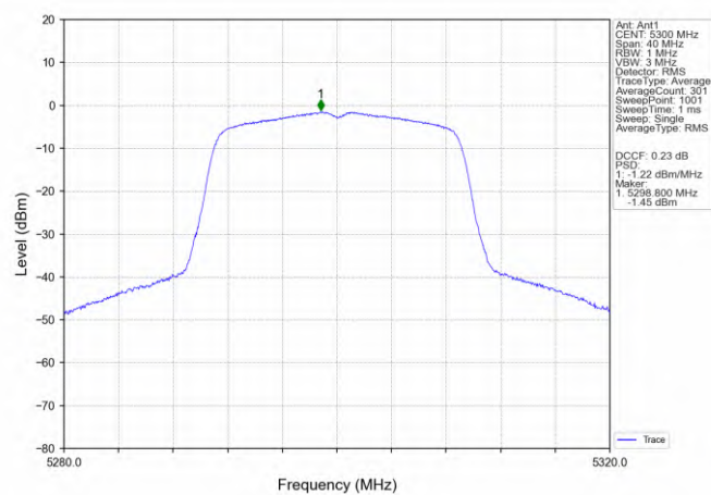
802.11n(HT20)_MCH_5300MHz_Ant1_NTNV
