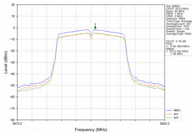
802.11ac(VHT40)_LCH_5510MHz_MIMO_NTNV
