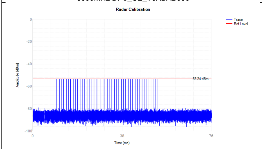
5600MHz DFS_CE_T6ABAB000
