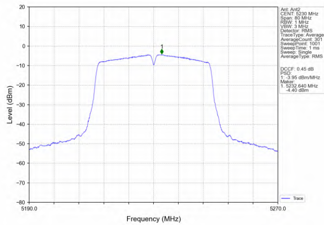
802.11n(HT40)_HCH_5230MHz_MIMO_NTNV
