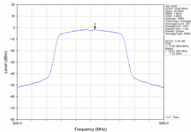
802.11ac(VHT20)_HCH_5240MHz_MIMO_NTNV
