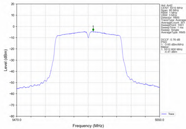
802.11ac(VHT40)_LCH_5510MHz_MIMO_NTNV
